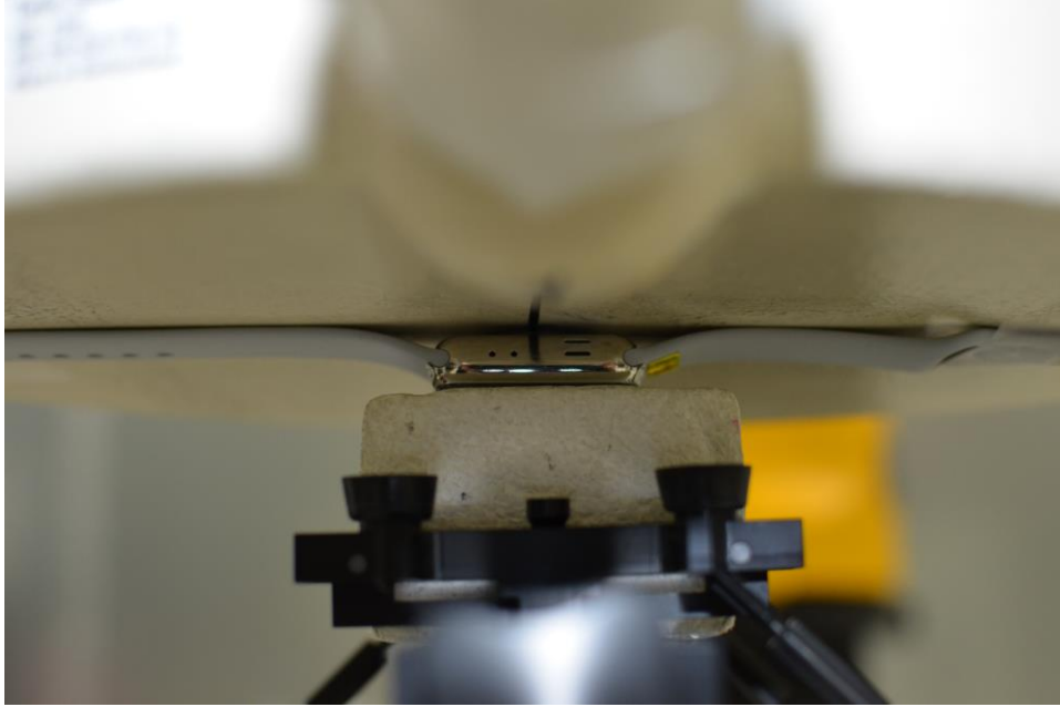
SAR Test Setup Photo 15: Stainless Steel with Sport wrist band, Back side at 0.0 cm
