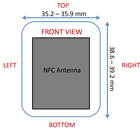
Figure F-2 NFC Antenna Location
