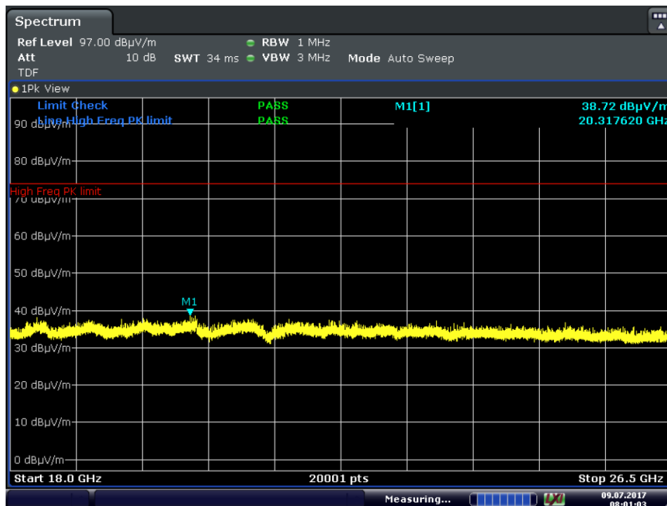
Plot 7-32. Radiated Spurious Plot above 18GHz (GFSK ePA, Pol. H)
