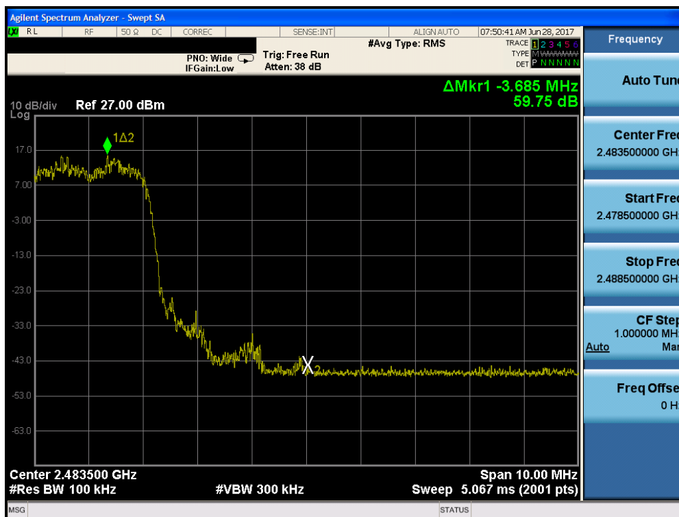
Plot 7-36. Band Edge Plot (Bluetooth with Hopping Enabled, 8DPSK, ePA - Ch.78)
