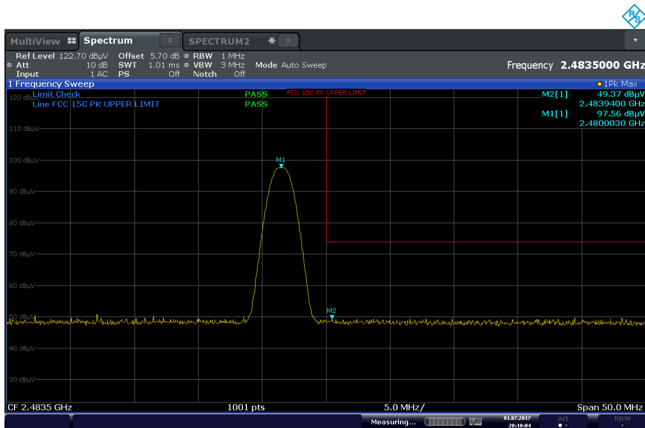
Plot 7-71. Radiated Restricted Upper Band Edge Measurement (Peak)
