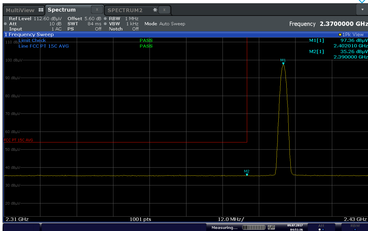
Plot 7-66. Radiated Restricted Lower Band Edge Measurement (Average)
