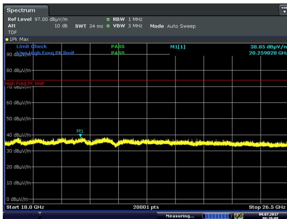
Plot 7-65. Radiated Spurious Plot above 18GHz (GFSK ePA, Pol. V)
