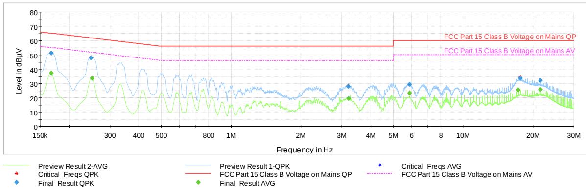
Plot 7-75. Line-Conducted Test Plot (L1)
