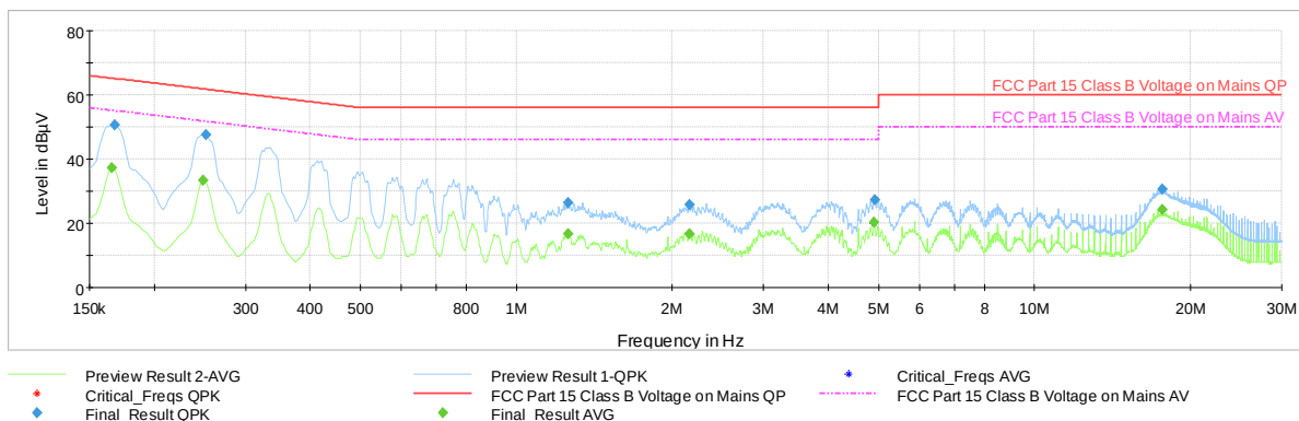
Plot 7-76. Line-Conducted Test Plot (N)
