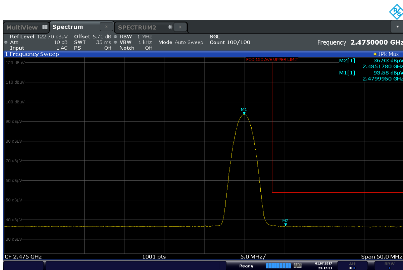
Plot 7-72. Radiated Restricted Upper Band Edge Measurement (Average)
