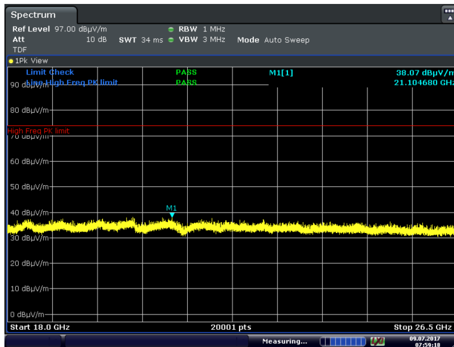
Plot 7-64. Radiated Spurious Plot above 18GHz (GFSK ePA, Pol. H)
