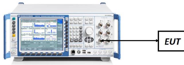
Figure 7-4. EIRP Measurement Setup
