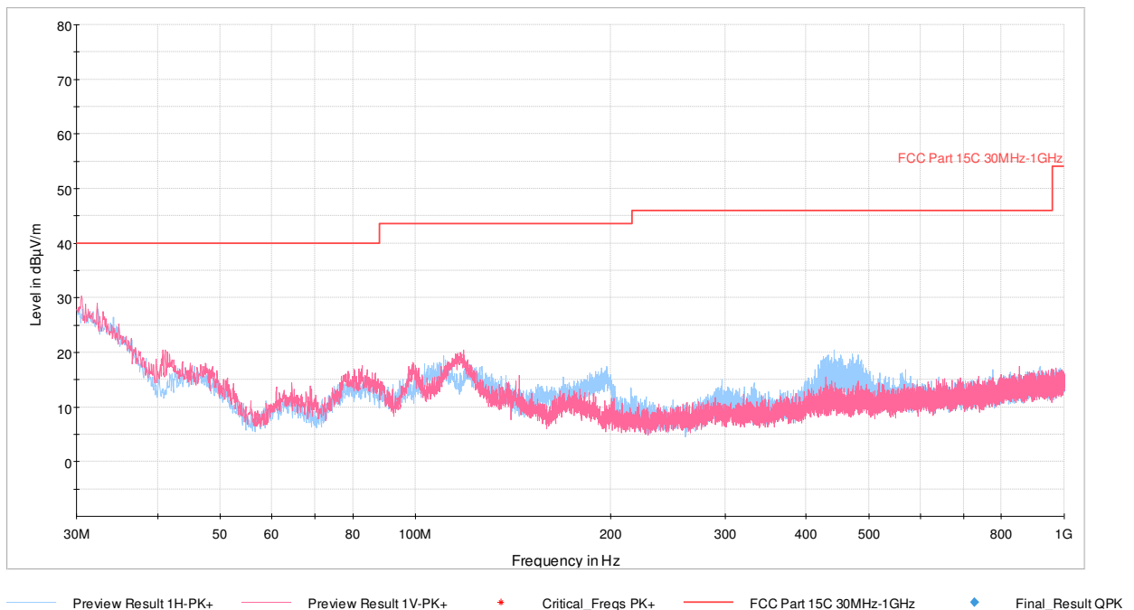
Plot 7-2. Radiated Spurious Plot 30MHz – 1GHz (CE A 848kbps, Pol. X)
