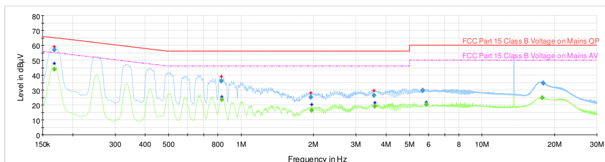
Plot 7-3. Line-Conducted Test Plot (L1)
