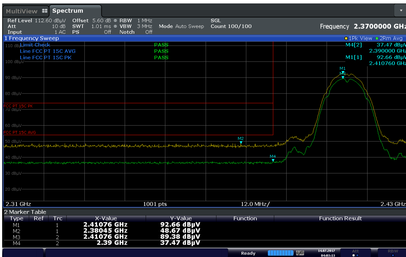
Plot 7-42. Radiated Restricted Lower Band Edge Measurement (Average & Peak)
