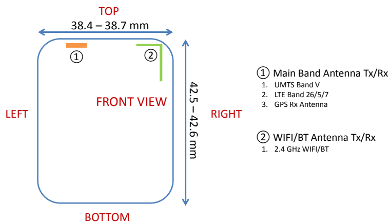
Figure F-1 DUT Antenna Locations
