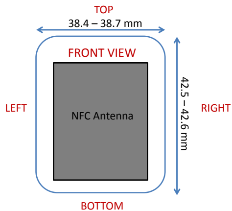
Figure F-2 NFC Antenna Location
