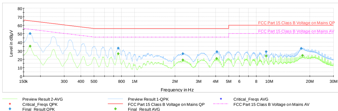
Plot 7-39. Line Conducted Plot with Bluetooth LE (GFSK ePA, L1)
