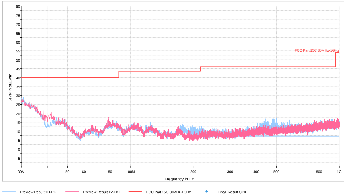
Plot 7-38. Radiated Spurious Plot below 1GHz (GFSK ePA, Pol. H & V)
