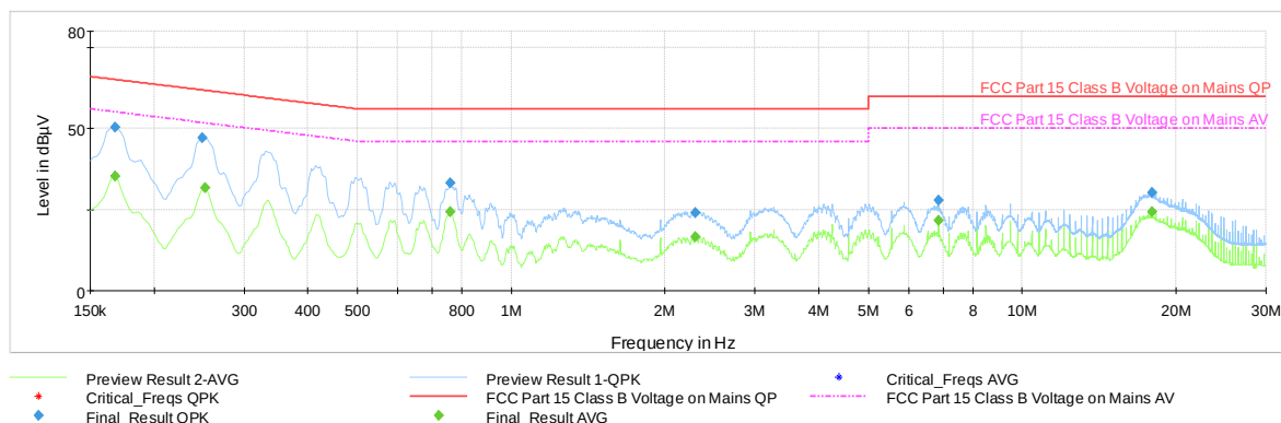
Plot 7-40. Line Conducted Plot with Bluetooth LE (GFSK ePA, N)
