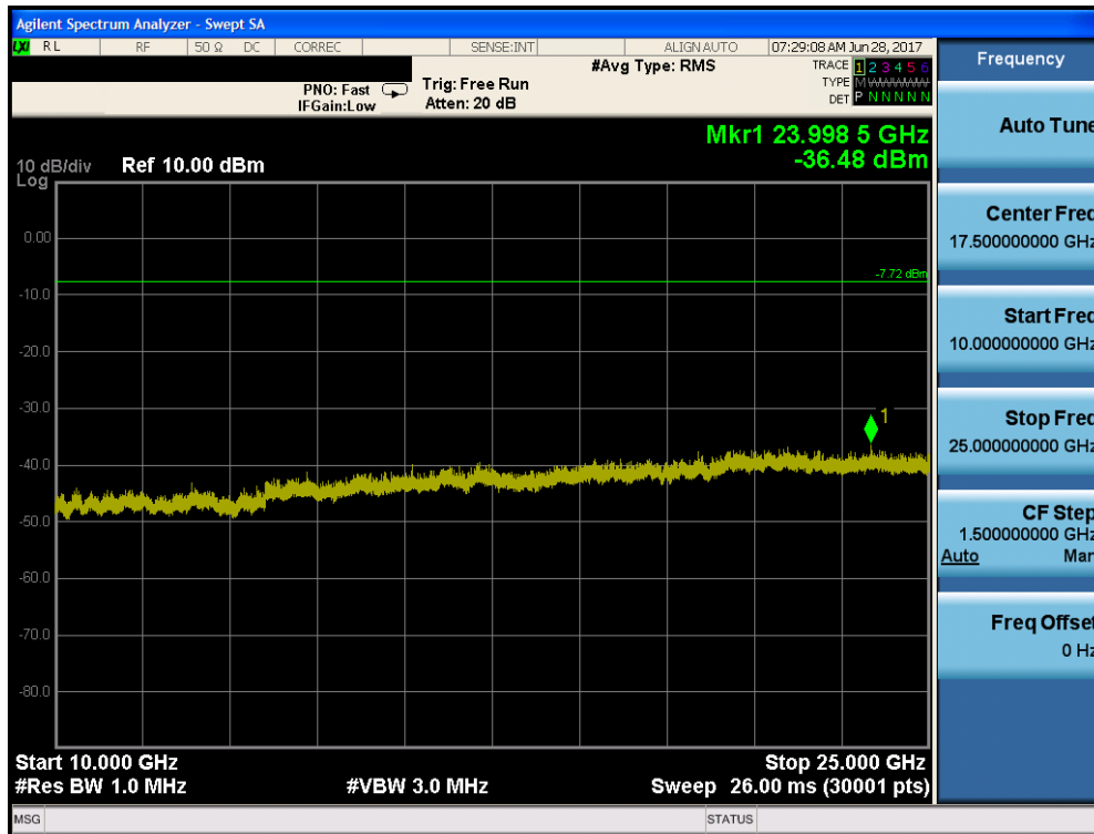
Plot 7-56. Conducted Spurious Plot (Bluetooth, 8DPSK, ePA – Ch. 0)
