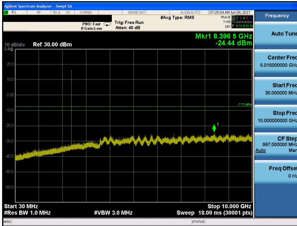
Plot 7-55. Conducted Spurious Plot (Bluetooth, 8DPSK, ePA – Ch. 0)
