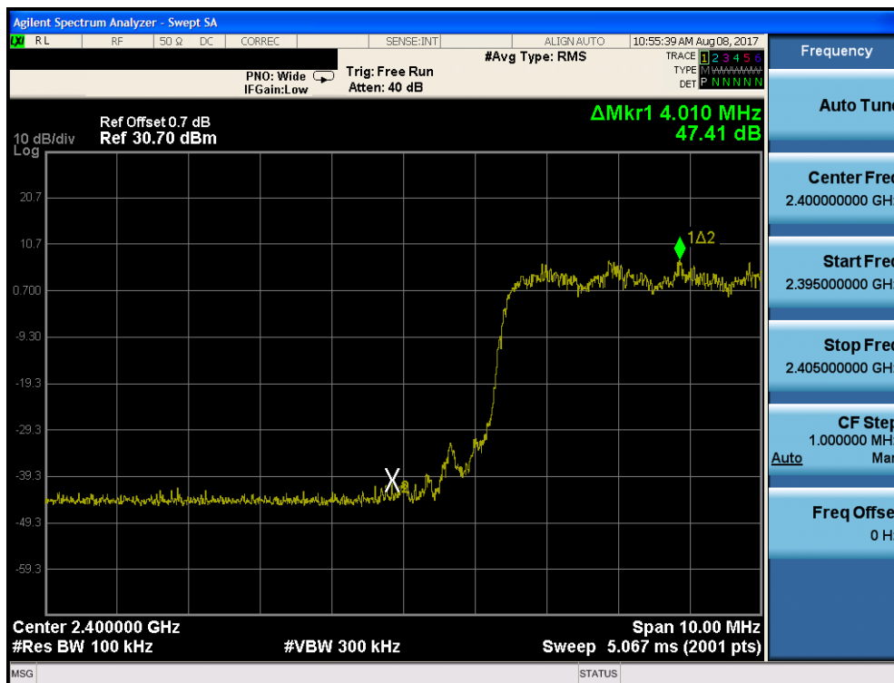
Plot 7-19. Band Edge Plot (Bluetooth with Hopping Enabled, \pi/4 DQPSK – Ch. 0)
