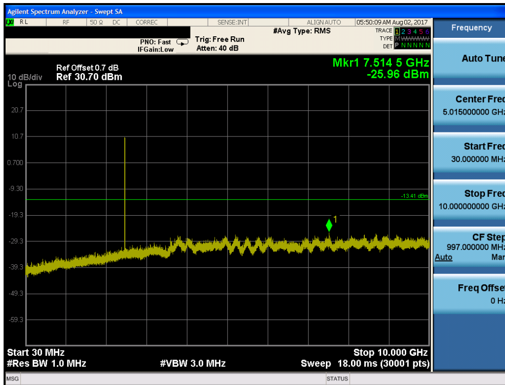
Plot 7-39. Conducted Spurious Plot (Bluetooth, \pi/4 DQPSK – Ch. 78)
