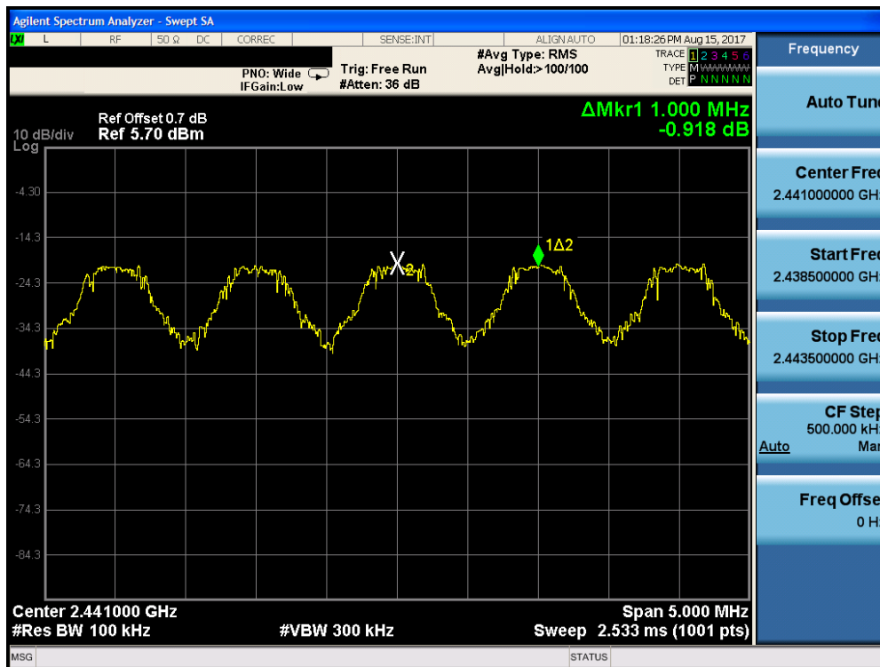
Plot 7-21. Channel Spacing Plot (Bluetooth, GFSK)
