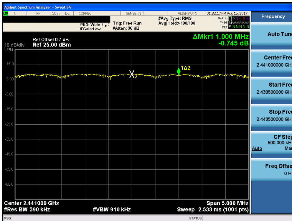
Plot 7-22. Channel Spacing Plot (Bluetooth, \pi/4 DQPSK )
