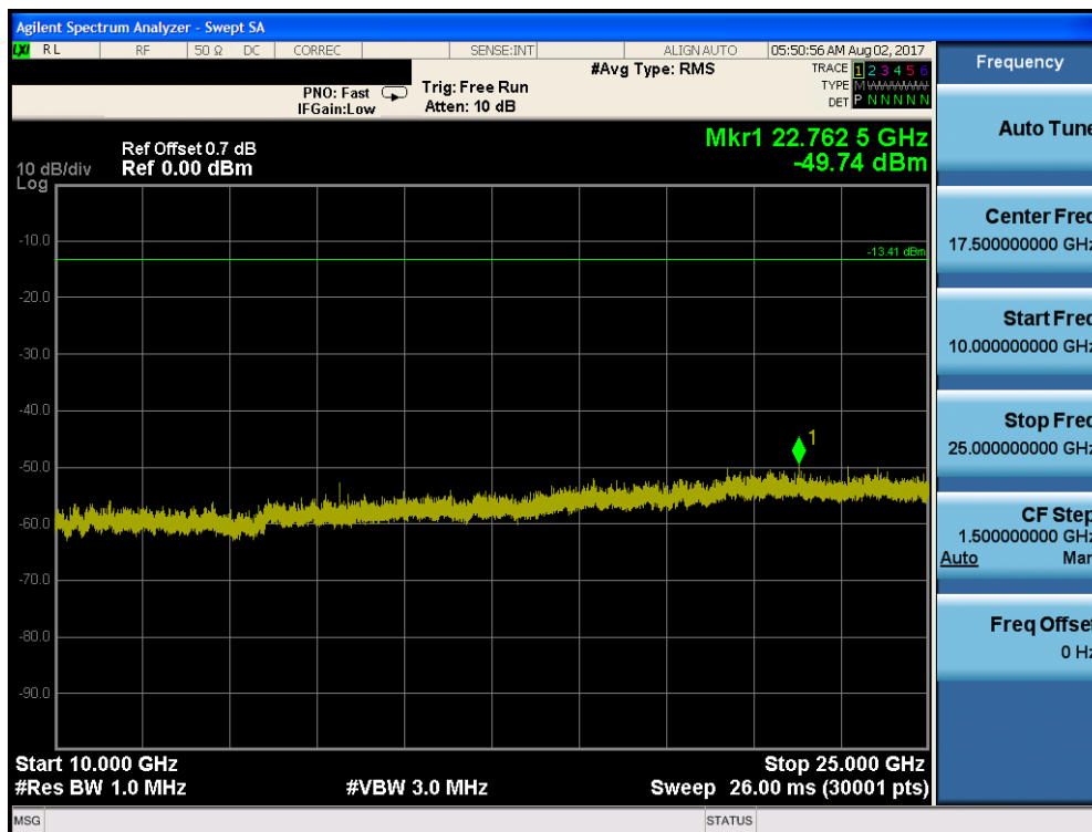
Plot 7-40. Conducted Spurious Plot (Bluetooth, \pi/4 DQPSK – Ch. 78)
