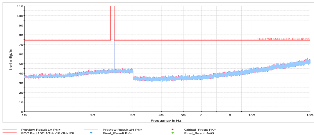
Plot 7-43. Radiated Spurious Plot above 1GHz (BT – Ch. 78, Ant. Pol. H & V)
