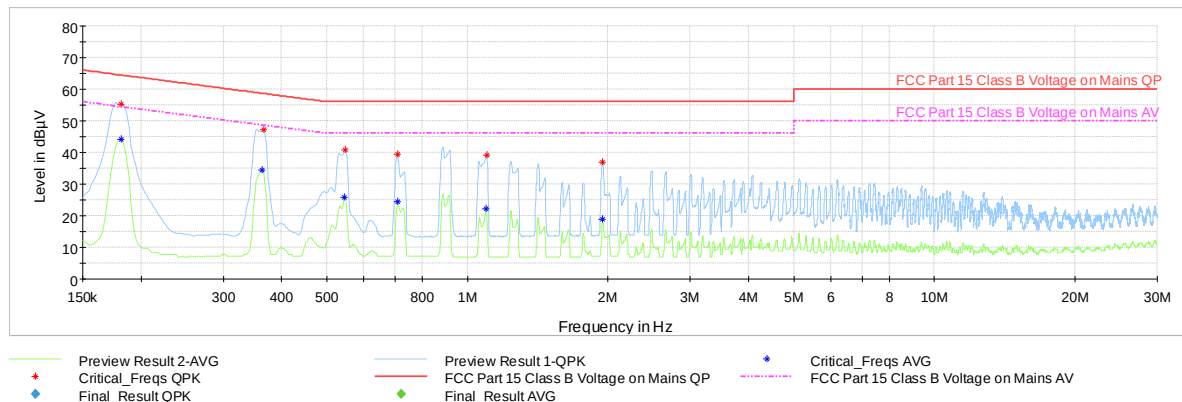
Plot 7-55. Line-Conducted Test Plot with AC Adapter (L1)
