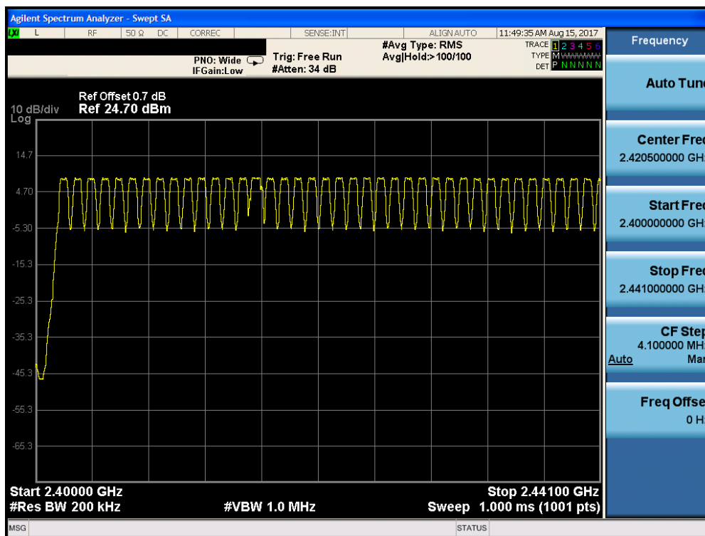
Plot 7-25. Low End Spectrum Channel Hopping Plot (Bluetooth, GFSK)
