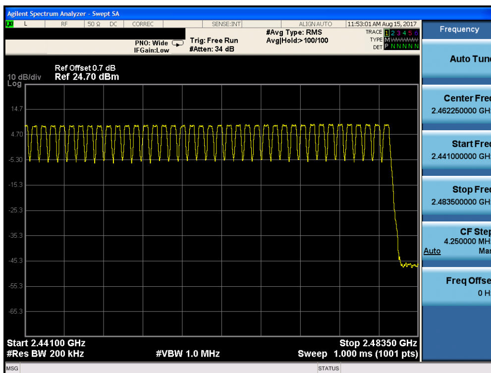
Plot 7-26. High End Spectrum Channel Hopping Plot (Bluetooth, GFSK)
