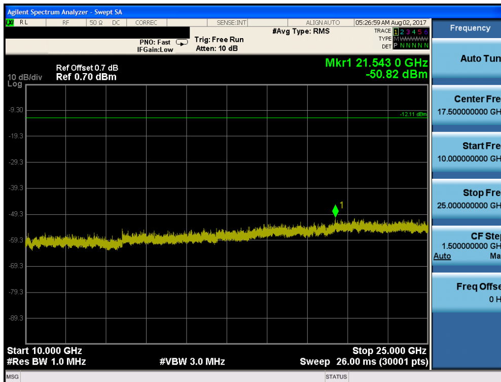
Plot 7-30. Conducted Spurious Plot (Bluetooth, GFSK – Ch. 0)
