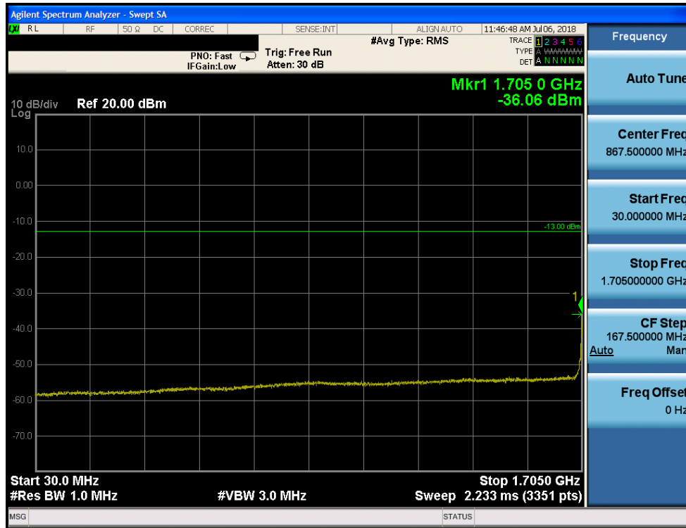
Plot 7-13. Conducted Spurious Plot (AWS WCDMA Mode - Low Channel)
