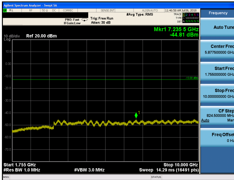
Plot 7-14. Conducted Spurious Plot (AWS WCDMA Mode - Low Channel)
