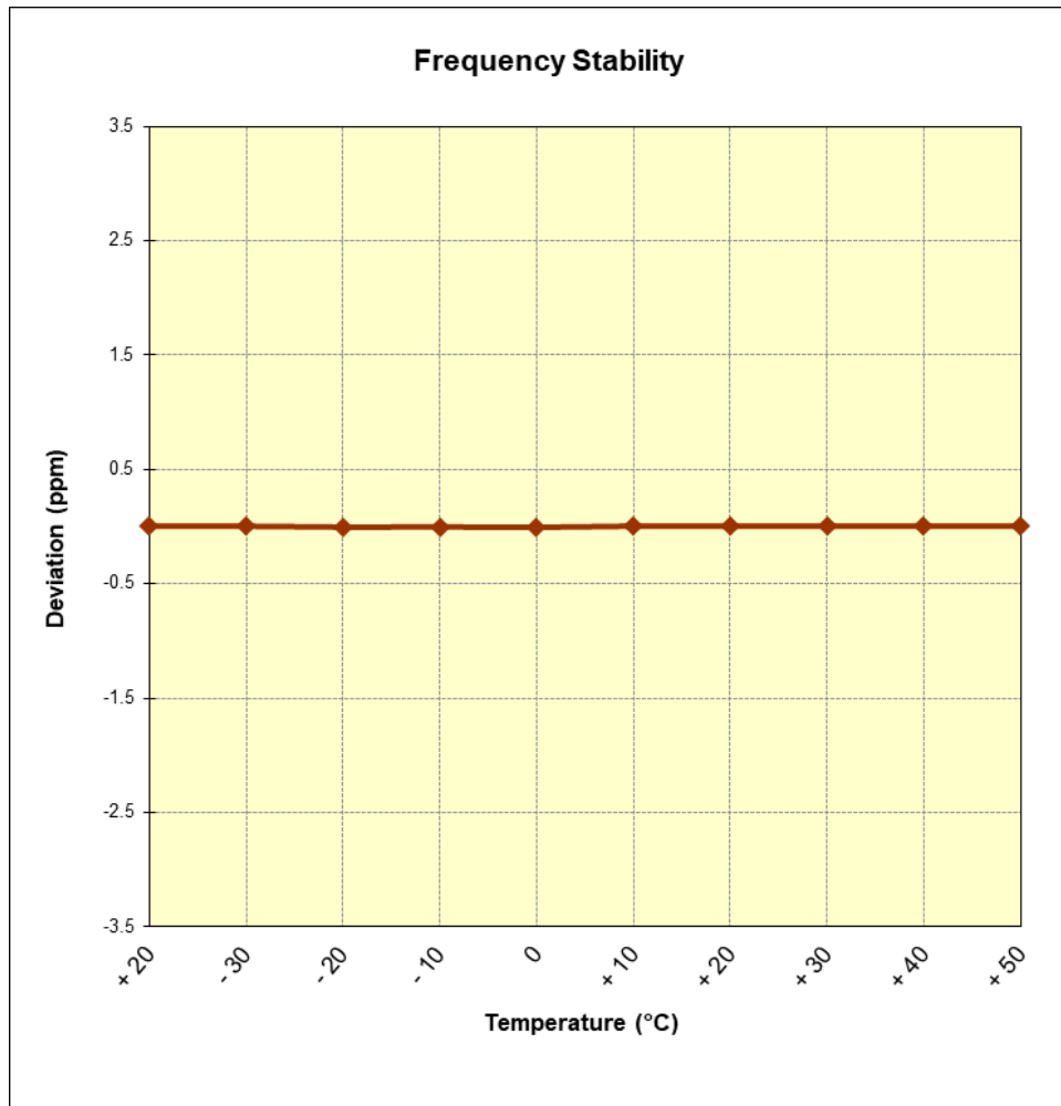
Figure 7-9. Frequency Stability Graph (PCS WCDMA Mode – Ch. 9400)
