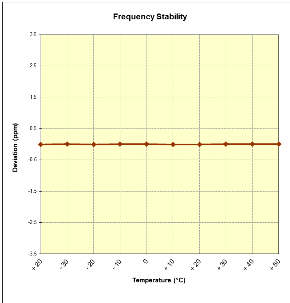
Figure 7-8. Frequency Stability Graph (AWS WCDMA Mode – Ch. 1413)
