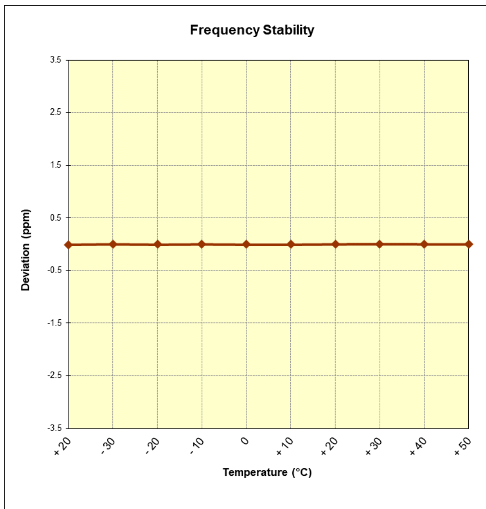
Figure 7-7. Frequency Stability Graph (Cellular WCDMA Mode – Ch. 4183)
