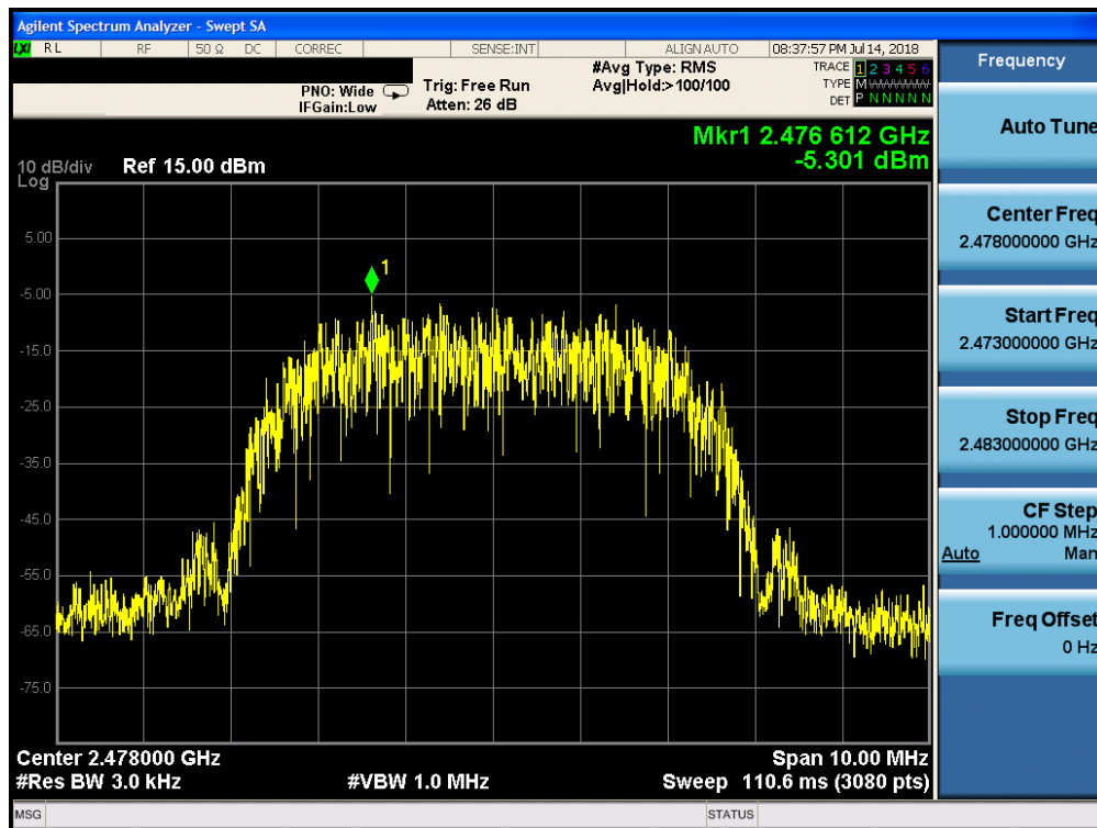
Plot 7-21. Power Spectral Density Plot (Bluetooth (HDR, ePA), 8Mbps – Ch. 75)
