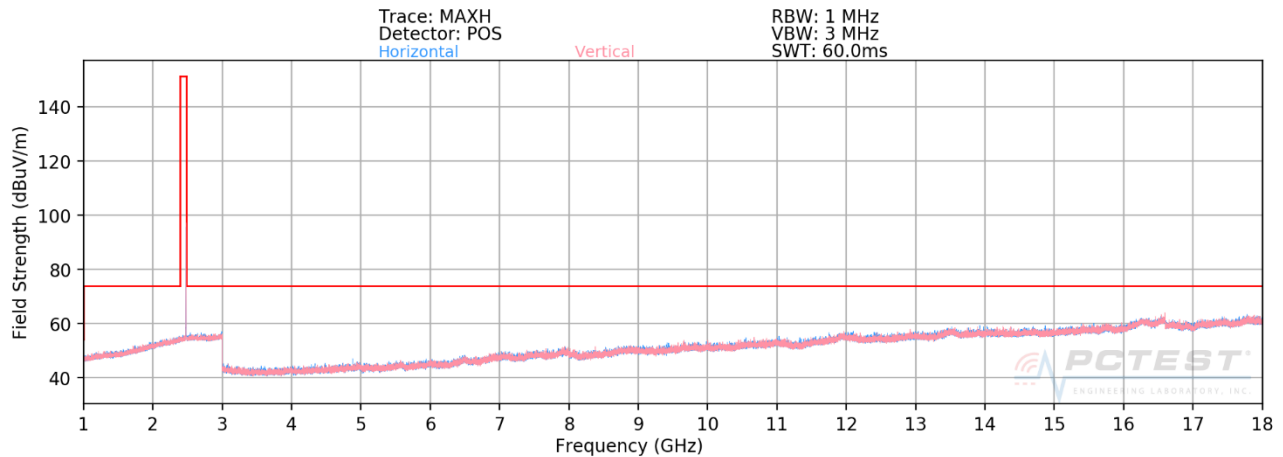
Plot 7-50. Radiated Spurious Plot (HDR8, ePA – Ch. 75, Ant. Pol. H & V)
