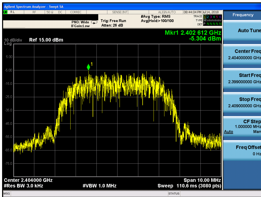
Plot 7-22. Power Spectral Density Plot (Bluetooth (HDR, iPA), 8Mbps – Ch. 1)
