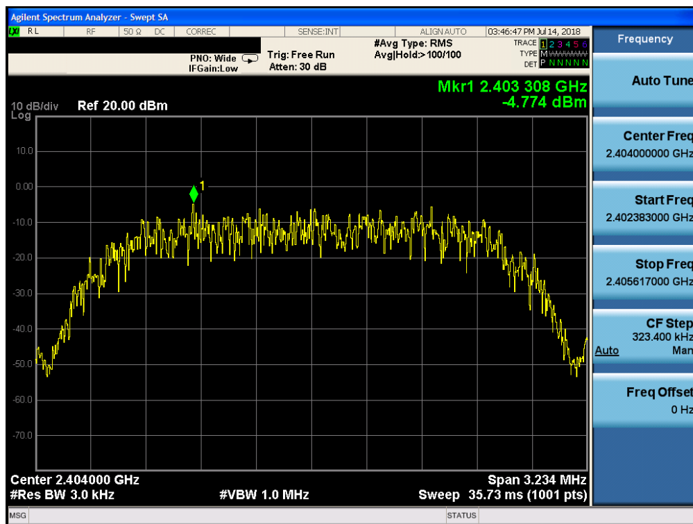
Plot 7-13. Power Spectral Density Plot (Bluetooth (HDR, ePA), 4Mbps – Ch. 1)
