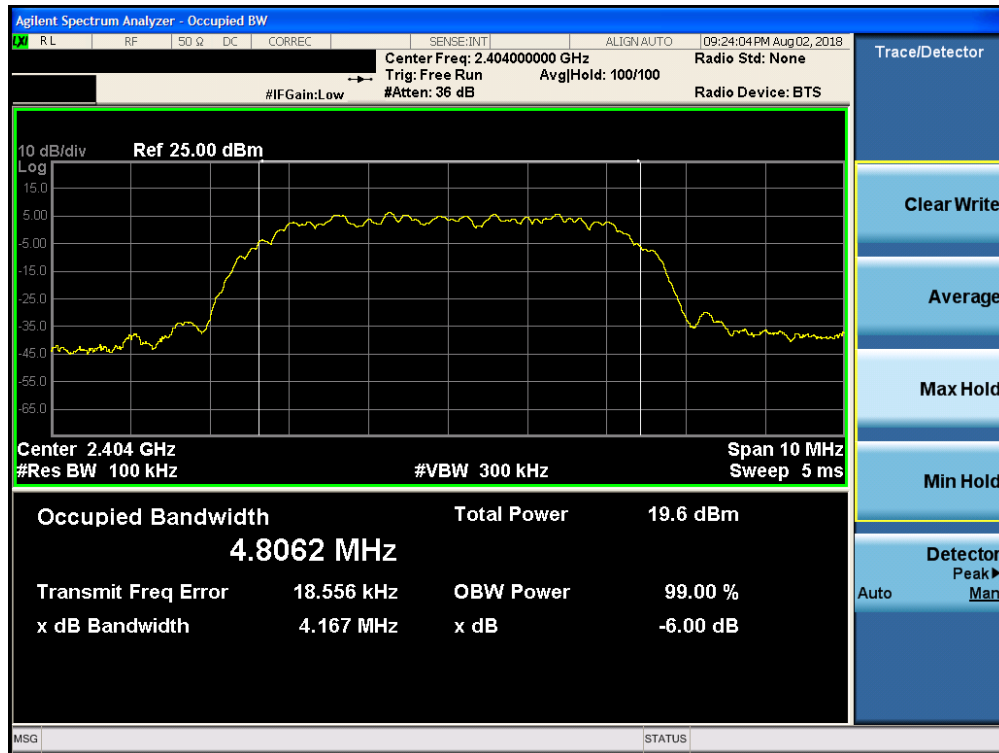
Plot 7-7. 6dB Bandwidth Plot (Bluetooth (HDR, ePA), 8Mbps – Ch. 1)
