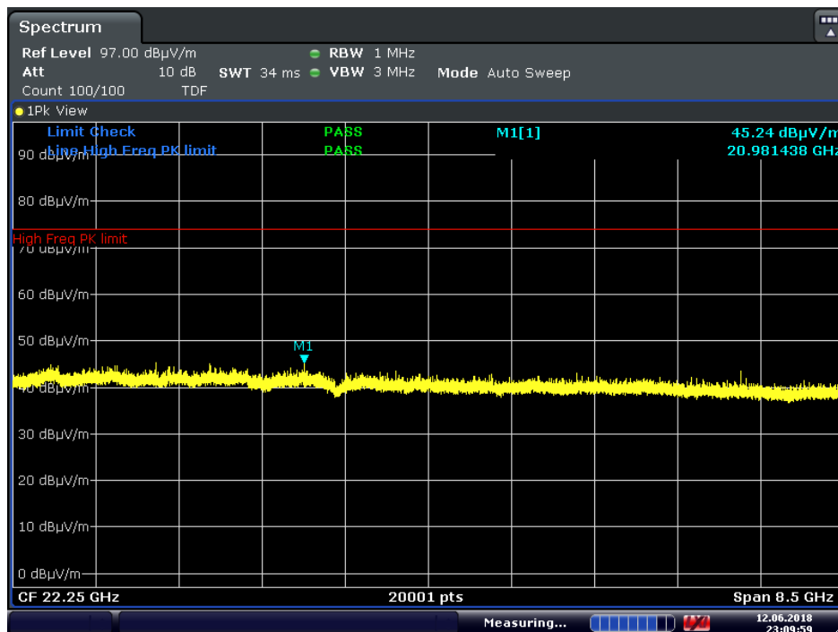
Plot 7-51. Radiated Spurious Plot above 18GHz (HDR8, ePA, Pol. H)
