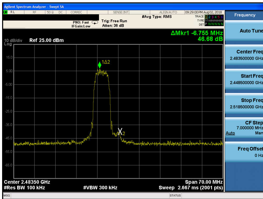
Plot 7-30. Band Edge Plot (Bluetooth (HDR, ePA), 8Mbps – Ch. 75)
