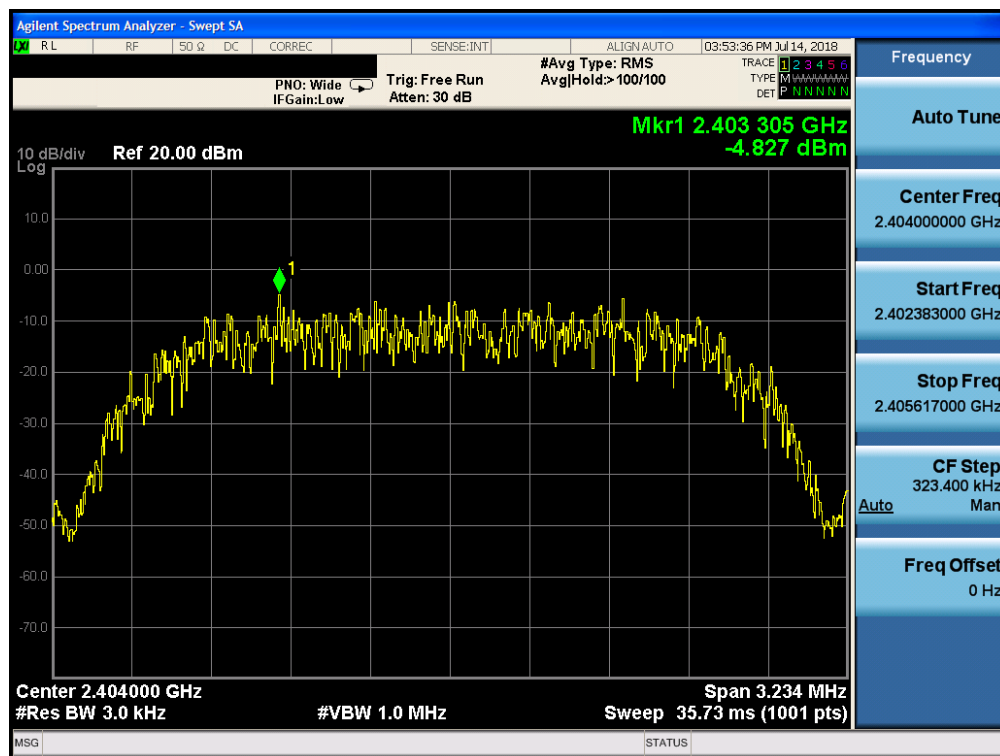
Plot 7-16. Power Spectral Density Plot (Bluetooth (HDR, iPA), 4Mbps – Ch. 1)
