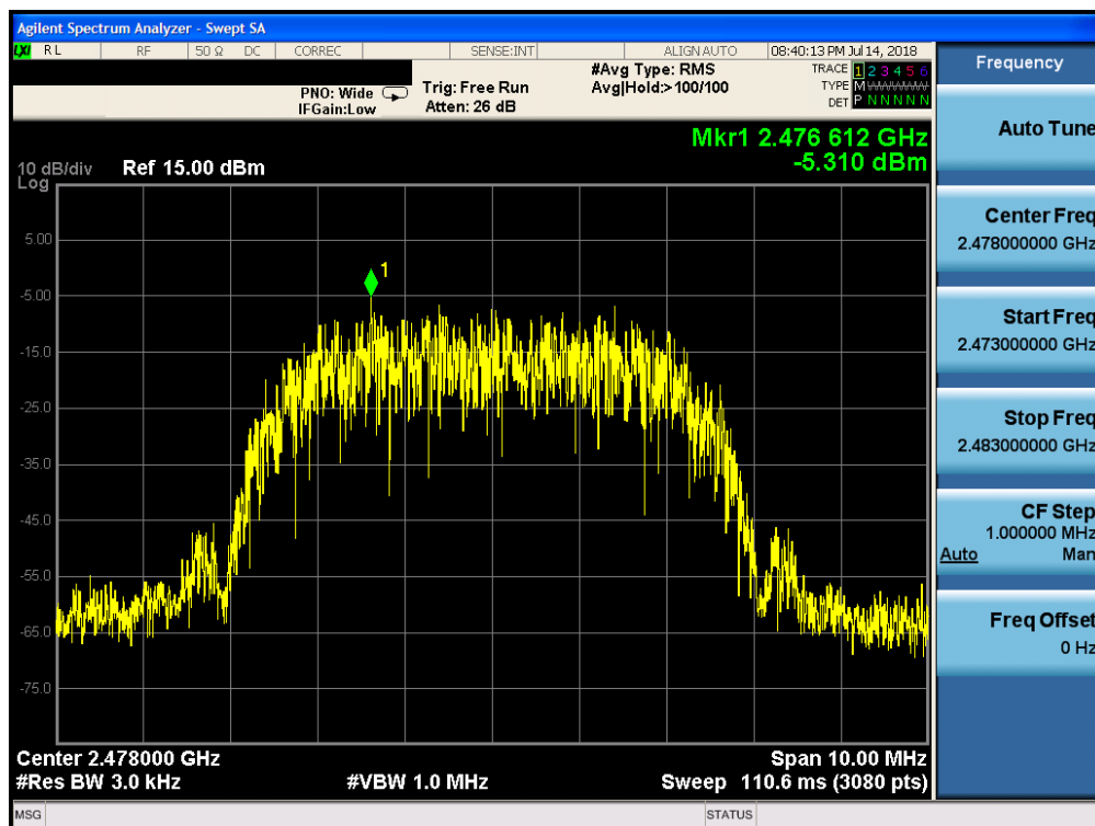
Plot 7-24. Power Spectral Density Plot (Bluetooth (HDR, iPA), 8Mbps – Ch. 75)
