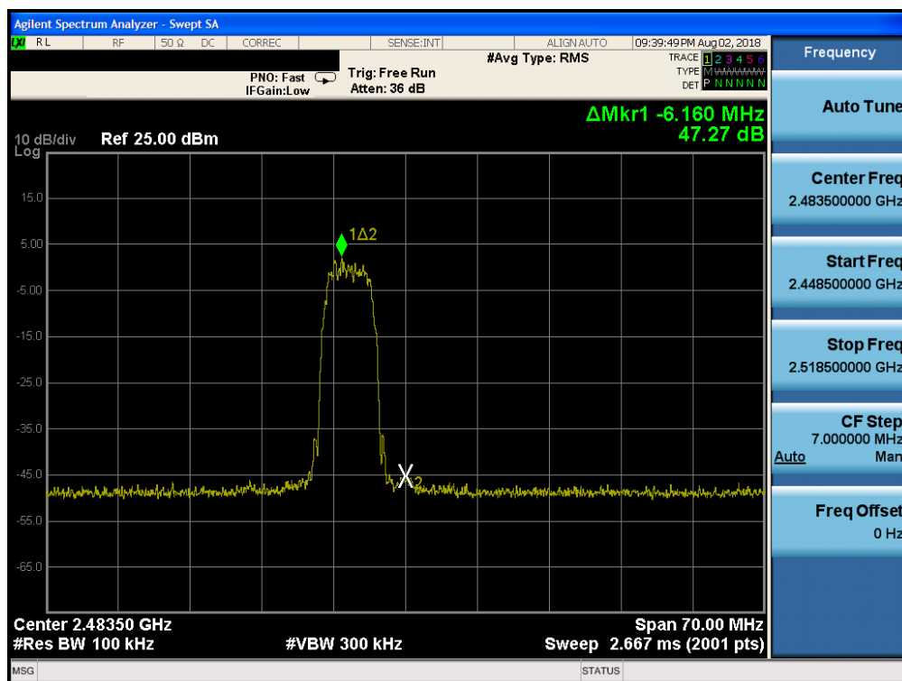
Plot 7-32. Band Edge Plot (Bluetooth (HDR, iPA), 8Mbps – Ch. 75)
