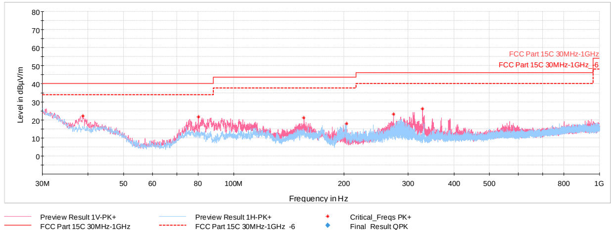
Plot 7-57. Radiated Spurious Plot below 1GHz (HDR4, ePA, Pol. H & V, with WCP + Laptop)
