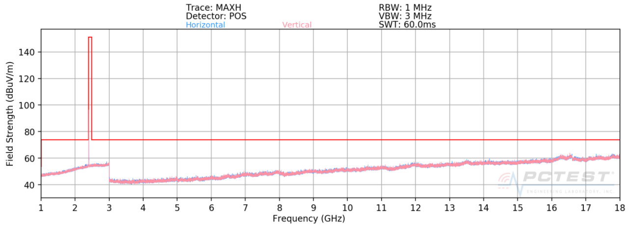
Plot 7-48. Radiated Spurious Plot (HDR8, ePA – Ch. 1, Ant. Pol. H & V)
