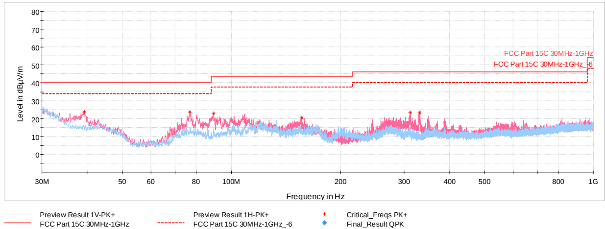
Plot 7-58. Radiated Spurious Plot below 1GHz (HDR8, ePA, Pol. H & V, with WCP + Laptop)
