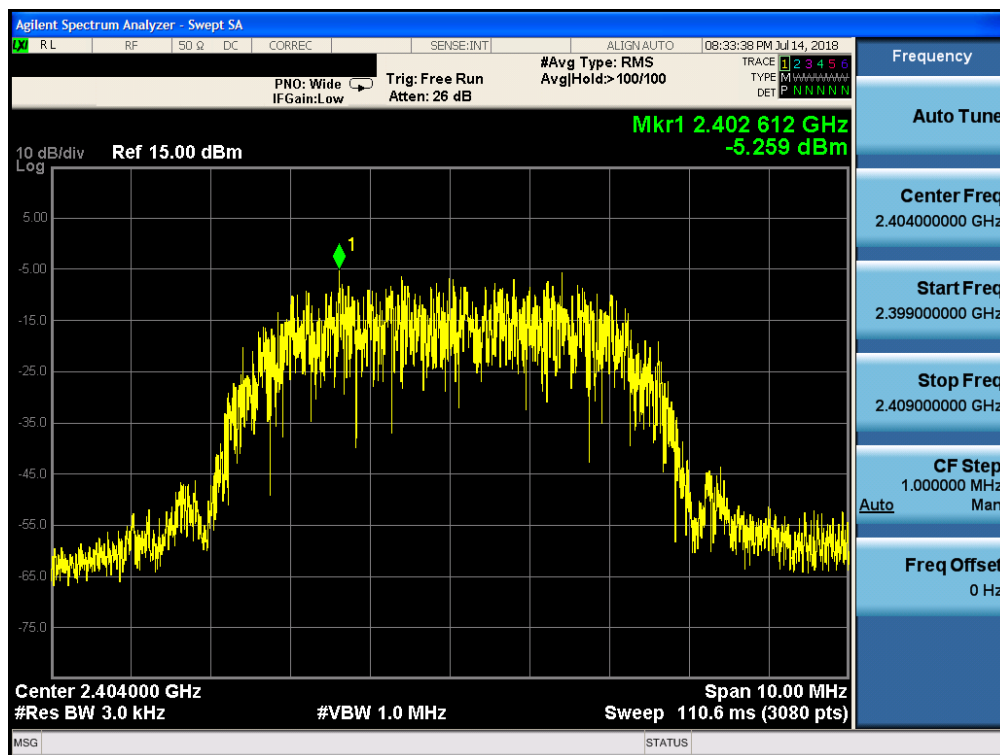
Plot 7-19. Power Spectral Density Plot (Bluetooth (HDR, ePA), 8Mbps – Ch. 1)
