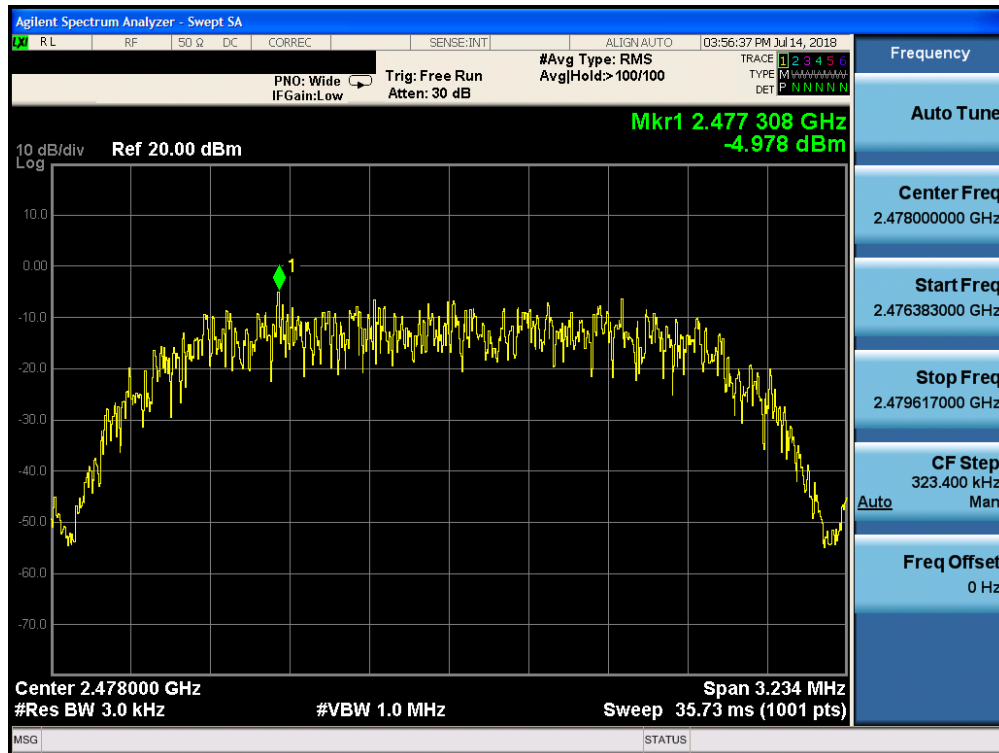
Plot 7-18. Power Spectral Density Plot (Bluetooth (HDR, iPA), 4Mbps – Ch. 75)
