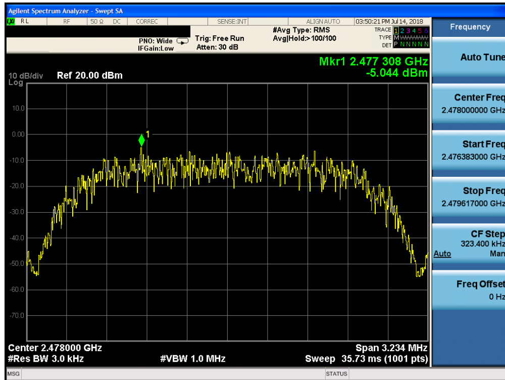
Plot 7-15. Power Spectral Density Plot (Bluetooth (HDR, ePA), 4Mbps – Ch. 75)
