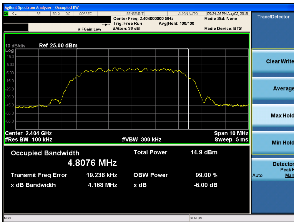
Plot 7-10. 6dB Bandwidth Plot (Bluetooth (HDR, iPA), 8Mbps – Ch. 1)
