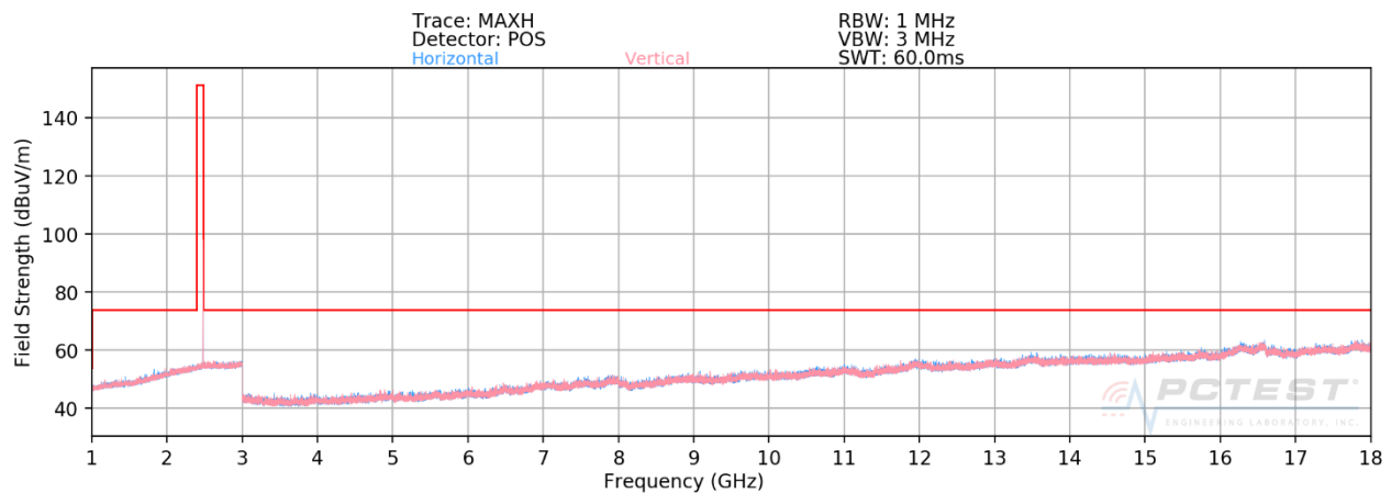
Plot 7-47. Radiated Spurious Plot (HDR4, ePA – Ch. 75, Ant. Pol. H & V)
