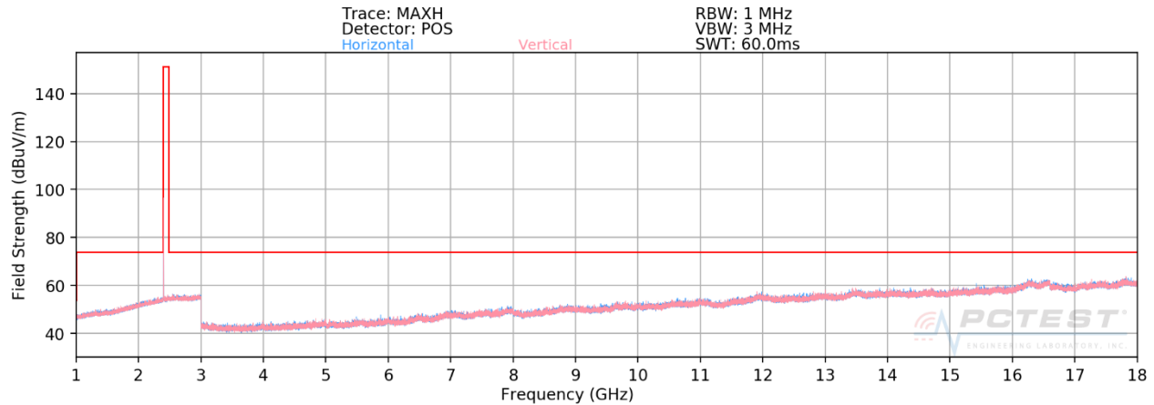
Plot 7-45. Radiated Spurious Plot (HDR4, ePA – Ch. 1, Ant. Pol. H & V)
