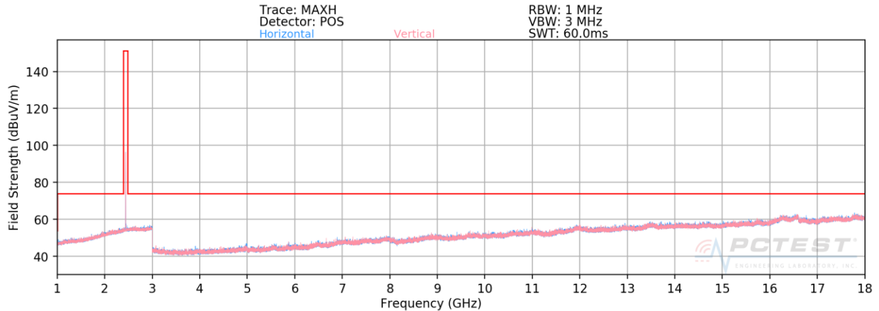
Plot 7-49. Radiated Spurious Plot (HDR8, ePA – Ch. 38, Ant. Pol. H & V)
