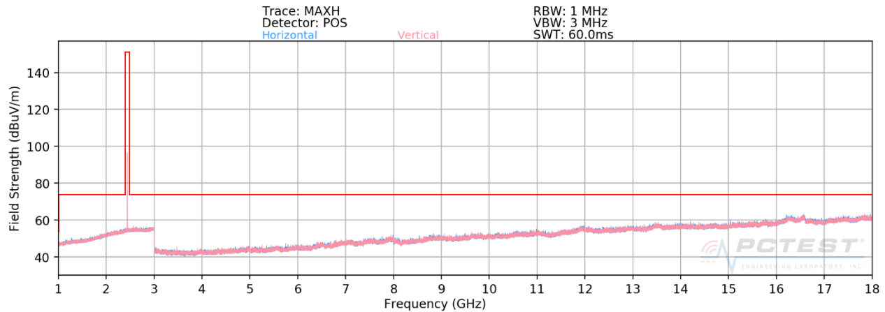
Plot 7-46. Radiated Spurious Plot (HDR4, ePA – Ch. 38, Ant. Pol. H & V)
