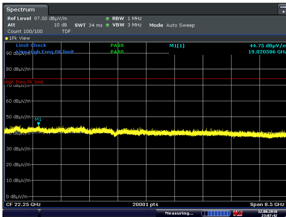
Plot 7-52. Radiated Spurious Plot above 18GHz (HDR8, ePA, Pol. V)
