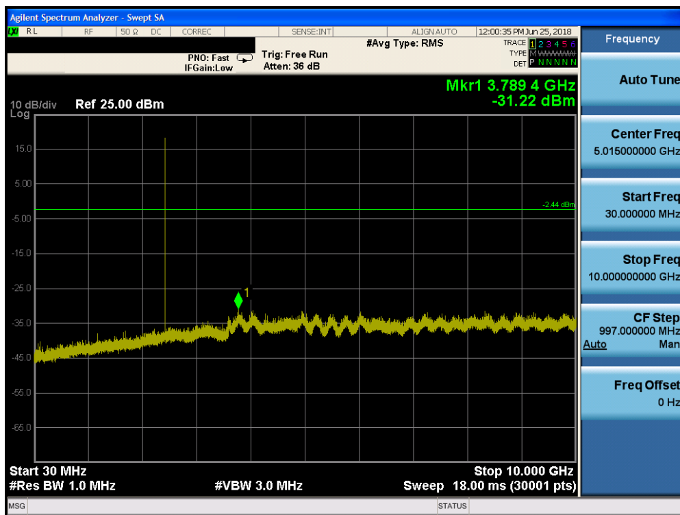
Plot 7-39. Conducted Spurious Plot (Bluetooth, GFSK, ePA – Ch. 39)
