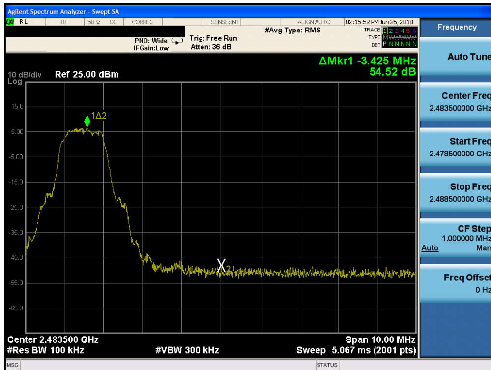
Plot 7-26. Band Edge Plot (Bluetooth with Hopping Disabled, 8DPSK, iPA – Ch. 78)
