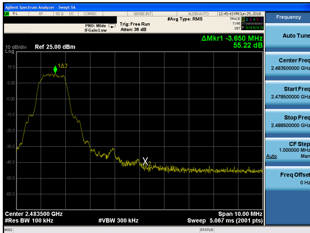
Plot 7-22. Band Edge Plot (Bluetooth with Hopping Disabled, 8DPSK, ePA – Ch. 78)
