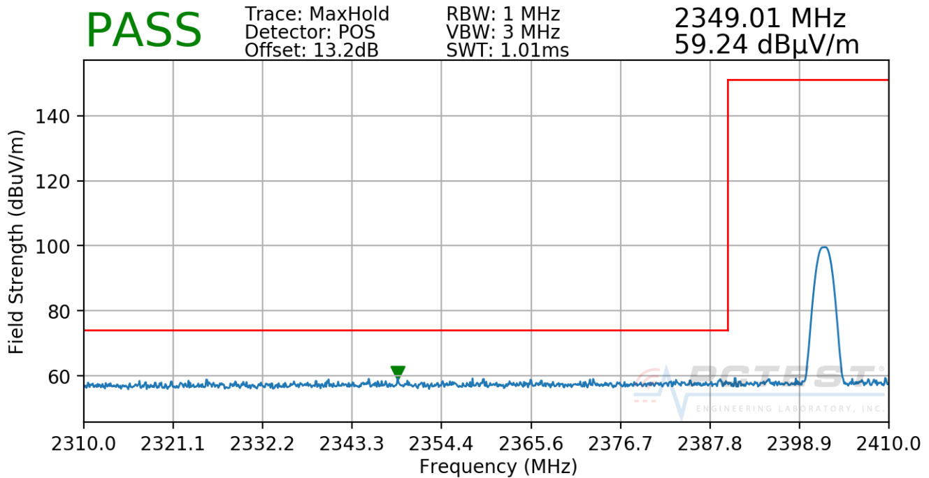
Plot 7-55. Radiated Restricted Lower Band Edge Measurement (Peak)
