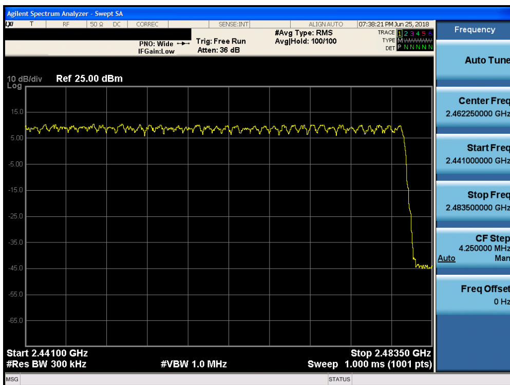
Plot 7-36. High End Spectrum Channel Hopping Plot (Bluetooth, 8DPSK, ePA)
