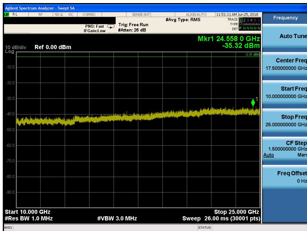
Plot 7-38. Conducted Spurious Plot (Bluetooth, GFSK, ePA – Ch. 0)
