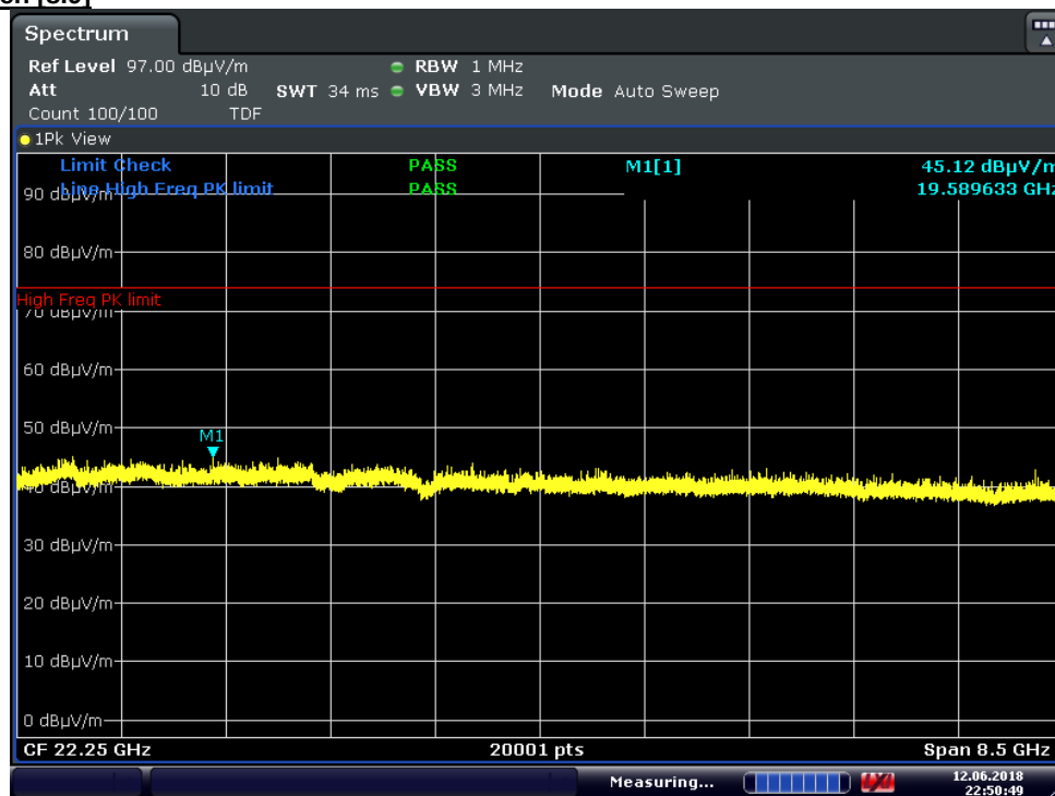
Plot 7-52. Radiated Spurious Plot above 18GHz (GFSK ePA, Ant. Pol. H)
