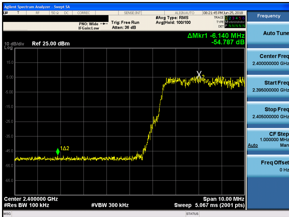
Plot 7-27. Band Edge Plot (Bluetooth with Hopping Enabled, 8DPSK, iPA – Ch. 0)
