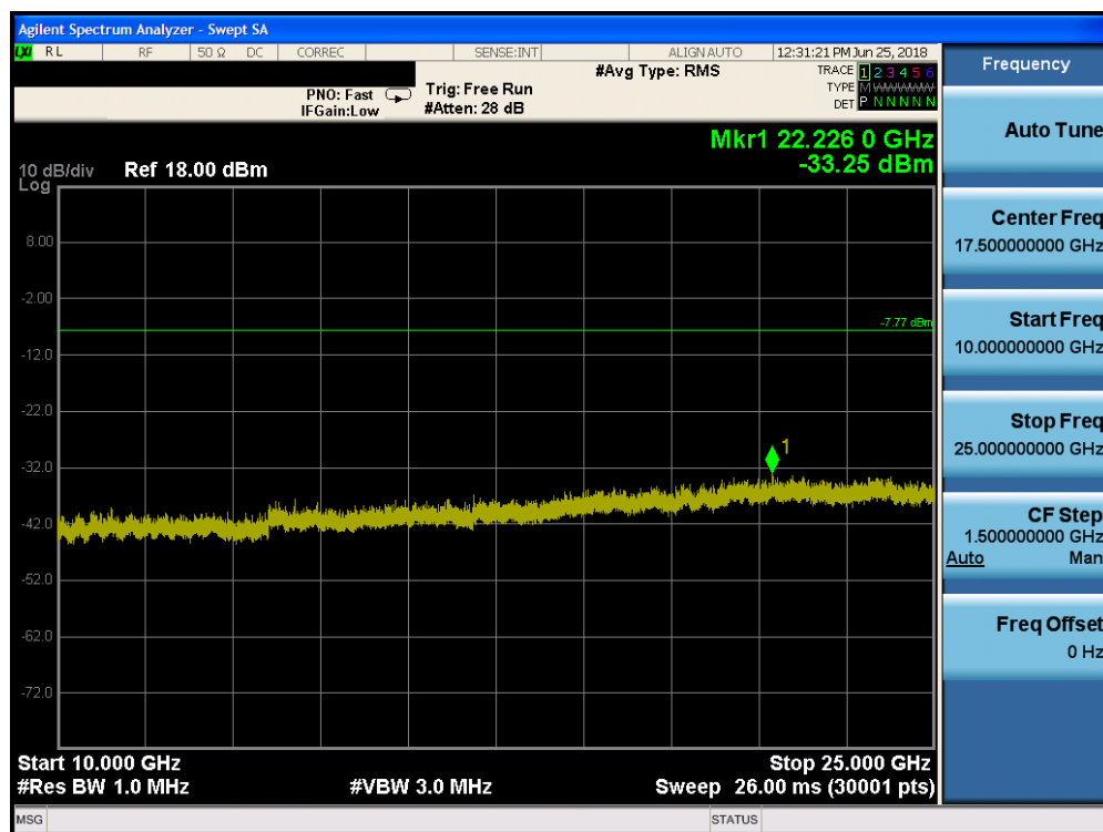
Plot 7-44. Conducted Spurious Plot (Bluetooth, 8DPSK, ePA – Ch. 0)
