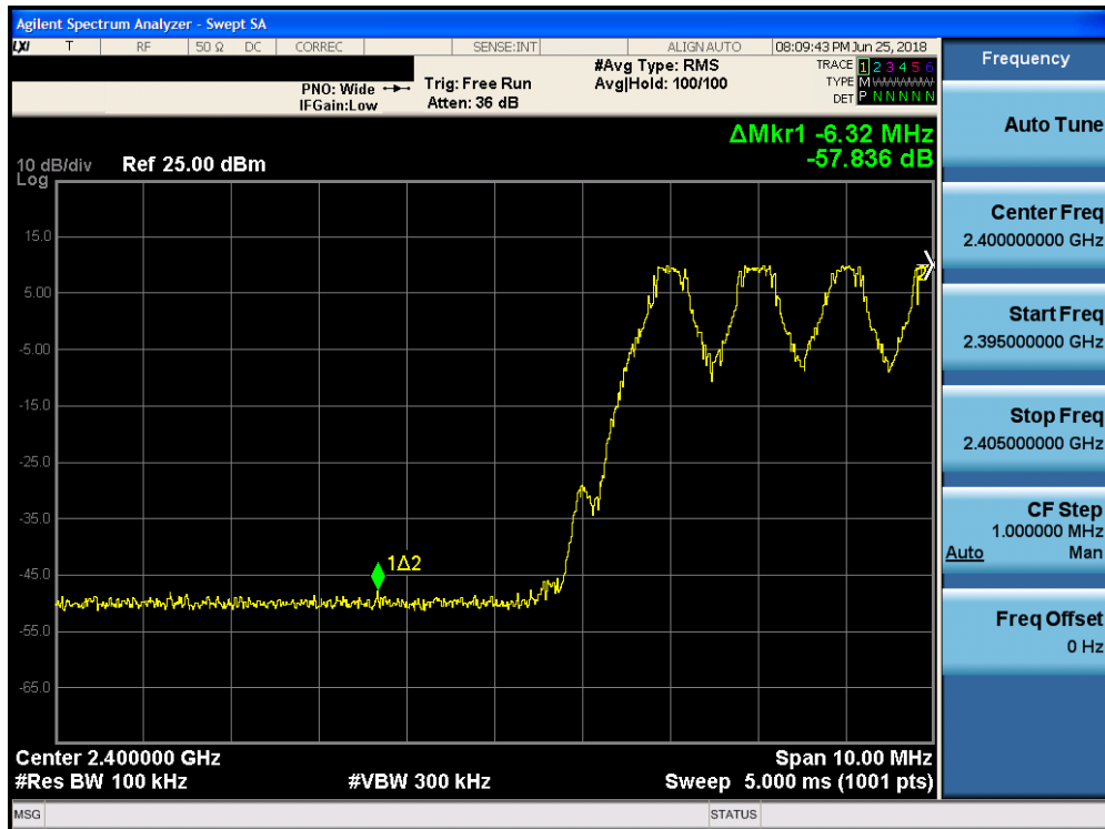
Plot 7-19. Band Edge Plot (Bluetooth with Hopping Enabled, GFSK, iPA – Ch. 0)
