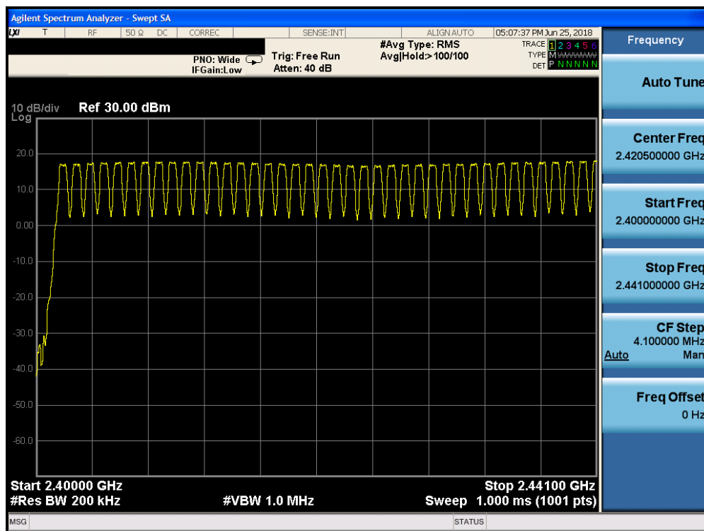
Plot 7-33. Low End Spectrum Channel Hopping Plot (Bluetooth, GFSK, ePA)
