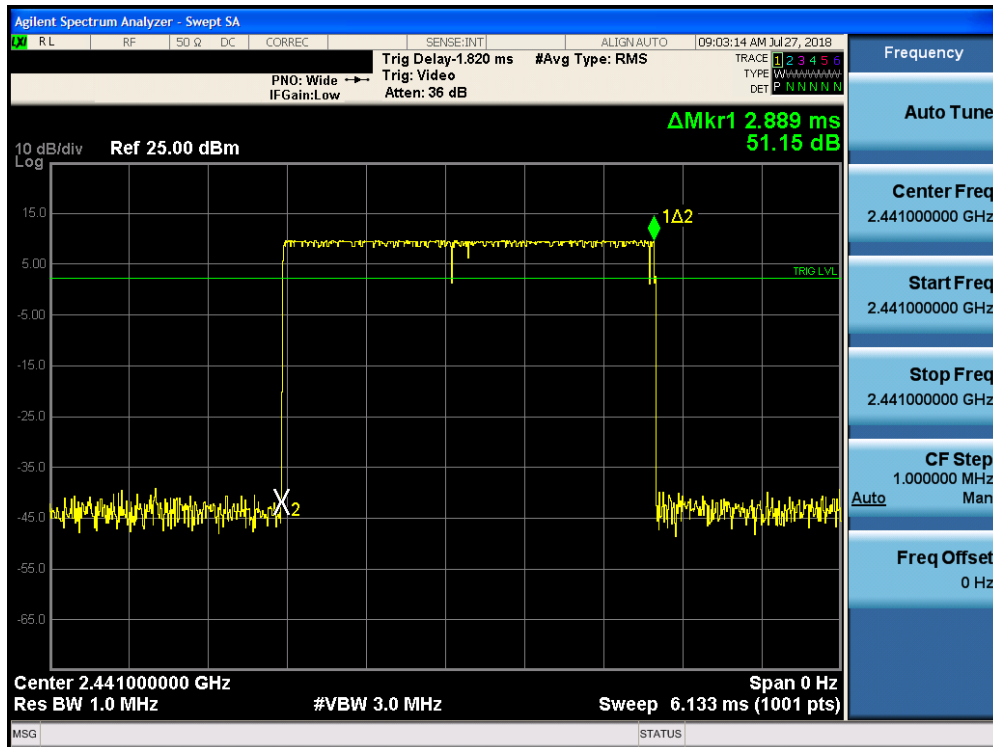
Plot 7-31. Time of Occupancy Plot (Bluetooth, GFSK, ePA)
