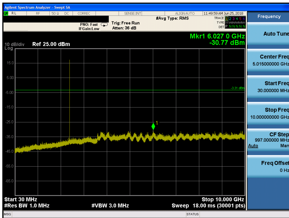
Plot 7-37. Conducted Spurious Plot (Bluetooth, GFSK, ePA – Ch. 0)
