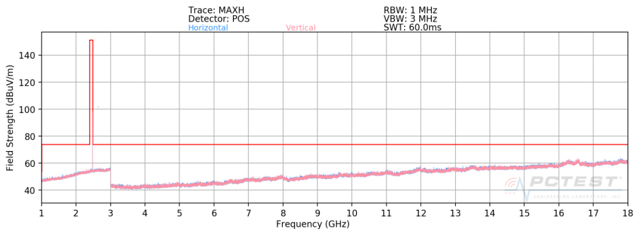
Plot 7-51. Radiated Spurious Plot above 1GHz (BT GFSK ePA – Ch. 78)
