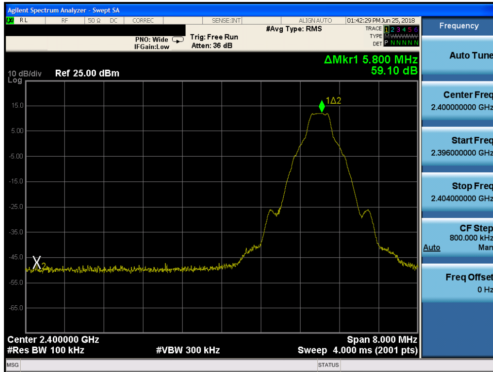
Plot 7-17. Band Edge Plot (Bluetooth with Hopping Disabled, GFSK, iPA – Ch. 0)
