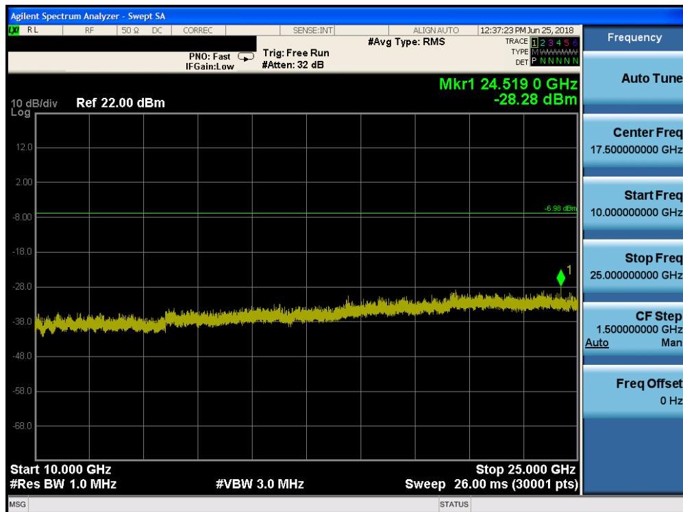
Plot 7-46. Conducted Spurious Plot (Bluetooth, 8DPSK, ePA – Ch. 39)
