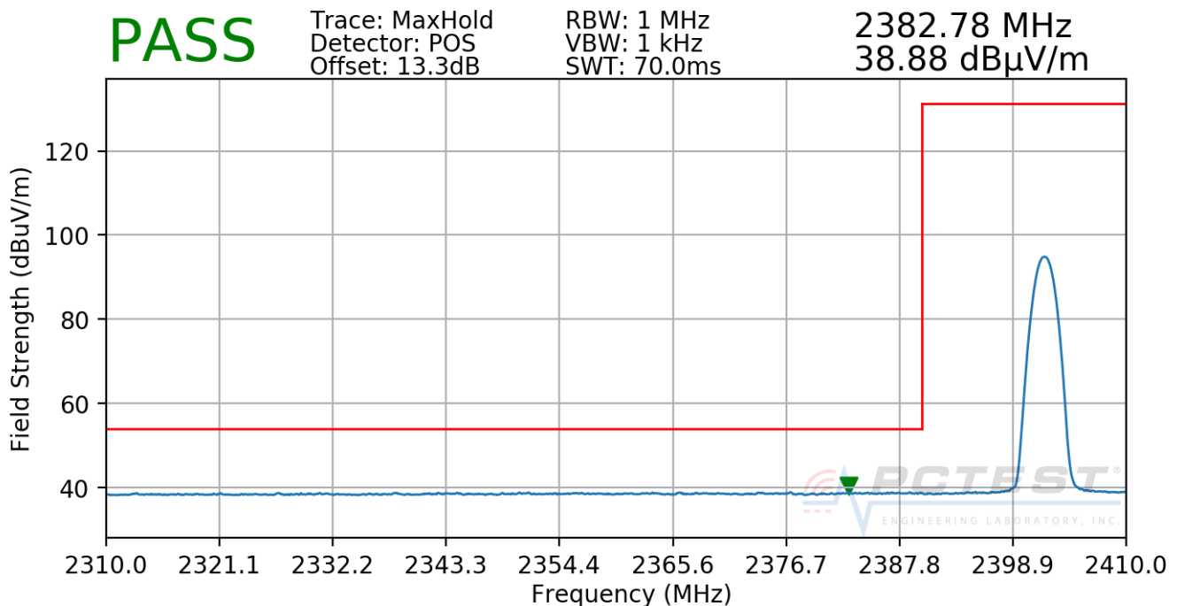
Plot 7-56. Radiated Restricted Lower Band Edge Measurement (Average)
