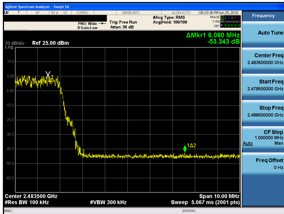
Plot 7-28. Band Edge Plot (Bluetooth with Hopping Enabled, 8DPSK, iPA – Ch. 78)
