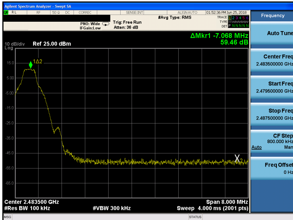
Plot 7-18. Band Edge Plot (Bluetooth with Hopping Disabled, GFSK, iPA – Ch. 78)
