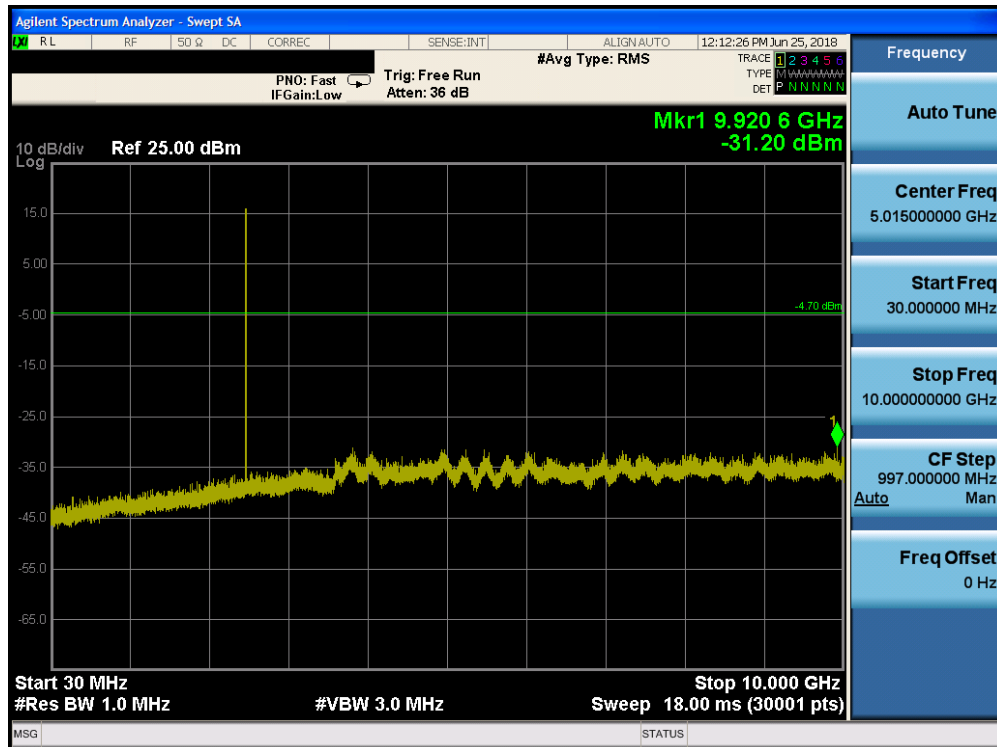
Plot 7-41. Conducted Spurious Plot (Bluetooth, GFSK, ePA – Ch. 78)
