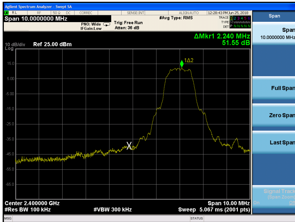
Plot 7-21. Band Edge Plot (Bluetooth with Hopping Disabled, 8DPSK, ePA – Ch. 0)
