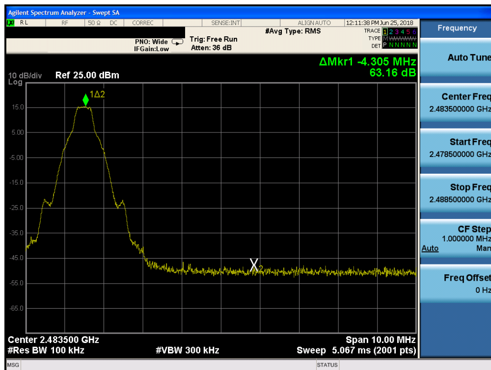
Plot 7-14. Band Edge Plot (Bluetooth with Hopping Disabled, GFSK, ePA – Ch. 78)
