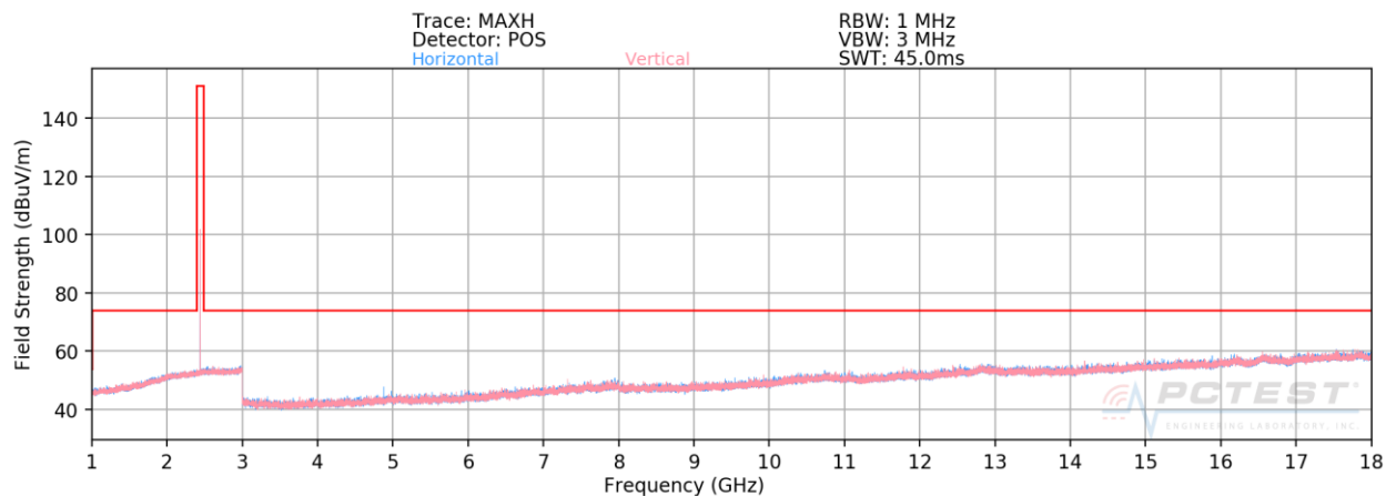
Plot 7-50. Radiated Spurious Plot above 1GHz (BT GFSK ePA – Ch. 39)
