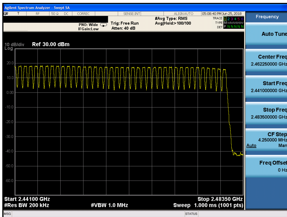
Plot 7-34. High End Spectrum Channel Hopping Plot (Bluetooth, GFSK, ePA)
