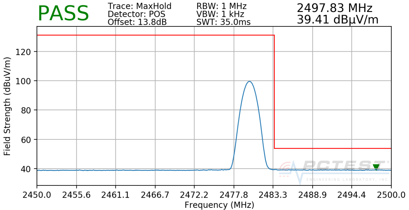
Plot 7-58. Radiated Restricted Upper Band Edge Measurement (Average)
