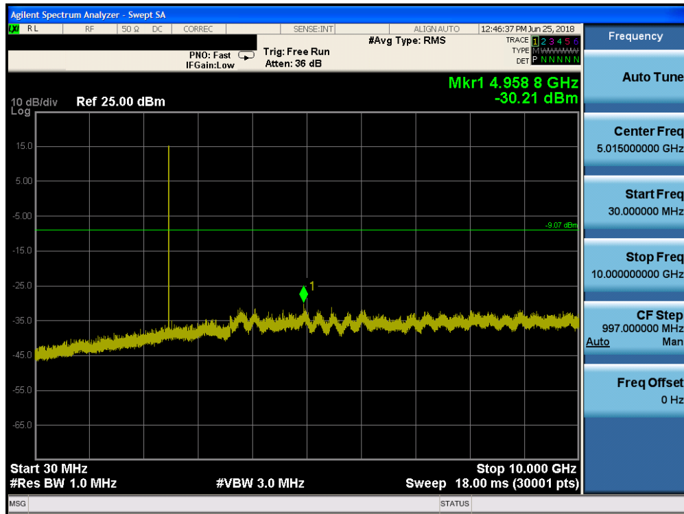
Plot 7-47. Conducted Spurious Plot (Bluetooth, 8DPSK, ePA – Ch. 78)
