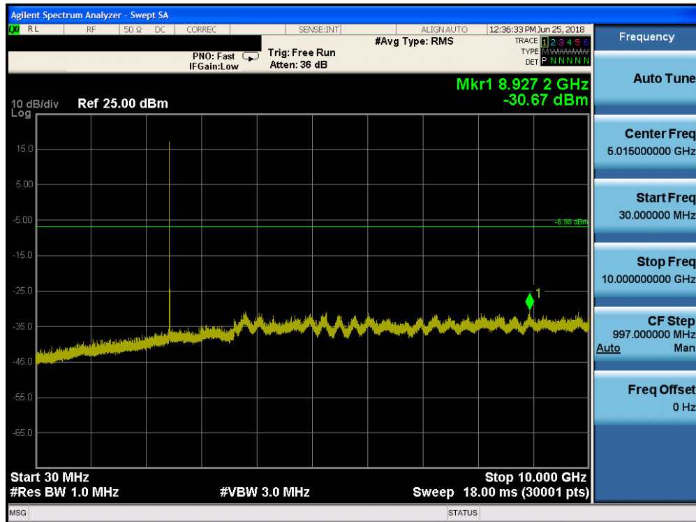
Plot 7-45. Conducted Spurious Plot (Bluetooth, 8DPSK, ePA – Ch. 39)
