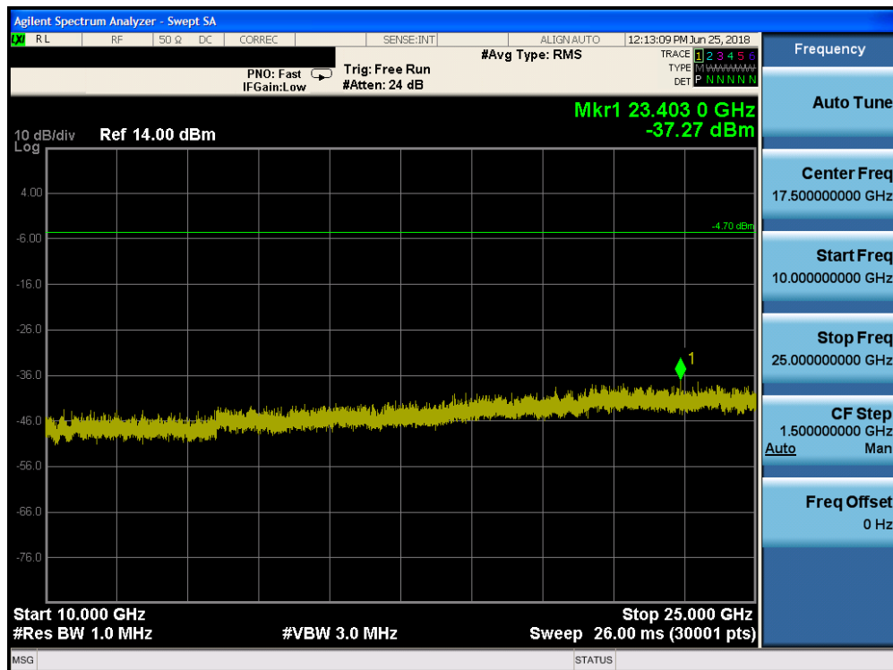
Plot 7-42. Conducted Spurious Plot (Bluetooth, GFSK, ePA – Ch. 78)
