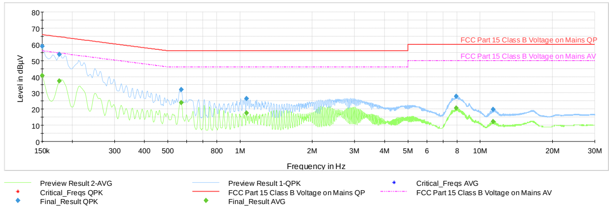
Plot 7-64. Line-Conducted Test Plot (N, with WCP + Laptop)
