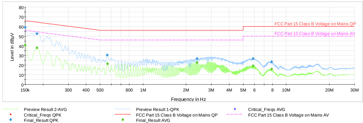
Plot 7-63. Line-Conducted Test Plot (L1, with WCP + Laptop)
