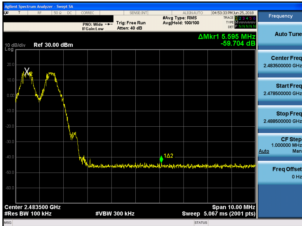
Plot 7-16. Band Edge Plot (Bluetooth with Hopping Enabled, GFSK, ePA – Ch. 78)
