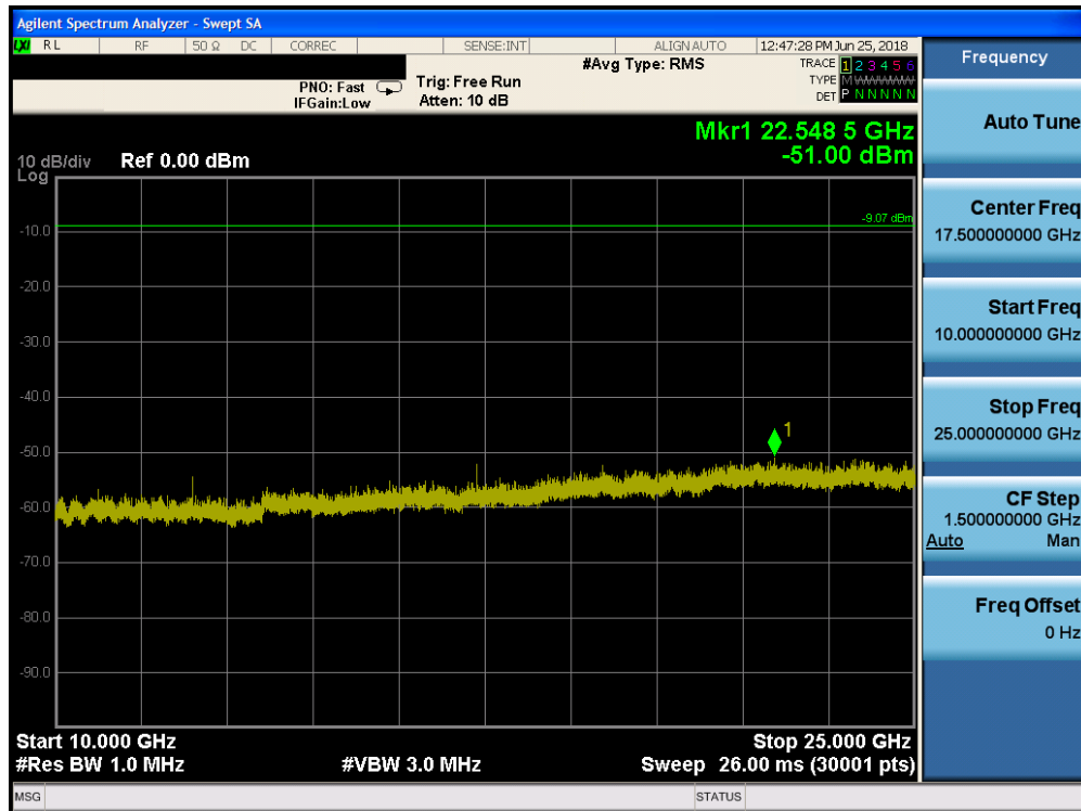
Plot 7-48. Conducted Spurious Plot (Bluetooth, 8DPSK, ePA – Ch. 78)
