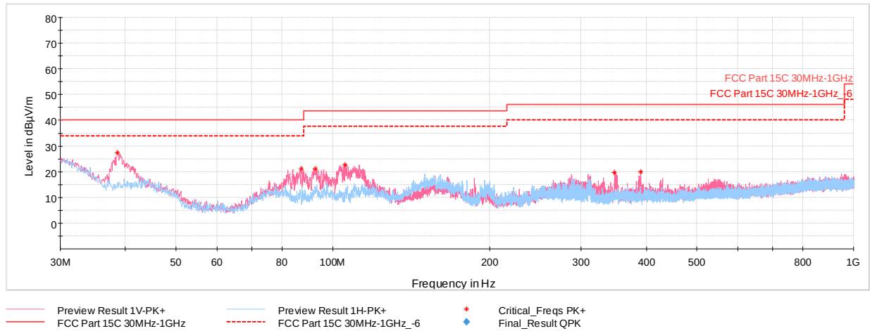
Plot 7-62. Radiated Spurious Plot below 1GHz (GFSK, ePA, with Laptop + Adapter attached)
