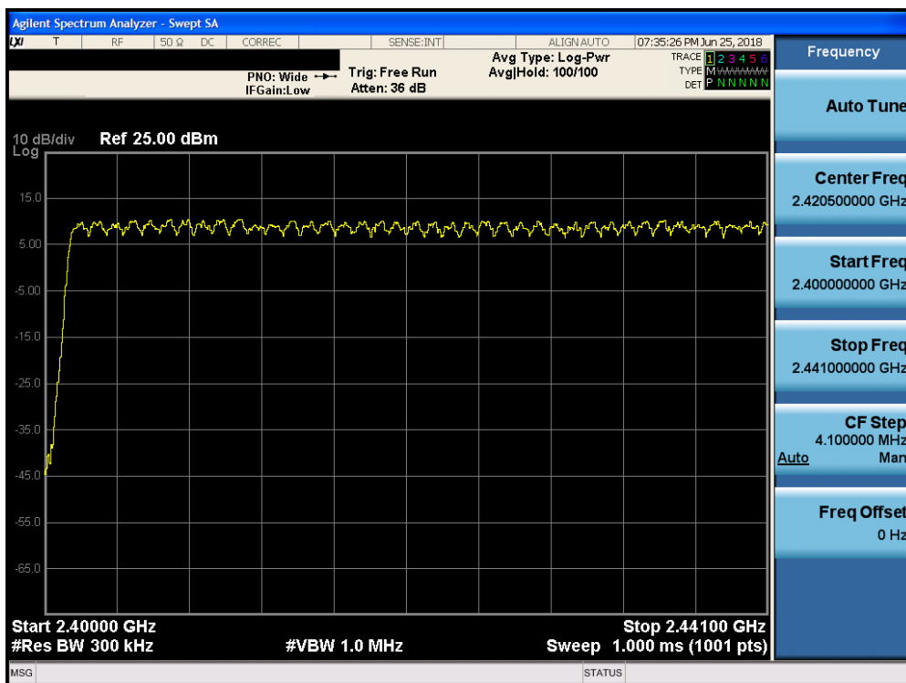
Plot 7-35. Low End Spectrum Channel Hopping Plot (Bluetooth, 8DPSK, ePA)
