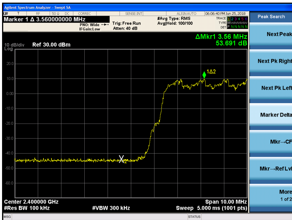
Plot 7-23. Band Edge Plot (Bluetooth with Hopping Enabled, 8DPSK, ePA – Ch. 0)
