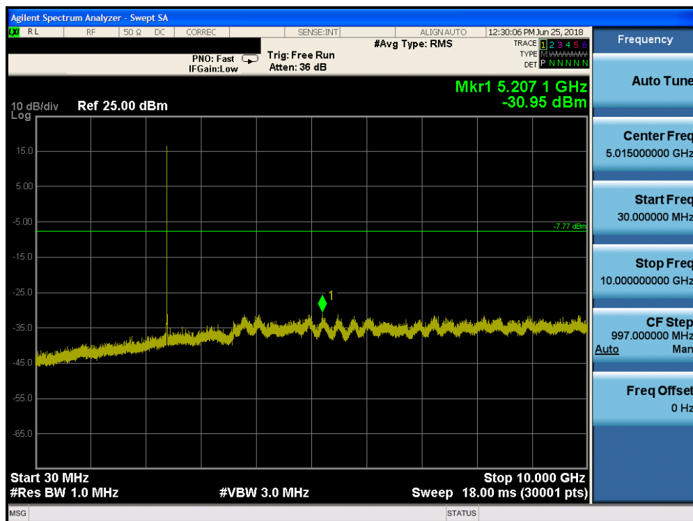
Plot 7-43. Conducted Spurious Plot (Bluetooth, 8DPSK, ePA – Ch. 0)
