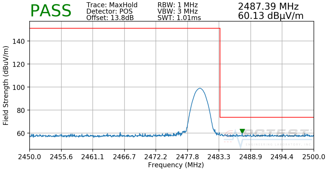
Plot 7-61. Radiated Restricted Upper Band Edge Measurement (Peak)
