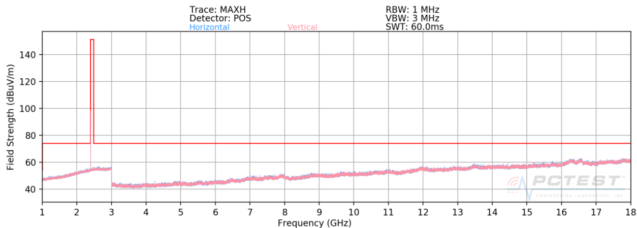
Plot 7-49. Radiated Spurious Plot above 1GHz (BT GFSK ePA – Ch. 0)
