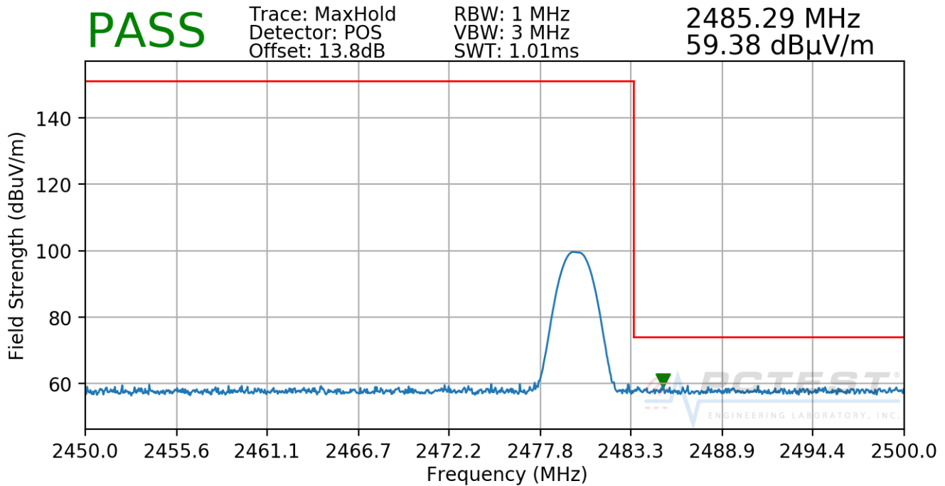
Plot 7-59. Radiated Restricted Upper Band Edge Measurement (Peak)
