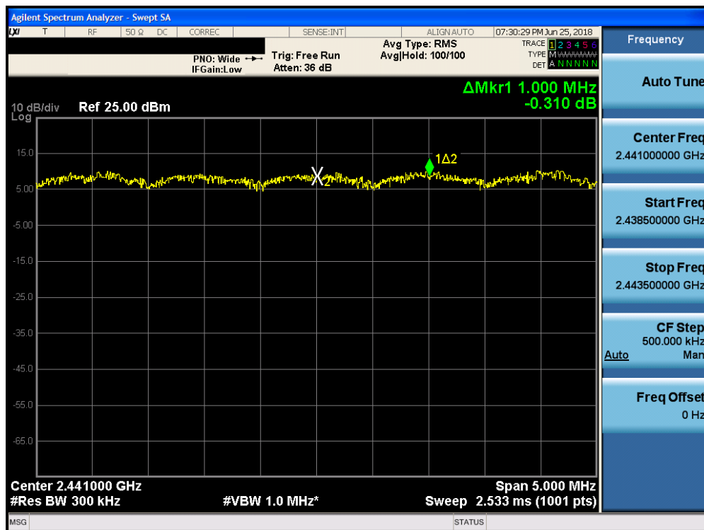
Plot 7-30. Channel Spacing Plot (Bluetooth, 8DPSK, ePA)
