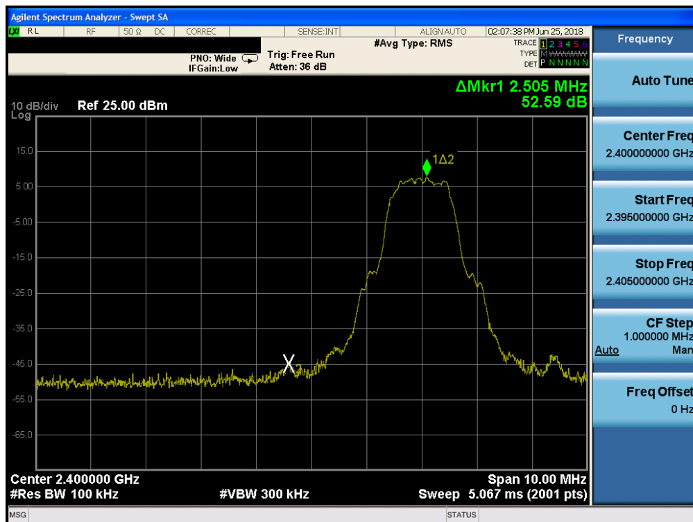
Plot 7-25. Band Edge Plot (Bluetooth with Hopping Disabled, 8DPSK, iPA – Ch. 0)
