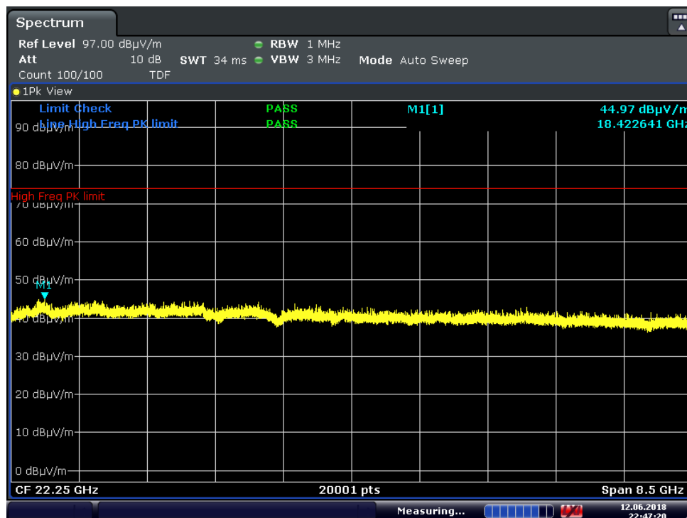
Plot 7-53. Radiated Spurious Plot above 18GHz (GFSK ePA, Ant. Pol. V)
