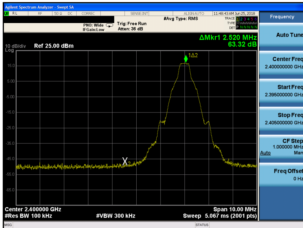
Plot 7-13. Band Edge Plot (Bluetooth with Hopping Disabled, GFSK, ePA – Ch. 0)
