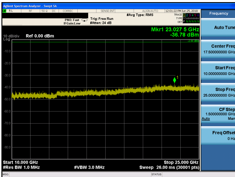
Plot 7-40. Conducted Spurious Plot (Bluetooth, GFSK, ePA Ch. 39)
