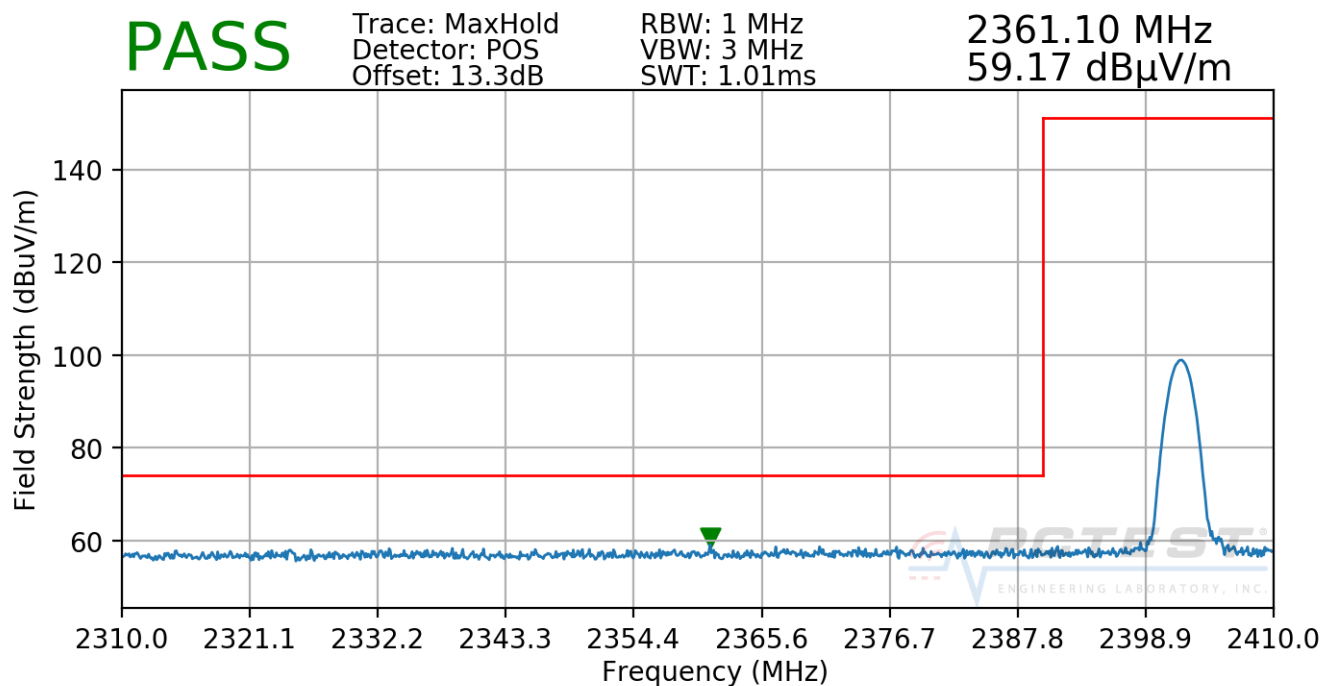
Plot 7-57. Radiated Restricted Lower Band Edge Measurement (Peak)
