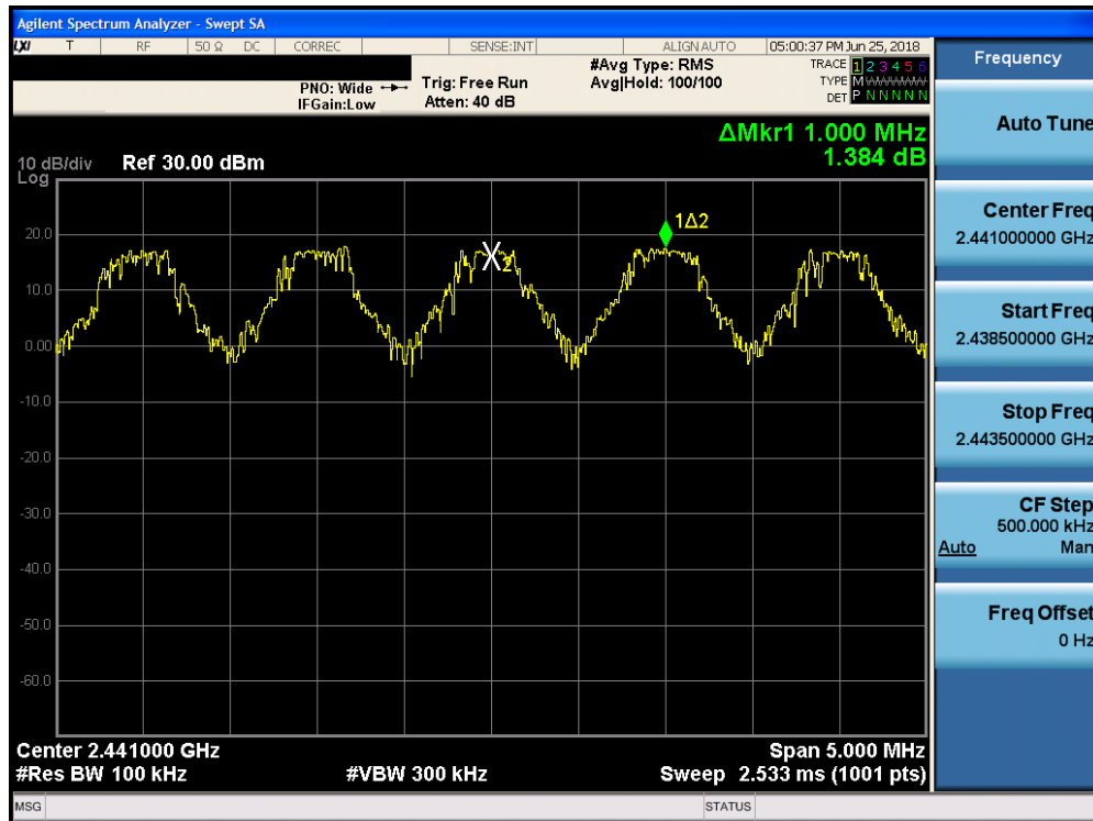
Plot 7-29. Channel Spacing Plot (Bluetooth, GFSK, ePA)
