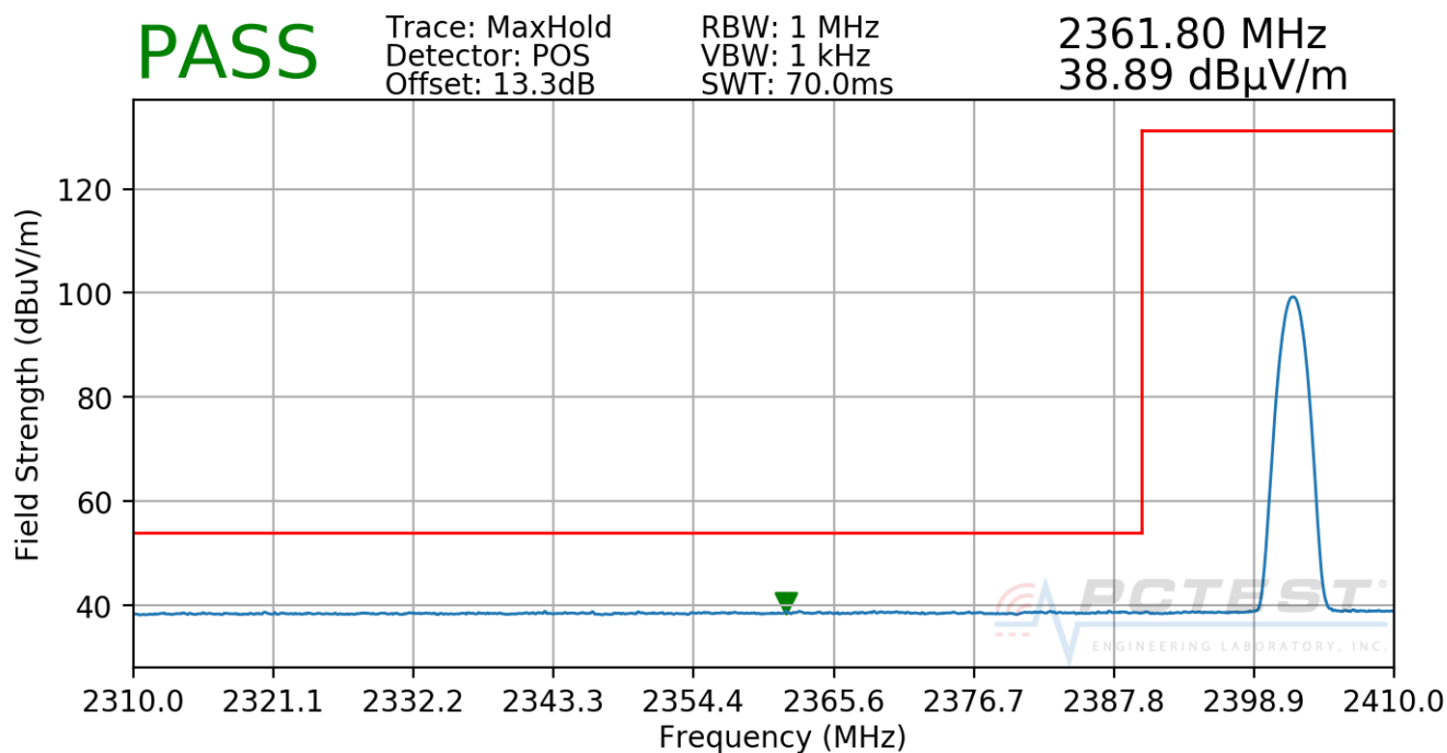
Plot 7-54. Radiated Restricted Lower Band Edge Measurement (Average)
