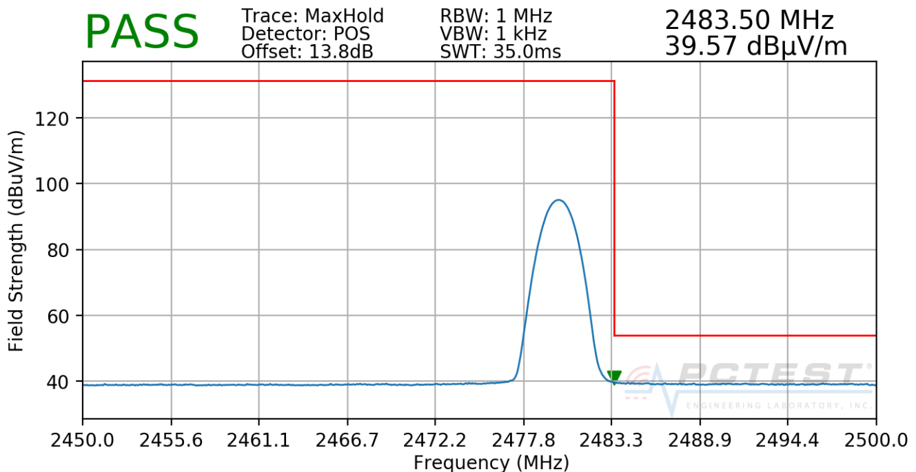
Plot 7-60. Radiated Restricted Upper Band Edge Measurement (Average)
