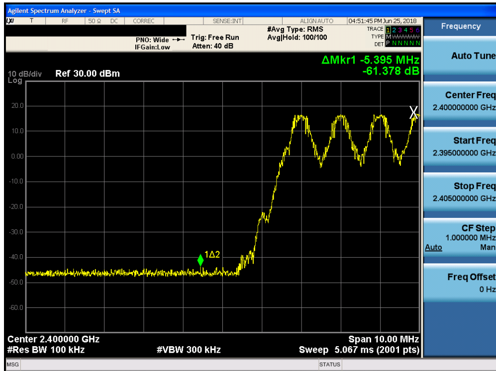
Plot 7-15. Band Edge Plot (Bluetooth with Hopping Enabled, GFSK, ePA – Ch. 0)
