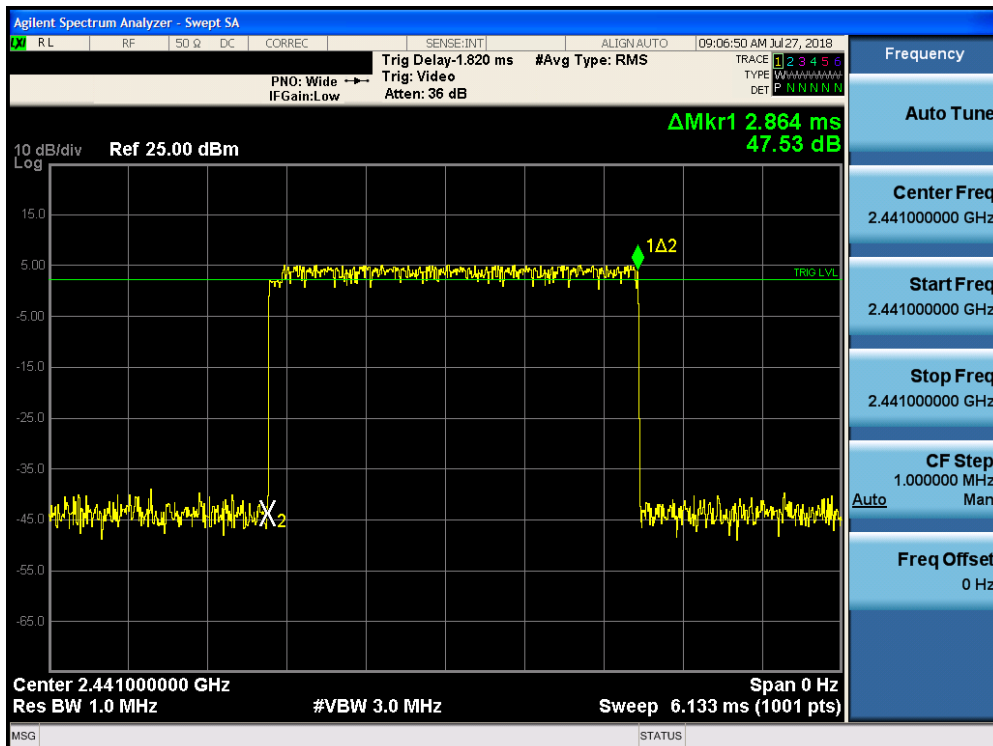
Plot 7-32. Time of Occupancy Plot (Bluetooth, 8DPSK, ePA)
