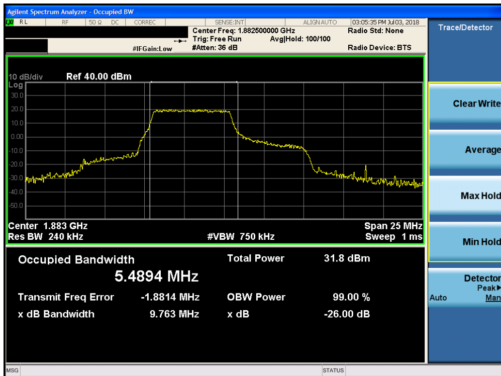
Plot 7-52. Occupied Bandwidth Plot (Band 25 - 10.0MHz 16-QAM - RB Size 27, RB Offset 0 Configuration)
