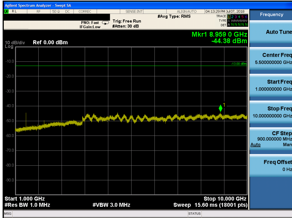
Plot 7-85. Conducted Spurious Plot (Band 12 - 10.0MHz QPSK - RB Size 1, RB Offset 0 - High Channel)
