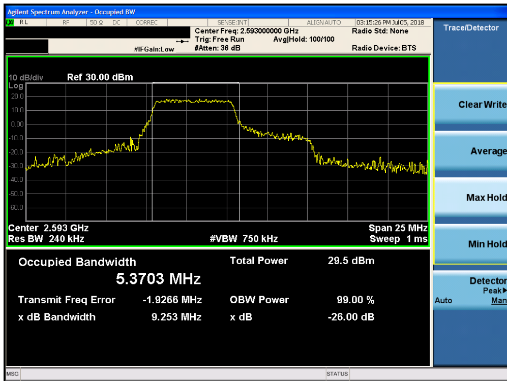
Plot 7-72. Occupied Bandwidth Plot (Band 41 - 10.0MHz 16-QAM - RB Size 27, RB Offset 0 Configuration)
