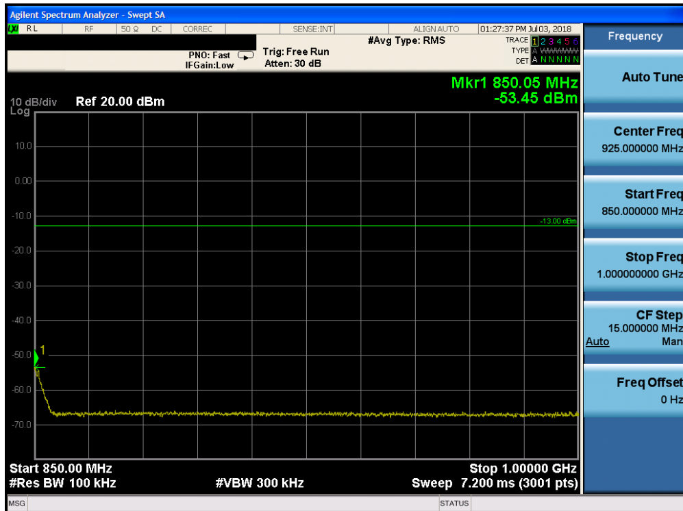
Plot 7-111. Conducted Spurious Plot (Band 26 - 10.0MHz QPSK - RB Size 1, RB Offset 0 - High Channel)
