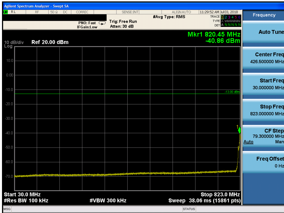
Plot 7-113. Conducted Spurious Plot (Band 5 - 10.0MHz QPSK - RB Size 1, RB Offset 0 - Low Channel)
