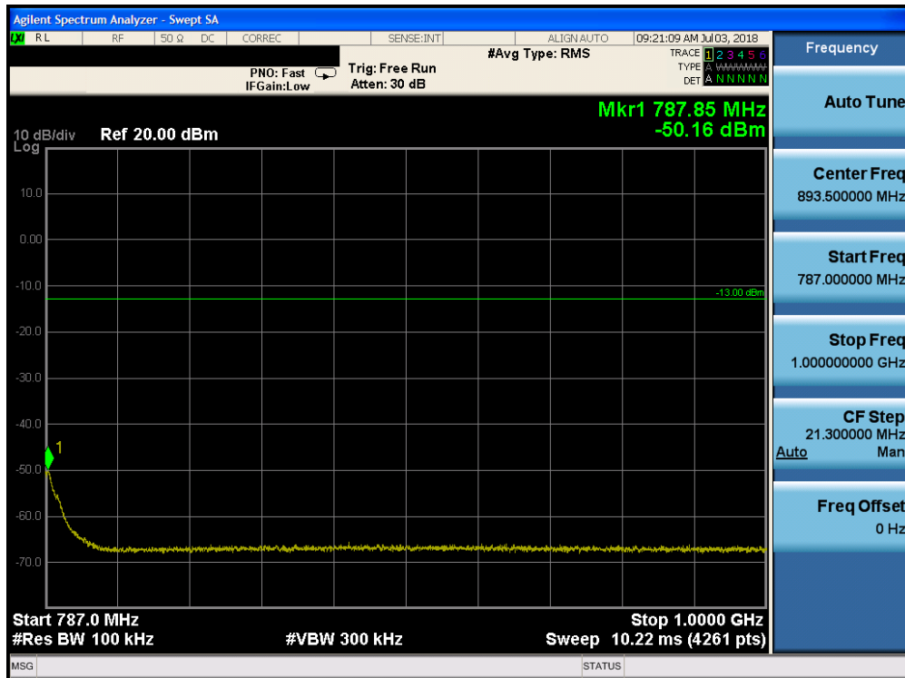
Plot 7-99. Conducted Spurious Plot (Band 13 - 5.0MHz QPSK - RB Size 1, RB Offset 0 - Mid Channel)
