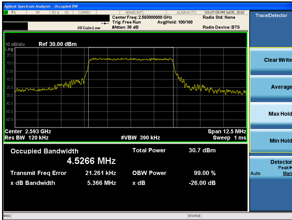
Plot 7-69. Occupied Bandwidth Plot (Band 41 - 5.0MHz QPSK - Full RB Configuration)
