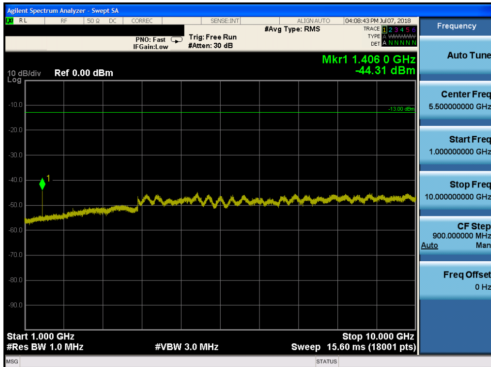
Plot 7-82. Conducted Spurious Plot (Band 12 - 10.0MHz QPSK - RB Size 1, RB Offset 0 - Mid Channel)
