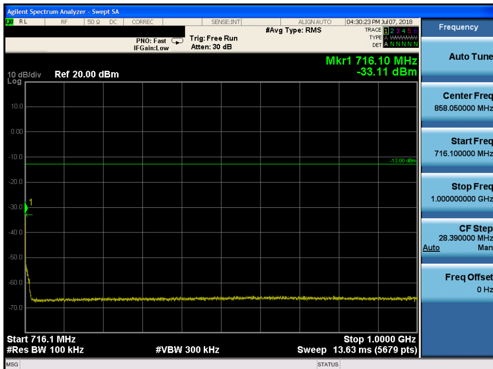
Plot 7-93. Conducted Spurious Plot (Band 17 - 10.0MHz QPSK - RB Size 1, RB Offset 0 - High Channel)
