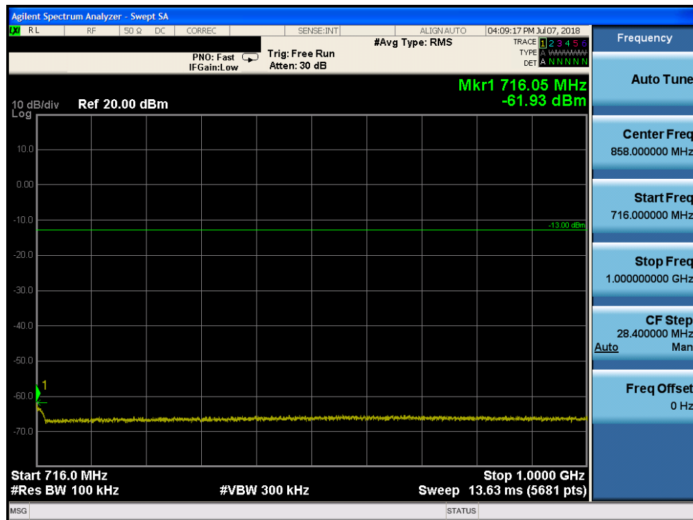
Plot 7-78. Conducted Spurious Plot (Band 12 - 10.0MHz QPSK - RB Size 1, RB Offset 0 - Low Channel)
