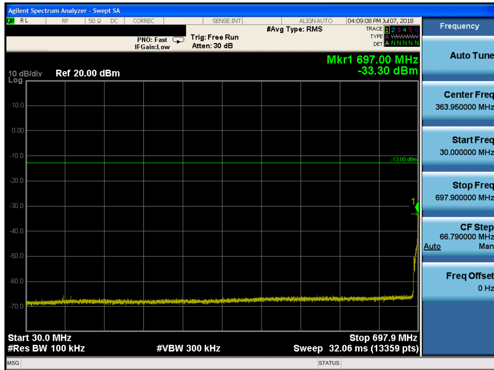
Plot 7-77. Conducted Spurious Plot (Band 12 - 10.0MHz QPSK - RB Size 1, RB Offset 0 - Low Channel)
