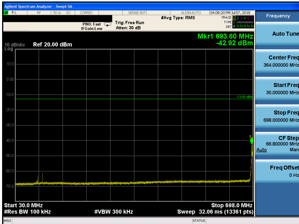
Plot 7-80. Conducted Spurious Plot (Band 12 - 10.0MHz QPSK - RB Size 1, RB Offset 0 - Mid Channel)
