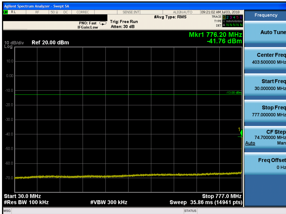
Plot 7-98. Conducted Spurious Plot (Band 13 - 5.0MHz QPSK - RB Size 1, RB Offset 0 - Mid Channel)
