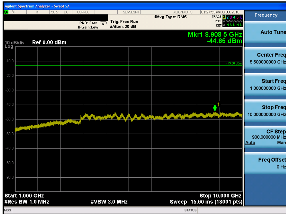
Plot 7-112. Conducted Spurious Plot (Band 26 - 10.0MHz QPSK - RB Size 1, RB Offset 0 - High Channel)
