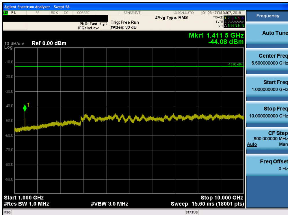
Plot 7-91. Conducted Spurious Plot (Band 17 - 10.0MHz QPSK - RB Size 1, RB Offset 0 - Mid Channel)
