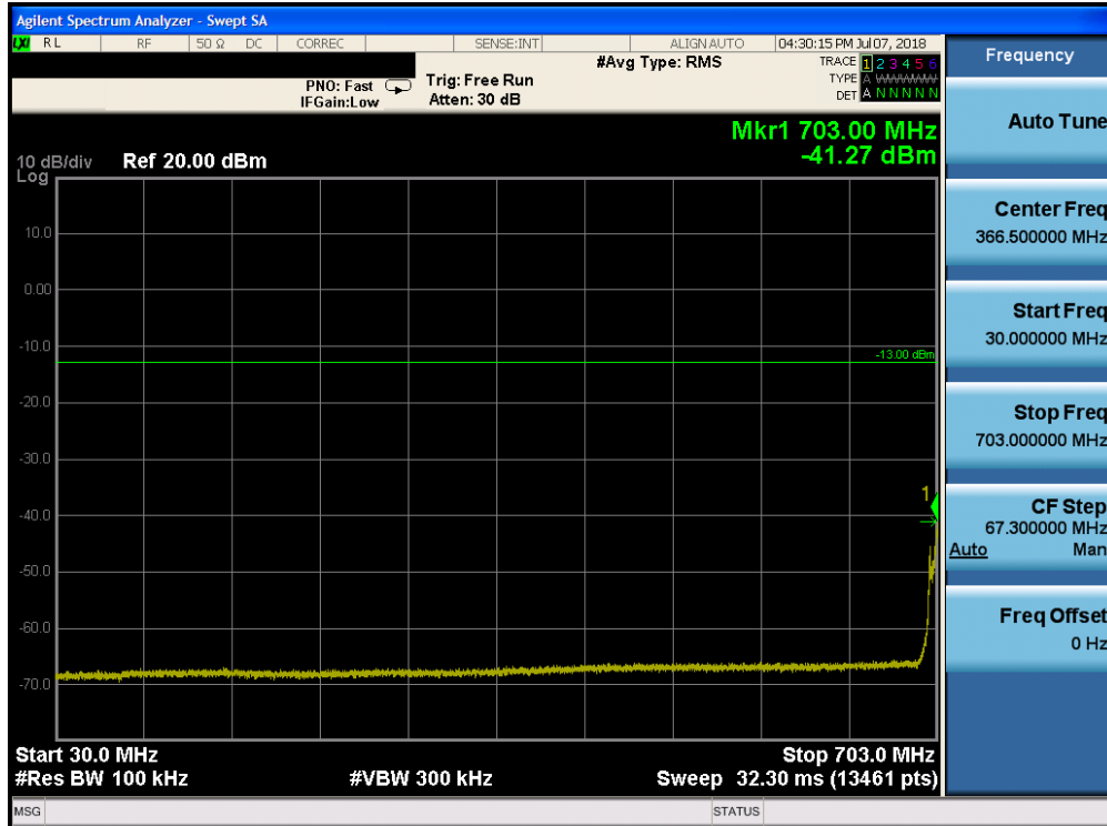
Plot 7-92. Conducted Spurious Plot (Band 17 - 10.0MHz QPSK - RB Size 1, RB Offset 0 - High Channel)
