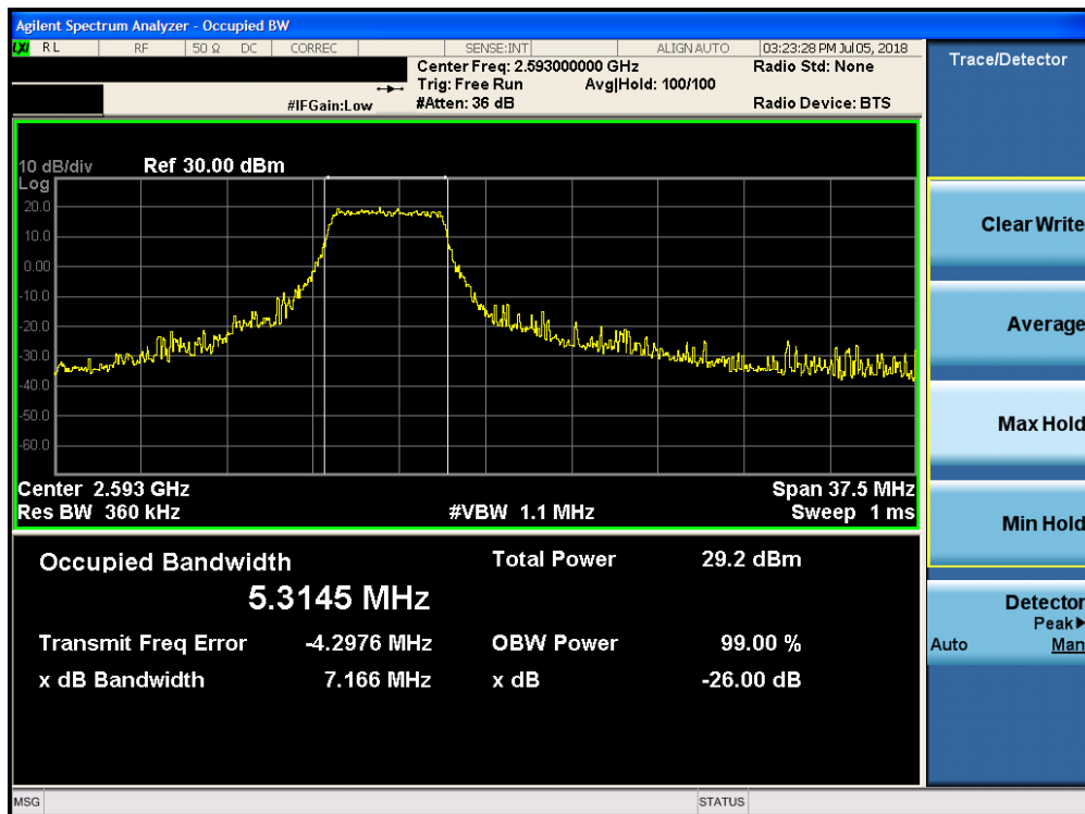
Plot 7-74. Occupied Bandwidth Plot (Band 41 - 15.0MHz 16-QAM - RB Size 27, RB Offset 0 Configuration)
