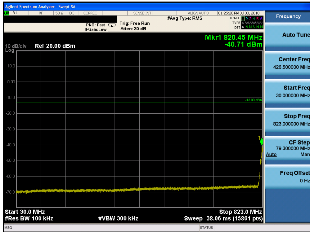
Plot 7-104. Conducted Spurious Plot (Band 26 - 10.0MHz QPSK - RB Size 1, RB Offset 0 - Low Channel)
