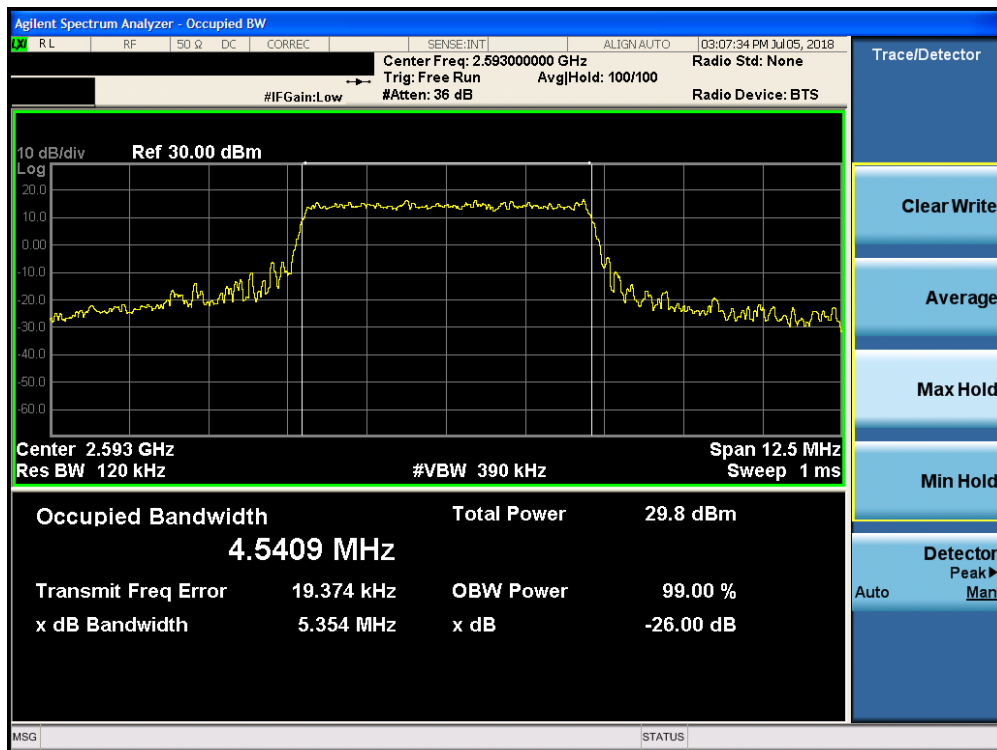
Plot 7-70. Occupied Bandwidth Plot (Band 41 - 5.0MHz 16-QAM - Full RB Configuration)
