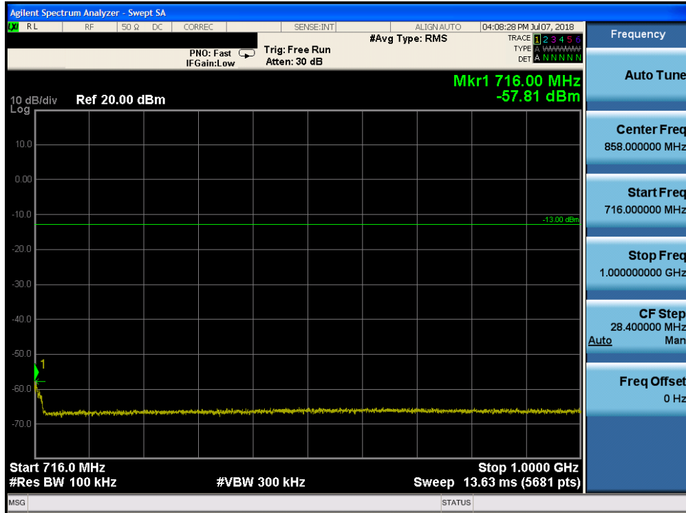
Plot 7-81. Conducted Spurious Plot (Band 12 - 10.0MHz QPSK - RB Size 1, RB Offset 0 - Mid Channel)
