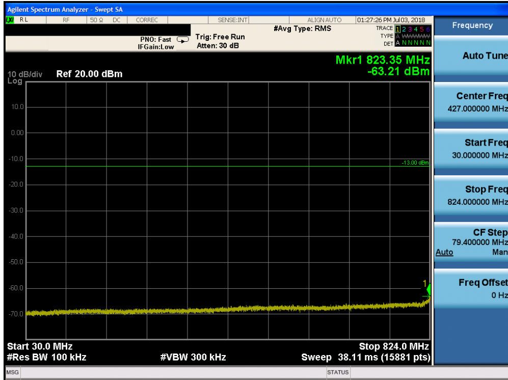
Plot 7-110. Conducted Spurious Plot (Band 26 - 10.0MHz QPSK - RB Size 1, RB Offset 0 - High Channel)
