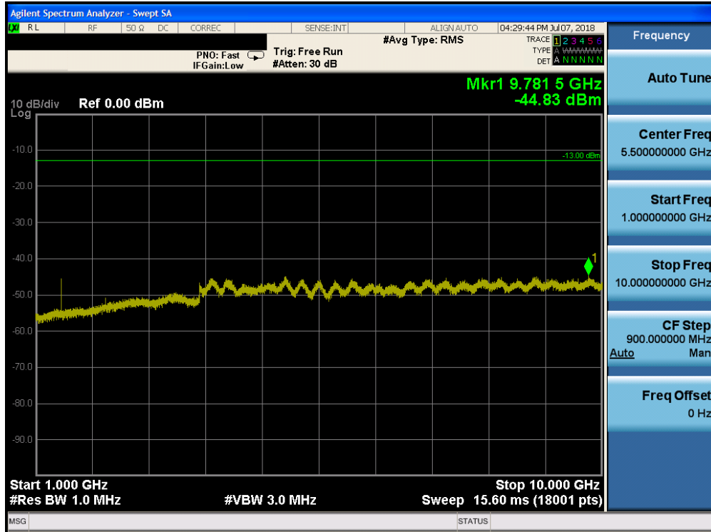
Plot 7-88. Conducted Spurious Plot (Band 17 - 10.0MHz QPSK - RB Size 1, RB Offset 0 - Low Channel)
