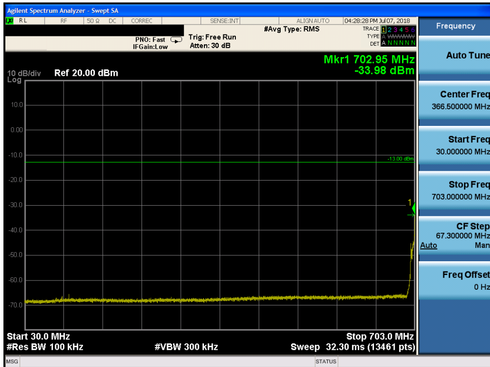
Plot 7-89. Conducted Spurious Plot (Band 17 - 10.0MHz QPSK - RB Size 1, RB Offset 0 - Mid Channel)
