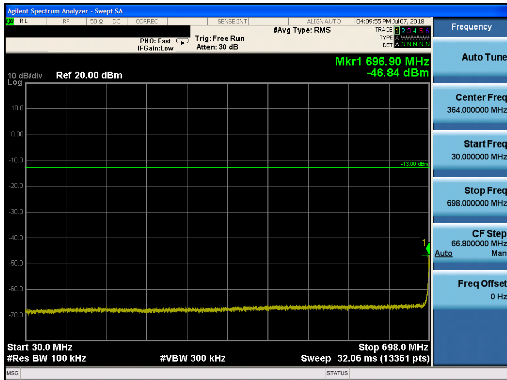
Plot 7-83. Conducted Spurious Plot (Band 12 - 10.0MHz QPSK - RB Size 1, RB Offset 0 - High Channel)
