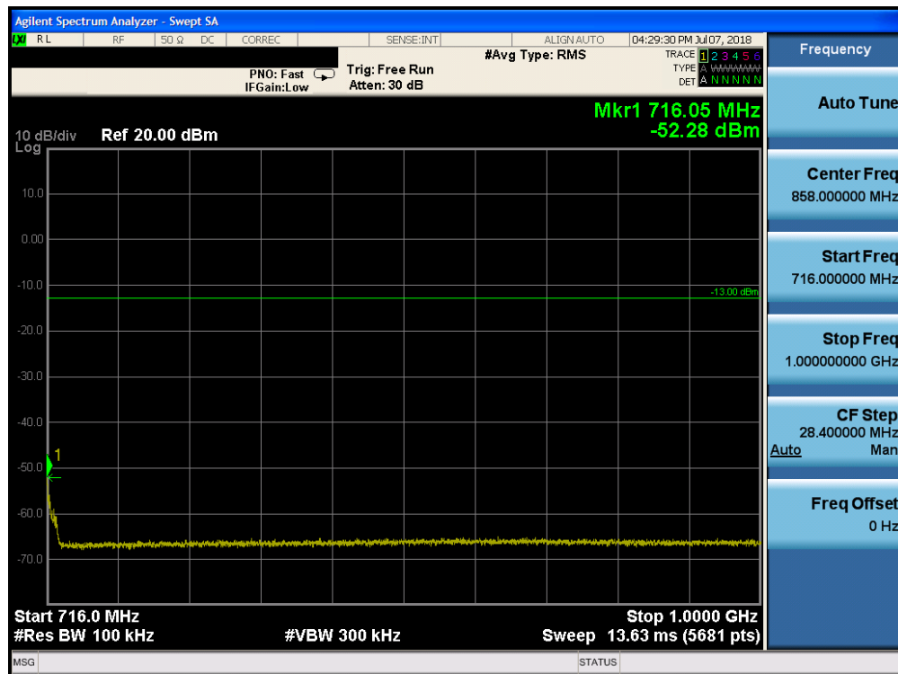
Plot 7-87. Conducted Spurious Plot (Band 17 - 10.0MHz QPSK - RB Size 1, RB Offset 0 - Low Channel)
