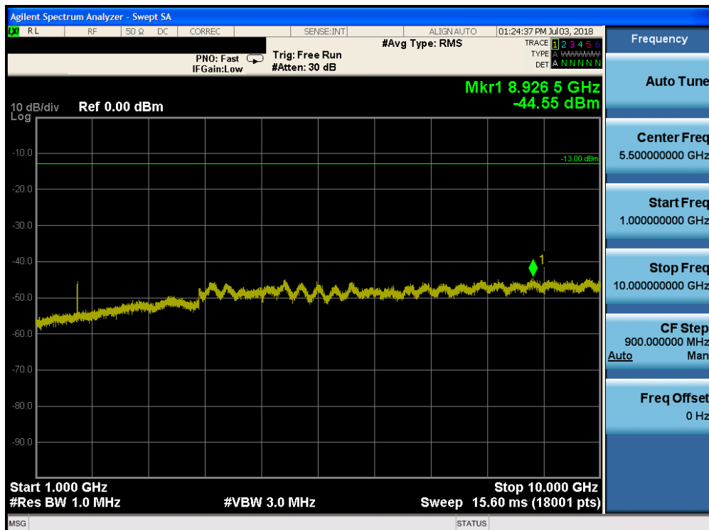
Plot 7-109. Conducted Spurious Plot (Band 26 - 10.0MHz QPSK - RB Size 1, RB Offset 0 - Mid Channel)
