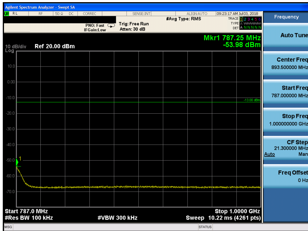
Plot 7-96. Conducted Spurious Plot (Band 13 - 5.0MHz QPSK - RB Size 1, RB Offset 0 - Low Channel)
