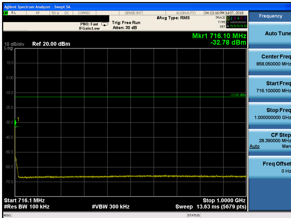
Plot 7-84. Conducted Spurious Plot (Band 12 - 10.0MHz QPSK - RB Size 1, RB Offset 0 - High Channel)
