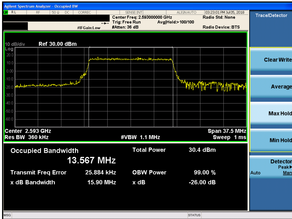
Plot 7-73. Occupied Bandwidth Plot (Band 41 - 15.0MHz QPSK - Full RB Configuration)
