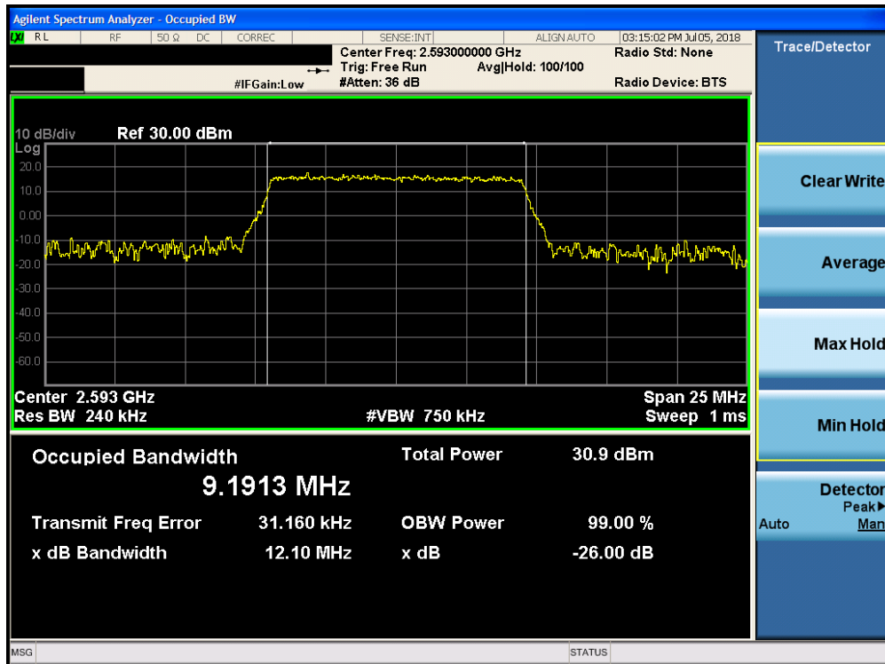
Plot 7-71. Occupied Bandwidth Plot (Band 41 - 10.0MHz QPSK - Full RB Configuration)
