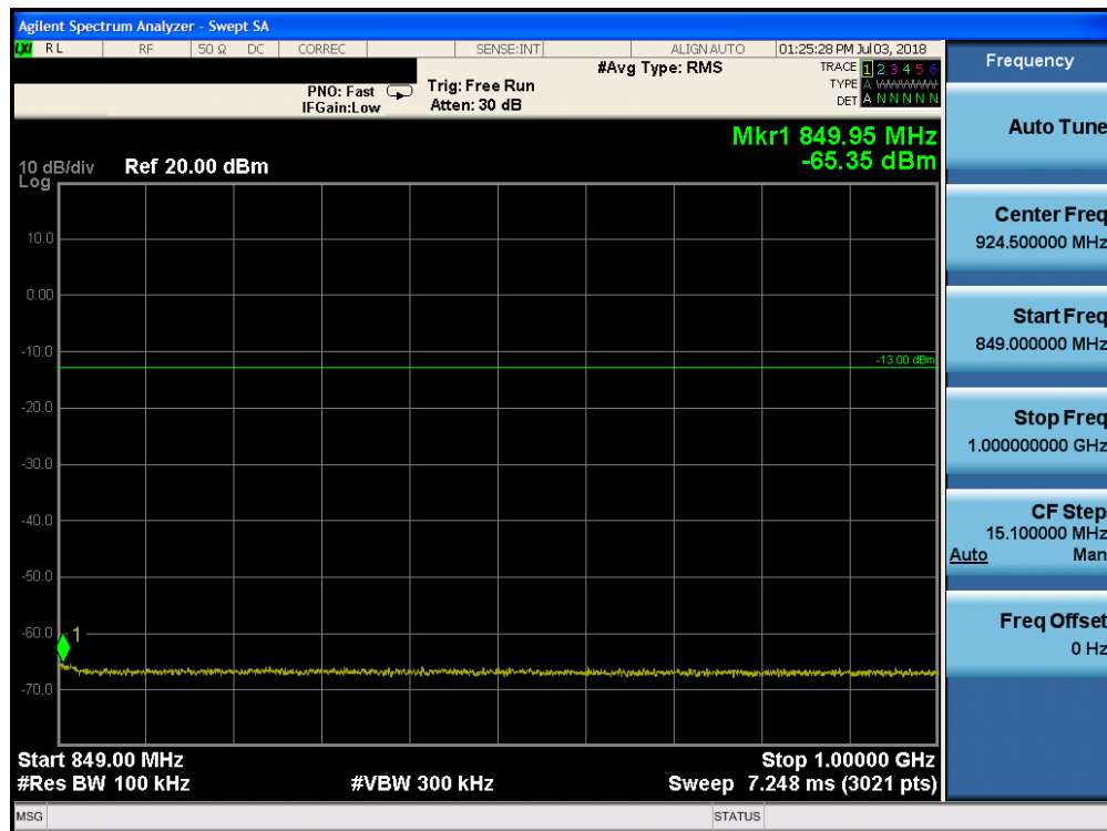
Plot 7-105. Conducted Spurious Plot (Band 26 - 10.0MHz QPSK - RB Size 1, RB Offset 0 - Low Channel)
