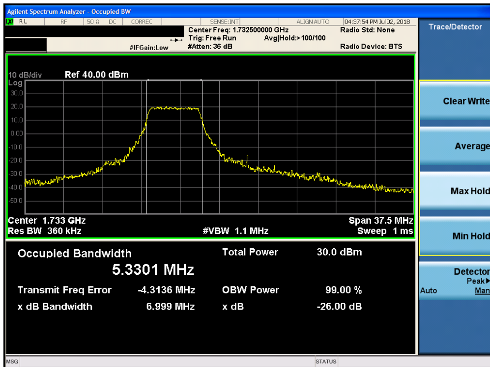
Plot 7-42. Occupied Bandwidth Plot (Band 4 - 15.0MHz 16-QAM - RB Size 27, RB Offset 0 Configuration)
