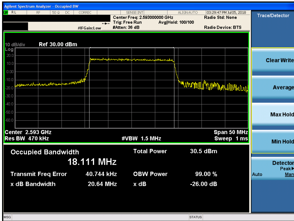
Plot 7-75. Occupied Bandwidth Plot (Band 41 – 20.0MHz QPSK - Full RB Configuration)
