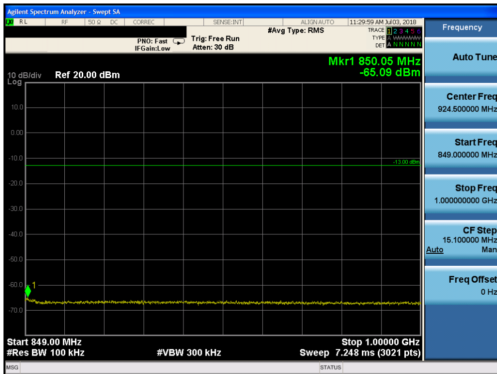
Plot 7-114. Conducted Spurious Plot (Band 5 - 10.0MHz QPSK - RB Size 1, RB Offset 0 - Low Channel)
