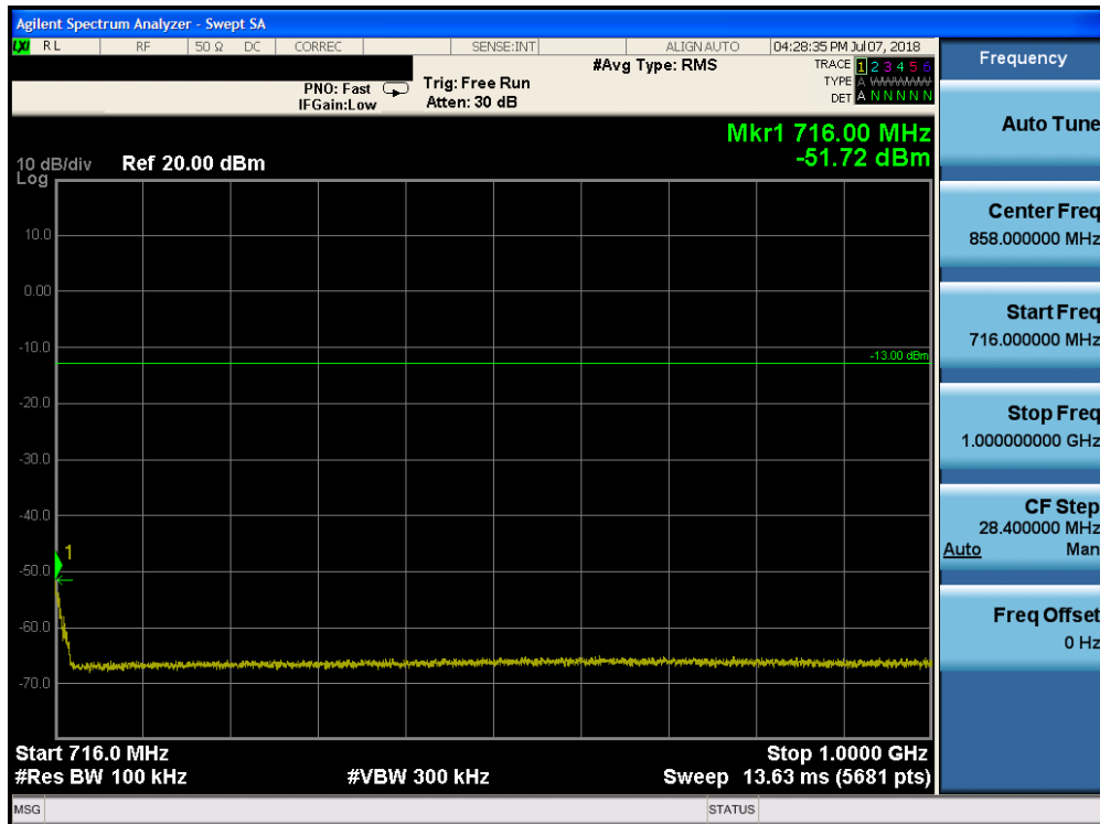
Plot 7-90. Conducted Spurious Plot (Band 17 - 10.0MHz QPSK - RB Size 1, RB Offset 0 - Mid Channel)
