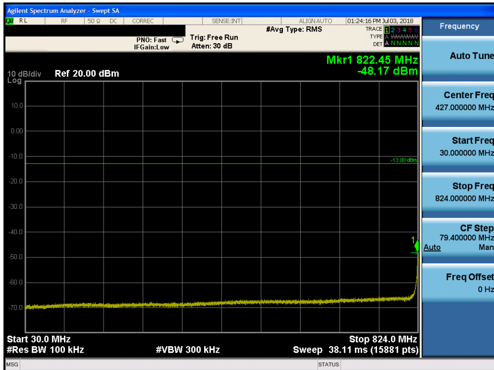
Plot 7-107. Conducted Spurious Plot (Band 26 - 10.0MHz QPSK - RB Size 1, RB Offset 0 - Mid Channel)
