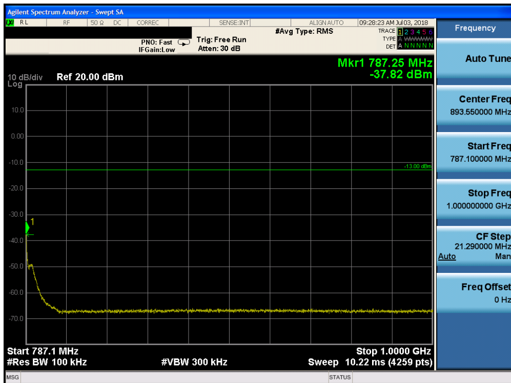
Plot 7-102. Conducted Spurious Plot (Band 13 - 5.0MHz QPSK - RB Size 1, RB Offset 0 - High Channel)
