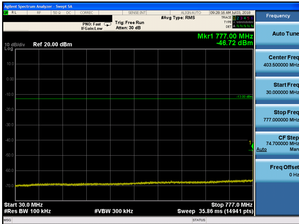
Plot 7-101. Conducted Spurious Plot (Band 13 - 5.0MHz QPSK - RB Size 1, RB Offset 0 - High Channel)
