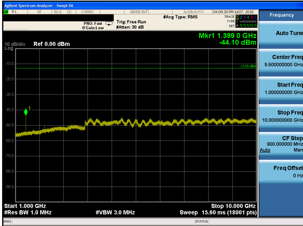
Plot 7-79. Conducted Spurious Plot (Band 12 - 10.0MHz QPSK - RB Size 1, RB Offset 0 - Low Channel)
