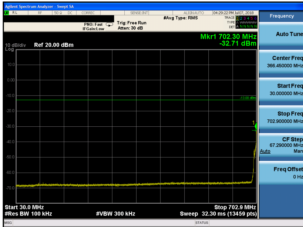
Plot 7-86. Conducted Spurious Plot (Band 17 - 10.0MHz QPSK - RB Size 1, RB Offset 0 - Low Channel)
