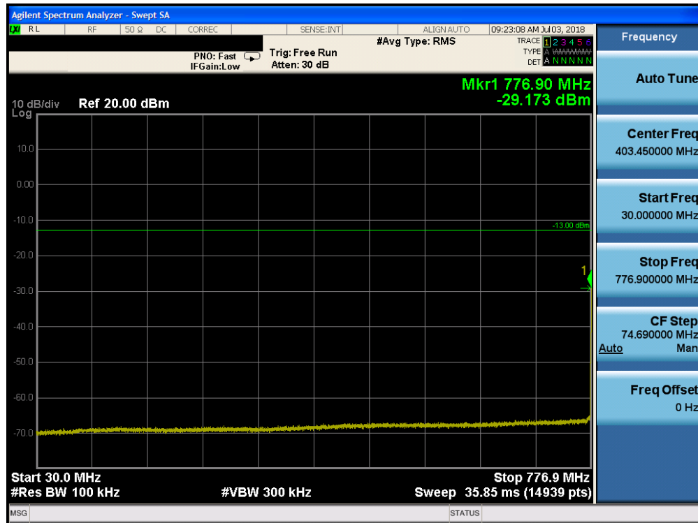
Plot 7-95. Conducted Spurious Plot (Band 13 - 5.0MHz QPSK - RB Size 1, RB Offset 0 - Low Channel)
