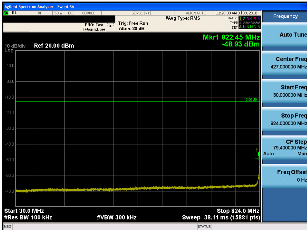
Plot 7-116. Conducted Spurious Plot (Band 5 - 10.0MHz QPSK - RB Size 1, RB Offset 0 - Mid Channel)
