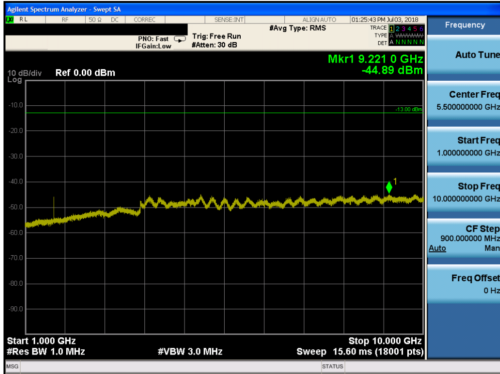
Plot 7-106. Conducted Spurious Plot (Band 26 - 10.0MHz QPSK - RB Size 1, RB Offset 0 - Low Channel)
