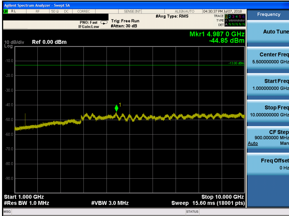
Plot 7-94. Conducted Spurious Plot (Band 17 - 10.0MHz QPSK - RB Size 1, RB Offset 0 - High Channel)
