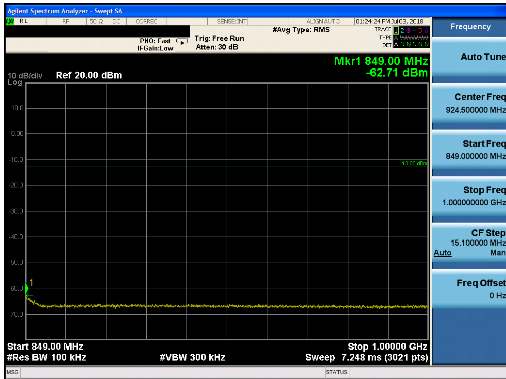
Plot 7-108. Conducted Spurious Plot (Band 26 - 10.0MHz QPSK - RB Size 1, RB Offset 0 - Mid Channel)
