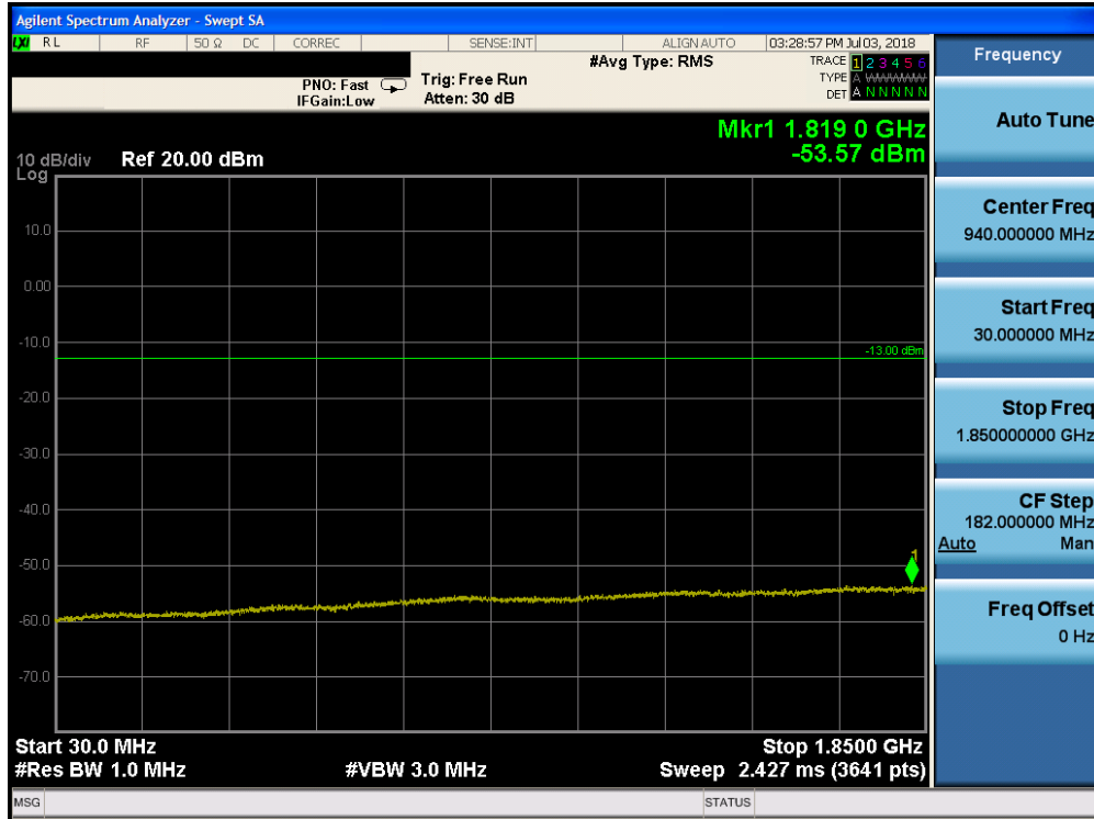
Plot 7-137. Conducted Spurious Plot (Band 25 – 20.0MHz QPSK - RB Size 1, RB Offset 0 - High Channel)
