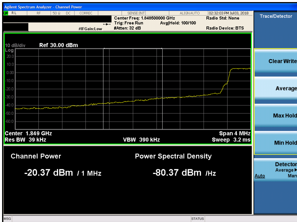
Plot 7-223. Lower Extended Band Edge Plot (Band 25 - 3.0MHz QPSK - Full RB Configuration)
