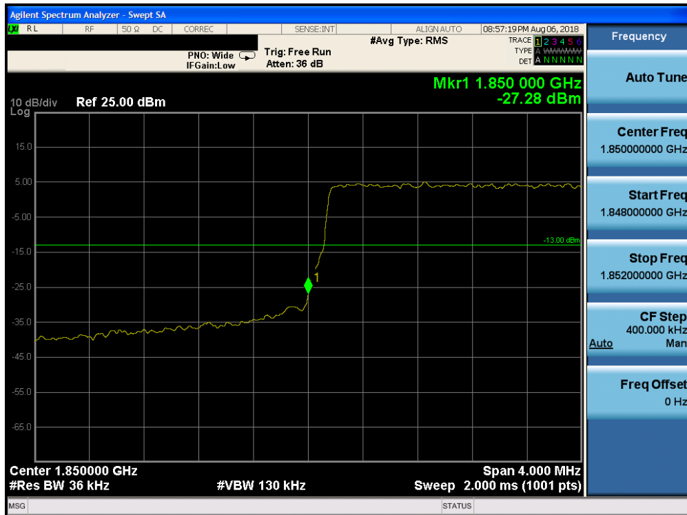
Plot 7-222. Lower Band Edge Plot (Band 25 - 3.0MHz QPSK - Full RB Configuration)
