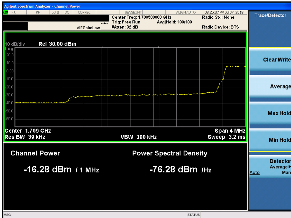
Plot 7-199. Lower Extended Band Edge Plot (Band 4 - 3.0MHz QPSK - Full RB Configuration)
