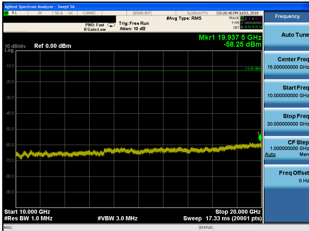
Plot 7-136. Conducted Spurious Plot (Band 25 - 20.0MHz QPSK - RB Size 1, RB Offset 0 - Mid Channel)
