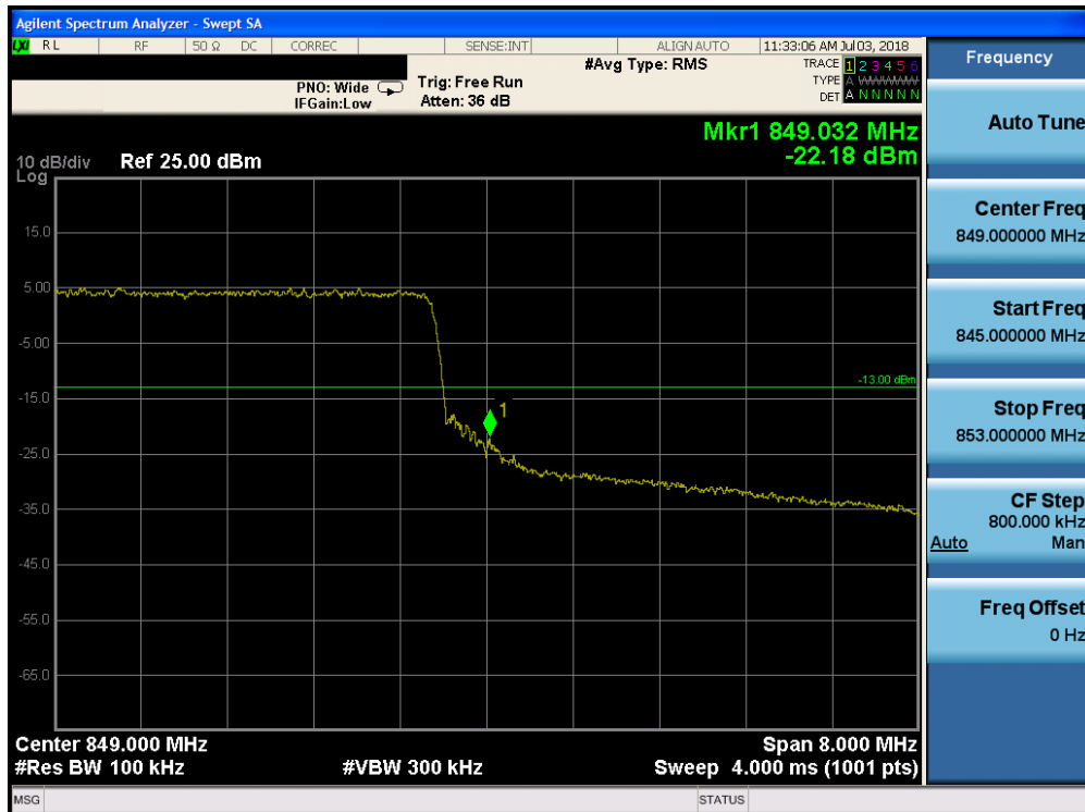
Plot 7-193. Upper Band Edge Plot (Band 5 - 10.0MHz QPSK - Full RB Configuration)
