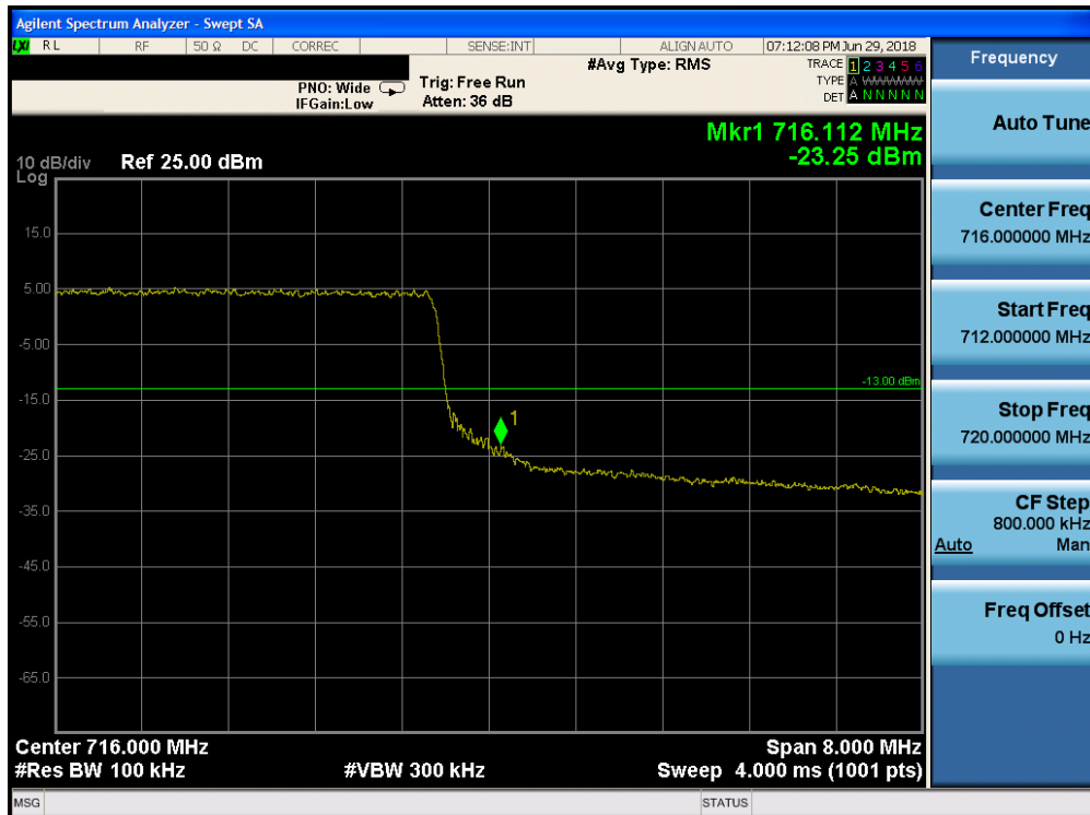
Plot 7-169. Upper Band Edge Plot (Band 17 - 10.0MHz QPSK - Full RB Configuration)
