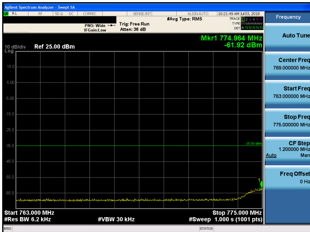
Plot 7-175. Lower Emission Mask Edge Plot (Band 13 - 10.0MHz QPSK - Full RB Configuration)
