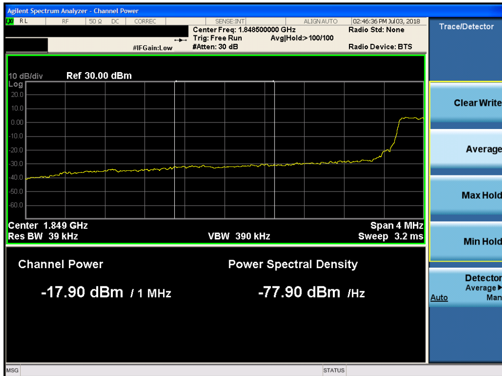
Plot 7-227. Lower Extended Band Edge Plot (Band 25 - 5.0MHz QPSK - Full RB Configuration)
