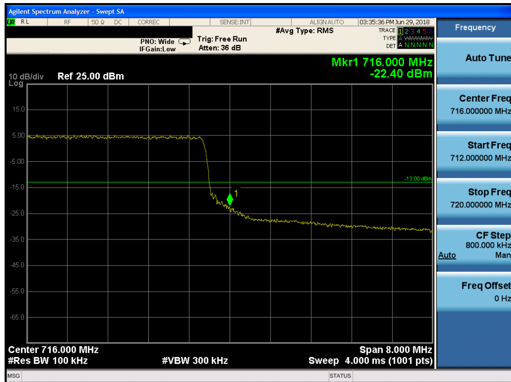
Plot 7-165. Upper Band Edge Plot (Band 12 - 10.0MHz QPSK - Full RB Configuration)
