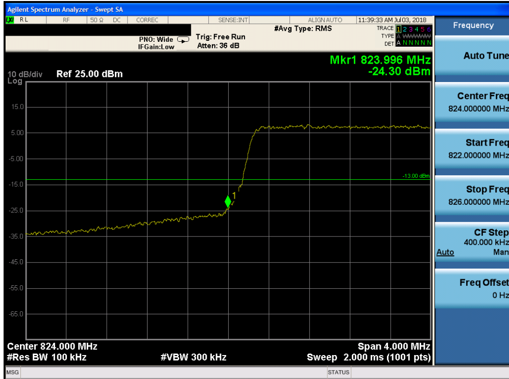
Plot 7-190. Lower Band Edge Plot (Band 5 - 5.0MHz QPSK - Full RB Configuration)
