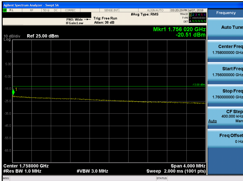
Plot 7-213. Upper Extended Band Edge Plot (Band 4 - 15.0MHz QPSK - Full RB Configuration)
