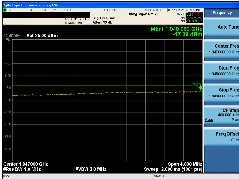
Plot 7-235. Lower Extended Band Edge Plot (Band 25 - 15.0MHz QPSK - Full RB Configuration)
