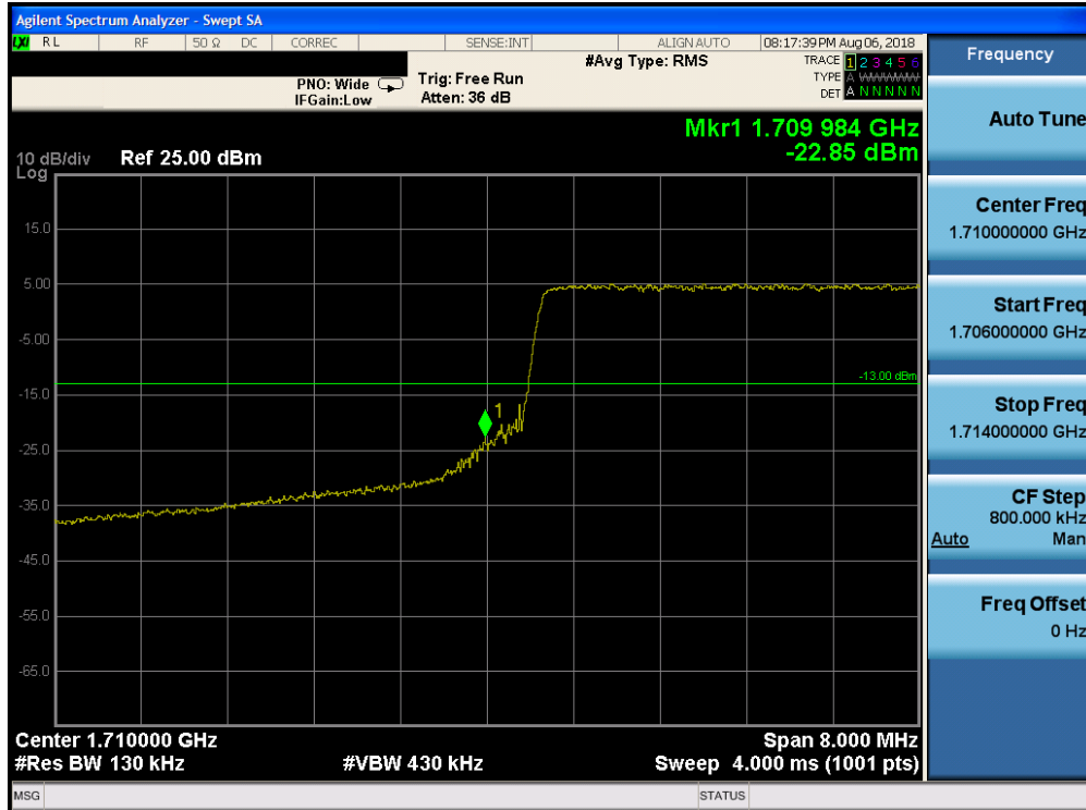
Plot 7-206. Lower Band Edge Plot (Band 4 - 10.0MHz QPSK - Full RB Configuration)
