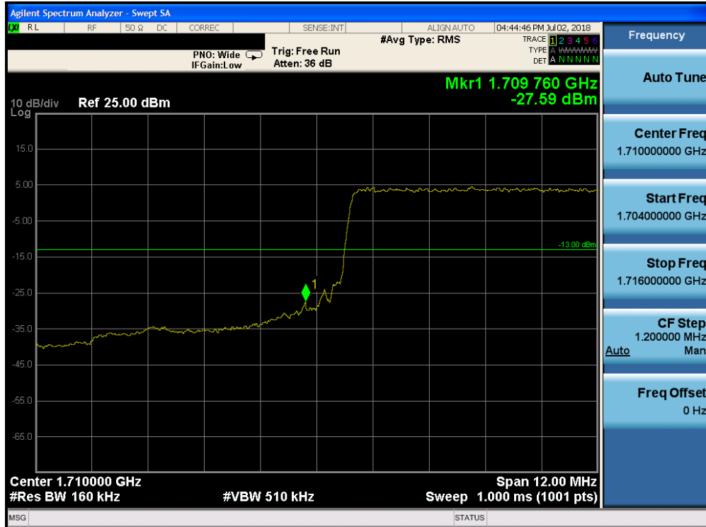
Plot 7-210. Lower Band Edge Plot (Band 4 - 15.0MHz QPSK - Full RB Configuration)
