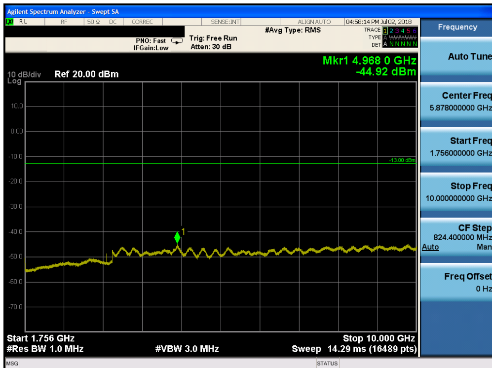
Plot 7-129. Conducted Spurious Plot (Band 4 - 20.0MHz QPSK - RB Size 1, RB Offset 0 - High Channel)
