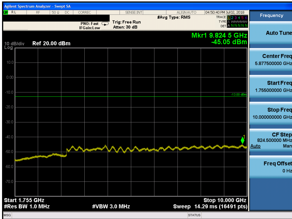
Plot 7-126. Conducted Spurious Plot (Band 4 - 20.0MHz QPSK - RB Size 1, RB Offset 0 - Mid Channel)
