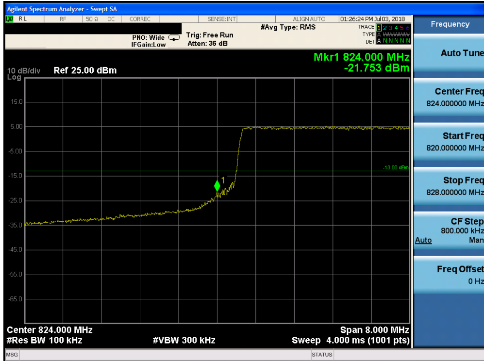
Plot 7-184. Lower Band Edge Plot (Band 26 - 10.0MHz QPSK - Full RB Configuration)
