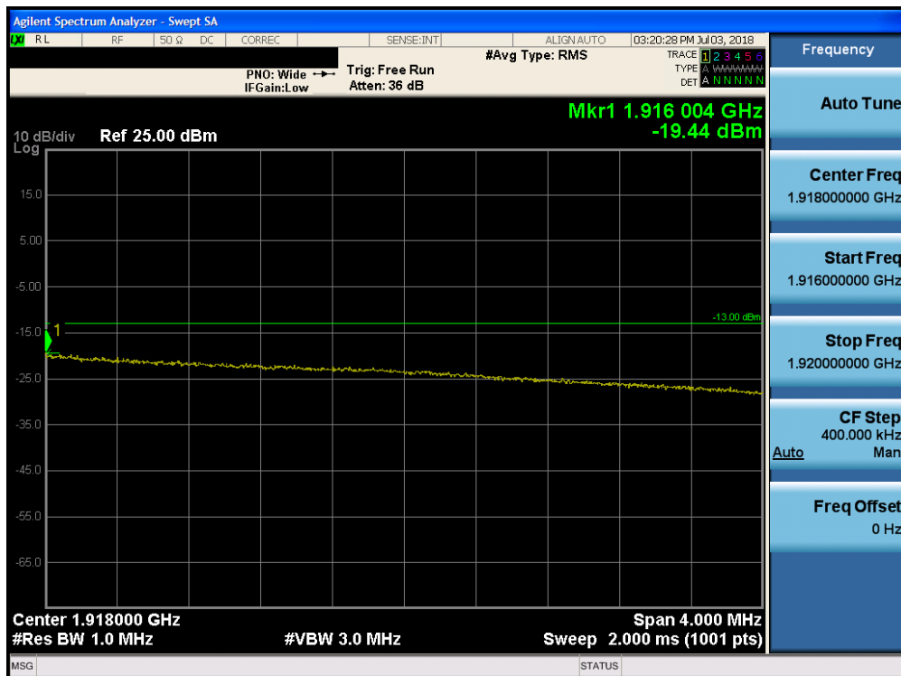
Plot 7-237. Upper Extended Band Edge Plot (Band 25 - 15.0MHz QPSK - Full RB Configuration)
