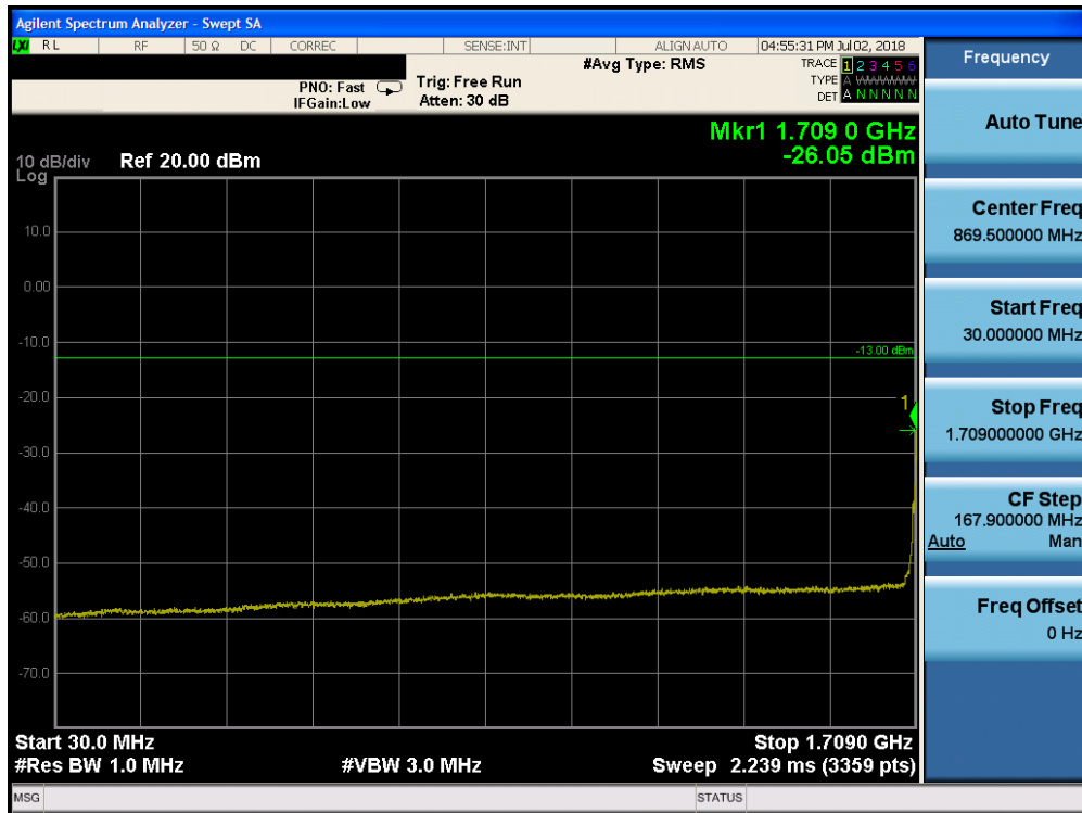
Plot 7-122. Conducted Spurious Plot (Band 4 - 20.0MHz QPSK - RB Size 1, RB Offset 0 - Low Channel)
