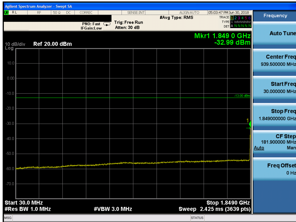
Plot 7-140. Conducted Spurious Plot (Band 2 - 20.0MHz QPSK - RB Size 1, RB Offset 0 - Low Channel)
