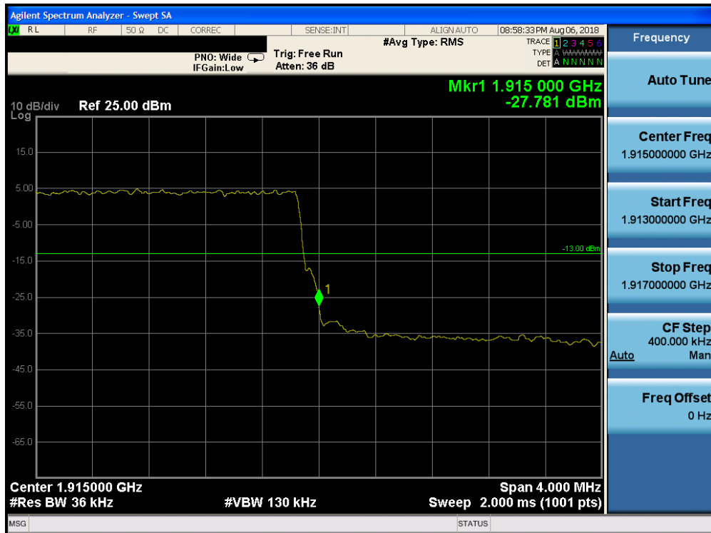
Plot 7-224. Upper Band Edge Plot (Band 25 - 3.0MHz QPSK - Full RB Configuration)
