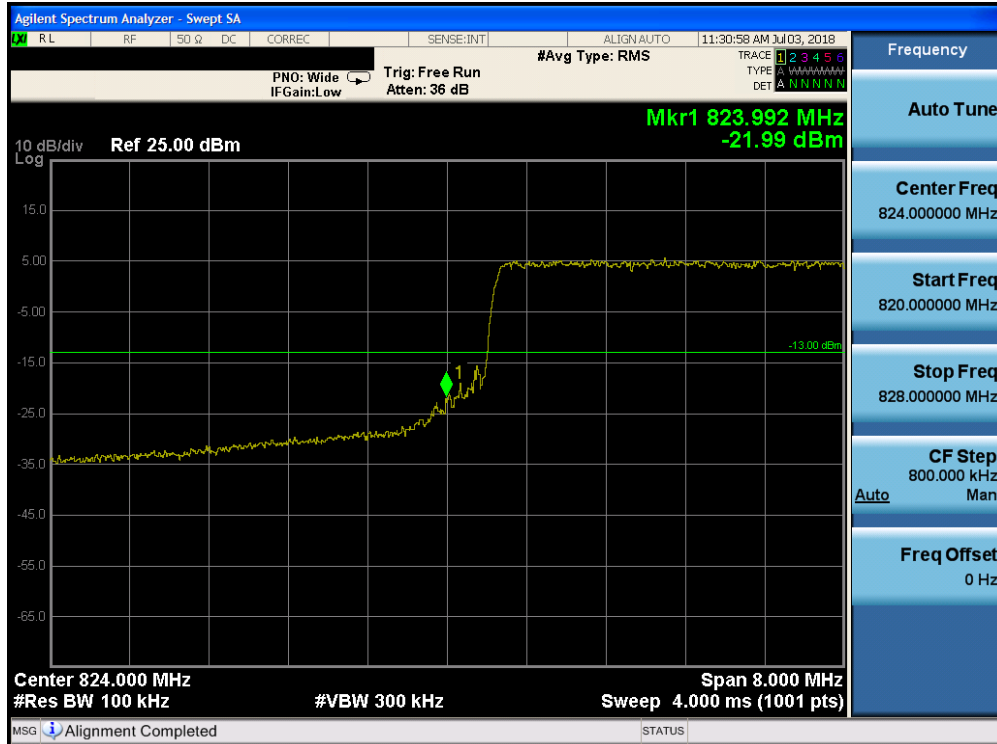
Plot 7-192. Lower Band Edge Plot (Band 5 - 10.0MHz QPSK - Full RB Configuration)
