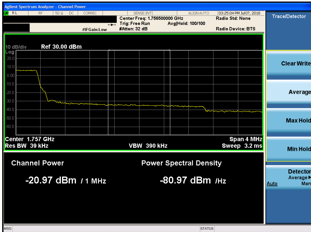
Plot 7-201. Upper Extended Band Edge Plot (Band 4 - 3.0MHz QPSK - Full RB Configuration)
