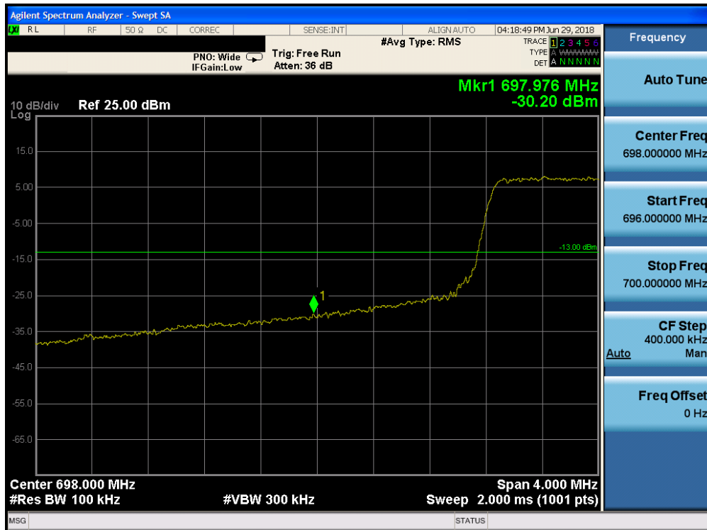
Plot 7-162. Lower Band Edge Plot (Band 12 - 5.0MHz QPSK - Full RB Configuration)
