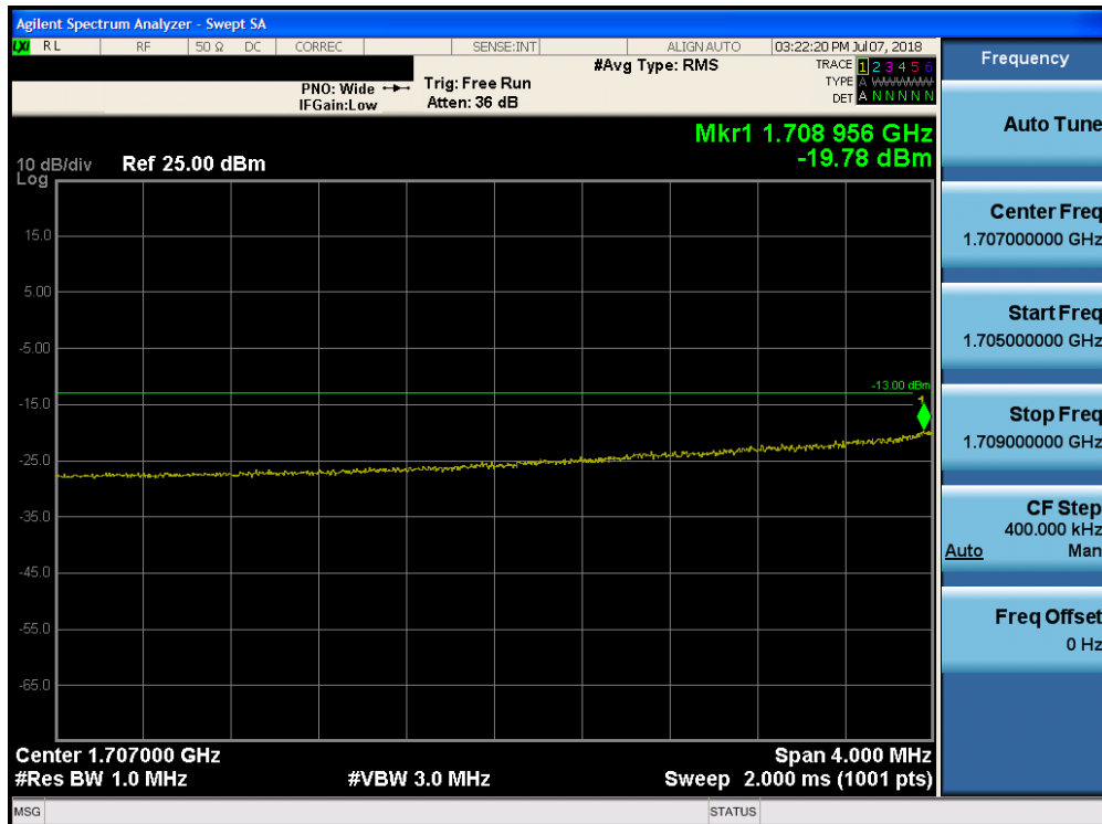
Plot 7-207. Lower Extended Band Edge Plot (Band 4 - 10.0MHz QPSK - Full RB Configuration)
