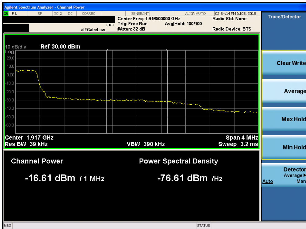
Plot 7-225. Upper Extended Band Edge Plot (Band 25 - 3.0MHz QPSK - Full RB Configuration)
