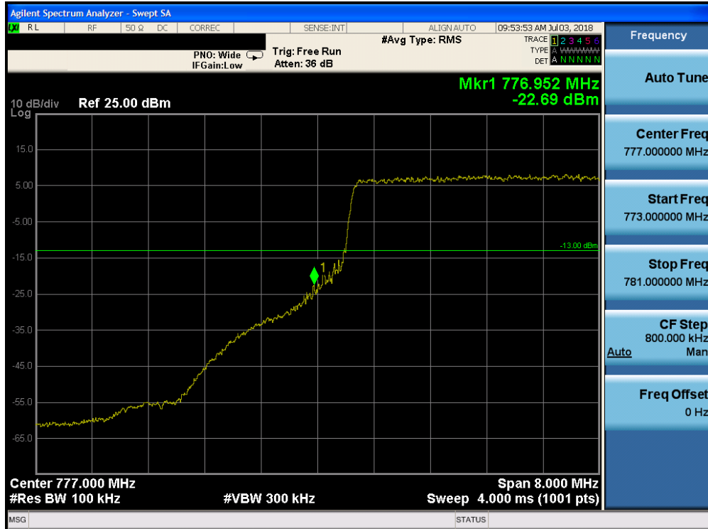
Plot 7-174. Lower Band Edge Plot (Band 13 - 10.0MHz QPSK - Full RB Configuration)
