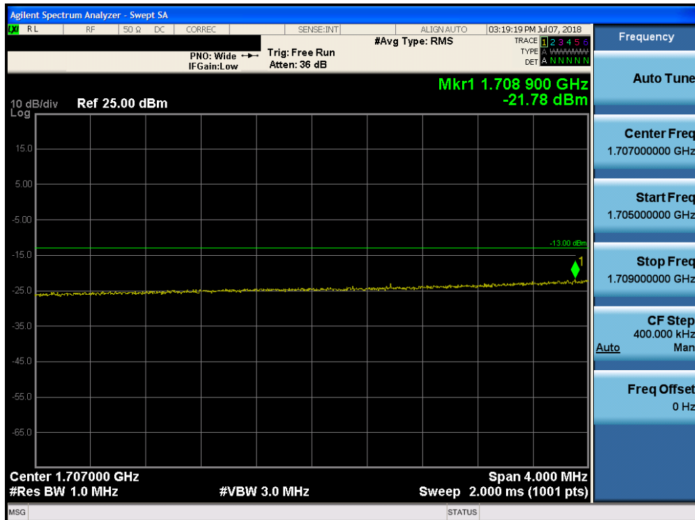
Plot 7-215. Lower Extended Band Edge Plot (Band 4 - 20.0MHz QPSK - Full RB Configuration)
