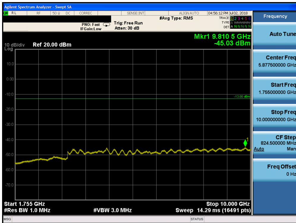
Plot 7-123. Conducted Spurious Plot (Band 4 - 20.0MHz QPSK - RB Size 1, RB Offset 0 - Low Channel)
