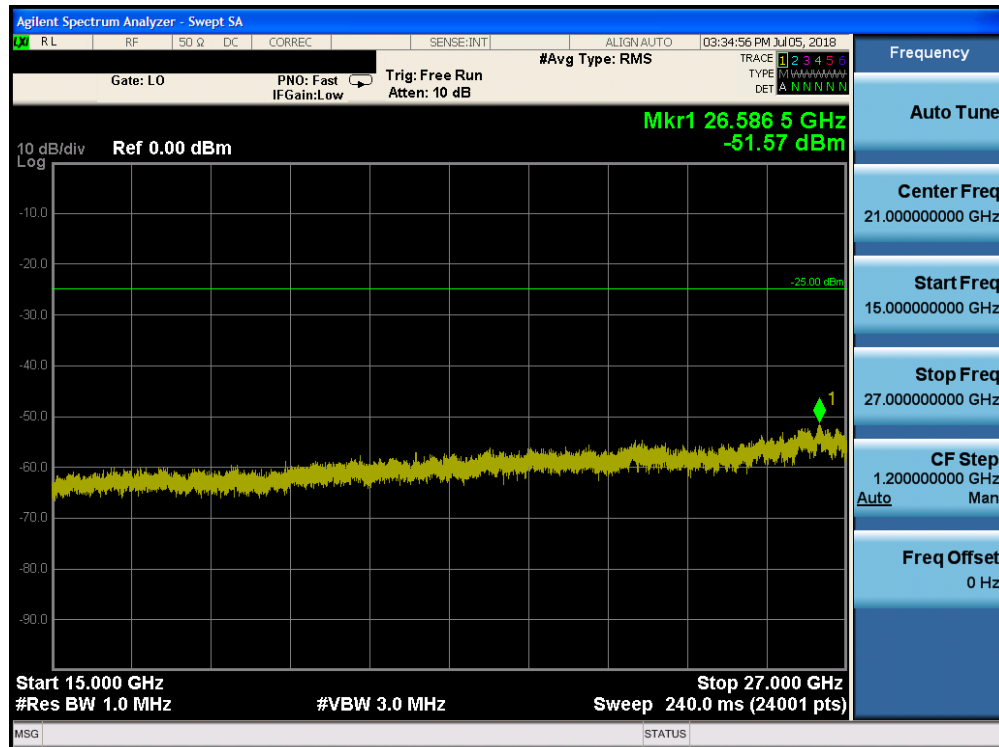
Plot 7-157. Conducted Spurious Plot (Band 41 - 20.0MHz QPSK - RB Size 1, RB Offset 0 - High Channel)
