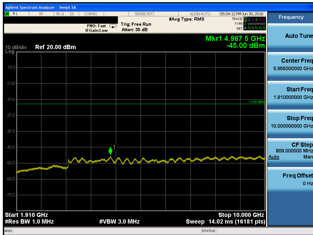
Plot 7-141. Conducted Spurious Plot (Band 2 - 20.0MHz QPSK - RB Size 1, RB Offset 0 - Low Channel)
