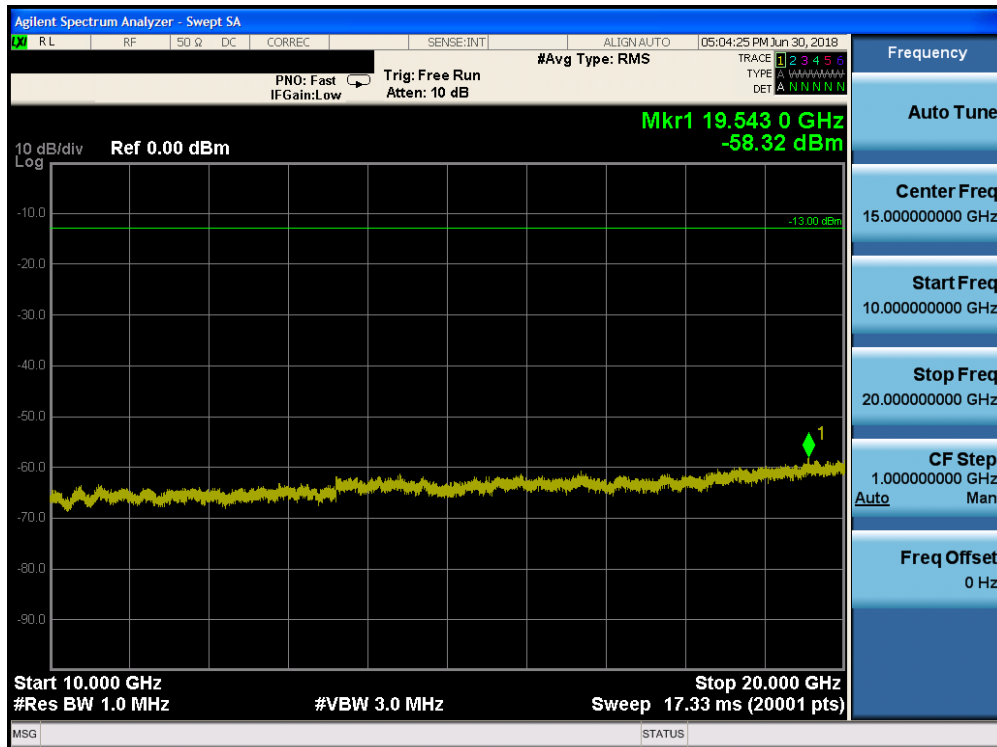
Plot 7-142. Conducted Spurious Plot (Band 2 - 20.0MHz QPSK - RB Size 1, RB Offset 0 - Low Channel)
