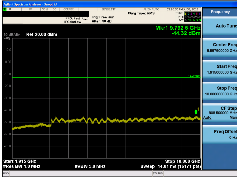
Plot 7-135. Conducted Spurious Plot (Band 25 - 20.0MHz QPSK - RB Size 1, RB Offset 0 - Mid Channel)
