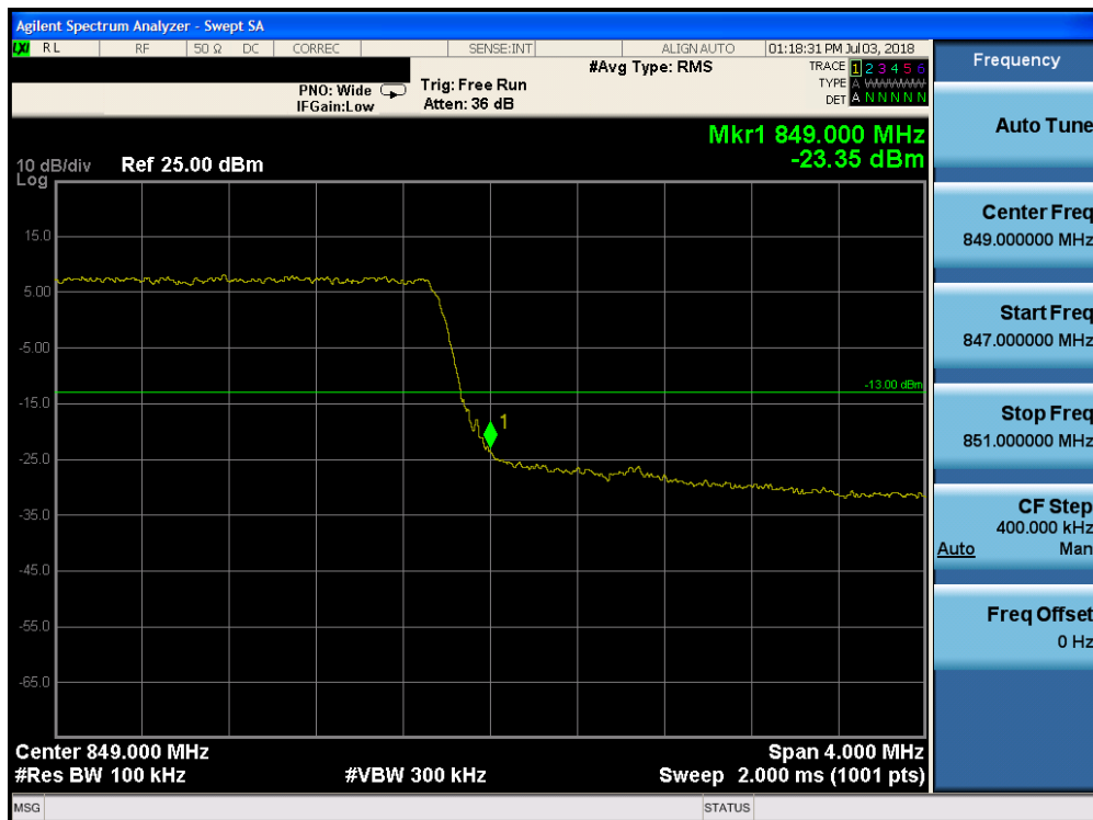
Plot 7-183. Upper Band Edge Plot (Band 26 - 5.0MHz QPSK - Full RB Configuration)
