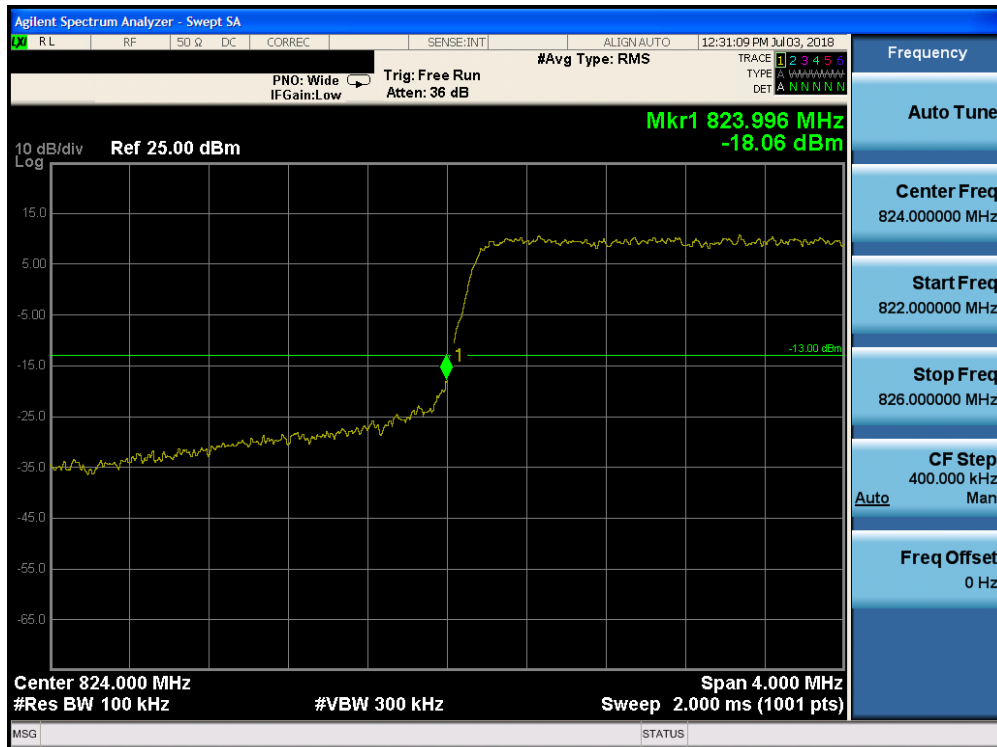
Plot 7-180. Lower Band Edge Plot (Band 26 - 3.0MHz QPSK - Full RB Configuration)
