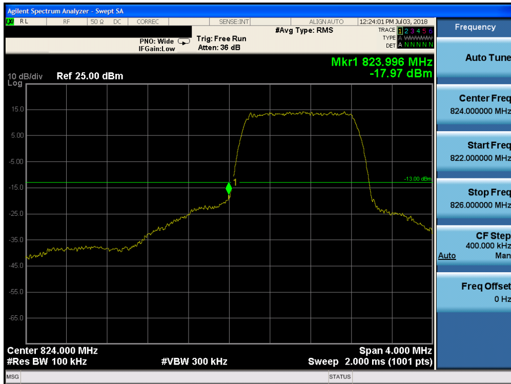
Plot 7-178. Lower Band Edge Plot (Band 26 - 1.4MHz QPSK - Full RB Configuration)
