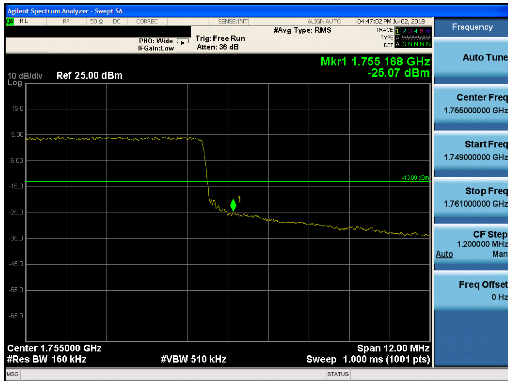
Plot 7-212. Upper Band Edge Plot (Band 4 - 15.0MHz QPSK - Full RB Configuration)
