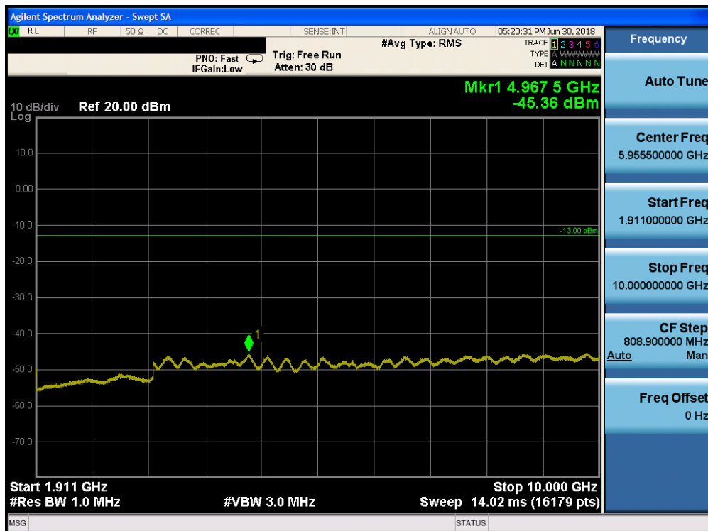
Plot 7-147. Conducted Spurious Plot (Band 2 - 20.0MHz QPSK - RB Size 1, RB Offset 0 - High Channel)
