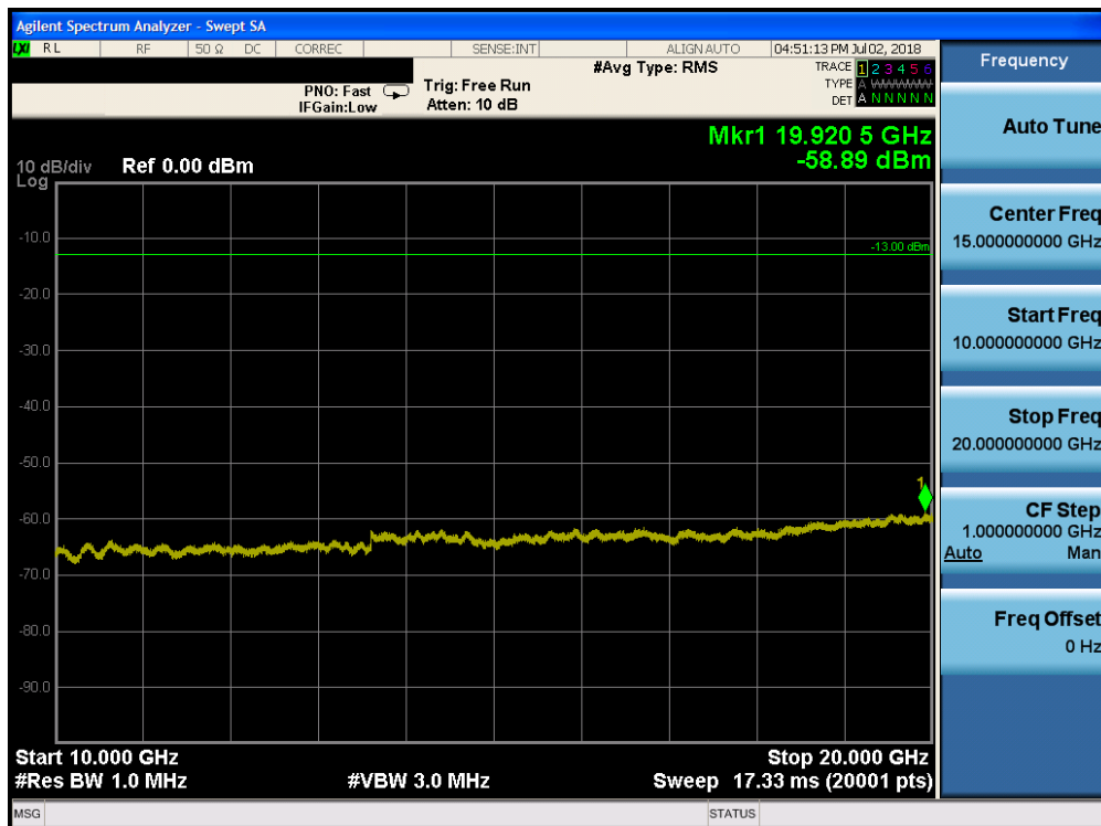
Plot 7-127. Conducted Spurious Plot (Band 4 - 20.0MHz QPSK - RB Size 1, RB Offset 0 - Mid Channel)
