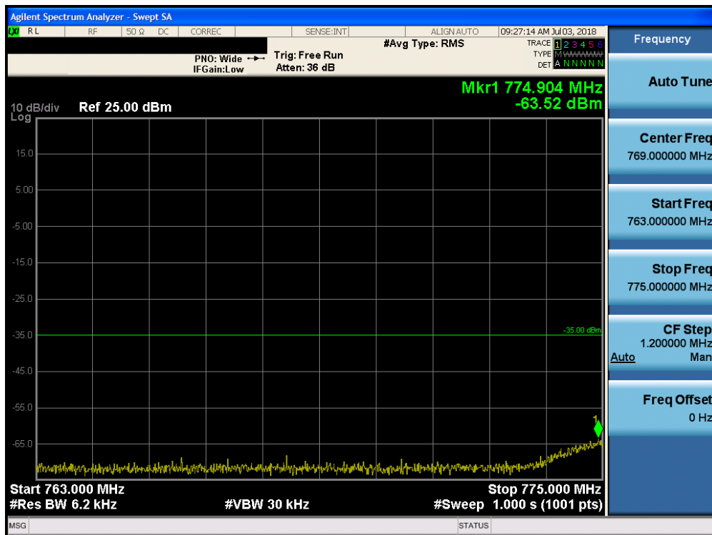
Plot 7-171. Lower Emission Mask Edge Plot (Band 13 - 5.0MHz QPSK - Full RB Configuration)
