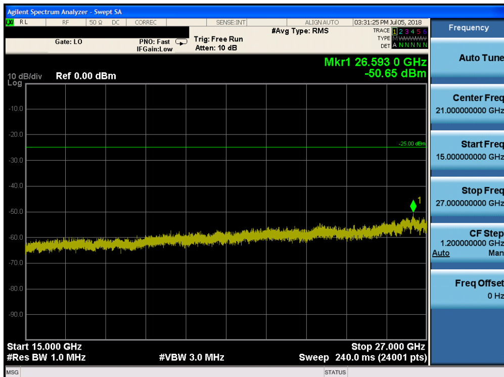
Plot 7-154. Conducted Spurious Plot (Band 41 - 20.0MHz QPSK - RB Size 1, RB Offset 0 - Mid Channel)
