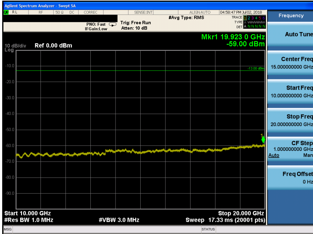
Plot 7-130. Conducted Spurious Plot (Band 4 - 20.0MHz QPSK - RB Size 1, RB Offset 0 - High Channel)
