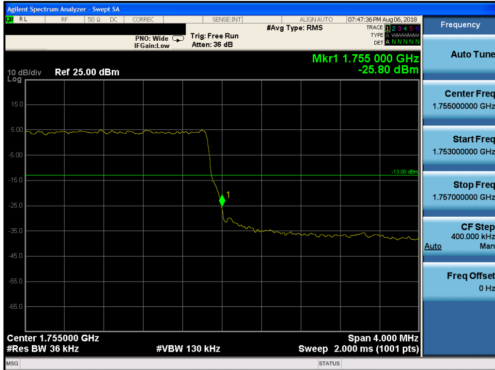
Plot 7-200. Upper Band Edge Plot (Band 4 - 3.0MHz QPSK - Full RB Configuration)
