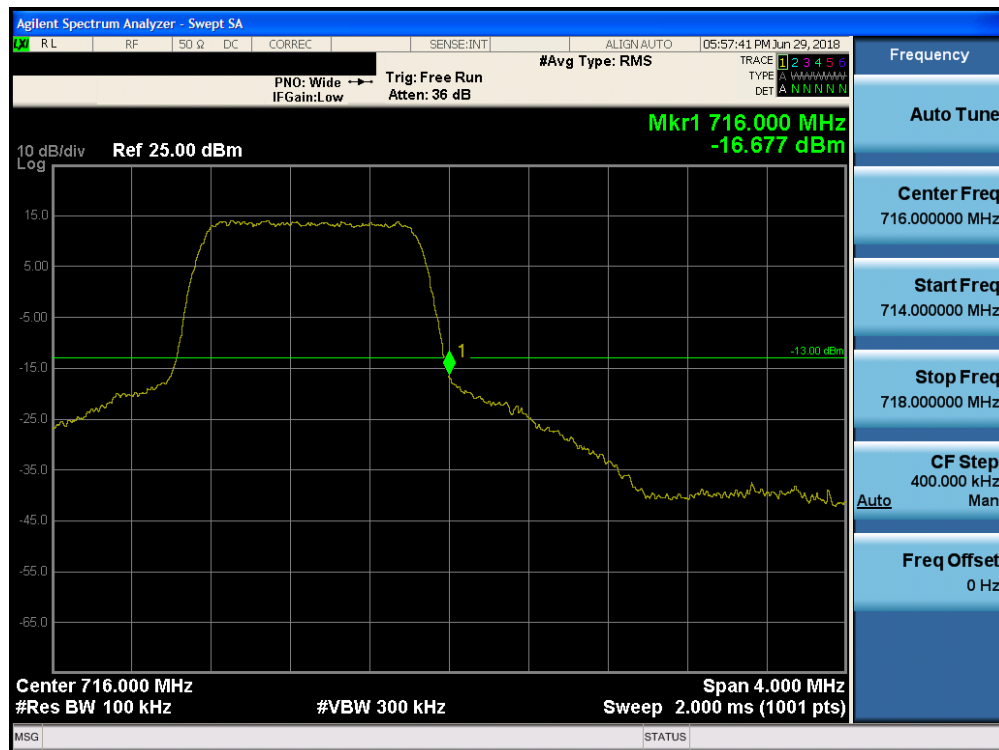
Plot 7-159. Upper Band Edge Plot (Band 12 - 1.4MHz QPSK - Full RB Configuration)
