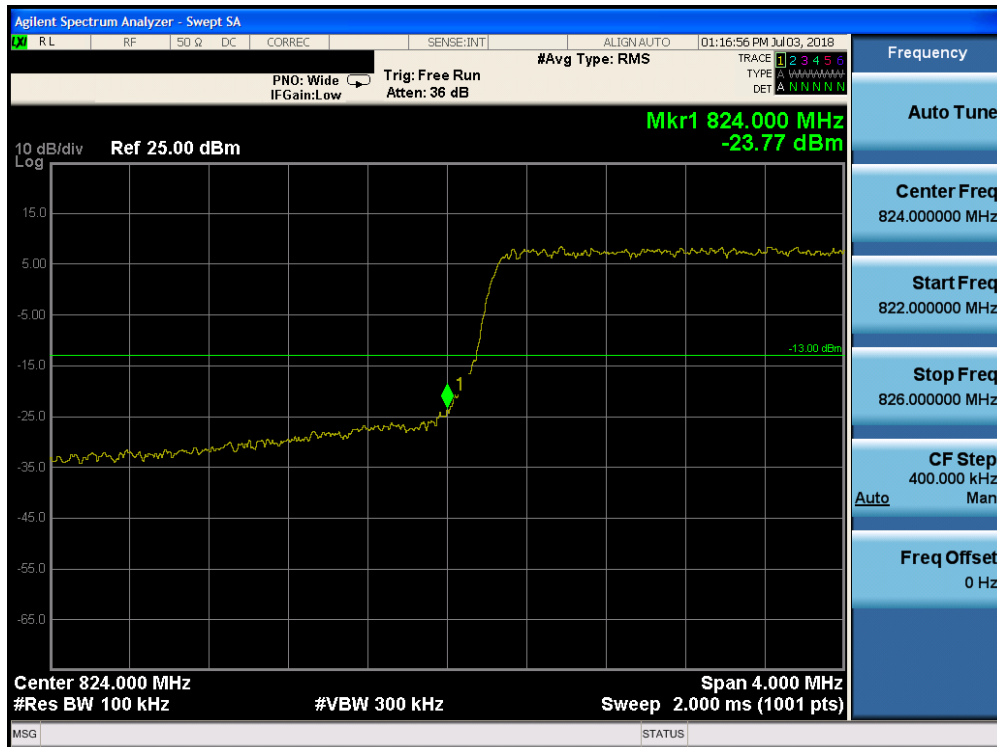
Plot 7-182. Lower Band Edge Plot (Band 26 - 5.0MHz QPSK - Full RB Configuration)
