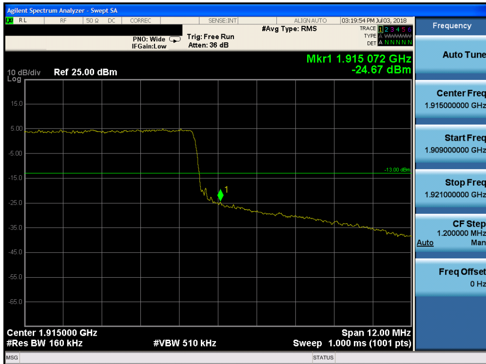
Plot 7-236. Upper Band Edge Plot (Band 25 - 15.0MHz QPSK - Full RB Configuration)
