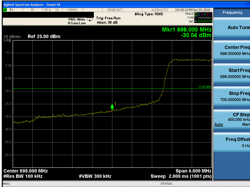
Plot 7-160. Lower Band Edge Plot (Band 12 - 3.0MHz QPSK - Full RB Configuration)
