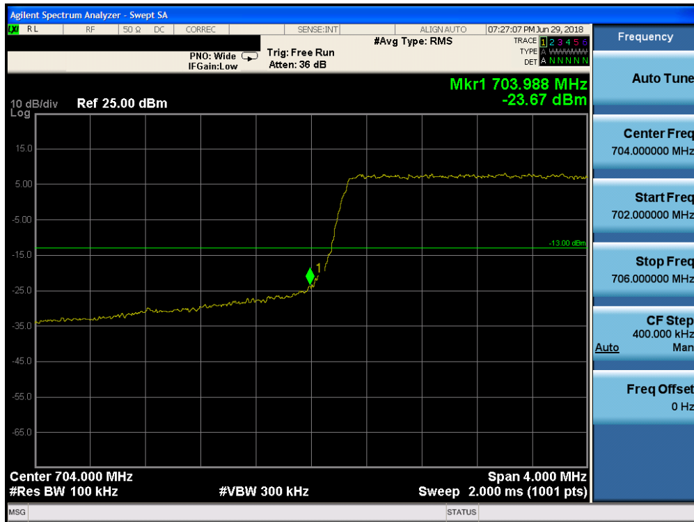
Plot 7-166. Lower Band Edge Plot (Band 17 - 5.0MHz QPSK - Full RB Configuration)
