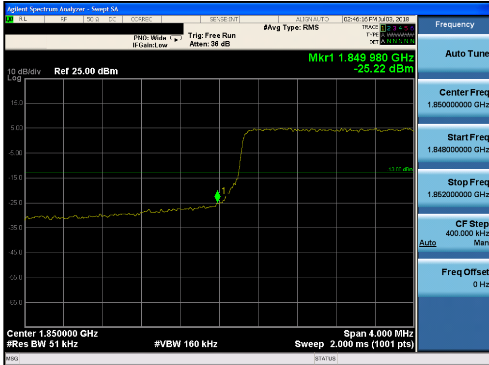
Plot 7-226. Lower Band Edge Plot (Band 25 - 5.0MHz QPSK - Full RB Configuration)
