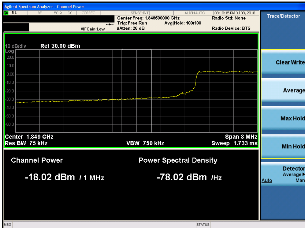
Plot 7-231. Lower Extended Band Edge Plot (Band 25 - 10.0MHz QPSK - Full RB Configuration)
