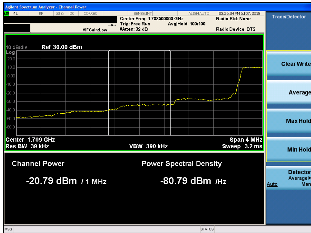
Plot 7-195. Lower Extended Band Edge Plot (Band 4 - 1.4MHz QPSK - Full RB Configuration)
