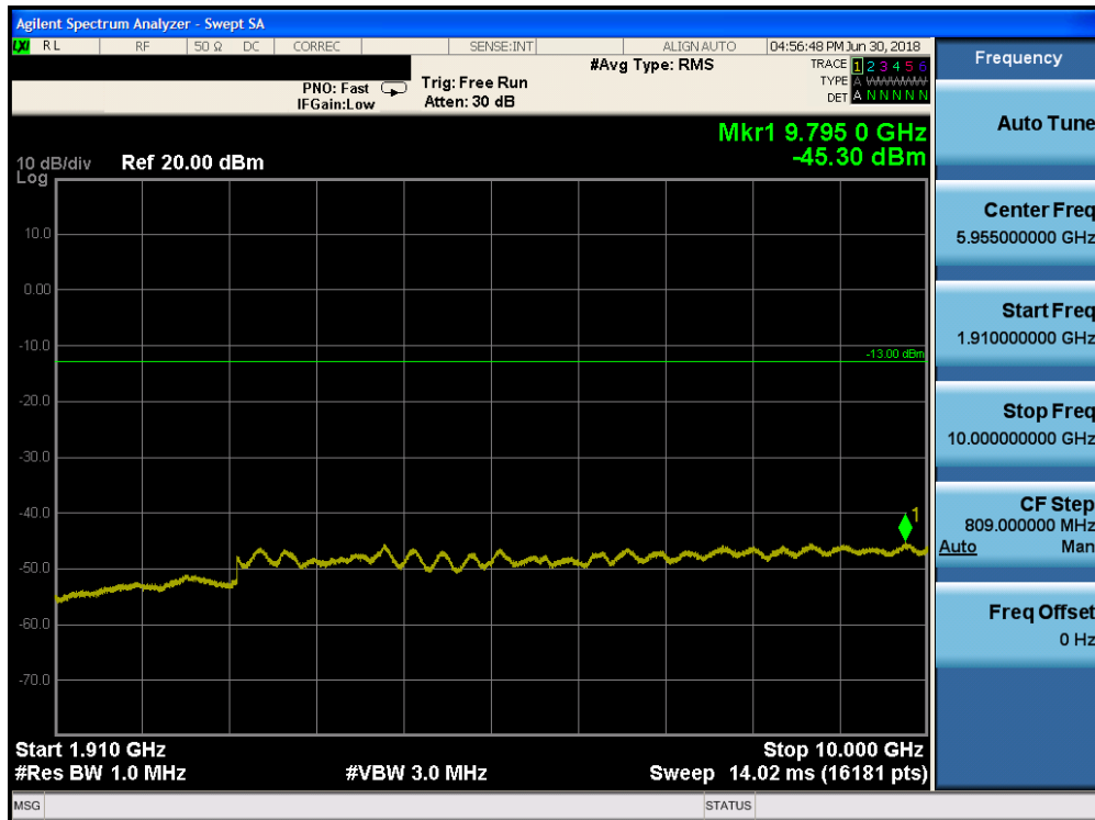
Plot 7-144. Conducted Spurious Plot (Band 2 - 20.0MHz QPSK - RB Size 1, RB Offset 0 - Mid Channel)
