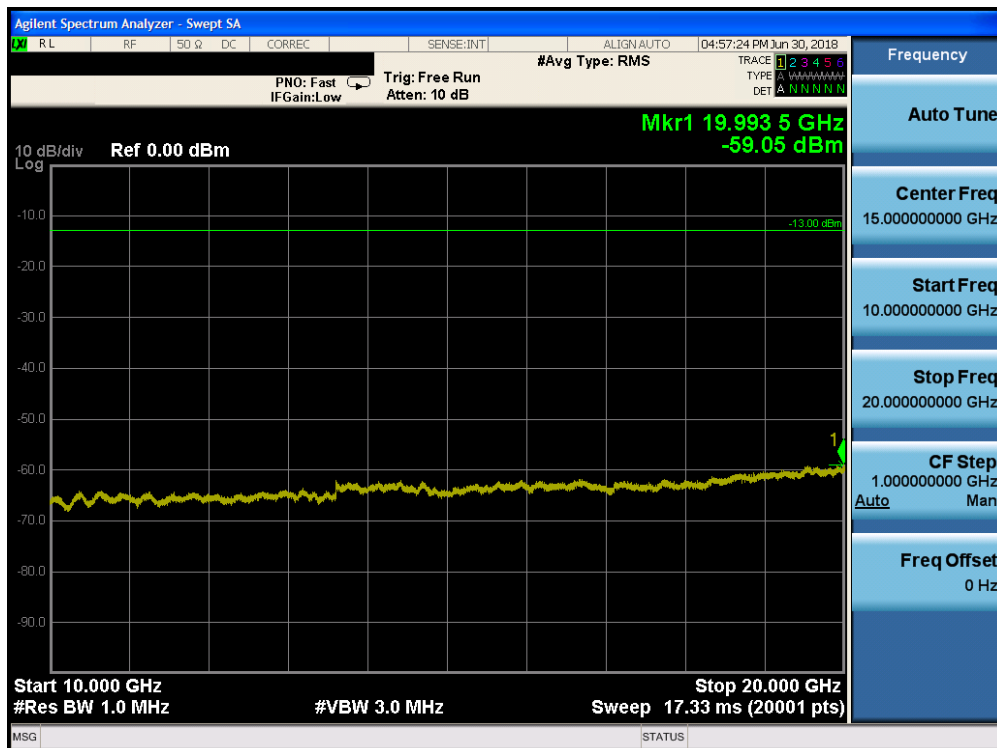
Plot 7-145. Conducted Spurious Plot (Band 2 - 20.0MHz QPSK - RB Size 1, RB Offset 0 - Mid Channel)
