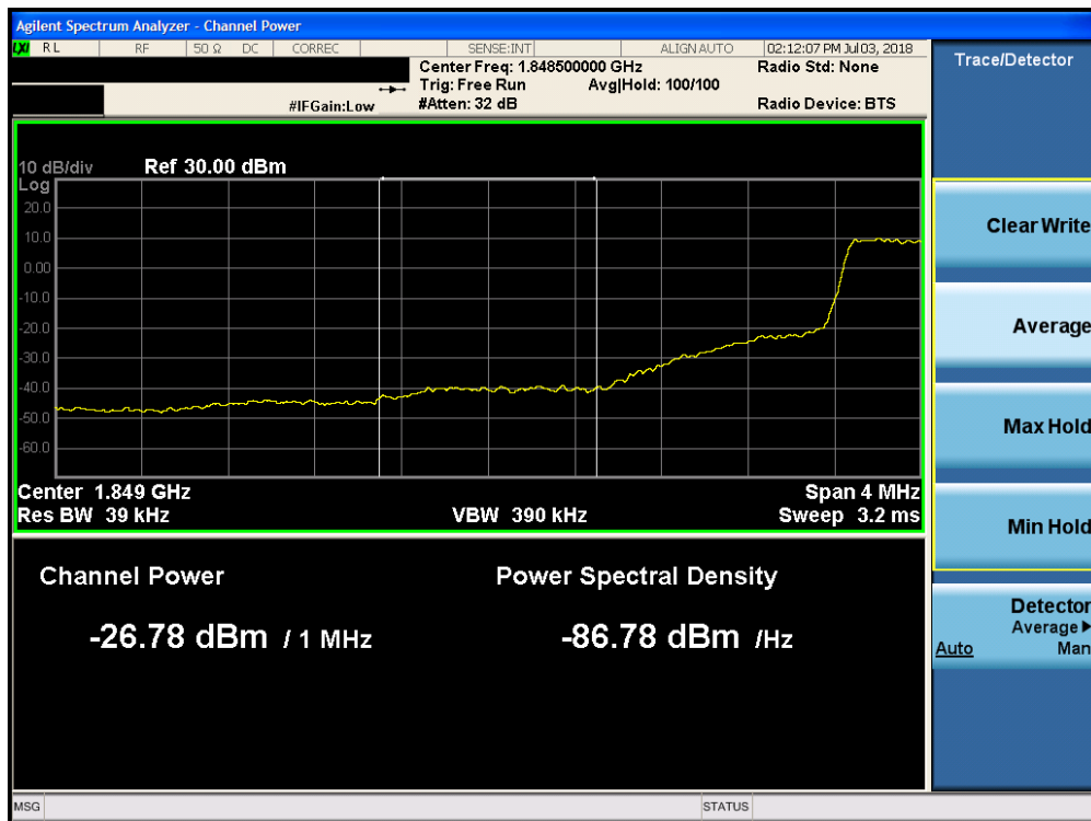
Plot 7-219. Lower Extended Band Edge Plot (Band 25 - 1.4MHz QPSK - Full RB Configuration)
