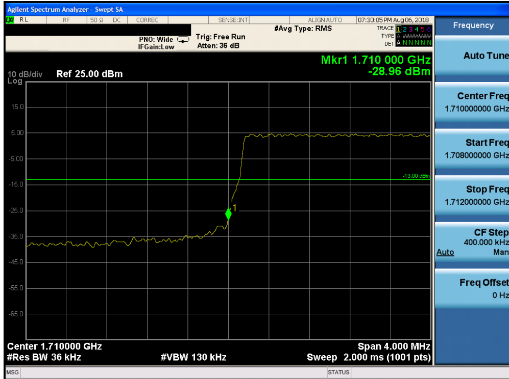
Plot 7-198. Lower Band Edge Plot (Band 4 - 3.0MHz QPSK - Full RB Configuration)
