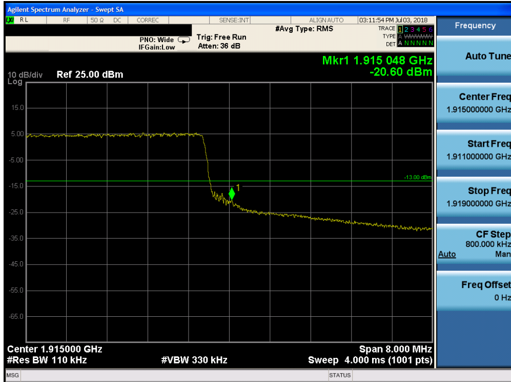
Plot 7-232. Upper Band Edge Plot (Band 25 - 10.0MHz QPSK - Full RB Configuration)
