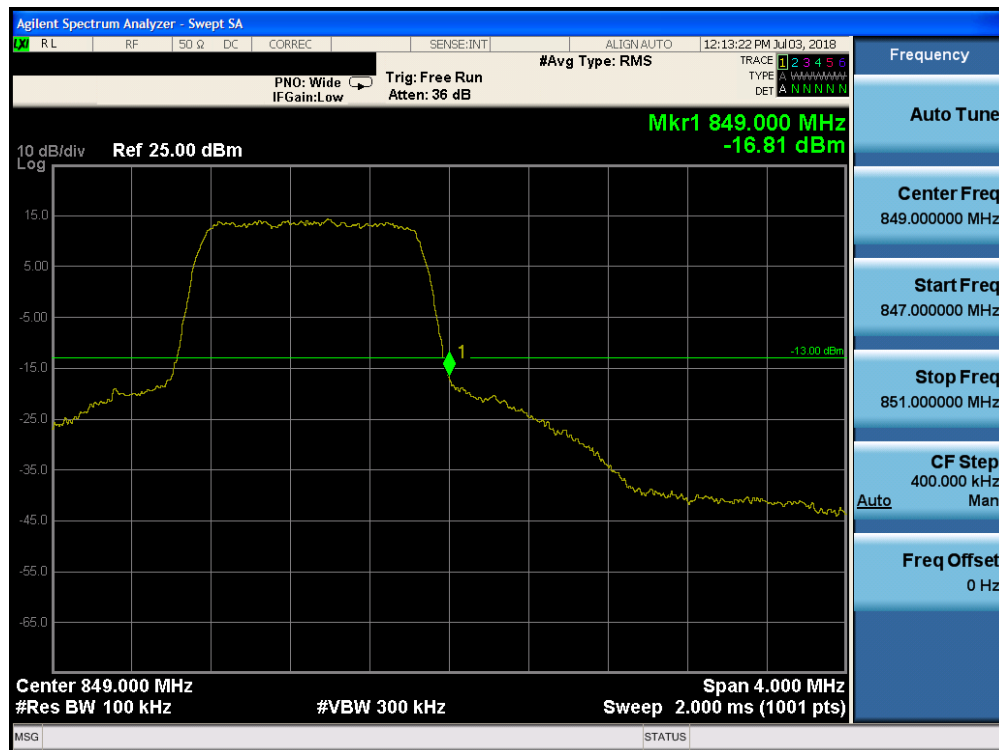
Plot 7-187. Upper Band Edge Plot (Band 5 - 1.4MHz QPSK - Full RB Configuration)
