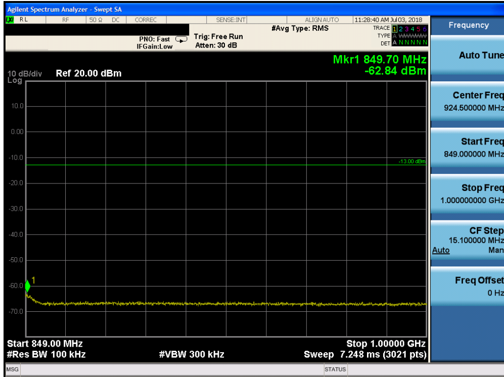
Plot 7-117. Conducted Spurious Plot (Band 5 - 10.0MHz QPSK - RB Size 1, RB Offset 0 - Mid Channel)
