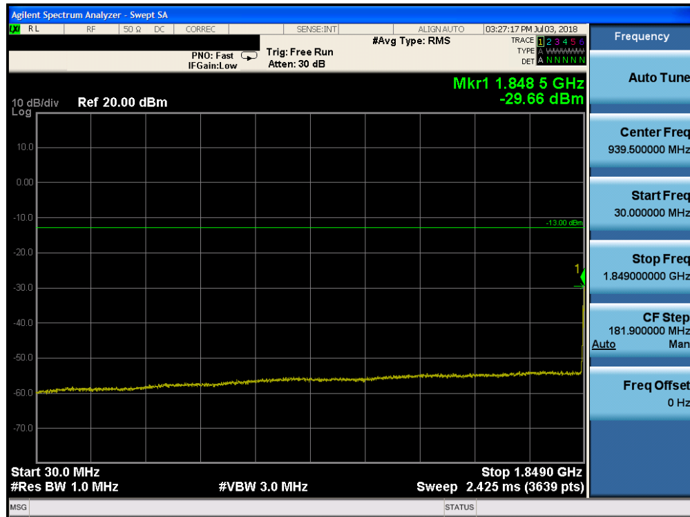
Plot 7-131. Conducted Spurious Plot (Band 25 - 20.0MHz QPSK - RB Size 1, RB Offset 0 - Low Channel)
