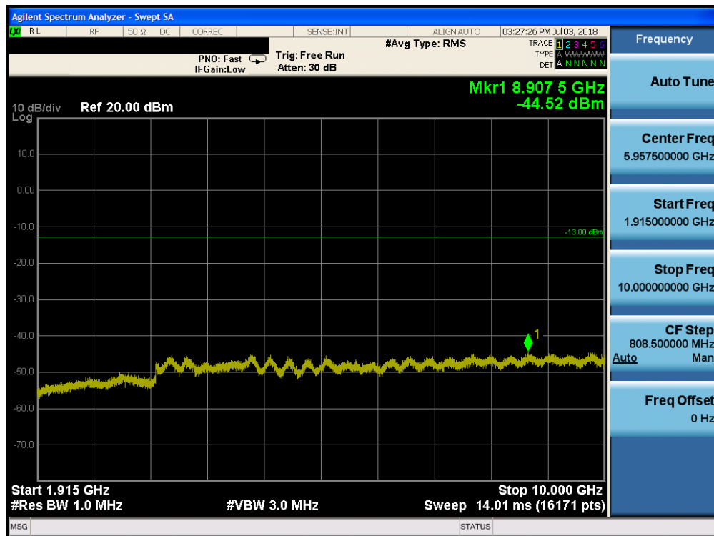
Plot 7-132. Conducted Spurious Plot (Band 25 - 20.0MHz QPSK - RB Size 1, RB Offset 0 - Low Channel)
