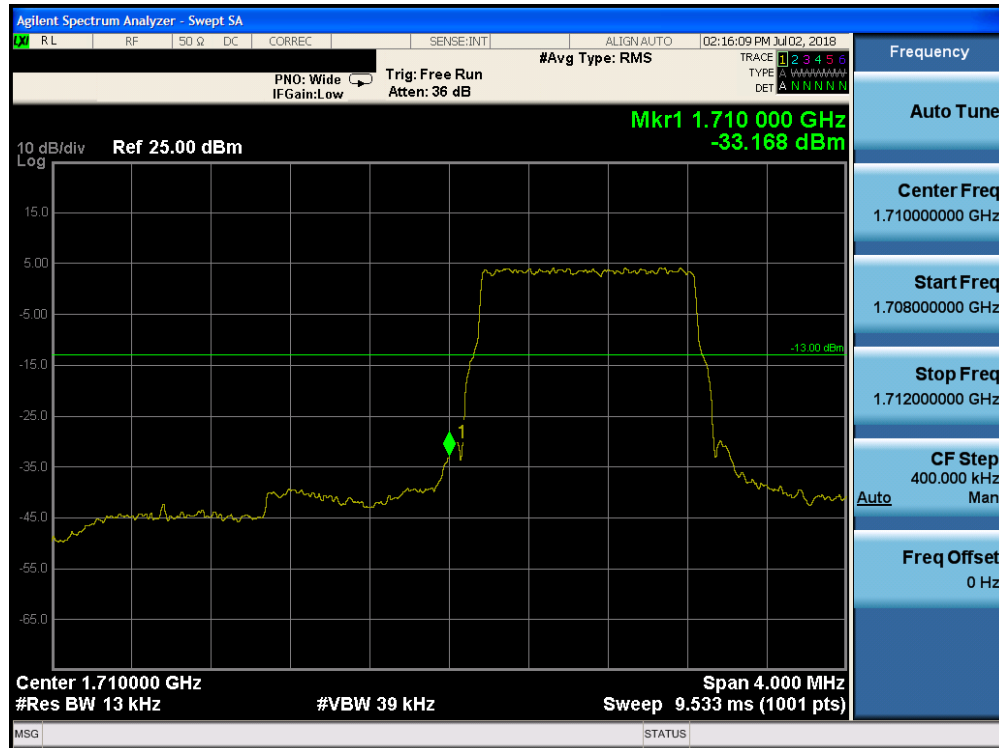
Plot 7-194. Lower Band Edge Plot (Band 4 - 1.4MHz QPSK - Full RB Configuration)
