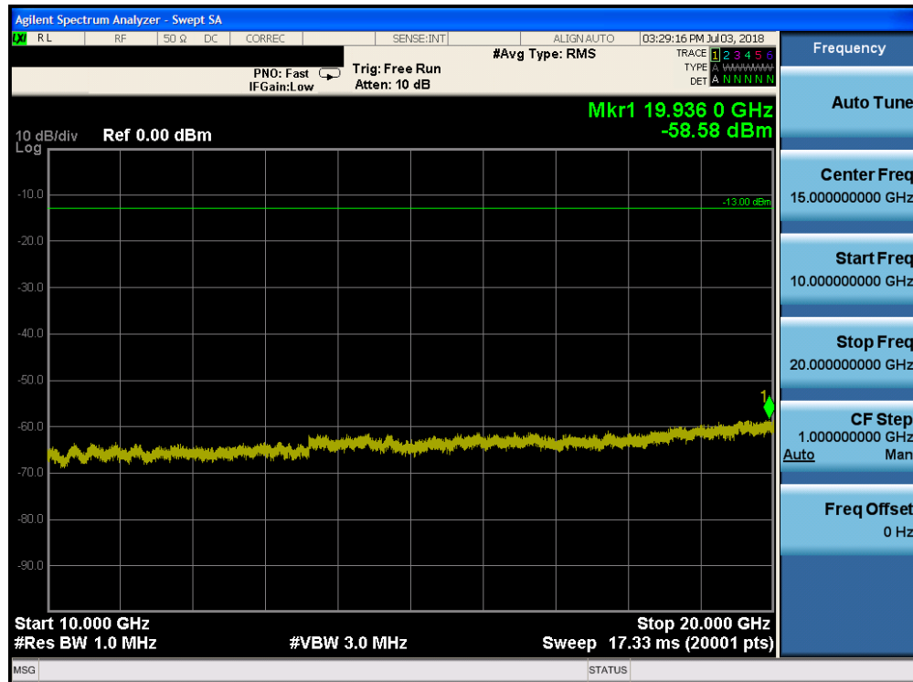
Plot 7-139. Conducted Spurious Plot (Band 25 - 20.0MHz QPSK - RB Size 1, RB Offset 0 - High Channel)
