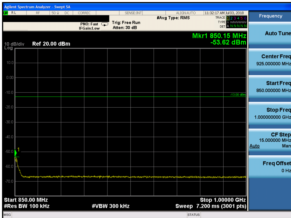
Plot 7-120. Conducted Spurious Plot (Band 5 - 10.0MHz QPSK - RB Size 1, RB Offset 0 - High Channel)
