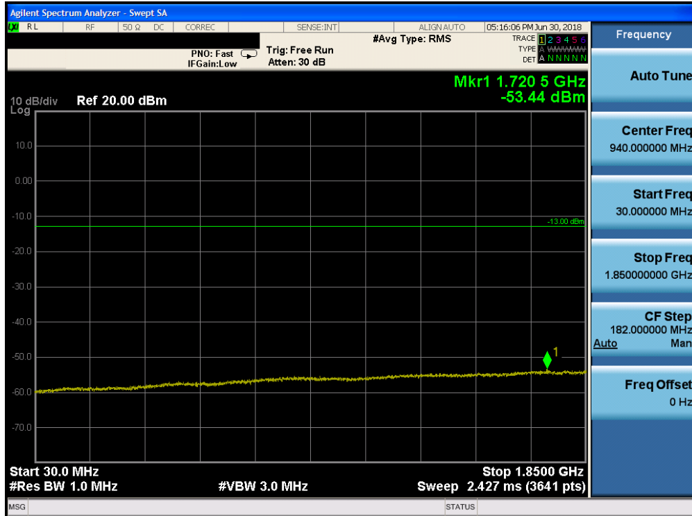
Plot 7-146. Conducted Spurious Plot (Band 2 - 20.0MHz QPSK - RB Size 1, RB Offset 0 - High Channel)
