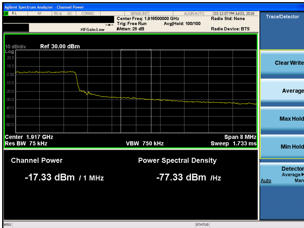
Plot 7-233. Upper Extended Band Edge Plot (Band 25 - 10.0MHz QPSK - Full RB Configuration)
