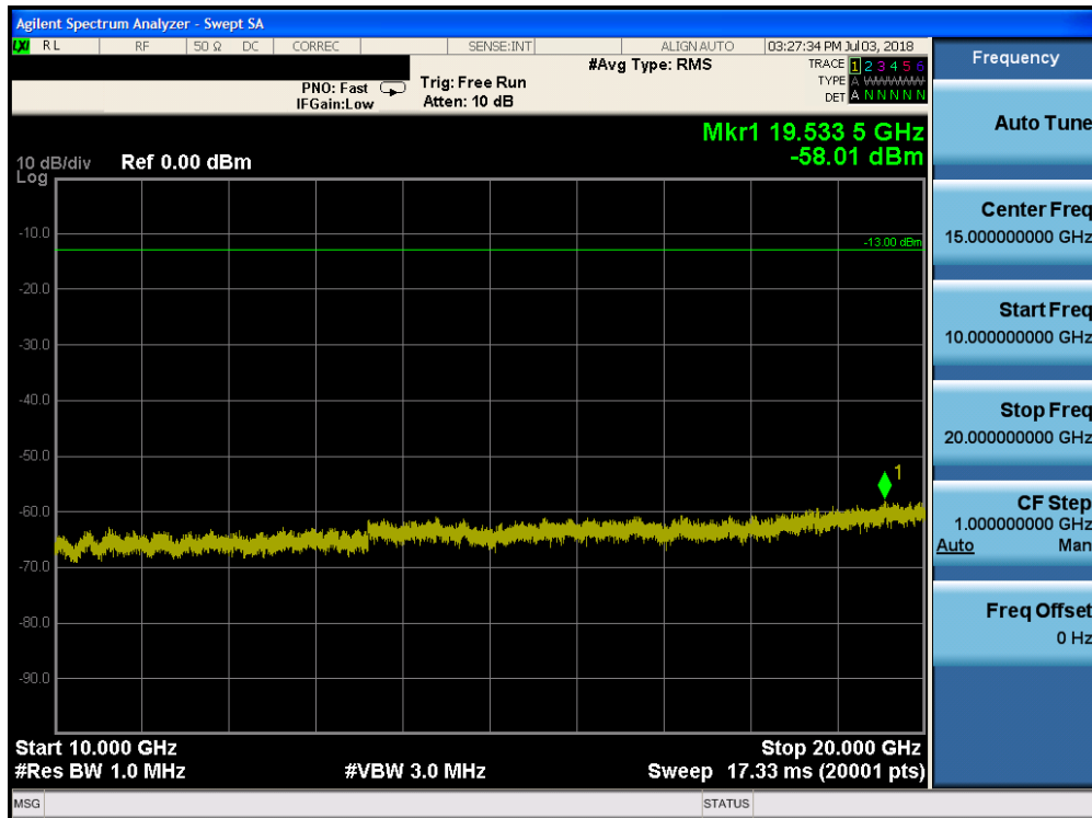
Plot 7-133. Conducted Spurious Plot (Band 25 - 20.0MHz QPSK - RB Size 1, RB Offset 0 - Low Channel)
