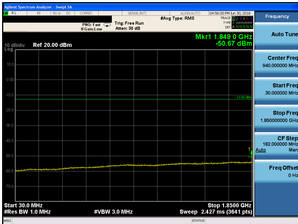
Plot 7-143. Conducted Spurious Plot (Band 2 - 20.0MHz QPSK - RB Size 1, RB Offset 0 - Mid Channel)
