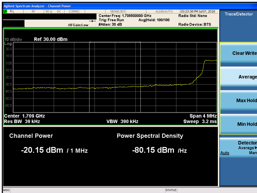
Plot 7-203. Lower Extended Band Edge Plot (Band 4 - 5.0MHz QPSK - Full RB Configuration)
