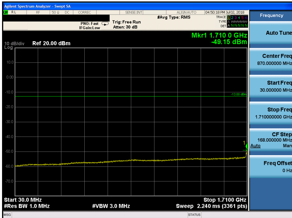
Plot 7-125. Conducted Spurious Plot (Band 4 - 20.0MHz QPSK - RB Size 1, RB Offset 0 - Mid Channel)
