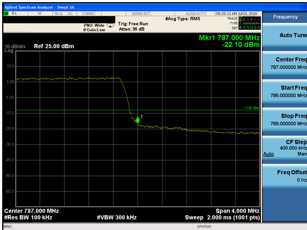
Plot 7-172. Upper Band Edge Plot (Band 13 - 5.0MHz QPSK - Full RB Configuration)
