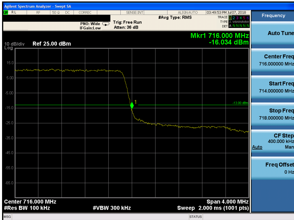
Plot 7-161. Upper Band Edge Plot (Band 12 - 3.0MHz QPSK - Full RB Configuration)
