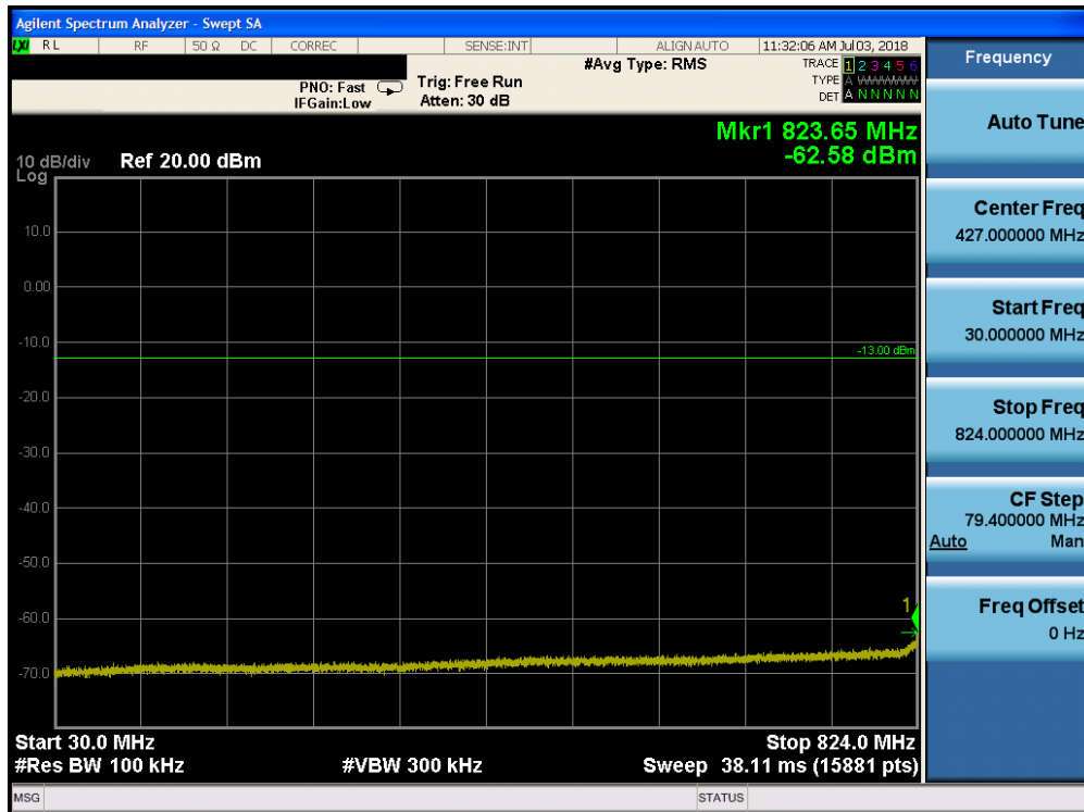
Plot 7-119. Conducted Spurious Plot (Band 5 - 10.0MHz QPSK - RB Size 1, RB Offset 0 - High Channel)
