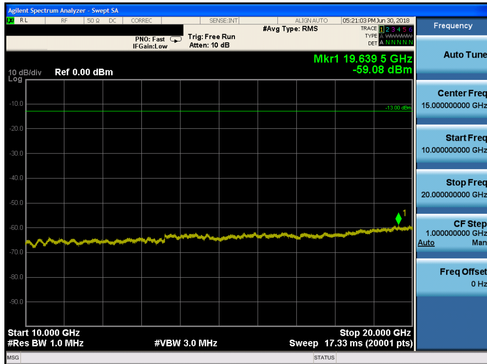
Plot 7-148. Conducted Spurious Plot (Band 2 - 20.0MHz QPSK - RB Size 1, RB Offset 0 - High Channel)
