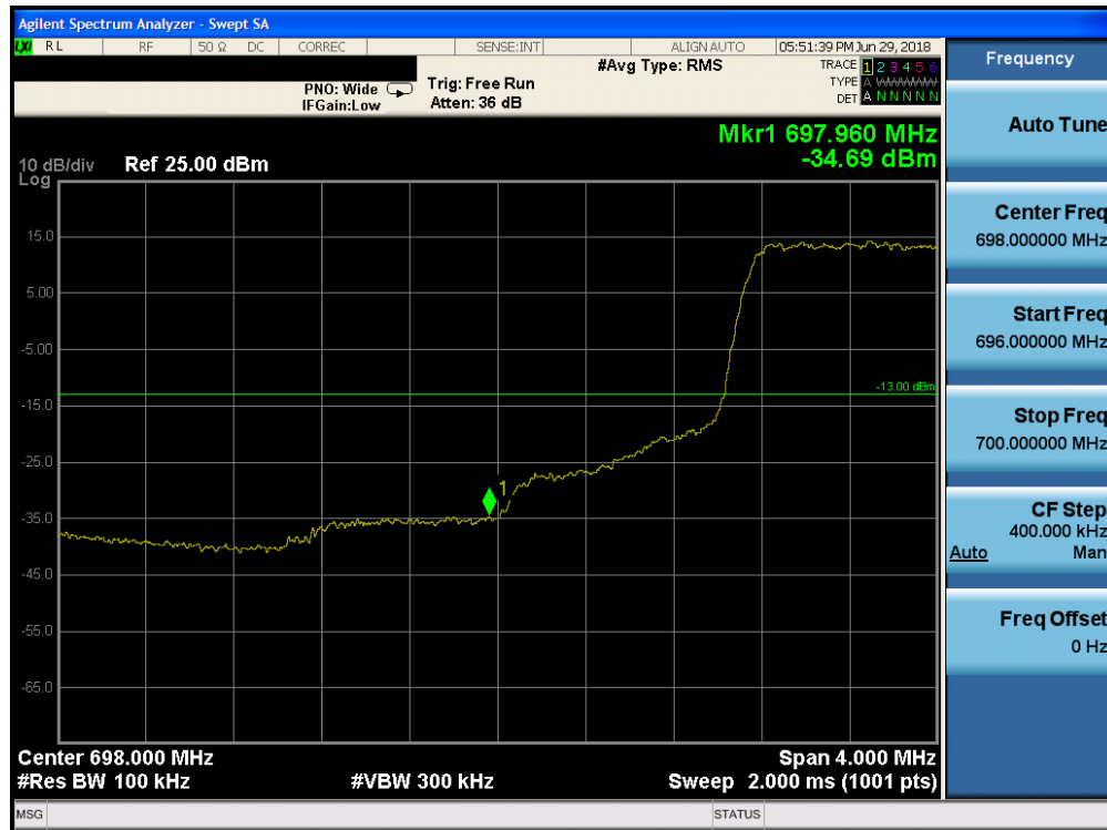
Plot 7-158. Lower Band Edge Plot (Band 12 - 1.4MHz QPSK - Full RB Configuration)
