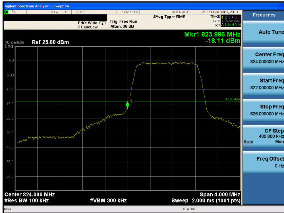
Plot 7-186. Lower Band Edge Plot (Band 5 - 1.4MHz QPSK - Full RB Configuration)
