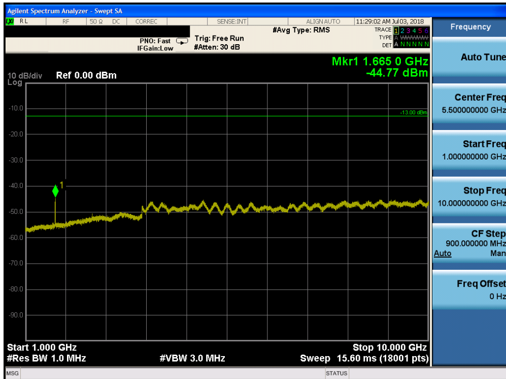
Plot 7-118. Conducted Spurious Plot (Band 5 - 10.0MHz QPSK - RB Size 1, RB Offset 0 - Mid Channel)
