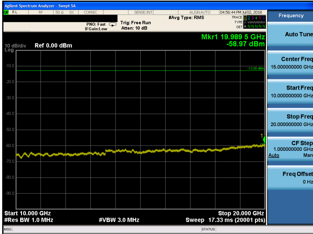
Plot 7-124. Conducted Spurious Plot (Band 4 - 20.0MHz QPSK - RB Size 1, RB Offset 0 - Low Channel)
