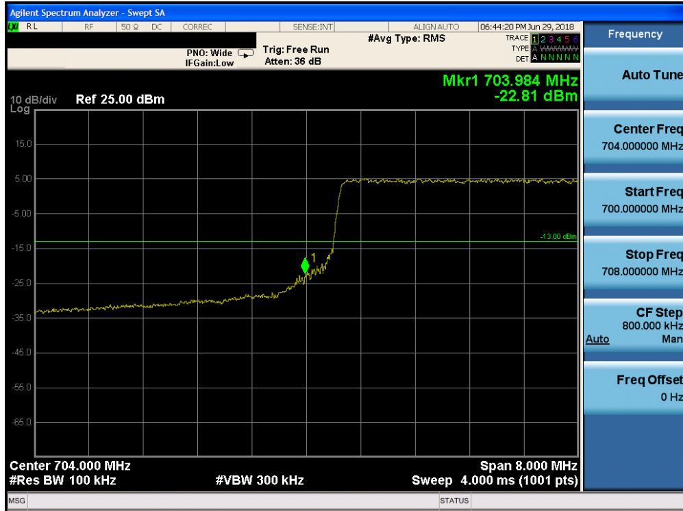
Plot 7-168. Lower Band Edge Plot (Band 17 - 10.0MHz QPSK - Full RB Configuration)
