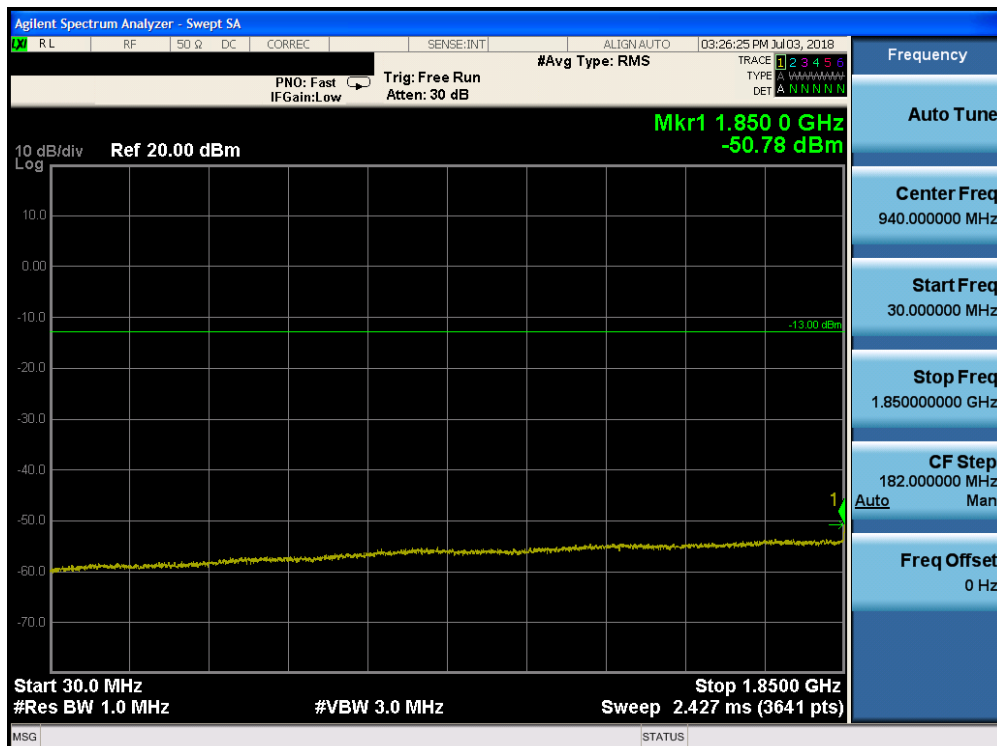
Plot 7-134. Conducted Spurious Plot (Band 25 - 20.0MHz QPSK - RB Size 1, RB Offset 0 - Mid Channel)
