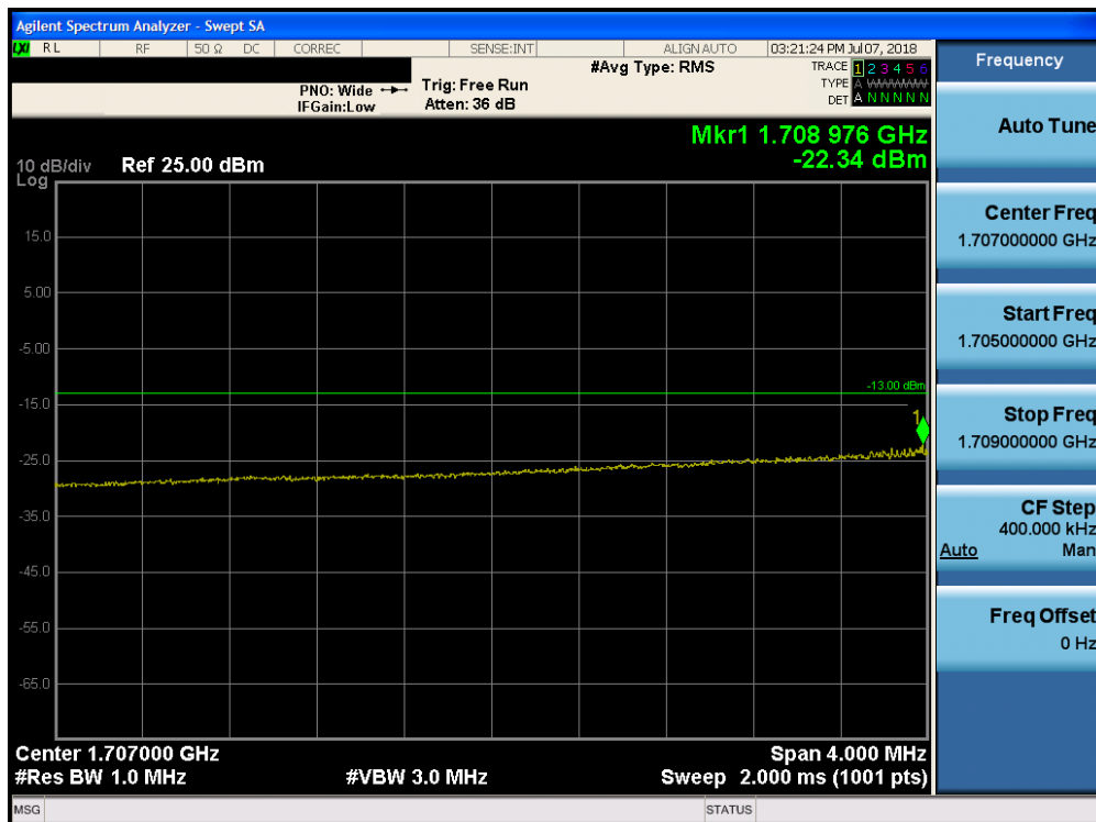
Plot 7-211. Lower Extended Band Edge Plot (Band 4 - 15.0MHz QPSK - Full RB Configuration)
