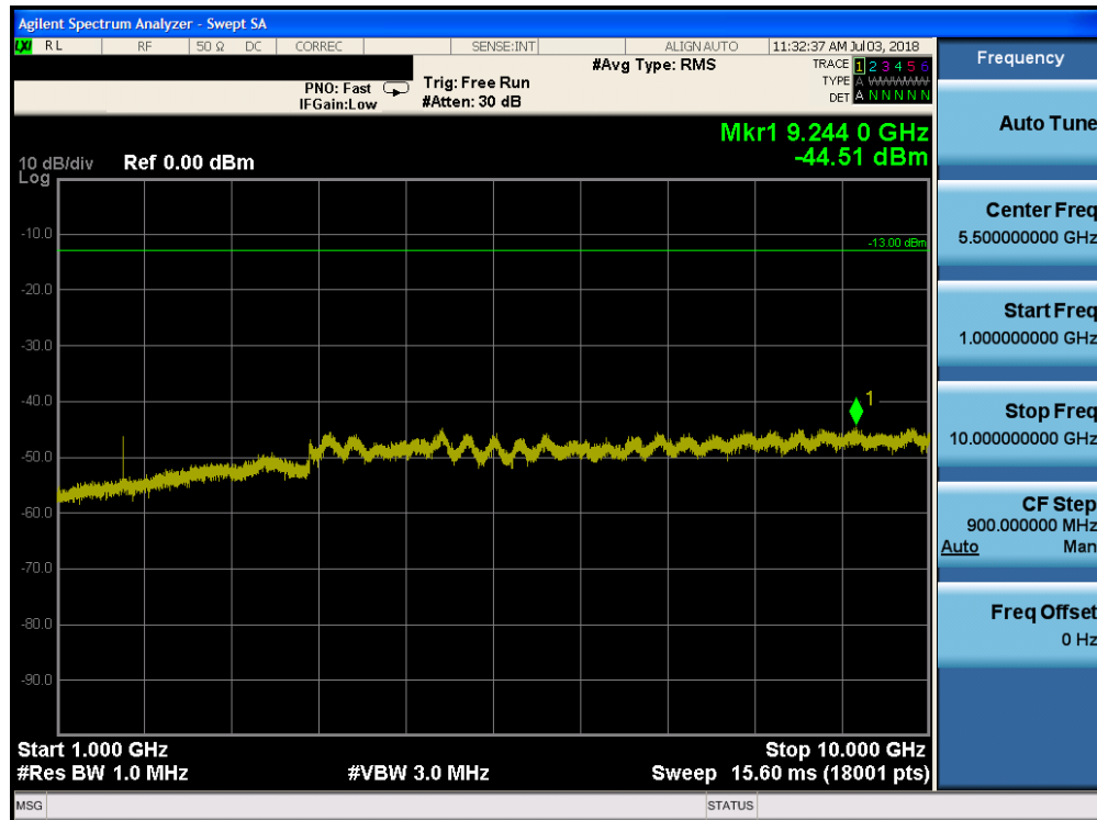
Plot 7-121. Conducted Spurious Plot (Band 5 - 10.0MHz QPSK - RB Size 1, RB Offset 0 - High Channel)
