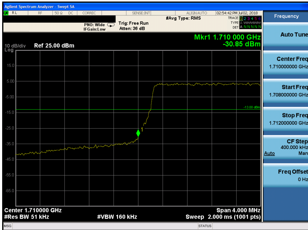
Plot 7-202. Lower Band Edge Plot (Band 4 - 5.0MHz QPSK - Full RB Configuration)
