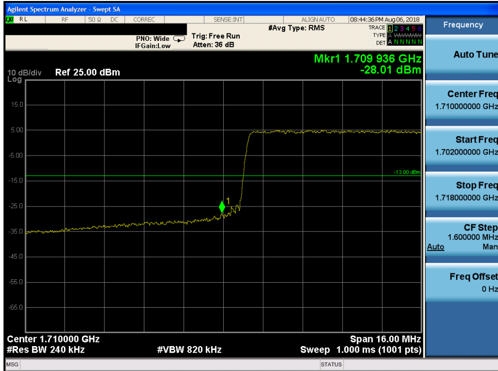
Plot 7-214. Lower Band Edge Plot (Band 4 - 20.0MHz QPSK - Full RB Configuration)
