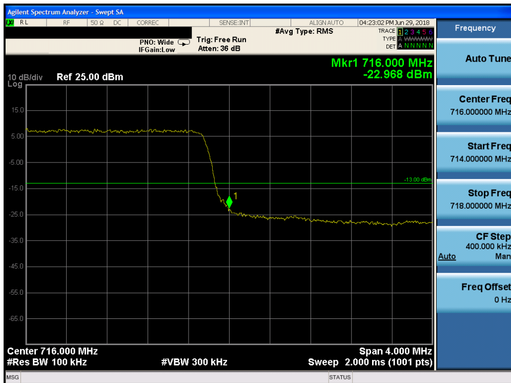
Plot 7-163. Upper Band Edge Plot (Band 12 - 5.0MHz QPSK - Full RB Configuration)
