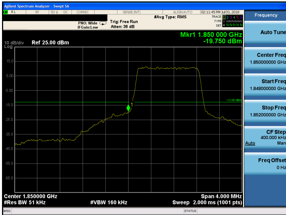
Plot 7-218. Lower Band Edge Plot (Band 25 - 1.4MHz QPSK - Full RB Configuration)
