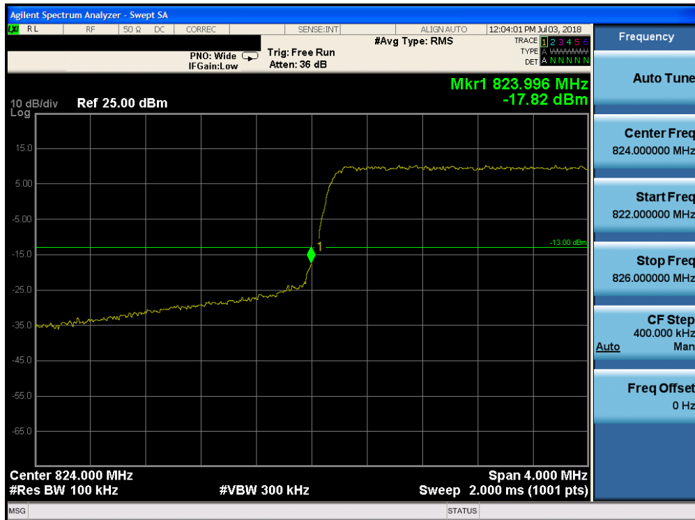
Plot 7-188. Lower Band Edge Plot (Band 5 - 3.0MHz QPSK - Full RB Configuration)
