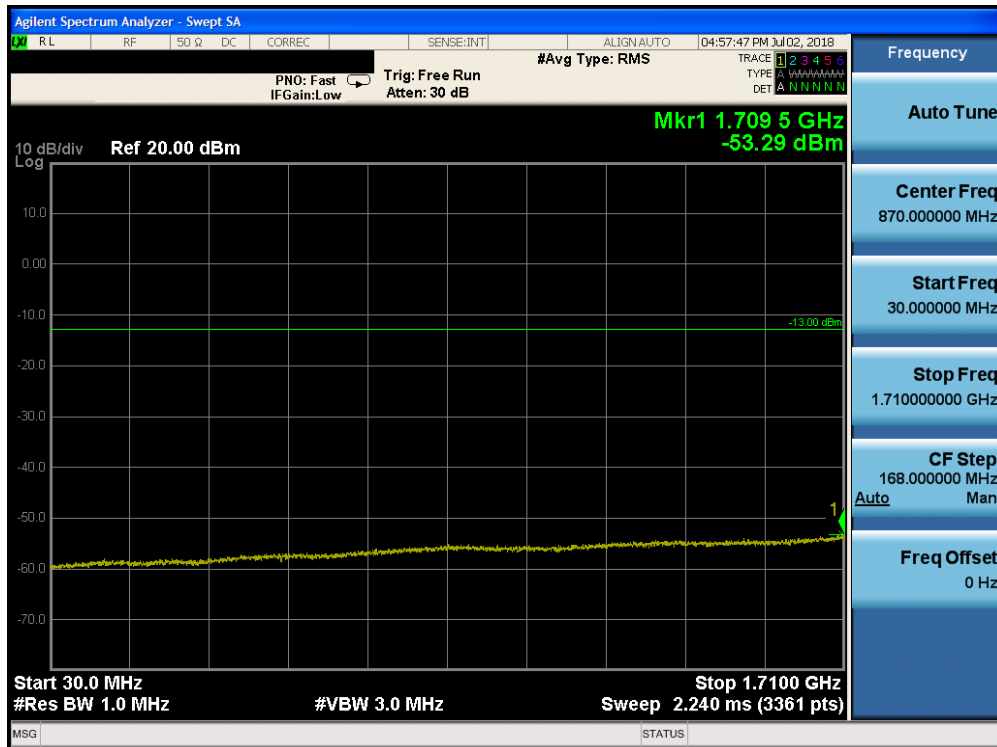
Plot 7-128. Conducted Spurious Plot (Band 4 - 20.0MHz QPSK - RB Size 1, RB Offset 0 - High Channel)
