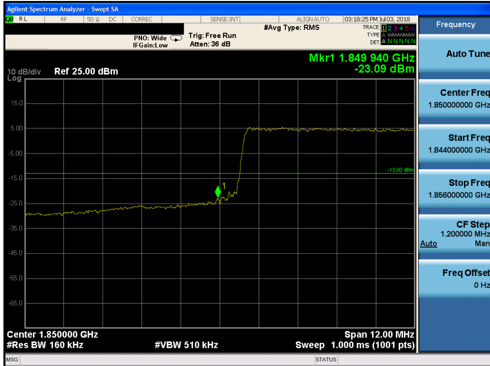
Plot 7-234. Lower Band Edge Plot (Band 25 - 15.0MHz QPSK - Full RB Configuration)
