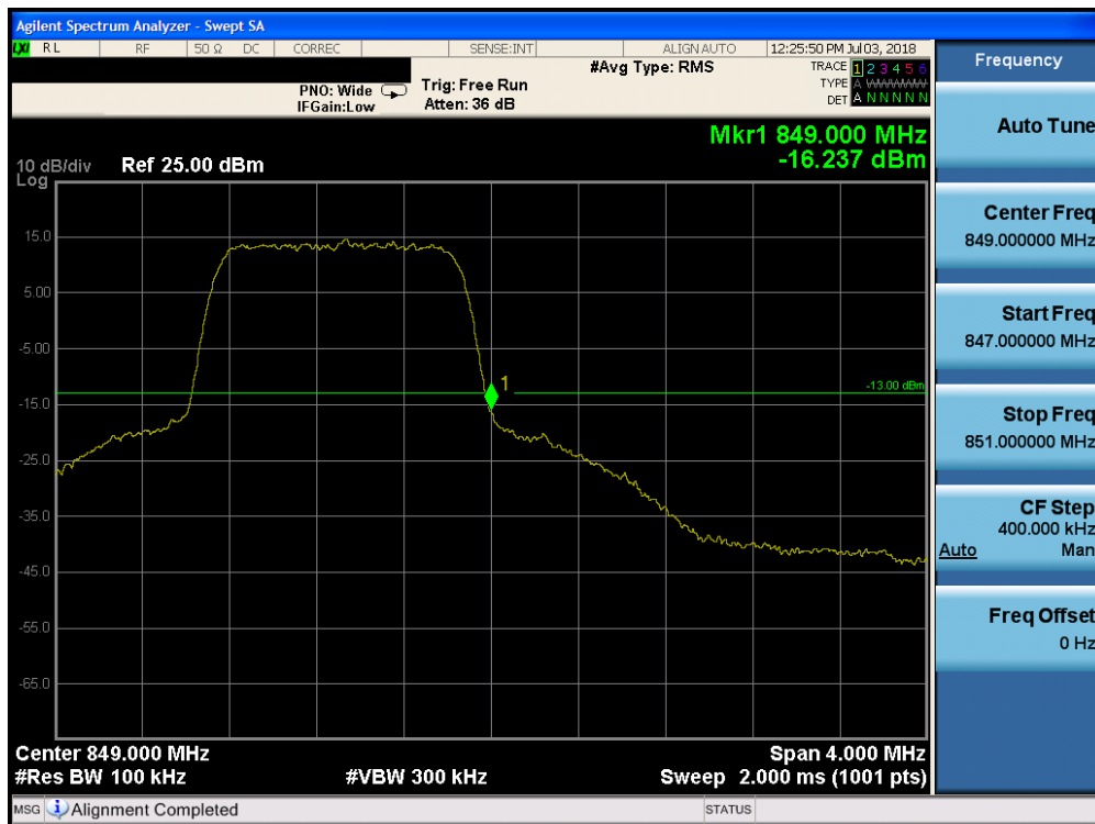
Plot 7-179. Upper Band Edge Plot (Band 26 - 1.4MHz QPSK - Full RB Configuration)
