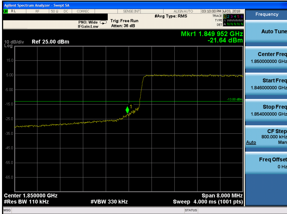
Plot 7-230. Lower Band Edge Plot (Band 25 - 10.0MHz QPSK - Full RB Configuration)
