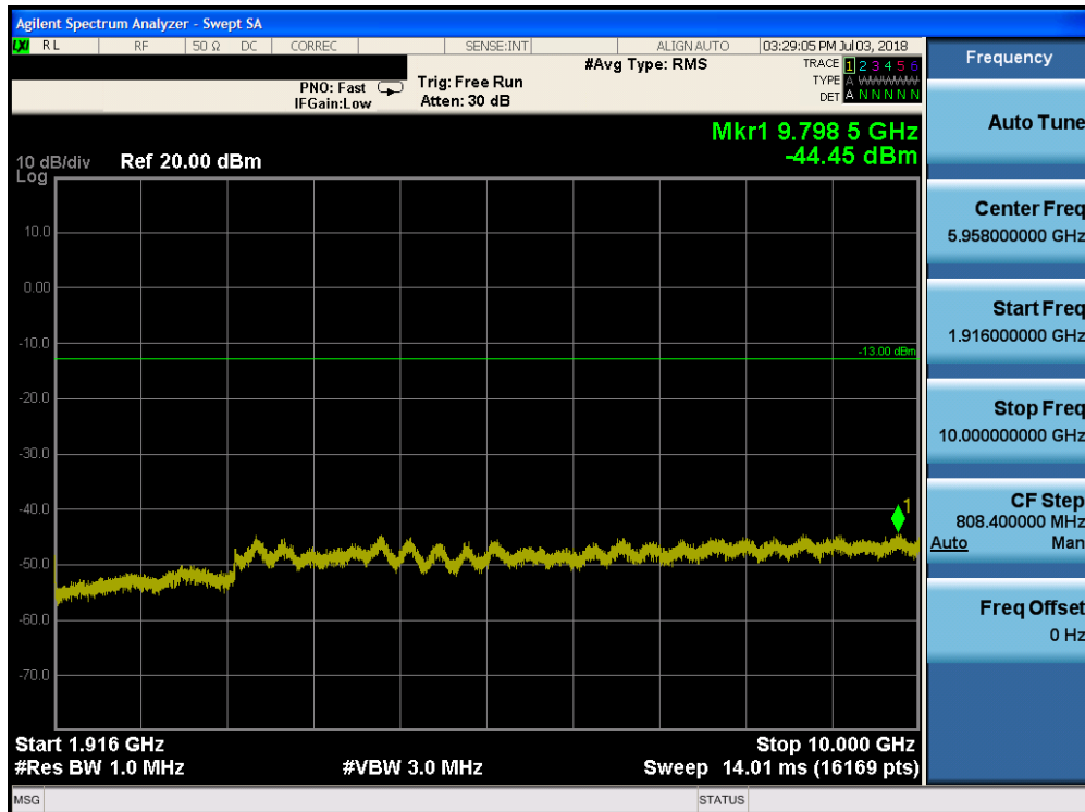
Plot 7-138. Conducted Spurious Plot (Band 25 - 20.0MHz QPSK - RB Size 1, RB Offset 0 - High Channel)
