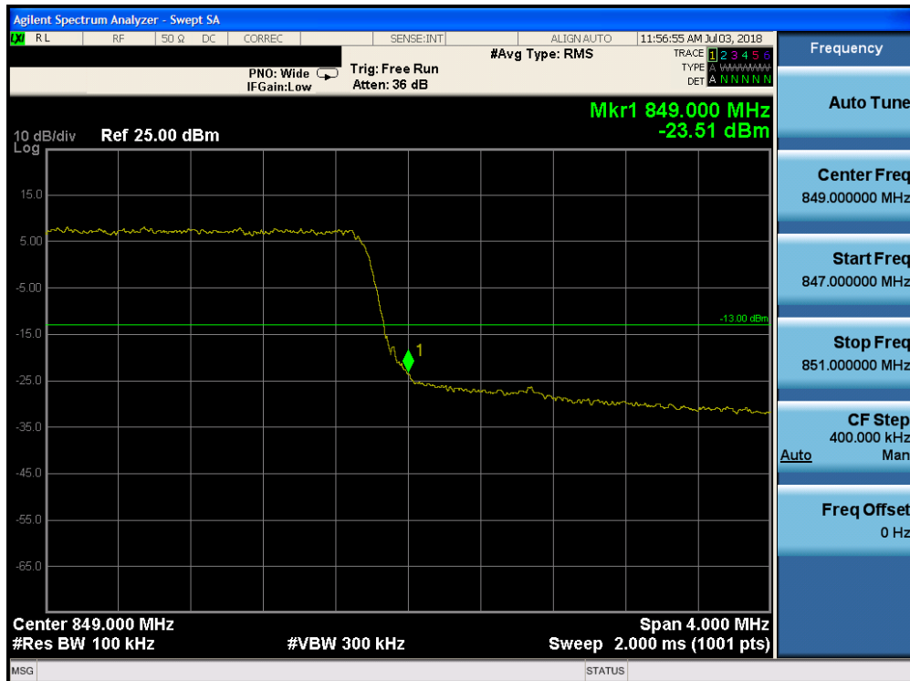
Plot 7-191. Upper Band Edge Plot (Band 5 - 5.0MHz QPSK - Full RB Configuration)
