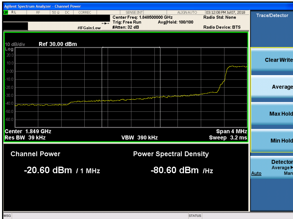
Plot 7-247. Lower Extended Band Edge Plot (Band 2 - 3.0MHz QPSK - Full RB Configuration)
