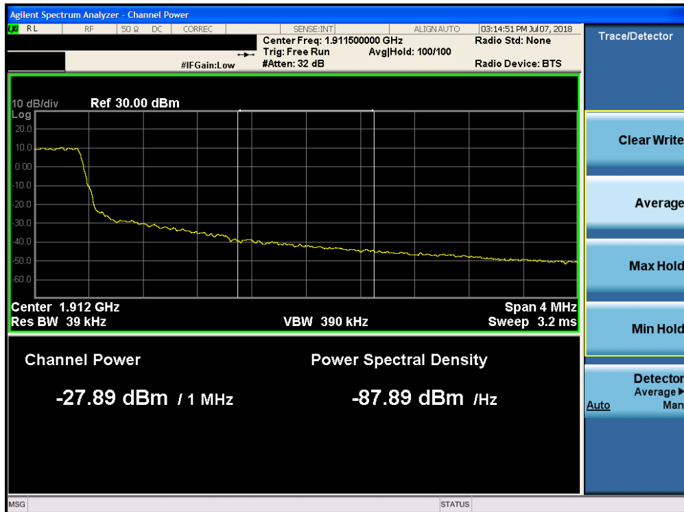
Plot 7-245. Upper Extended Band Edge Plot (Band 2 - 1.4MHz QPSK - Full RB Configuration)
