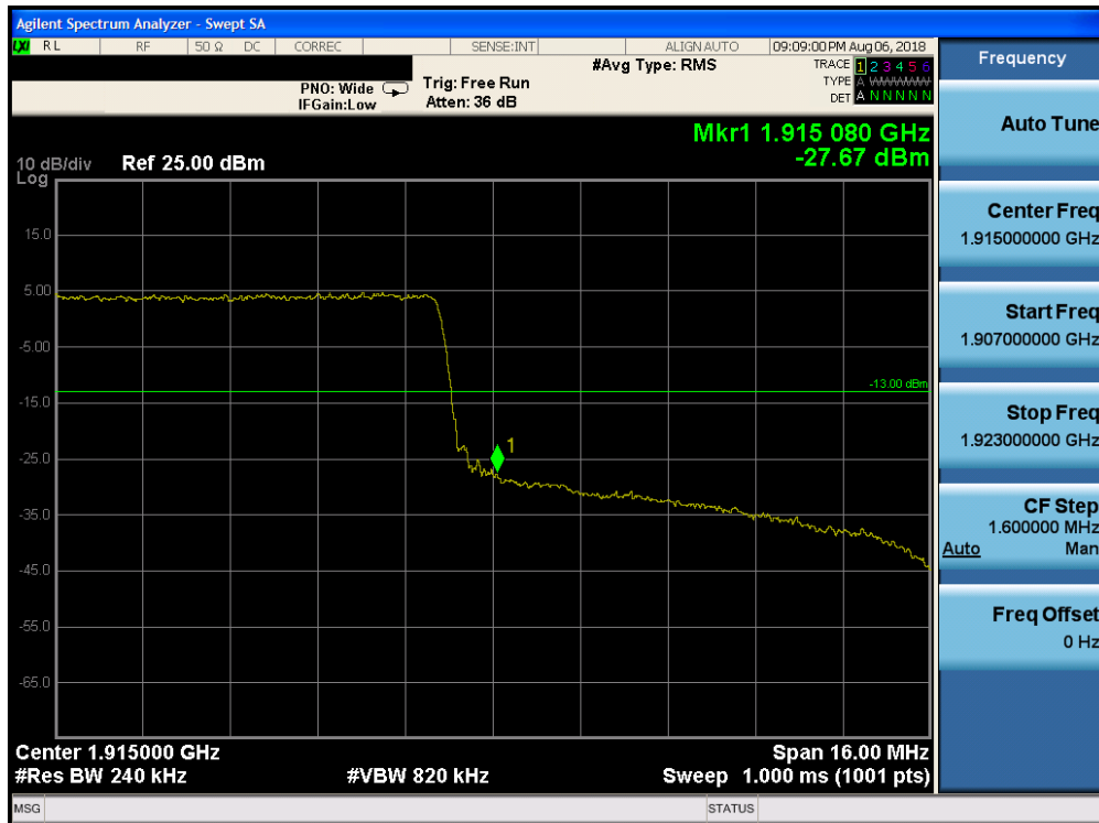
Plot 7-240. Upper Band Edge Plot (Band 25 - 20.0MHz QPSK - Full RB Configuration)
