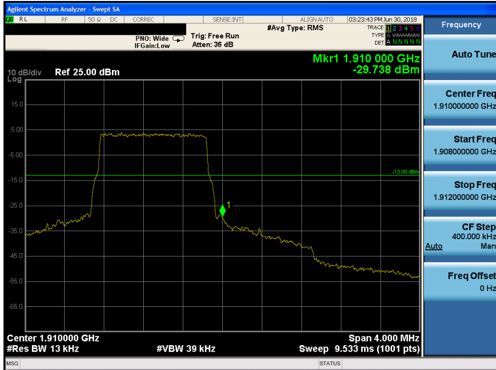
Plot 7-244. Upper Band Edge Plot (Band 2 - 1.4MHz QPSK - Full RB Configuration)
