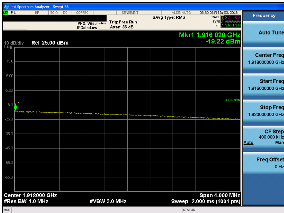
Plot 7-241. Upper Extended Band Edge Plot (Band 25 - 20.0MHz QPSK - Full RB Configuration)
