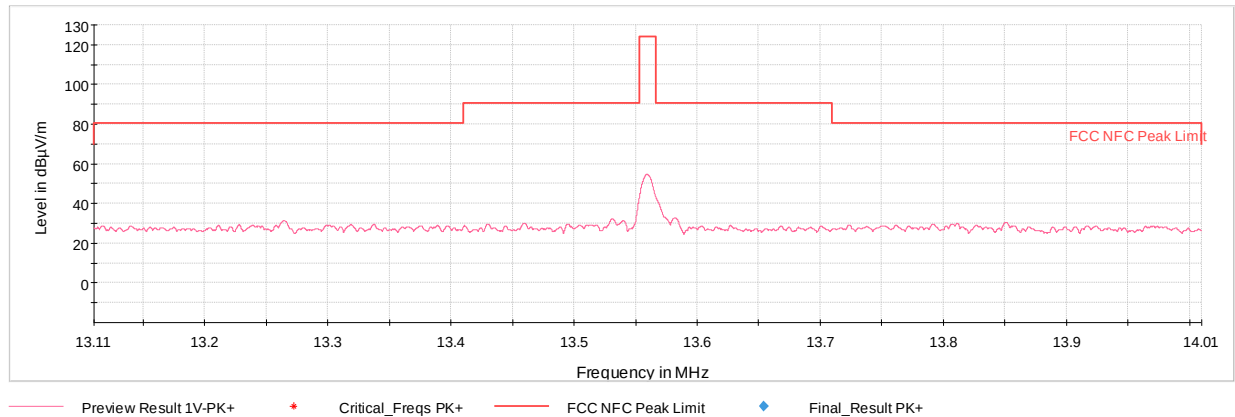
Plot 7-1. In Band Radiated Spurious Plot (CE A 848kbps, Pol. X)
