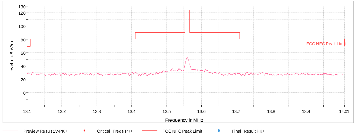
Plot 7-4. In Band Radiated Spurious Plot (Reader 100 Ask 1 out of 4, Pol. X)
