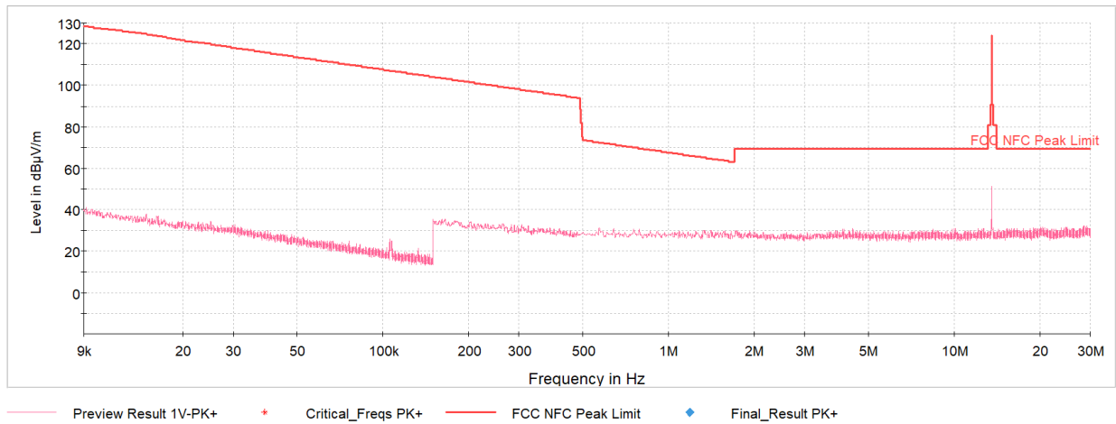
Plot 7-7. Radiated Spurious Plot 9kHz – 30MHz (Reader 100 Ask 1 out of 4, Pol. X)
