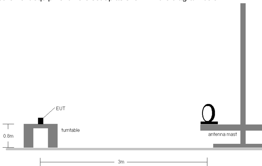
Figure 7-9. Radiated Test Setup
