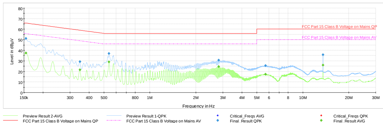
Plot 7-11. Line-Conducted Test Plot (N, with WCP + Laptop)
