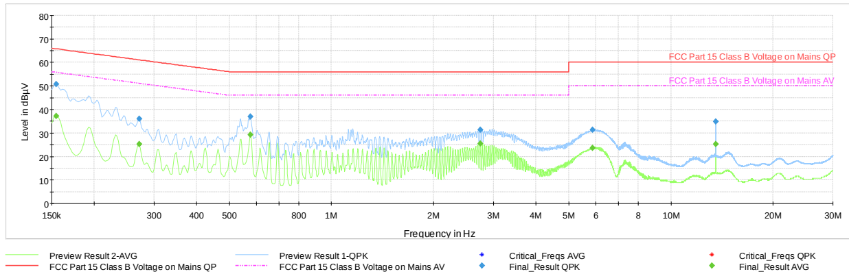
Plot 7-10. Line-Conducted Test Plot (L1, with WCP + Laptop)
