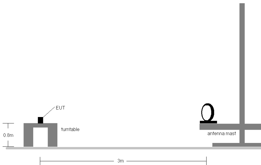
Figure 7-10. Radiated Test Setup < 30MHz
