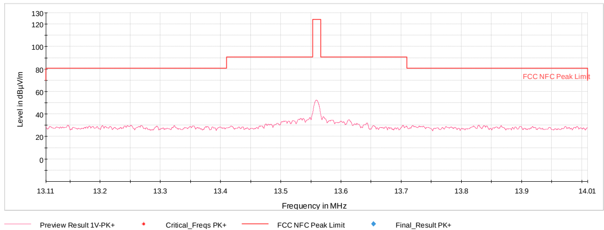
Plot 7-5. In Band Radiated Spurious Plot (Reader 100 Ask 1 out of 256, Pol. X)
