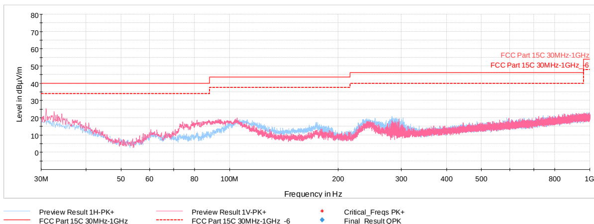
Plot 7-9. Radiated Spurious Plot 30MHz – 1GHz (Reader 100 Ask 1 out of 4, Pol. H & V)
