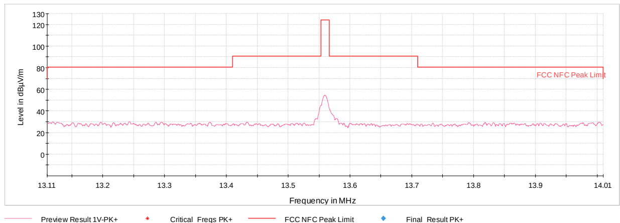
Plot 7-2. In Band Radiated Spurious (CE B 848kbps, Pol. X)
