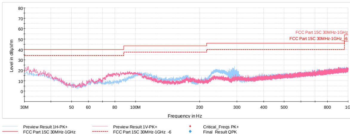
Plot 7-8. Radiated Spurious Plot 30MHz – 1GHz (CE A 848kbps, Pol. H & V)
