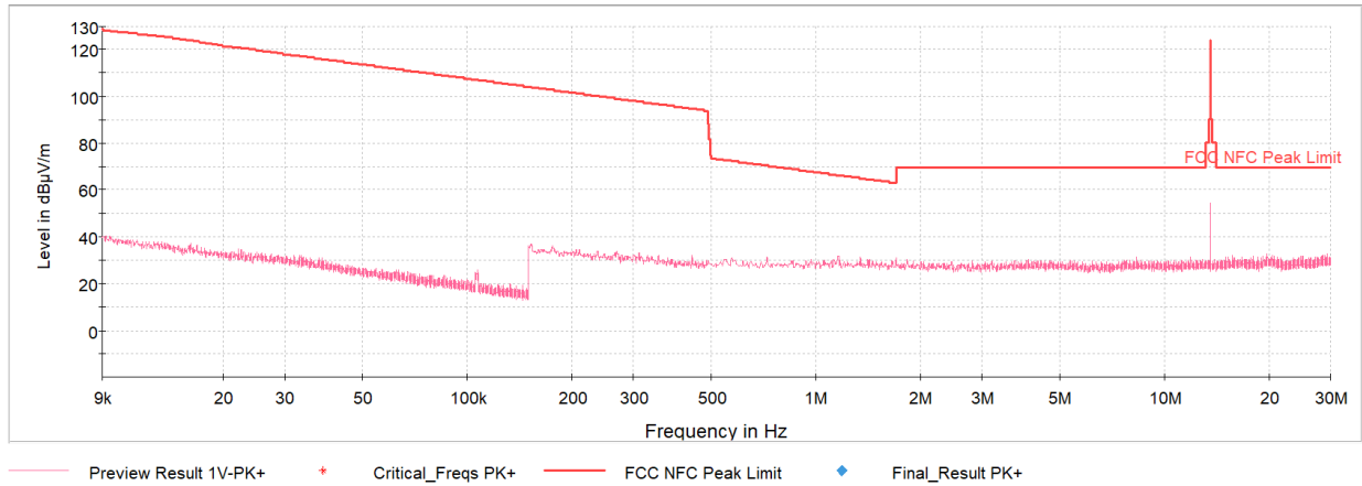
Plot 7-6. Radiated Spurious Plot 9kHz – 30MHz (CE A 848kbps, Pol. X)
