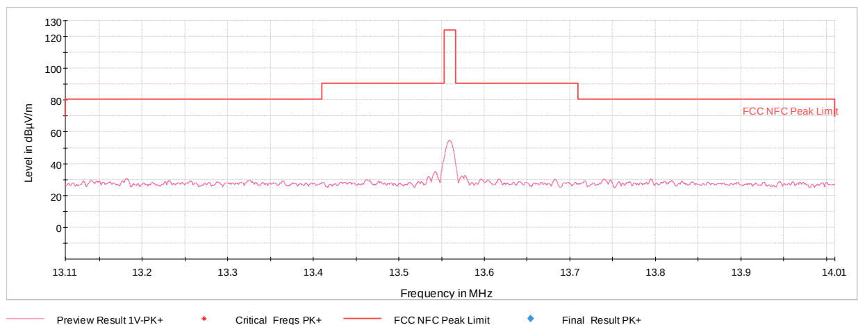
Plot 7-3. In Band Radiated Spurious Plot (CE F 424kbps, Pol. X)
