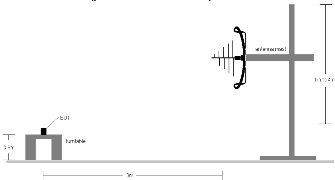
Figure 7-11. Radiated Test Setup > 30MHz
