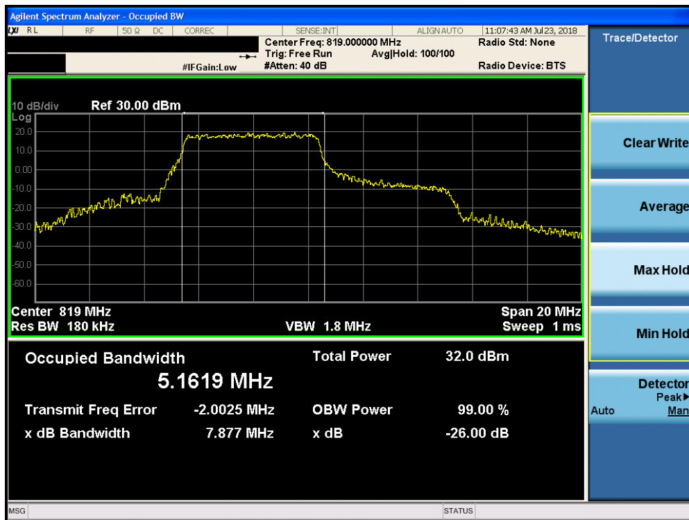
Plot 7-8. Occupied Bandwidth Plot (10MHz 16-QAM – RB Size 27)
