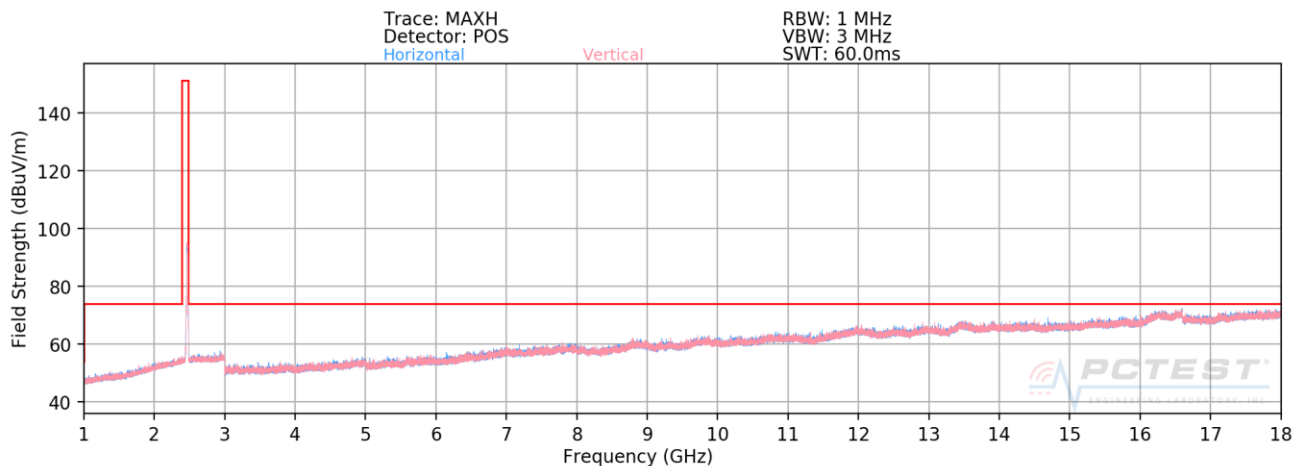
Plot 7-33. Radiated Spurious Plot above 1GHz (802.11b – Ch. 13)
