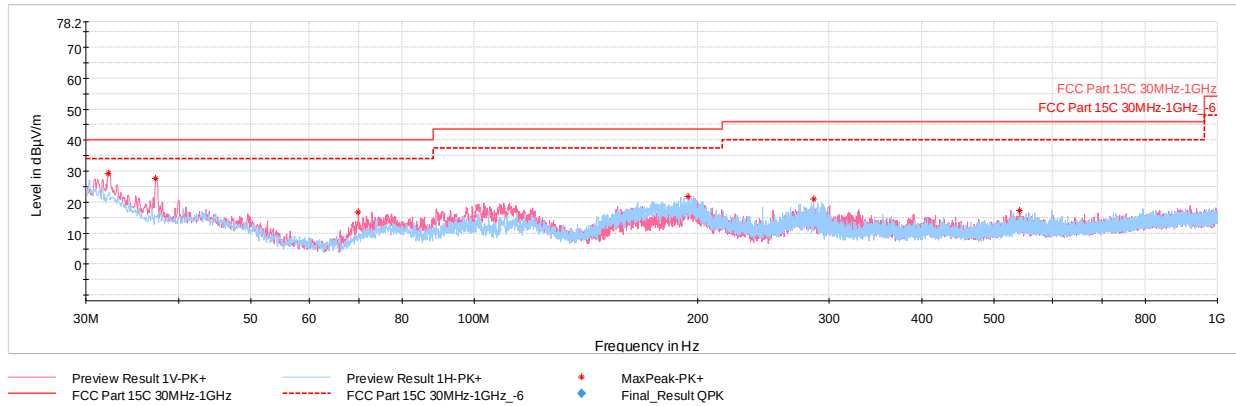
Plot 7-45. Radiated Spurious Plot below 1GHz (802.11b – Ch. 7, Pol. H & V, with WCP + Laptop)
