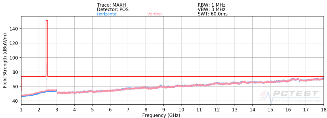
Plot 7-32. Radiated Spurious Plot above 1GHz (802.11b – Ch. 7)
