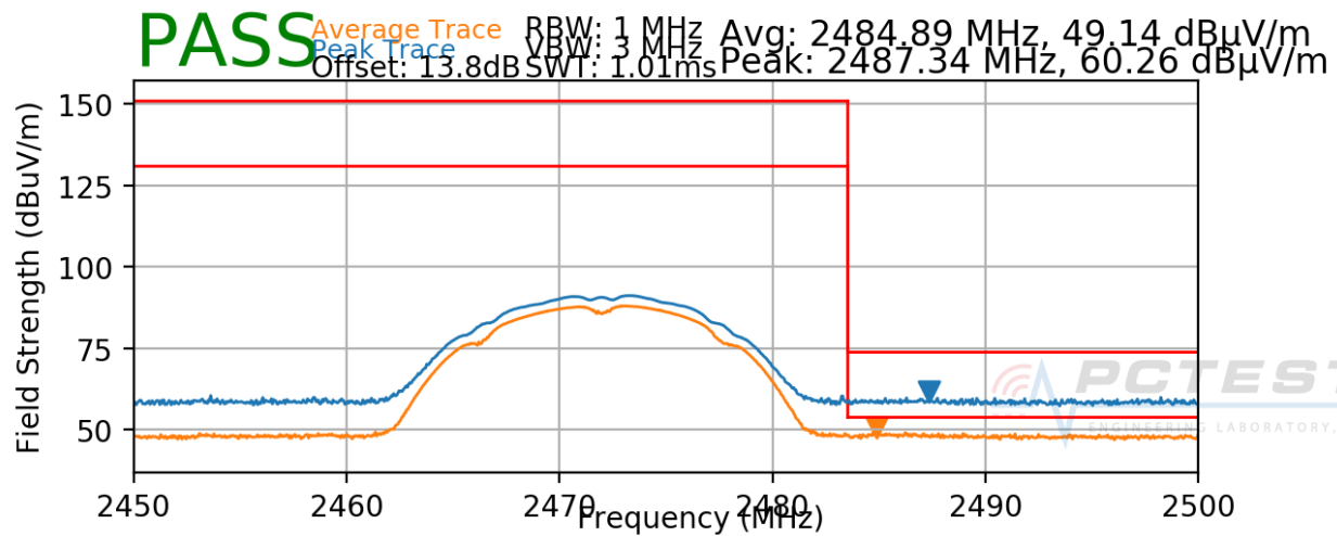
Plot 7-38. Radiated Restricted Upper Band Edge Measurement (Average & Peak)
