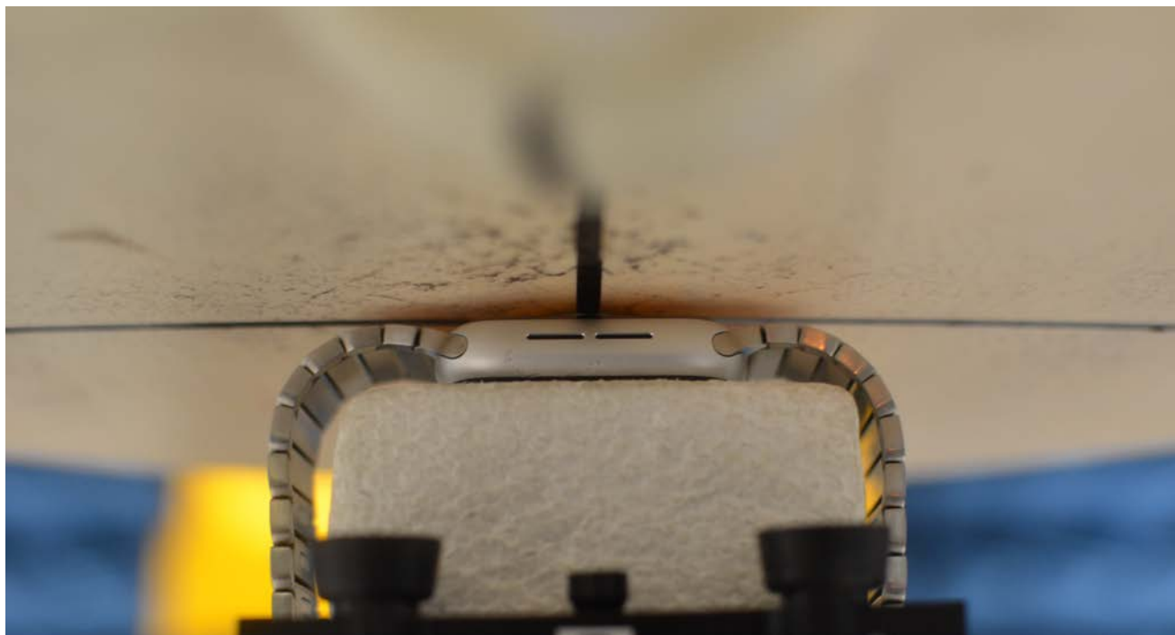
SAR Test Setup Photo 8: Aluminum with Metal Links wristband, Back side at 0.0 cm
