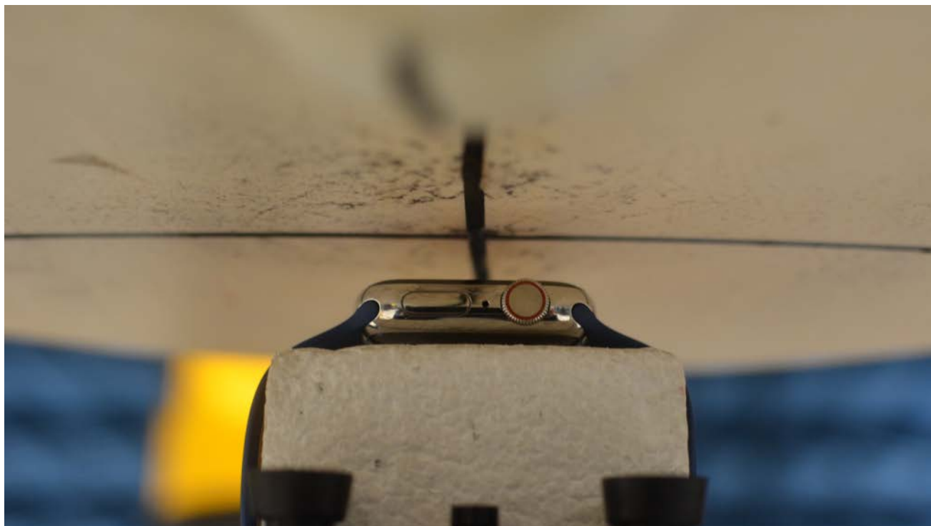
SAR Test Setup Photo 4: Stainless Steel with Sport wristband, Front side at 1.0 cm
