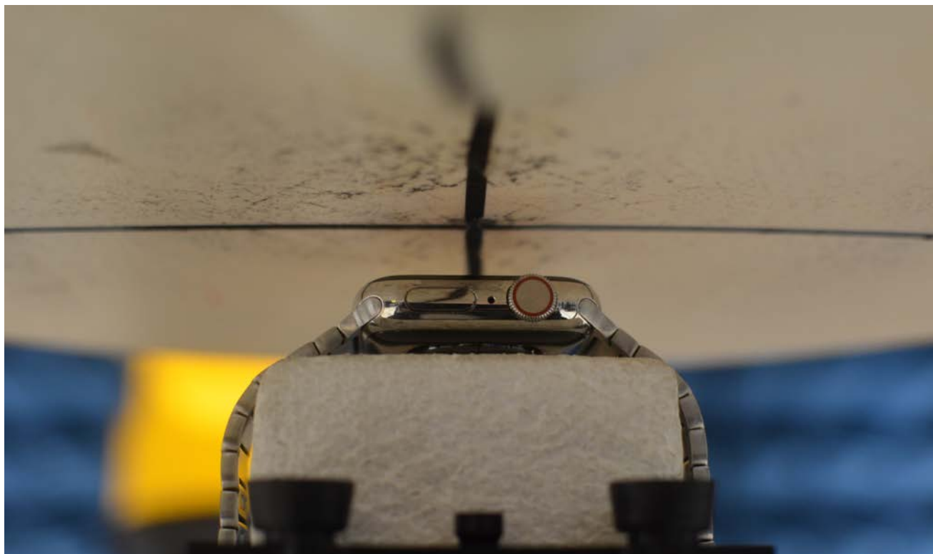
SAR Test Setup Photo 5: Stainless Steel with Metal Links wristband, Front side at 1.0 cm
