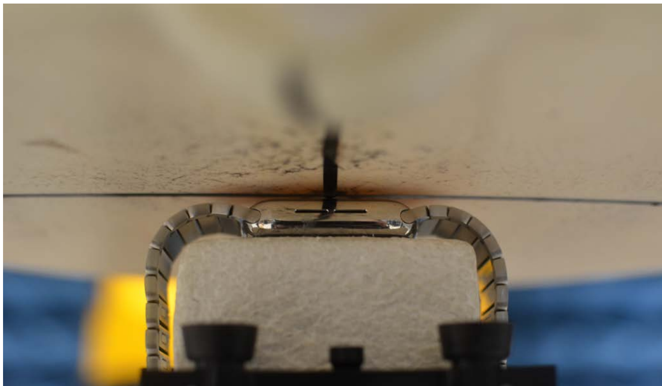
SAR Test Setup Photo 11: Stainless Steel with Metal Links wristband, Back side at 0.0 cm
