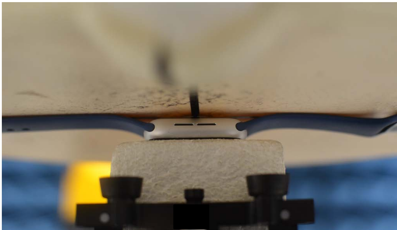
SAR Test Setup Photo 7: Aluminum with Sport wristband, Back side at 0.0 cm
