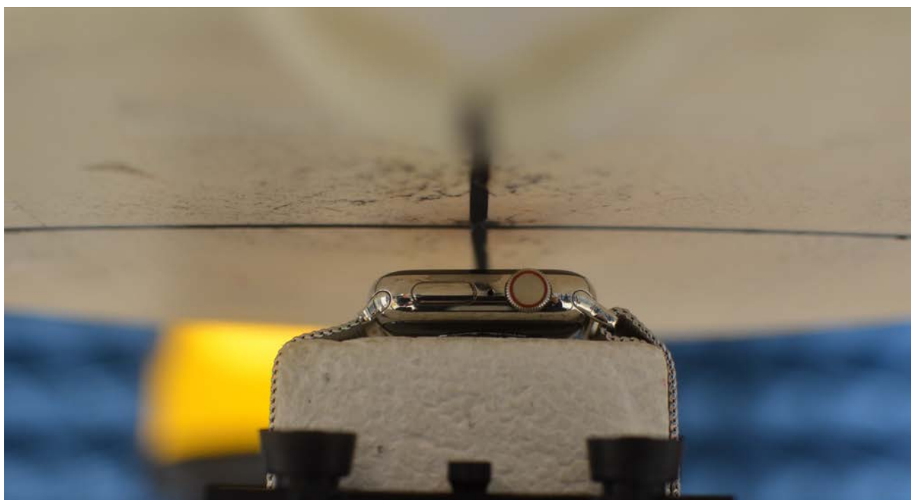
SAR Test Setup Photo 6: Stainless Steel with Metal Loop wristband, Front side at 1.0 cm
