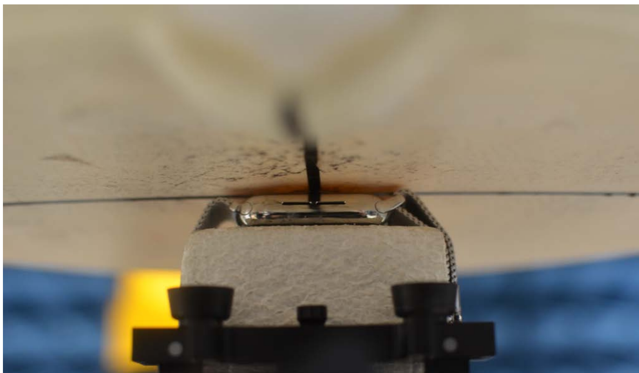
SAR Test Setup Photo 12: Stainless Steel with Metal Loop wristband, Back side at 0.0 cm
