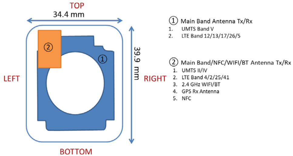
Figure F-1 DUT Antenna Locations
