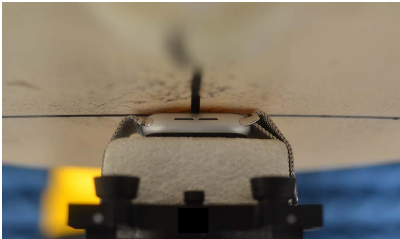
SAR Test Setup Photo 9: Aluminum with Metal Loop wristband, Back side at 0.0 cm
