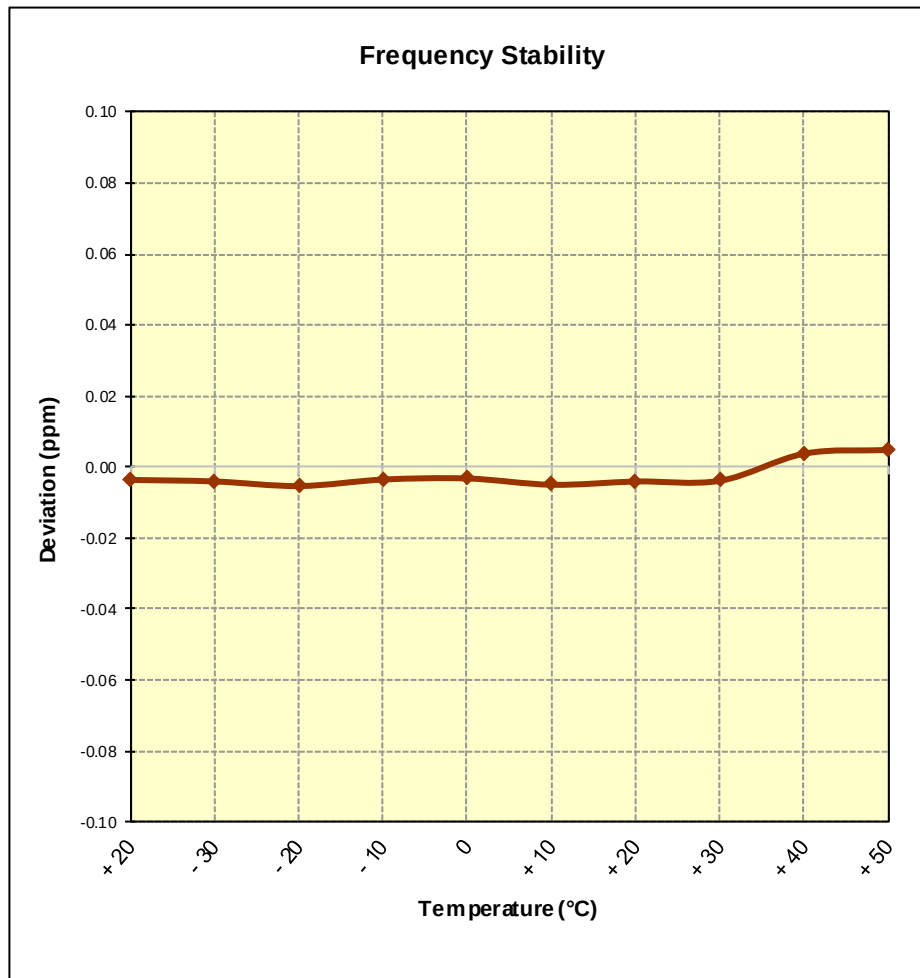
Figure 7-9. Frequency Stability Graph (PCS WCDMA Mode – Ch. 9400)
