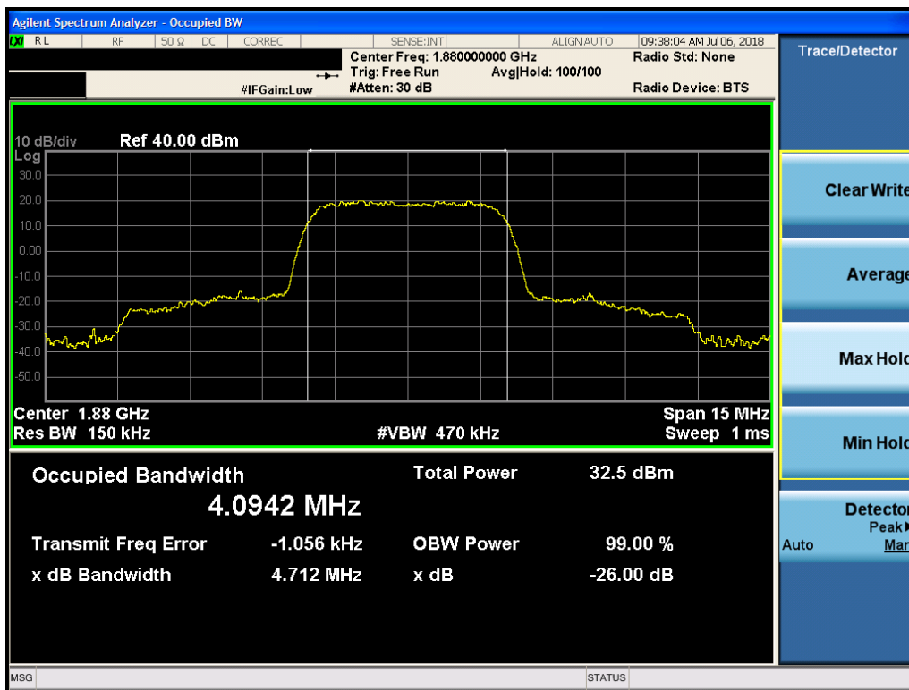
Plot 7-3. Occupied Bandwidth Plot (PCS WCDMA Mode)
