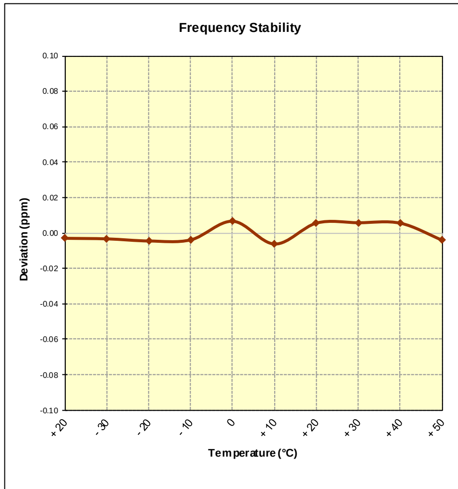
Figure 7-7. Frequency Stability Graph (Cellular WCDMA Mode – Ch. 4183)
