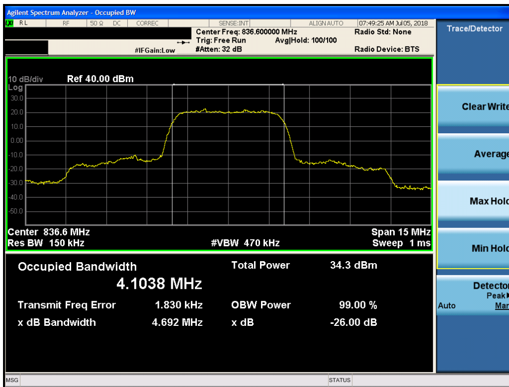
Plot 7-1. Occupied Bandwidth Plot (Cellular WCDMA Mode)
