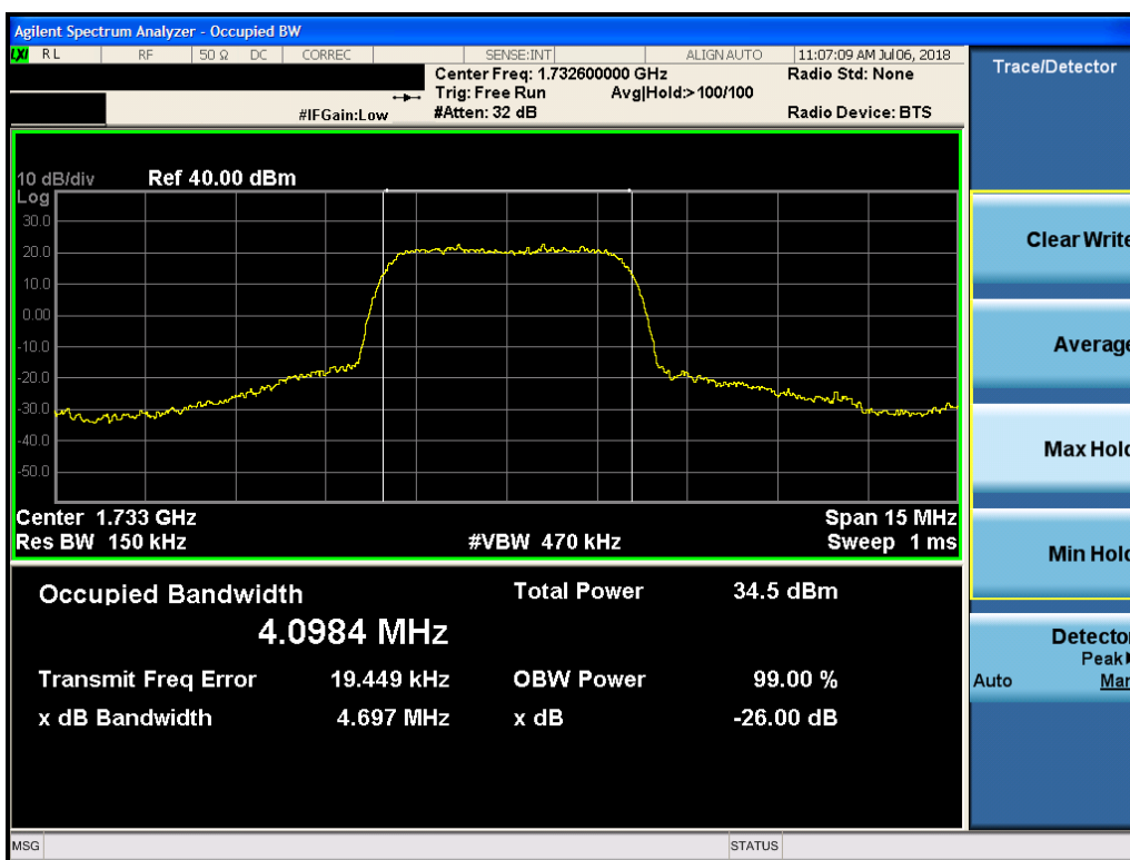
Plot 7-2. Occupied Bandwidth Plot (AWS WCDMA Mode)
