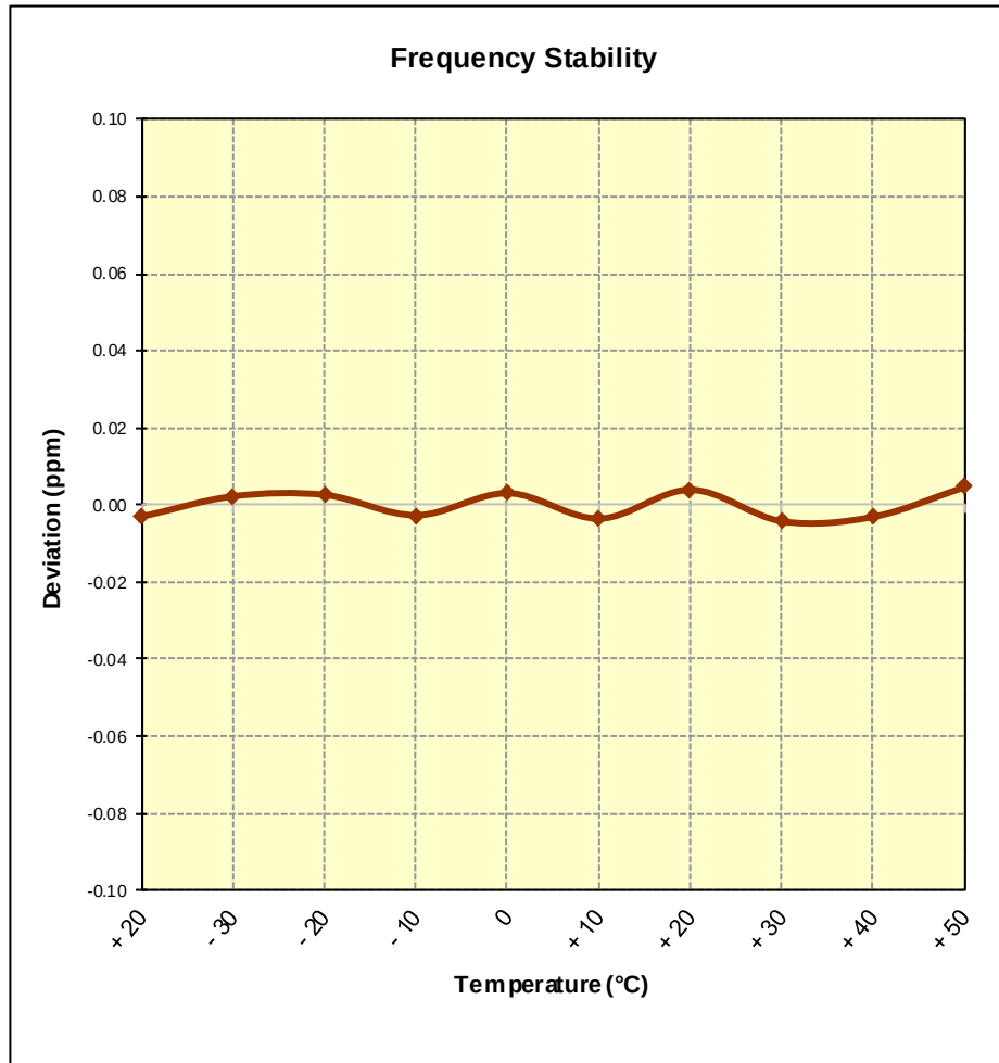
Figure 7-8. Frequency Stability Graph (AWS WCDMA Mode – Ch. 1413)
