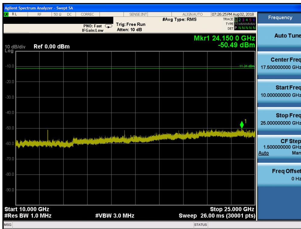
Plot 7-34. Conducted Spurious Plot (Bluetooth (HDR, ePA), 4Mbps – Ch. 1)
