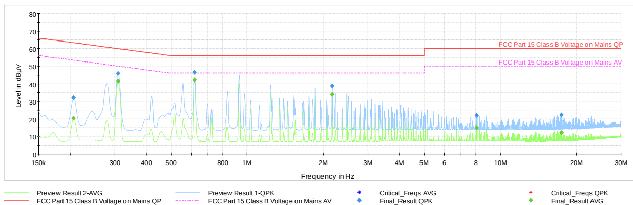
Plot 7-56. Line Conducted Plot with Bluetooth HDR (L1)
