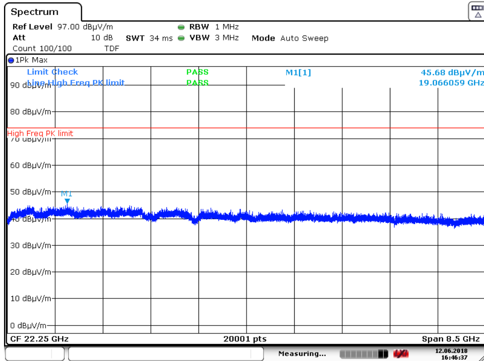
Plot 7-48. Radiated Spurious Plot above 18GHz (HDR8, ePA, Pol. H)
