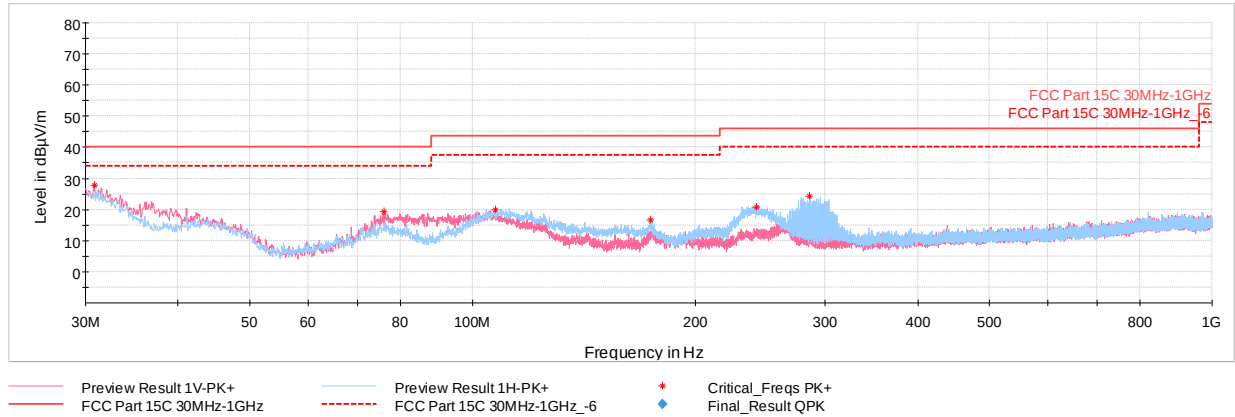
Plot 7-54. Radiated Spurious Plot below 1GHz (HDR8 ePA, Pol. H & V, with WCP + AC/DC Adapter attached)
