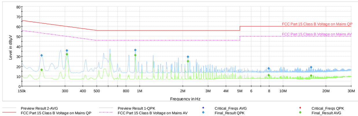
Plot 7-57. Line Conducted Plot with Bluetooth HDR (N)
