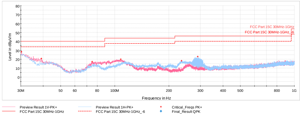
Plot 7-55. Radiated Spurious Plot below 1GHz (HDR4 ePA, Pol. H & V, with WCP + AC/DC Adapter attached)
