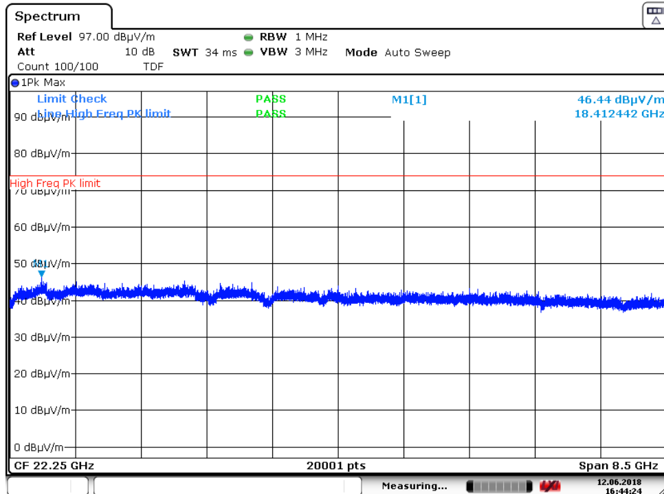
Plot 7-49. Radiated Spurious Plot above 18GHz (HDR8, ePA, Pol. V)
