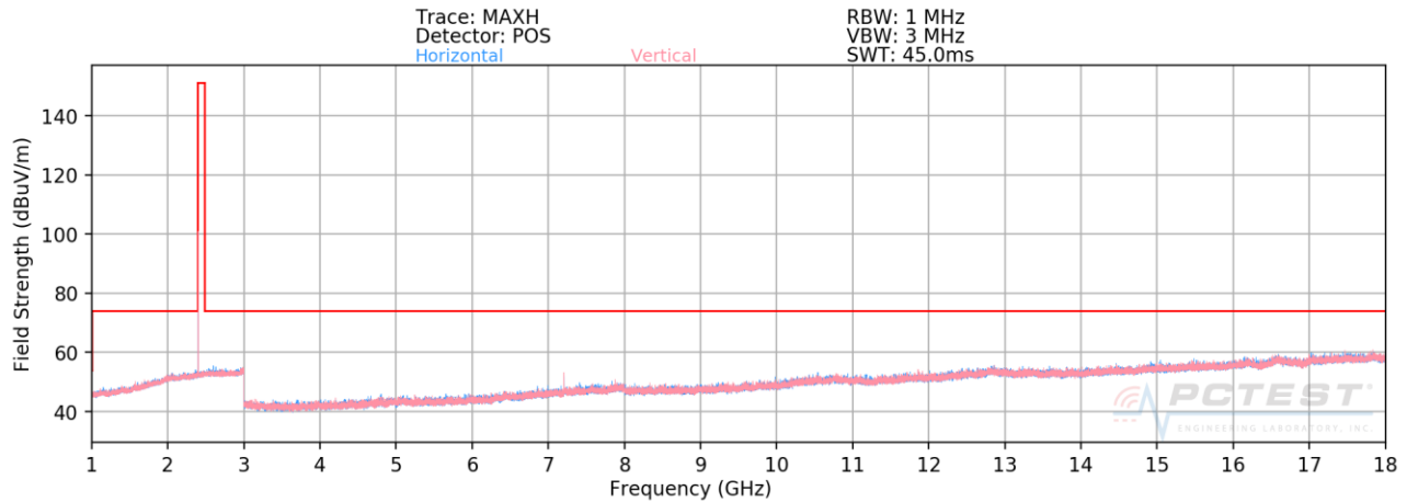
Plot 7-41. Radiated Spurious Plot (1Mbps, ePA – Ch. 0, Ant. Pol. H & V)
