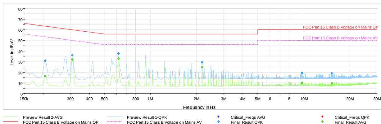
Plot 7-52. Line Conducted Plot with Bluetooth LE (N)
