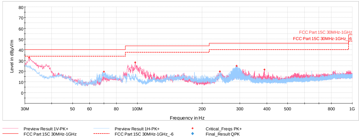
Plot 7-50. Radiated Spurious Plot below 1GHz (1Mbps ePA, Pol. H & V, with WCP + Laptop)
