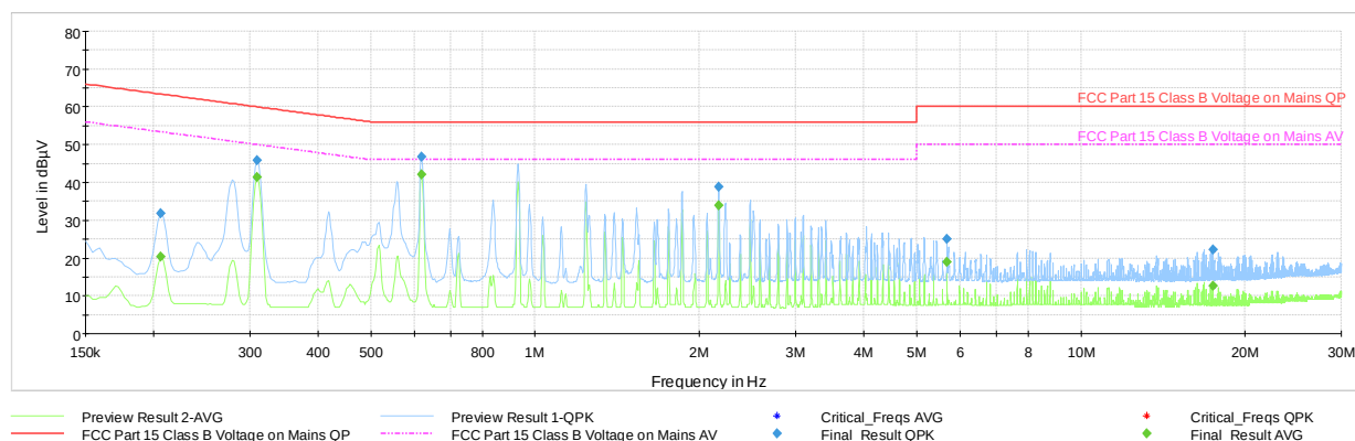
Plot 7-51. Line Conducted Plot with Bluetooth LE (L1)
