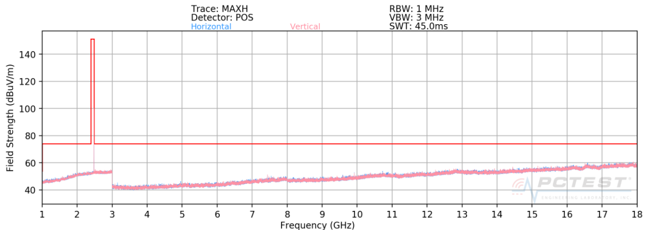
Plot 7-43. Radiated Spurious Plot (1Mbps, ePA – Ch. 39, Ant. Pol. H & V)
