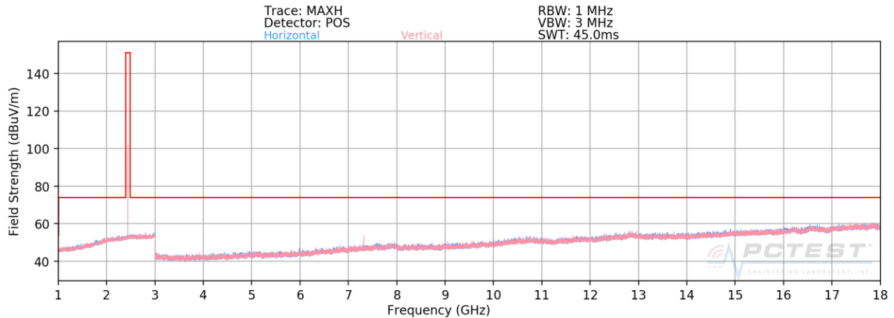
Plot 7-42. Radiated Spurious Plot (1Mbps, ePA – Ch. 19, Ant. Pol. H & V)
