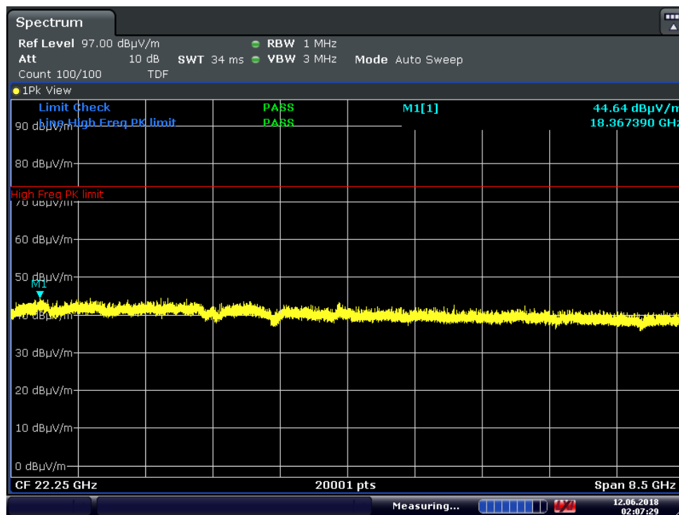
Plot 7-45. Radiated Spurious Plot above 18GHz (1Mbps, ePA, Pol. V)
