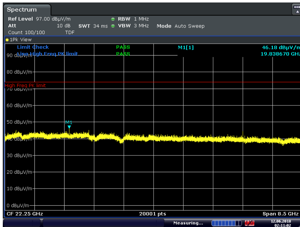
Plot 7-44. Radiated Spurious Plot above 18GHz (1Mbps, ePA, Pol. H)
