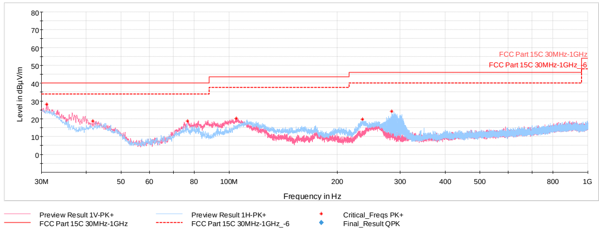
Plot 7-74. Radiated Spurious Plot below 1GHz (GFSK, ePA, with WCP + AC/DC Adapter)
