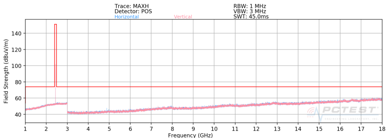
Plot 7-62. Radiated Spurious Plot above 1GHz (BT GFSK ePA – Ch. 39)
