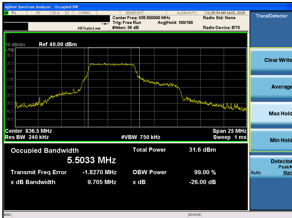
Plot 7-24. Occupied Bandwidth Plot (Band 5 - 10.0MHz 16-QAM - RB Size 27, RB Offset 0 Configuration)
