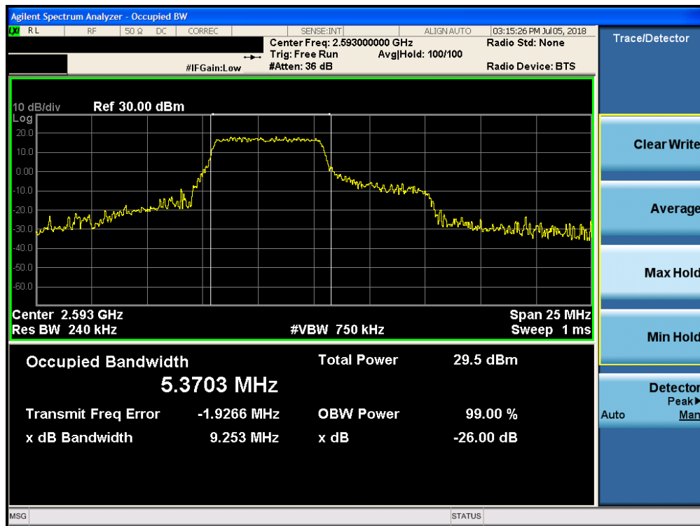
Plot 7-74. Occupied Bandwidth Plot (Band 41 - 10.0MHz 16-QAM - RB Size 27, RB Offset 0 Configuration)
