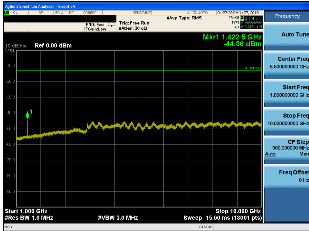
Plot 7-87. Conducted Spurious Plot (Band 12 - 5.0MHz QPSK - RB Size 1, RB Offset 0 - High Channel)
