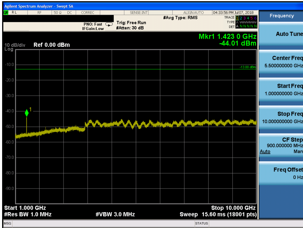
Plot 7-96. Conducted Spurious Plot (Band 17 - 5.0MHz QPSK - RB Size 1, RB Offset 0 - High Channel)
