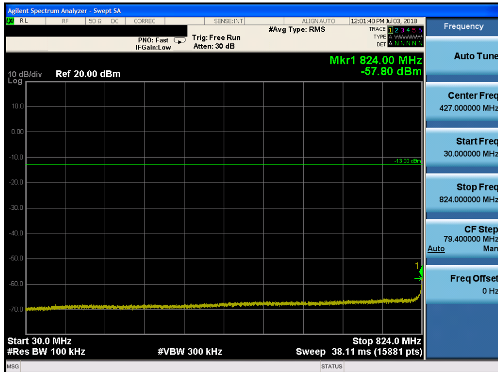
Plot 7-118. Conducted Spurious Plot (Band 5 - 3.0MHz QPSK - RB Size 1, RB Offset 0 - Mid Channel)
