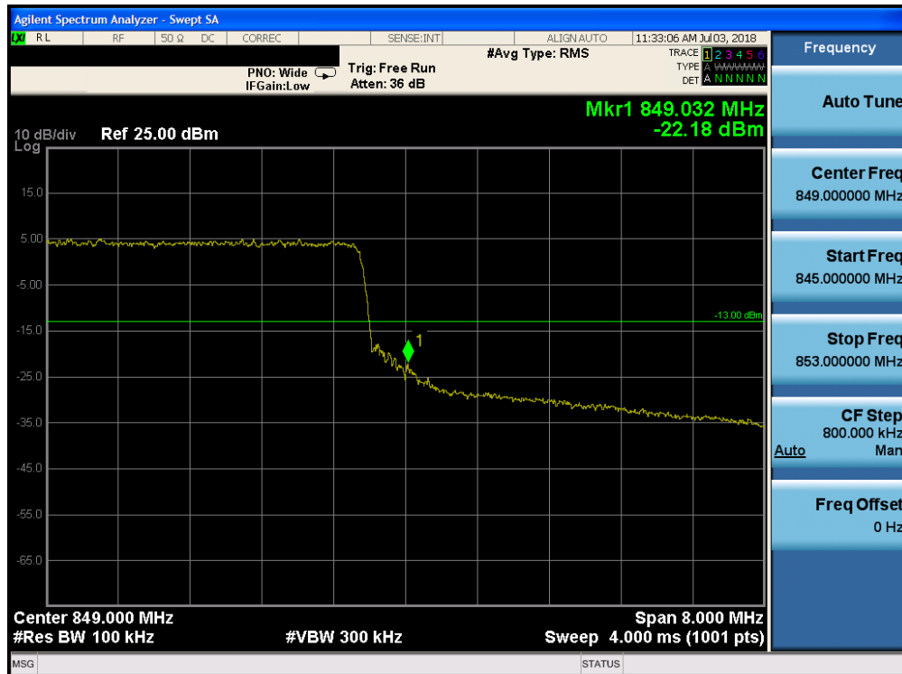
Plot 7-197. Upper Band Edge Plot (Band 5 - 10.0MHz QPSK - Full RB Configuration)
