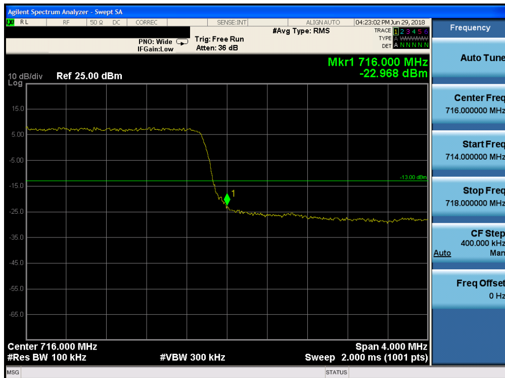
Plot 7-165. Upper Band Edge Plot (Band 12 - 5.0MHz QPSK - Full RB Configuration)
