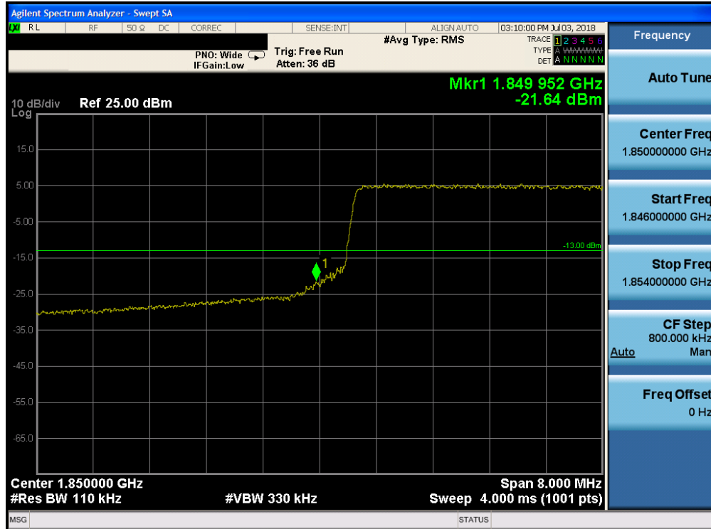
Plot 7-234. Lower Band Edge Plot (Band 25 - 10.0MHz QPSK - Full RB Configuration)
