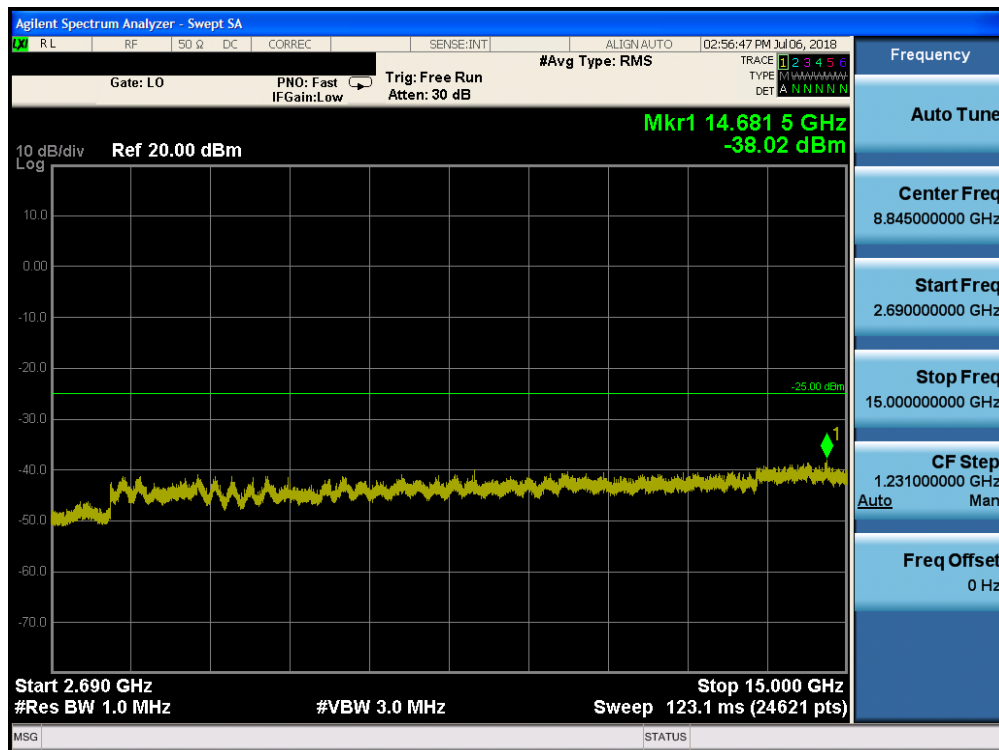
Plot 7-152. Conducted Spurious Plot (Band 41 - 20.0MHz QPSK - RB Size 1, RB Offset 0 - Low Channel)
