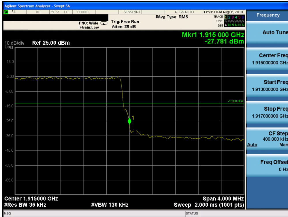
Plot 7-228. Upper Band Edge Plot (Band 25 - 3.0MHz QPSK - Full RB Configuration)
