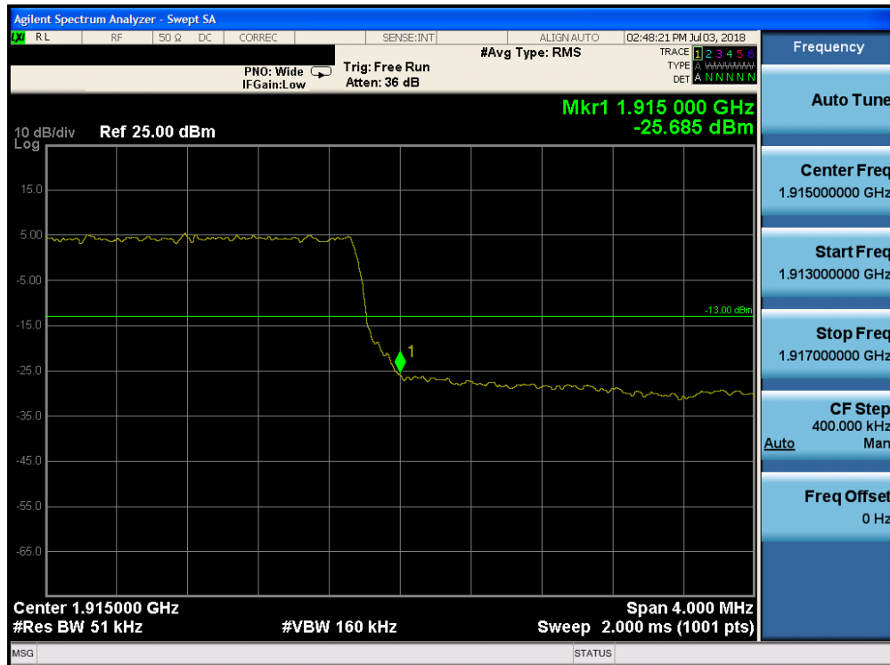
Plot 7-232. Upper Band Edge Plot (Band 25 - 5.0MHz QPSK - Full RB Configuration)
