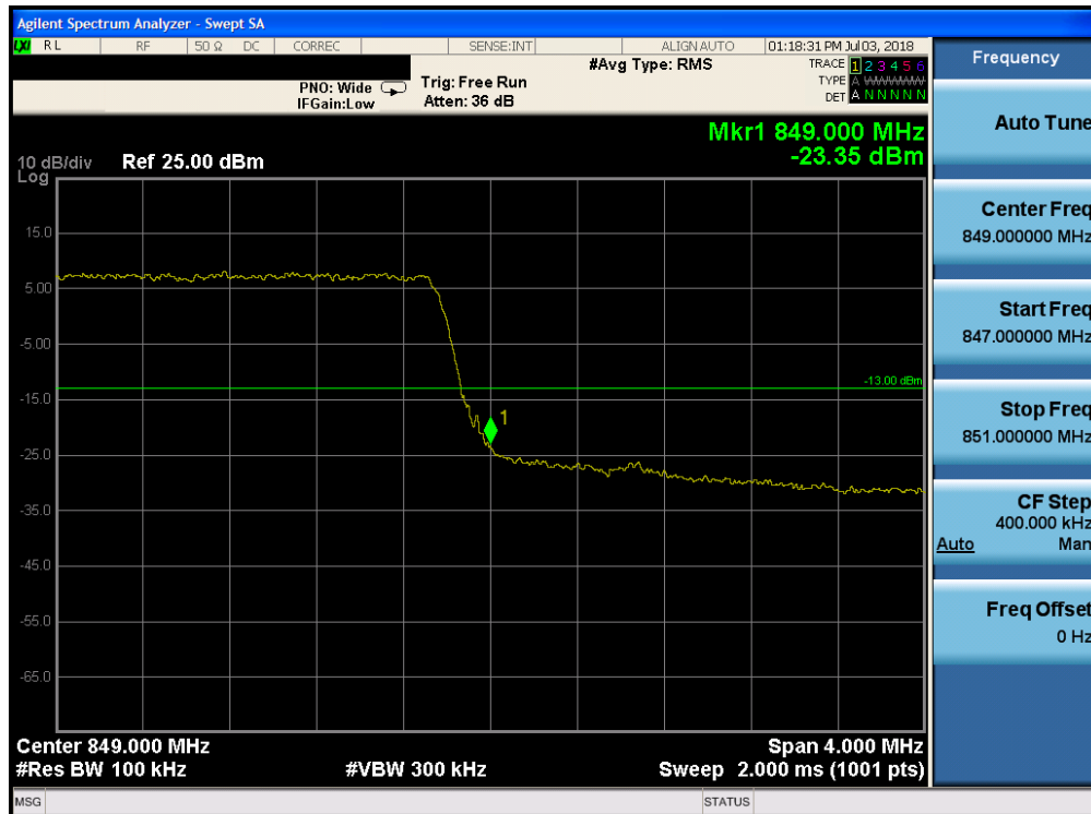
Plot 7-185. Upper Band Edge Plot (Band 26 - 5.0MHz QPSK - Full RB Configuration)
