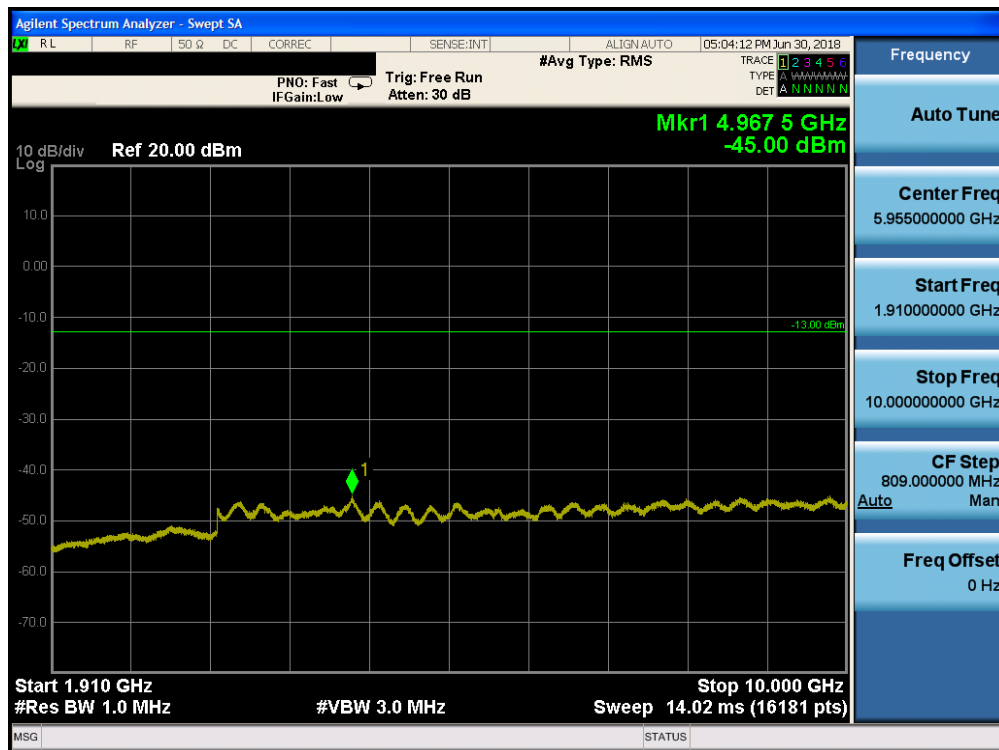
Plot 7-143. Conducted Spurious Plot (Band 2 - 20.0MHz QPSK - RB Size 1, RB Offset 0 - Low Channel)
