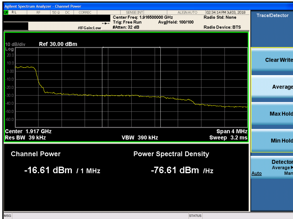
Plot 7-229. Upper Extended Band Edge Plot (Band 25 - 3.0MHz QPSK - Full RB Configuration)
