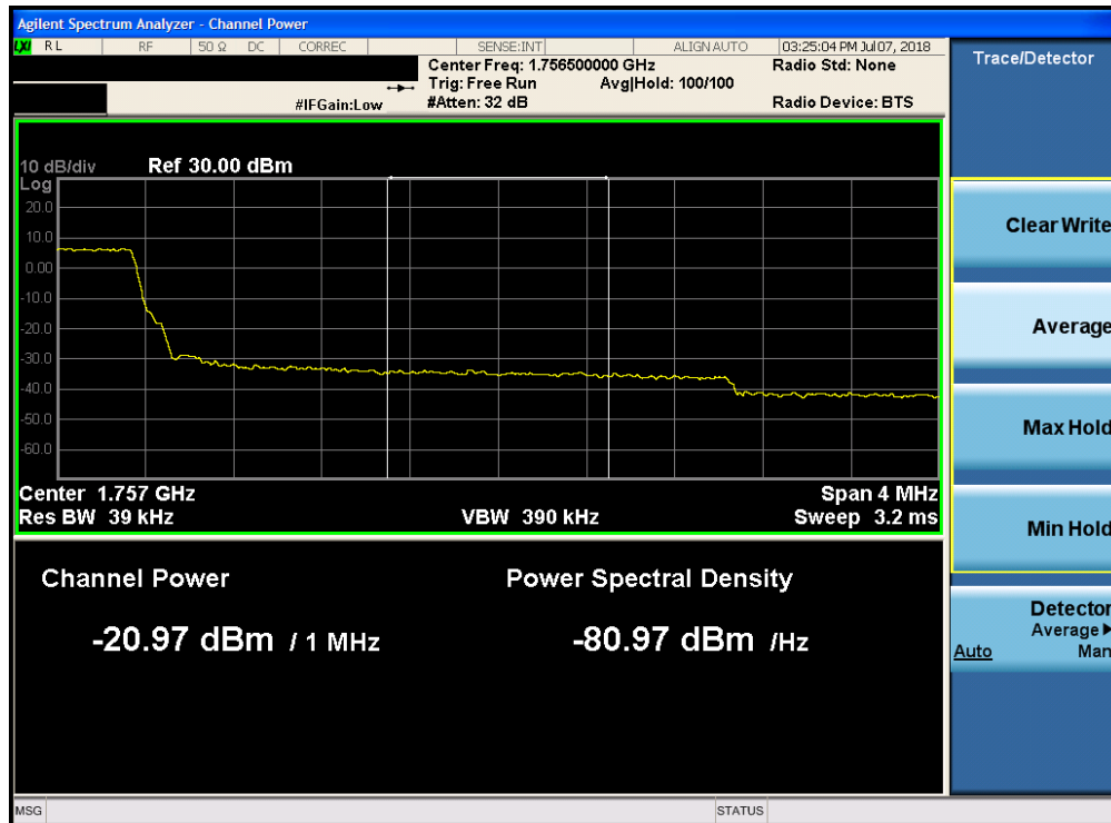
Plot 7-205. Upper Extended Band Edge Plot (Band 4 - 3.0MHz QPSK - Full RB Configuration)
