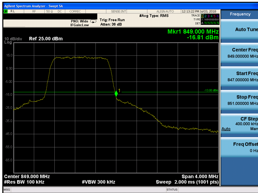
Plot 7-191. Upper Band Edge Plot (Band 5 - 1.4MHz QPSK - Full RB Configuration)
