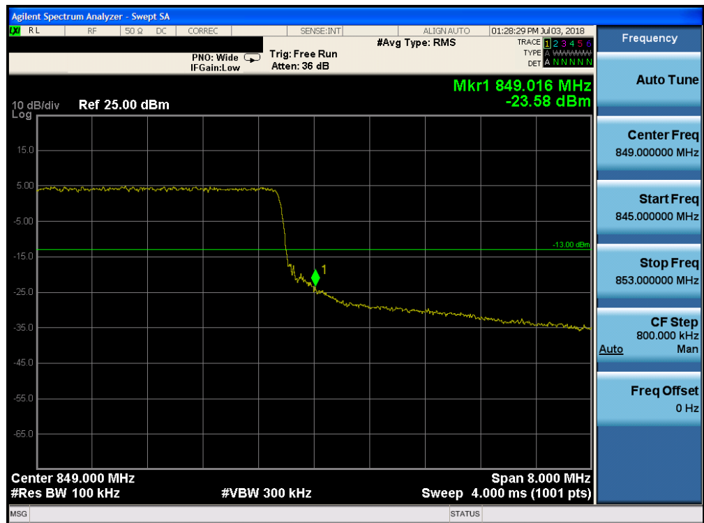
Plot 7-187. Upper Band Edge Plot (Band 26 - 10.0MHz QPSK - Full RB Configuration)
