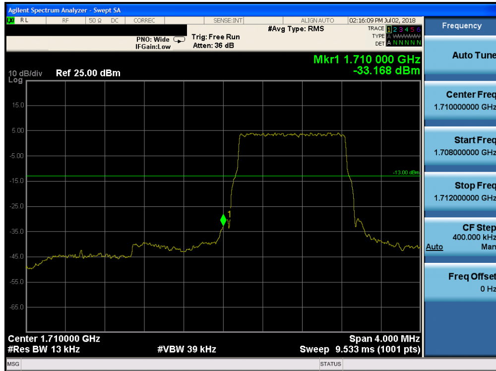
Plot 7-198. Lower Band Edge Plot (Band 4 - 1.4MHz QPSK - Full RB Configuration)
