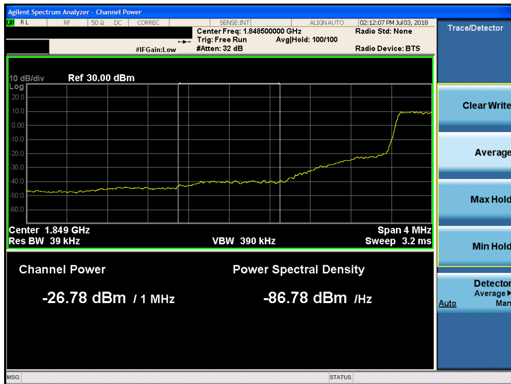
Plot 7-223. Lower Extended Band Edge Plot (Band 25 - 1.4MHz QPSK - Full RB Configuration)
