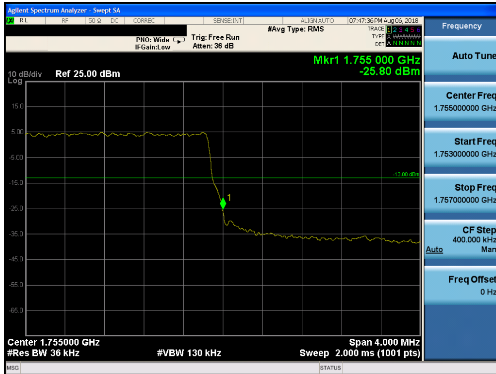
Plot 7-204. Upper Band Edge Plot (Band 4 - 3.0MHz QPSK - Full RB Configuration)
