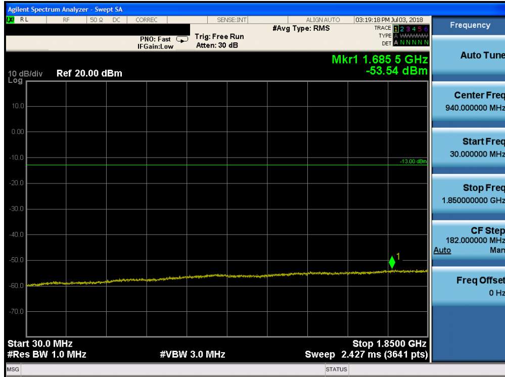
Plot 7-139. Conducted Spurious Plot (Band 25 - 15.0MHz QPSK - RB Size 1, RB Offset 0 - High Channel)
