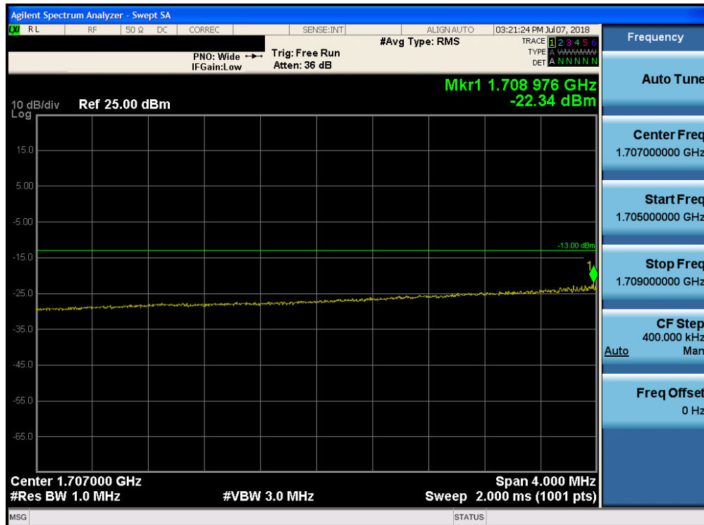
Plot 7-215. Lower Extended Band Edge Plot (Band 4 - 15.0MHz QPSK - Full RB Configuration)
