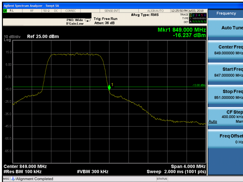
Plot 7-181. Upper Band Edge Plot (Band 26 - 1.4MHz QPSK - Full RB Configuration)
