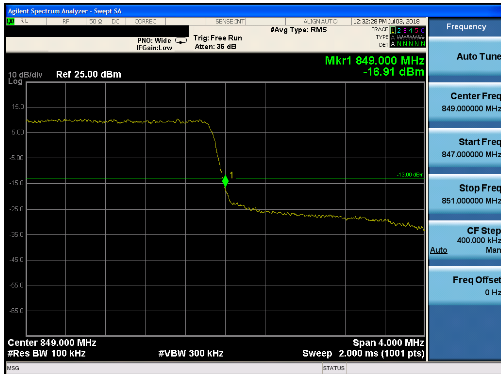
Plot 7-183. Upper Band Edge Plot (Band 26 - 3.0MHz QPSK - Full RB Configuration)
