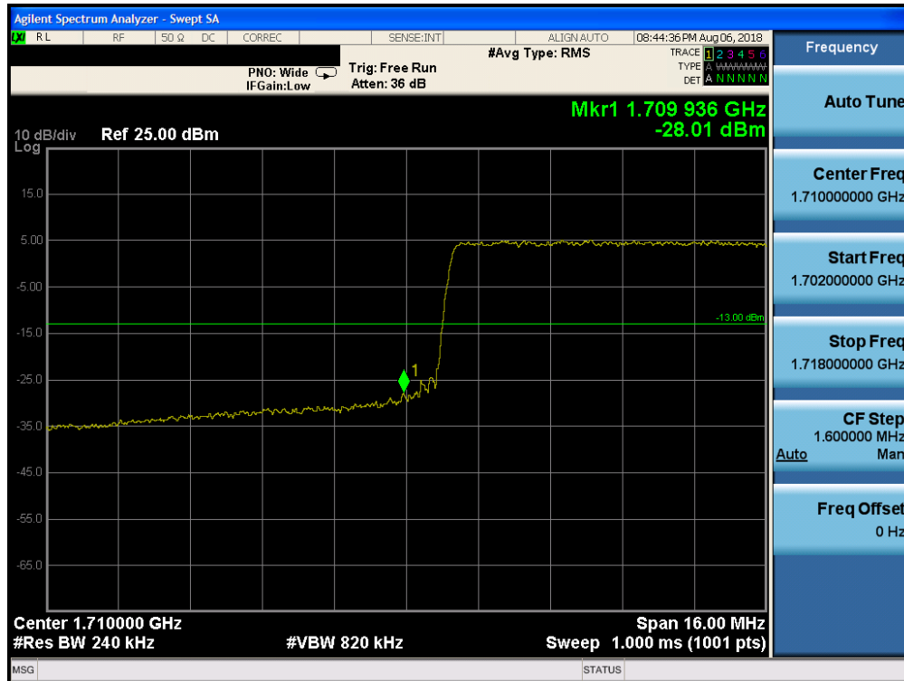
Plot 7-218. Lower Band Edge Plot (Band 4 - 20.0MHz QPSK - Full RB Configuration)
