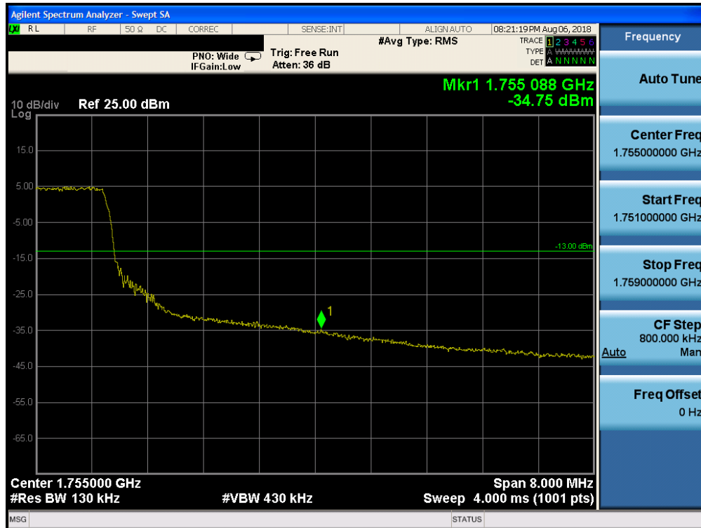
Plot 7-212. Upper Band Edge Plot (Band 4 - 10.0MHz QPSK - Full RB Configuration)
