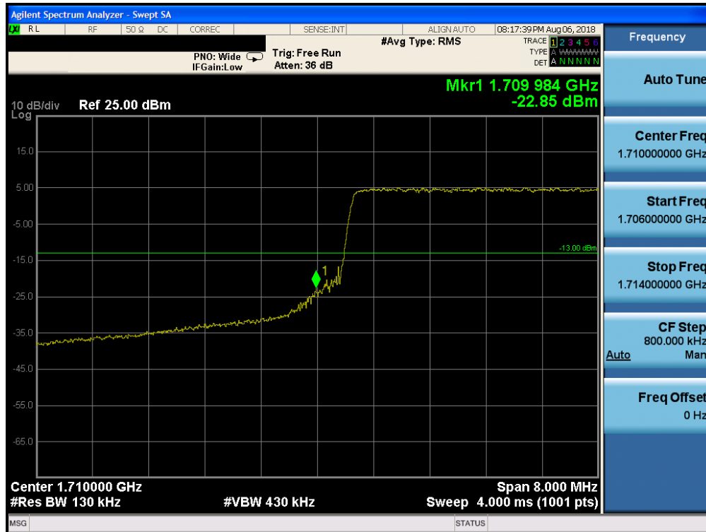
Plot 7-210. Lower Band Edge Plot (Band 4 - 10.0MHz QPSK - Full RB Configuration)
