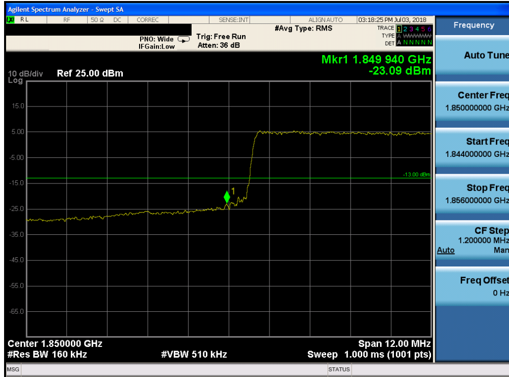
Plot 7-238. Lower Band Edge Plot (Band 25 - 15.0MHz QPSK - Full RB Configuration)
