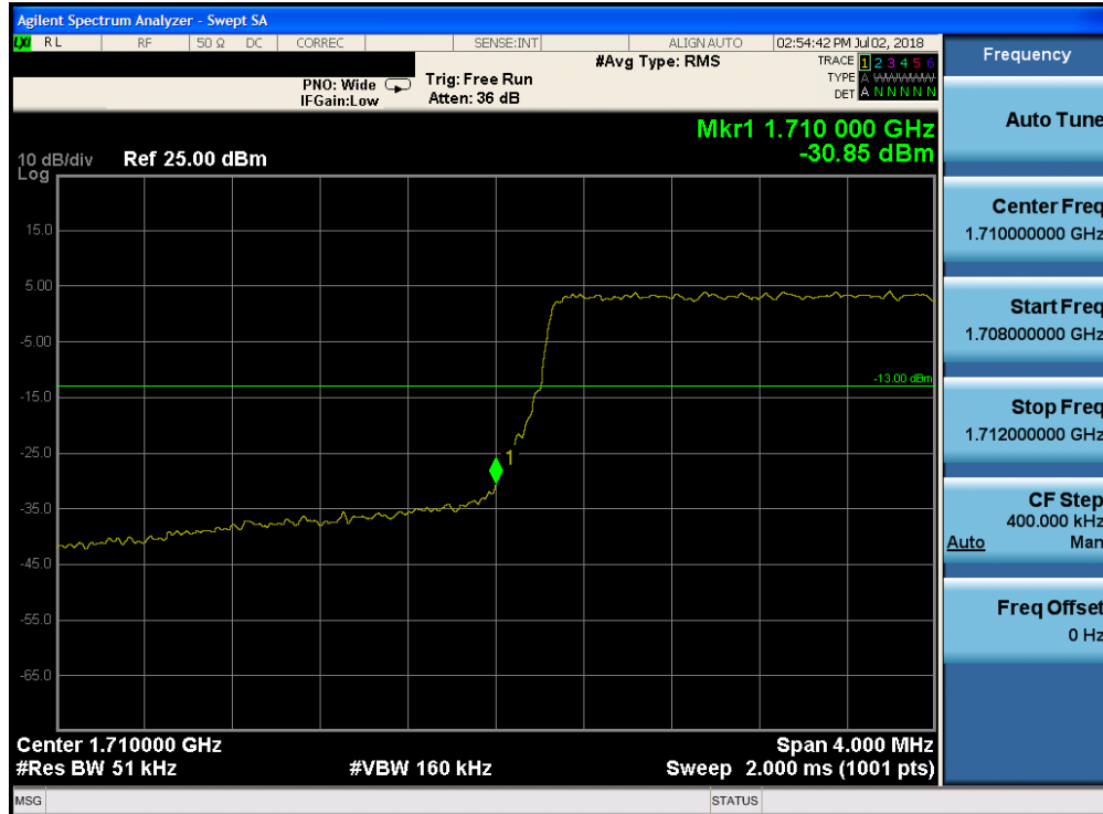
Plot 7-206. Lower Band Edge Plot (Band 4 - 5.0MHz QPSK - Full RB Configuration)
