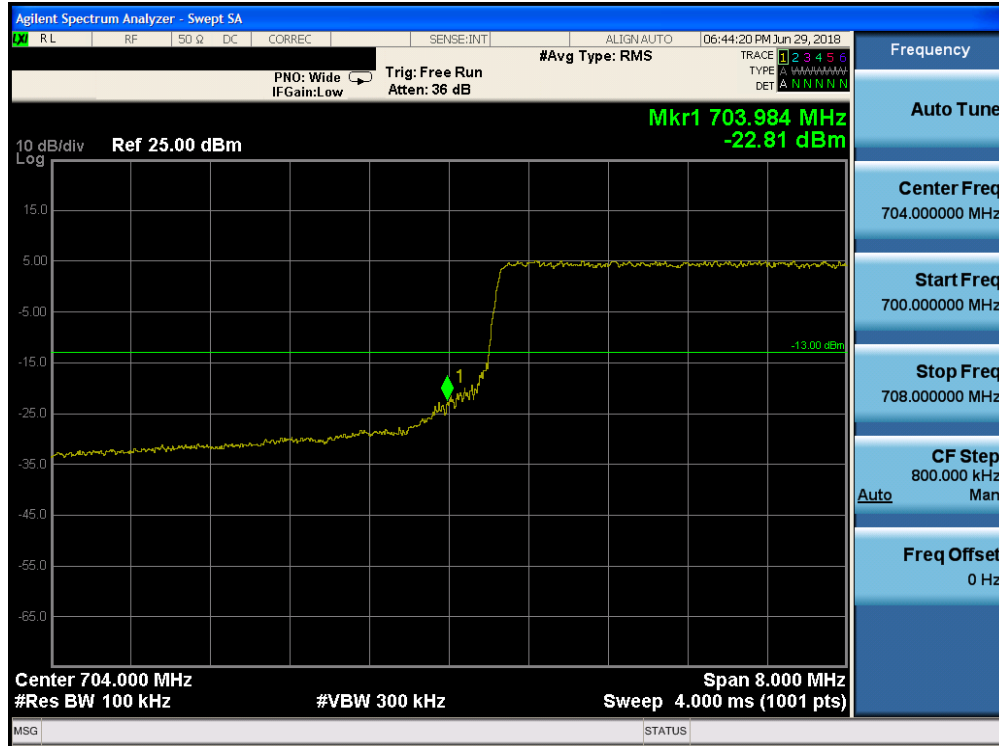
Plot 7-170. Lower Band Edge Plot (Band 17 - 10.0MHz QPSK - Full RB Configuration)
