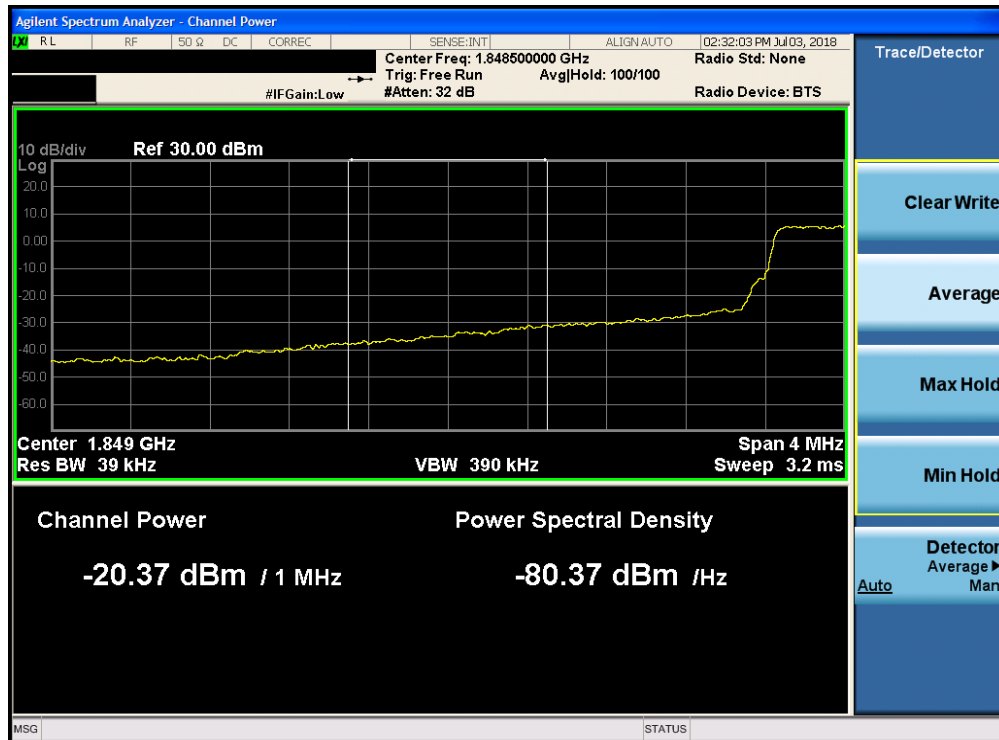
Plot 7-227. Lower Extended Band Edge Plot (Band 25 - 3.0MHz QPSK - Full RB Configuration)
