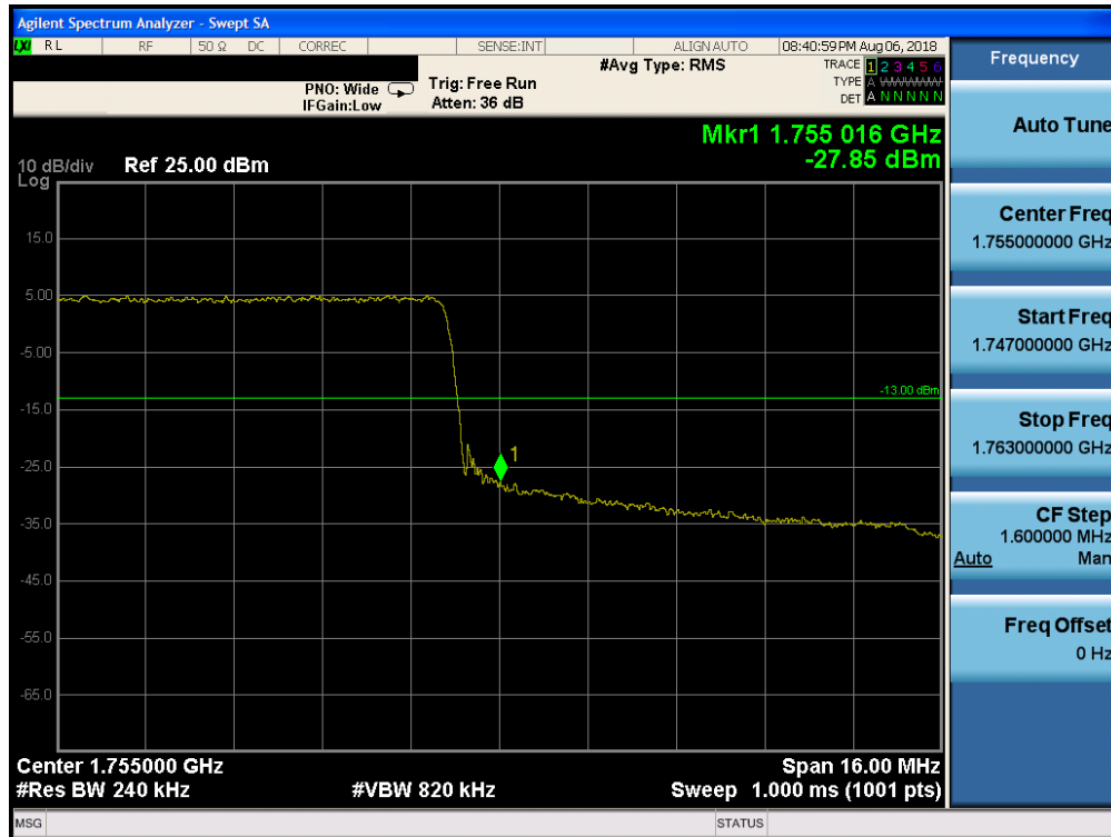
Plot 7-220. Upper Band Edge Plot (Band 4 - 20.0MHz QPSK - Full RB Configuration)
