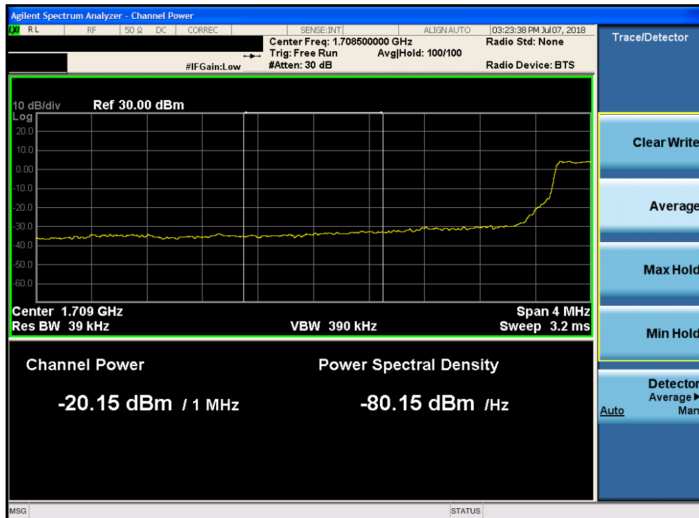
Plot 7-207. Lower Extended Band Edge Plot (Band 4 - 5.0MHz QPSK - Full RB Configuration)
