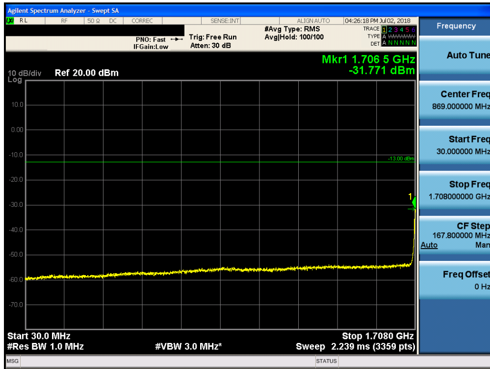
Plot 7-124. Conducted Spurious Plot (Band 4 - 10.0MHz QPSK - RB Size 1, RB Offset 0 - Low Channel)
