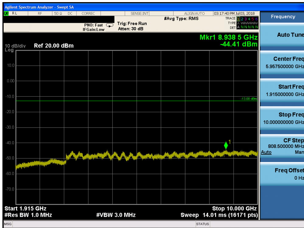
Plot 7-134. Conducted Spurious Plot (Band 25 - 15.0MHz QPSK - RB Size 1, RB Offset 0 - Low Channel)
