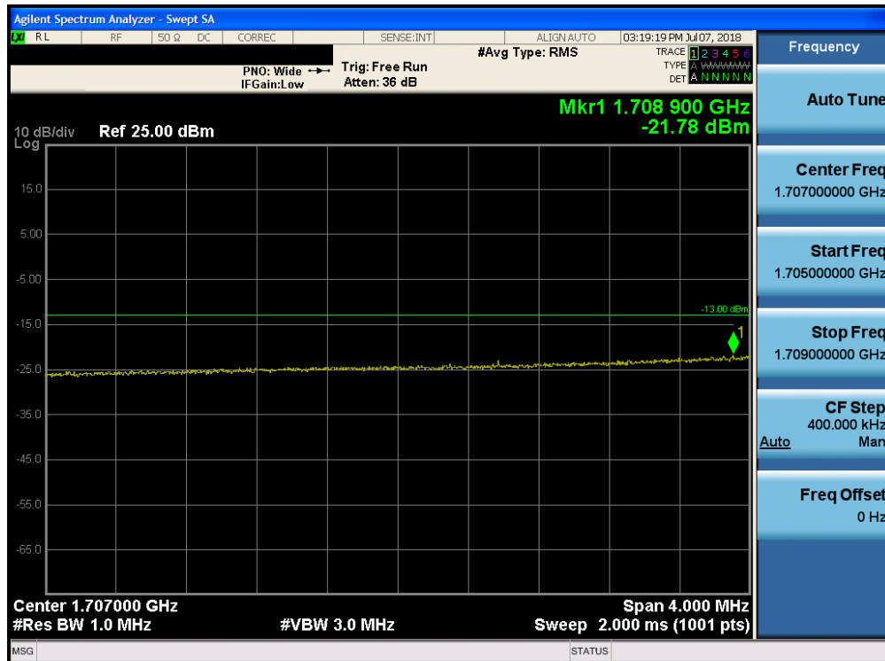
Plot 7-219. Lower Extended Band Edge Plot (Band 4 - 20.0MHz QPSK - Full RB Configuration)
