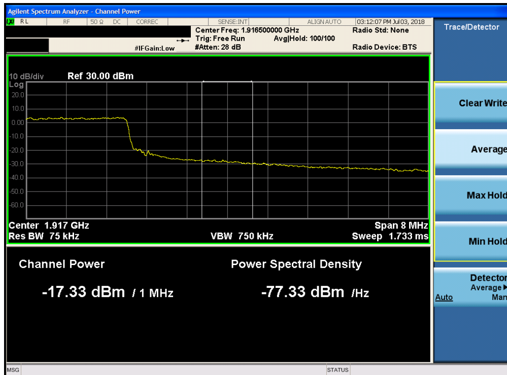
Plot 7-237. Upper Extended Band Edge Plot (Band 25 - 10.0MHz QPSK - Full RB Configuration)
