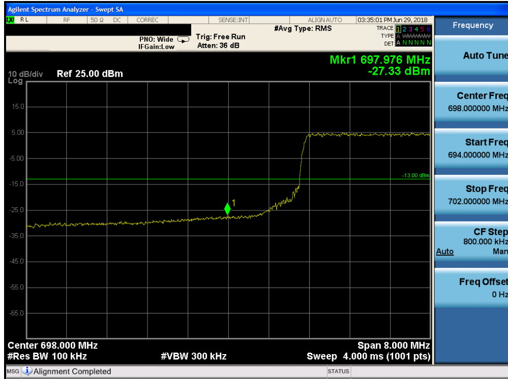
Plot 7-166. Lower Band Edge Plot (Band 12 - 10.0MHz QPSK - Full RB Configuration)
