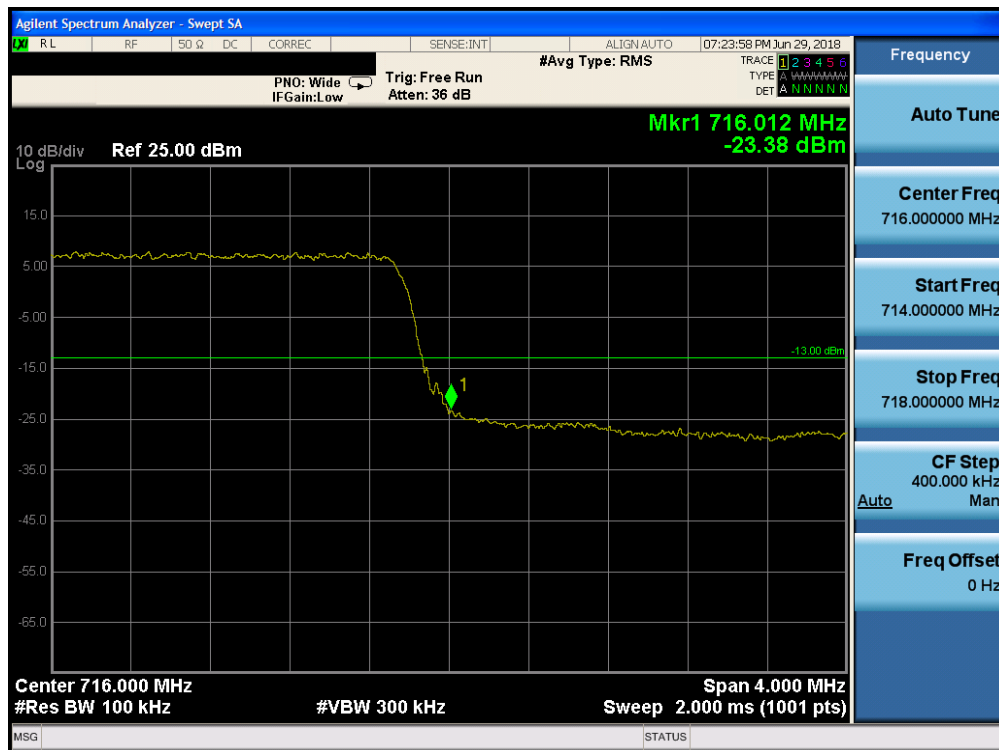
Plot 7-169. Upper Band Edge Plot (Band 17 - 5.0MHz QPSK - Full RB Configuration)
