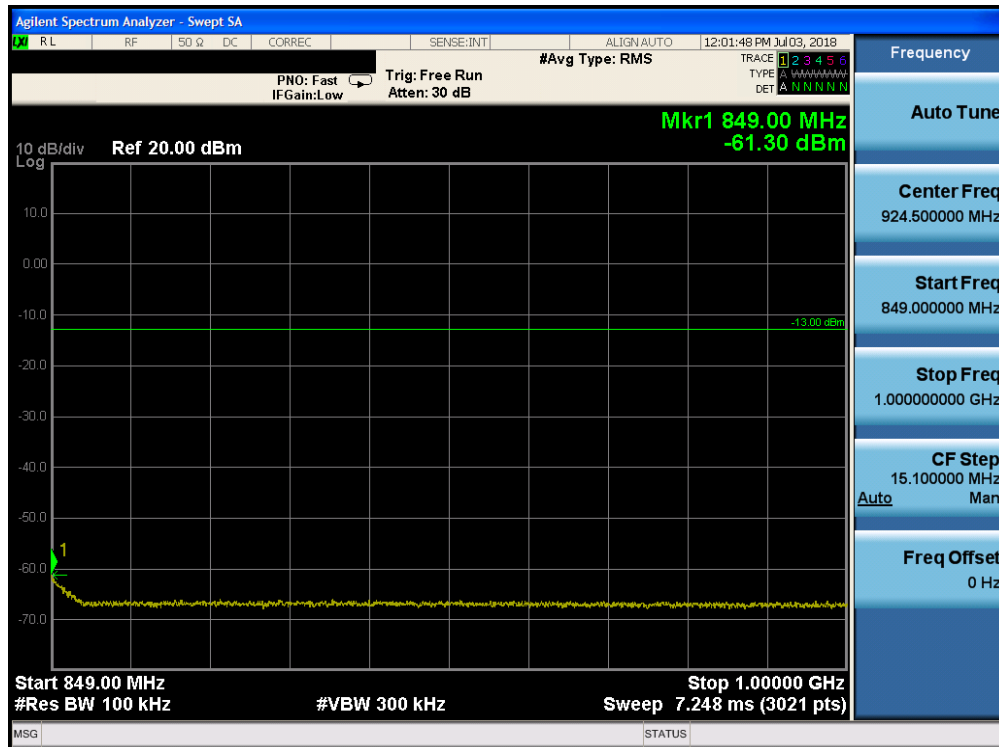
Plot 7-119. Conducted Spurious Plot (Band 5 - 3.0MHz QPSK - RB Size 1, RB Offset 0 - Mid Channel)
