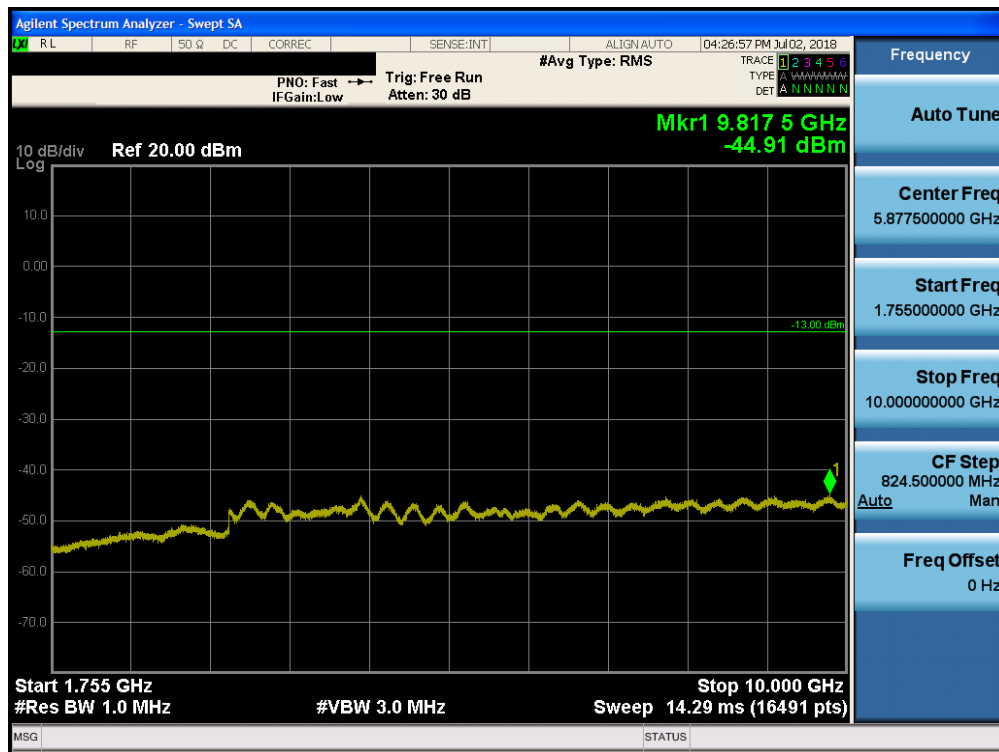
Plot 7-125. Conducted Spurious Plot (Band 4 - 10.0MHz QPSK - RB Size 1, RB Offset 0 - Low Channel)
