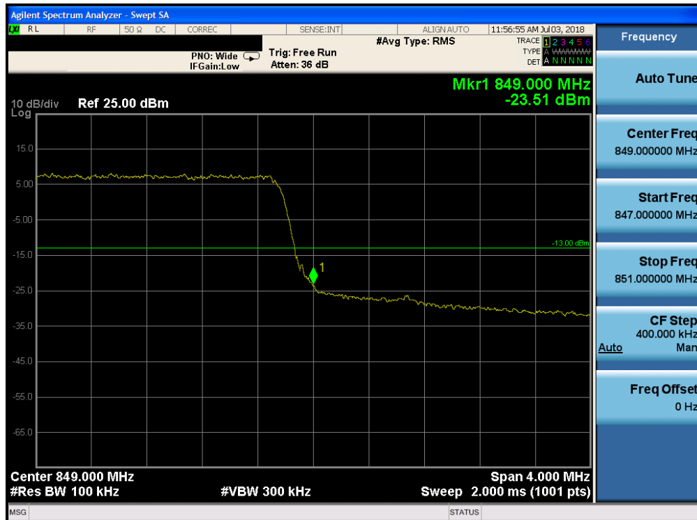
Plot 7-195. Upper Band Edge Plot (Band 5 - 5.0MHz QPSK - Full RB Configuration)
