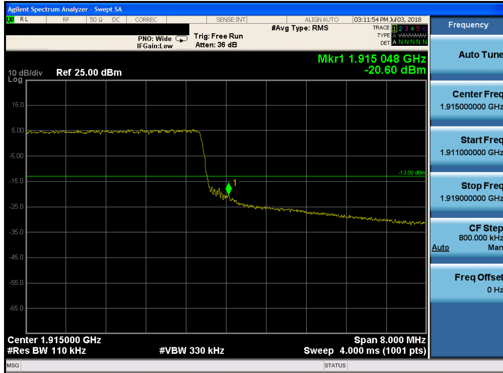
Plot 7-236. Upper Band Edge Plot (Band 25 - 10.0MHz QPSK - Full RB Configuration)
