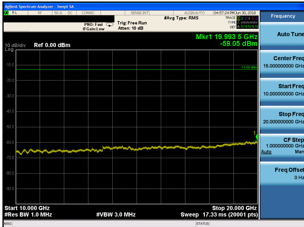
Plot 7-147. Conducted Spurious Plot (Band 2 - 20.0MHz QPSK - RB Size 1, RB Offset 0 - Mid Channel)
