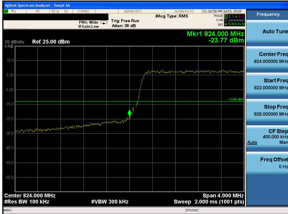
Plot 7-184. Lower Band Edge Plot (Band 26 - 5.0MHz QPSK - Full RB Configuration)
