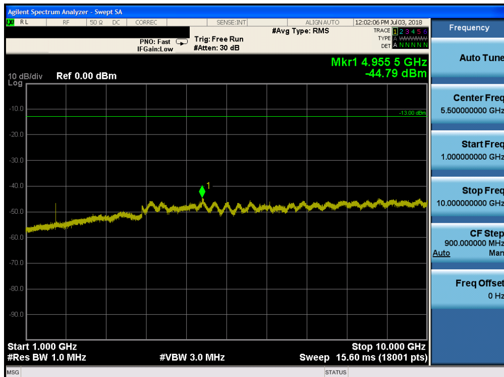
Plot 7-120. Conducted Spurious Plot (Band 5 - 3.0MHz QPSK - RB Size 1, RB Offset 0 - Mid Channel)
