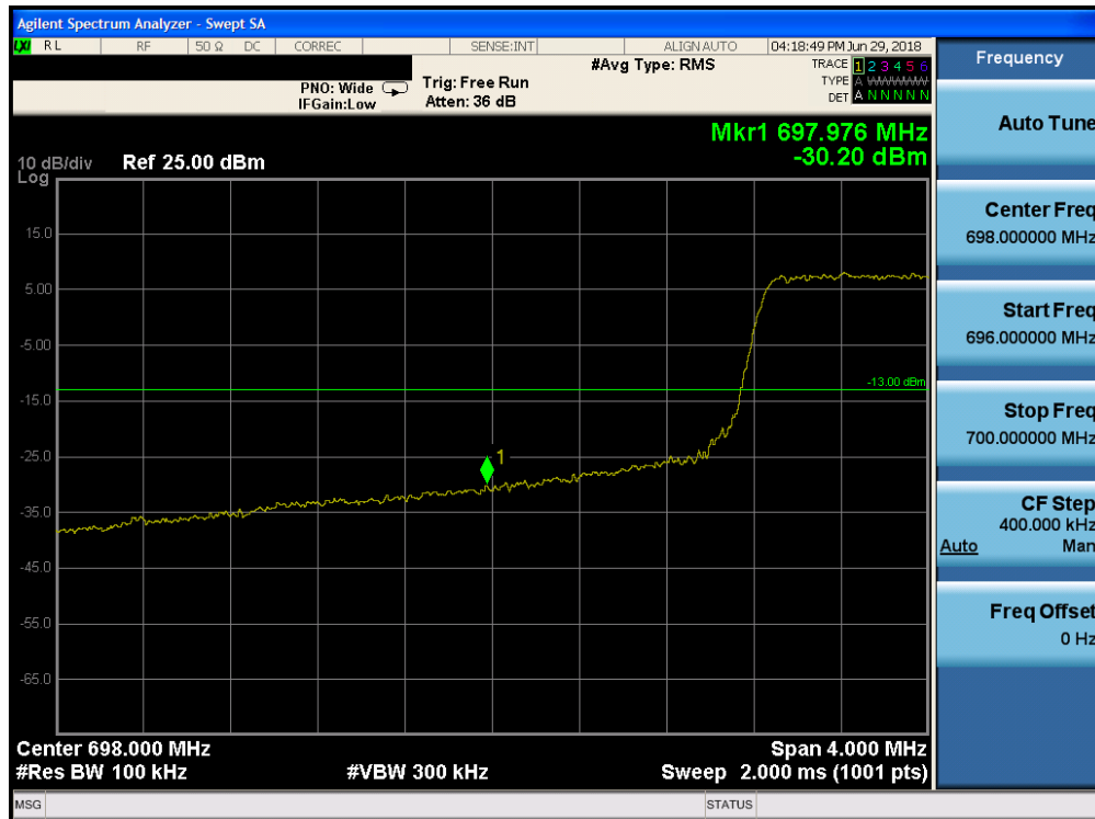
Plot 7-164. Lower Band Edge Plot (Band 12 - 5.0MHz QPSK - Full RB Configuration)
