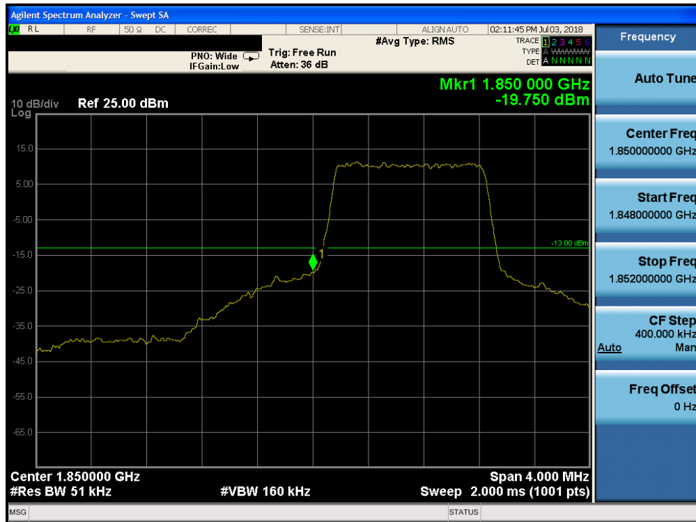
Plot 7-222. Lower Band Edge Plot (Band 25 - 1.4MHz QPSK - Full RB Configuration)
