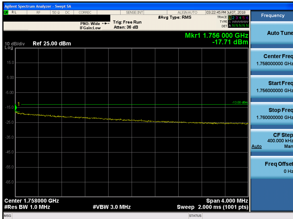
Plot 7-213. Upper Extended Band Edge Plot (Band 4 - 10.0MHz QPSK - Full RB Configuration)
