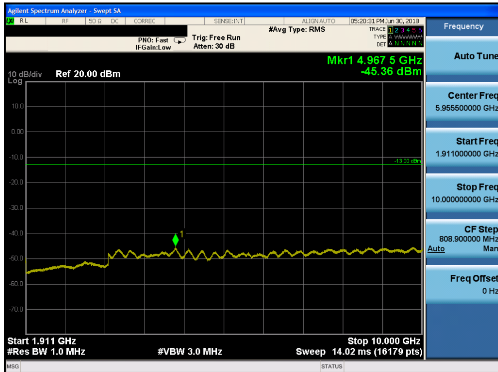
Plot 7-149. Conducted Spurious Plot (Band 2 - 20.0MHz QPSK - RB Size 1, RB Offset 0 - High Channel)
