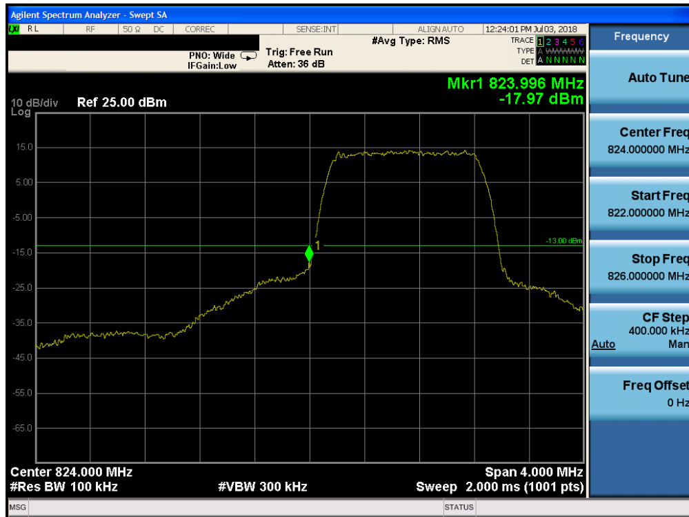
Plot 7-180. Lower Band Edge Plot (Band 26 - 1.4MHz QPSK - Full RB Configuration)
