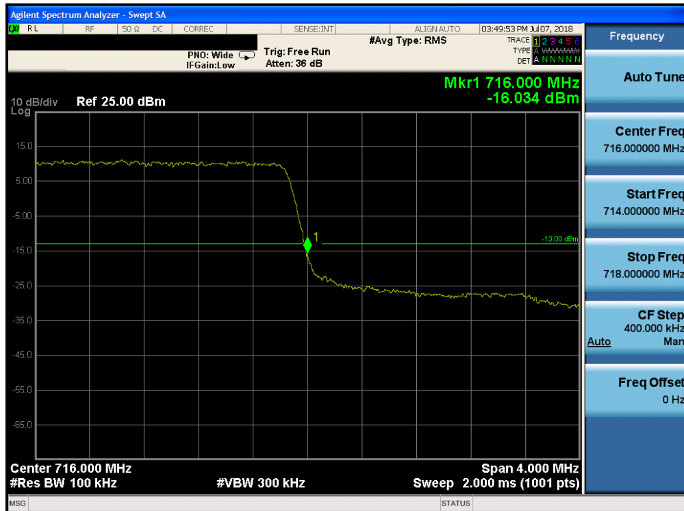
Plot 7-163. Upper Band Edge Plot (Band 12 - 3.0MHz QPSK - Full RB Configuration)
