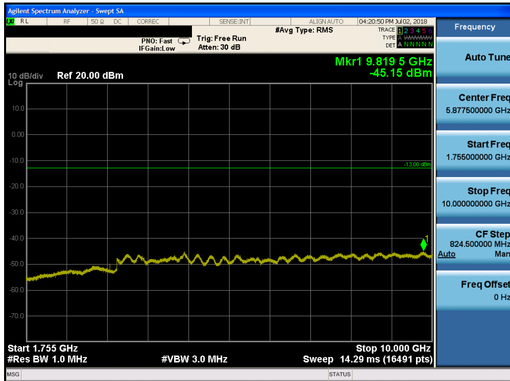
Plot 7-128. Conducted Spurious Plot (Band 4 - 10.0MHz QPSK - RB Size 1, RB Offset 0 - Mid Channel)
