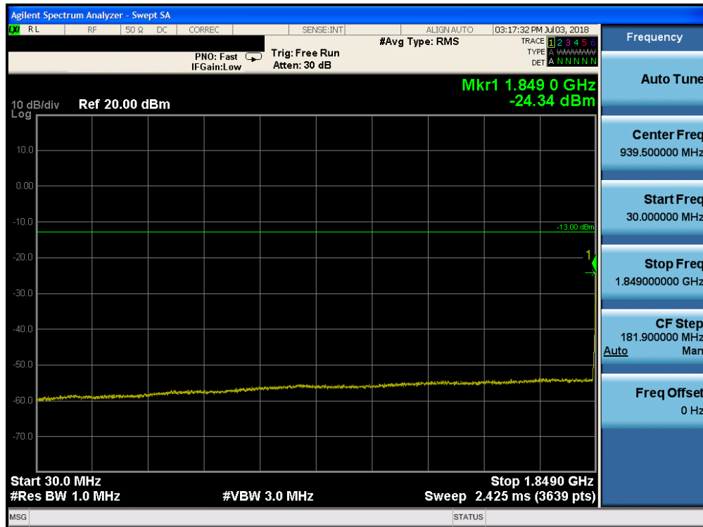
Plot 7-133. Conducted Spurious Plot (Band 25 - 15.0MHz QPSK - RB Size 1, RB Offset 0 - Low Channel)
