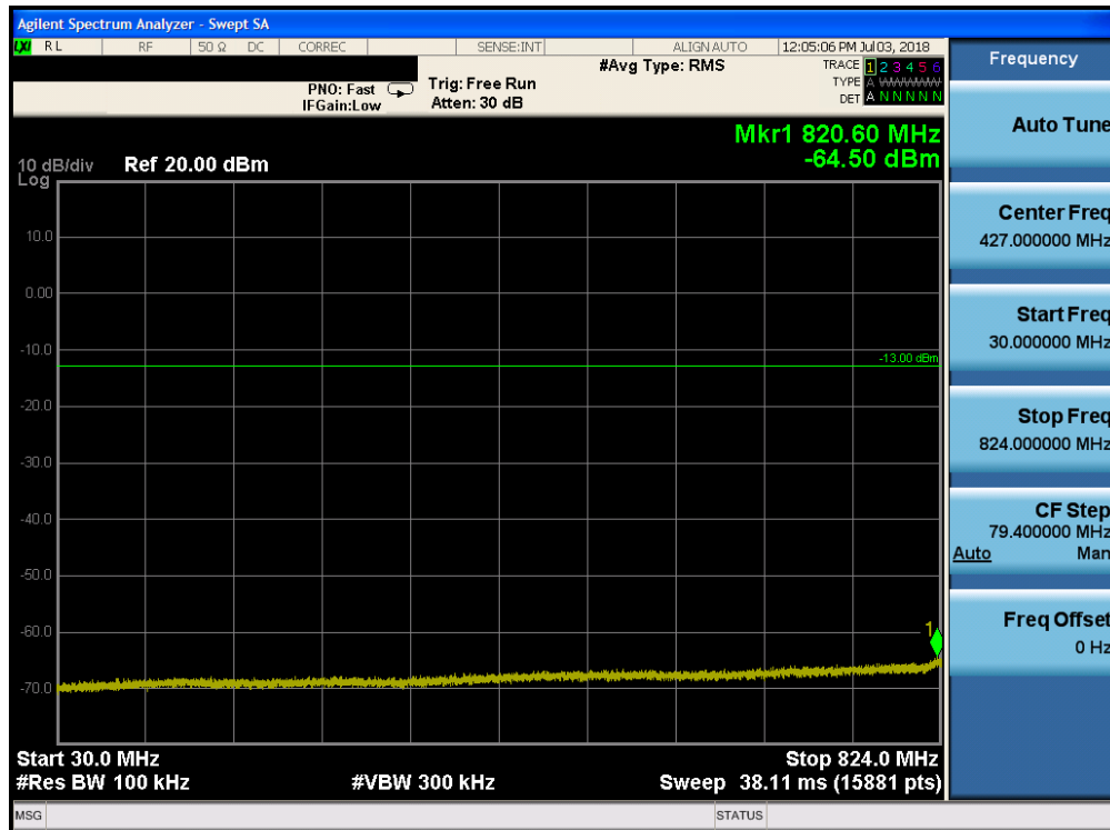
Plot 7-121. Conducted Spurious Plot (Band 5 - 3.0MHz QPSK - RB Size 1, RB Offset 0 - High Channel)
