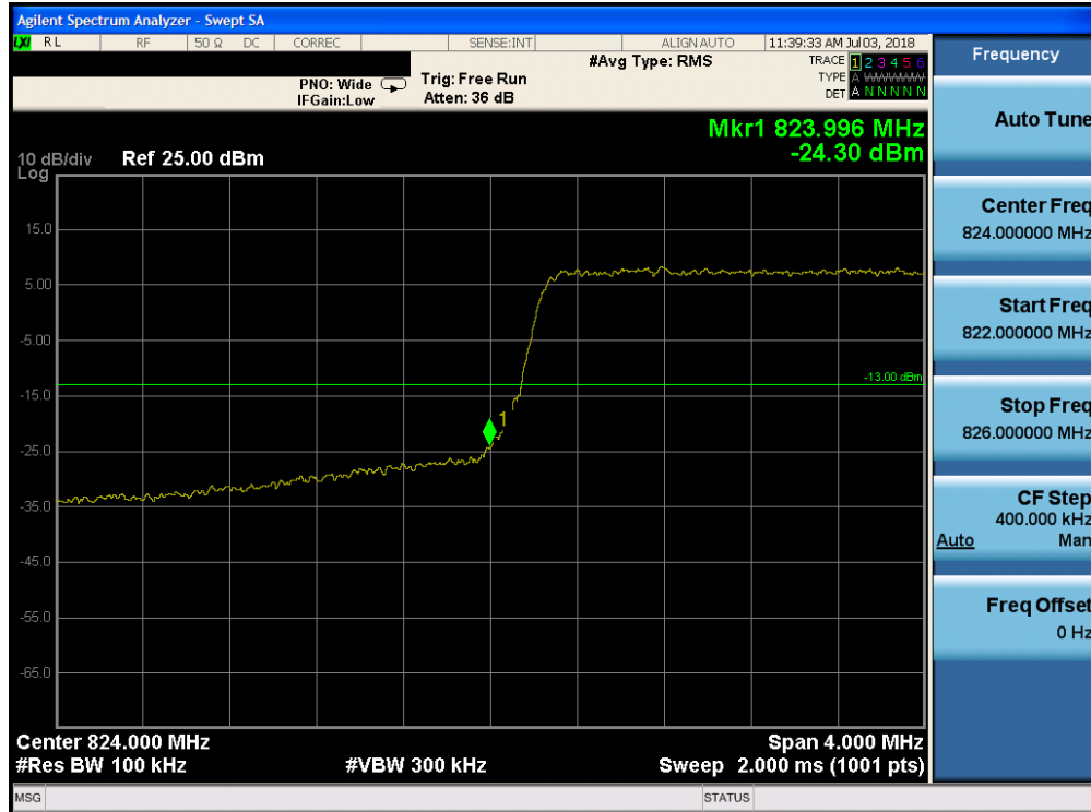
Plot 7-194. Lower Band Edge Plot (Band 5 - 5.0MHz QPSK - Full RB Configuration)
