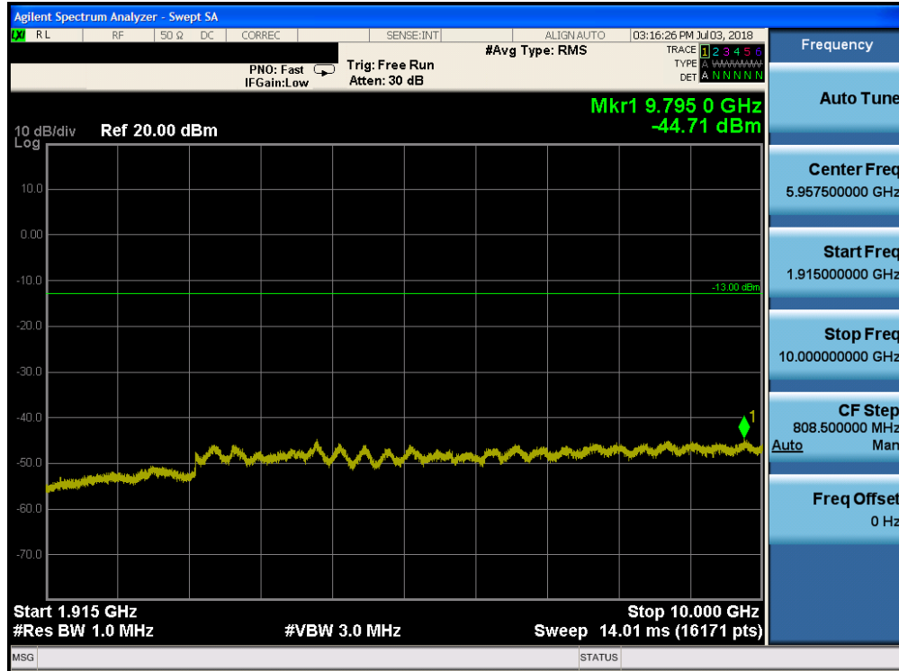
Plot 7-137. Conducted Spurious Plot (Band 25 - 15.0MHz QPSK - RB Size 1, RB Offset 0 - Mid Channel)
