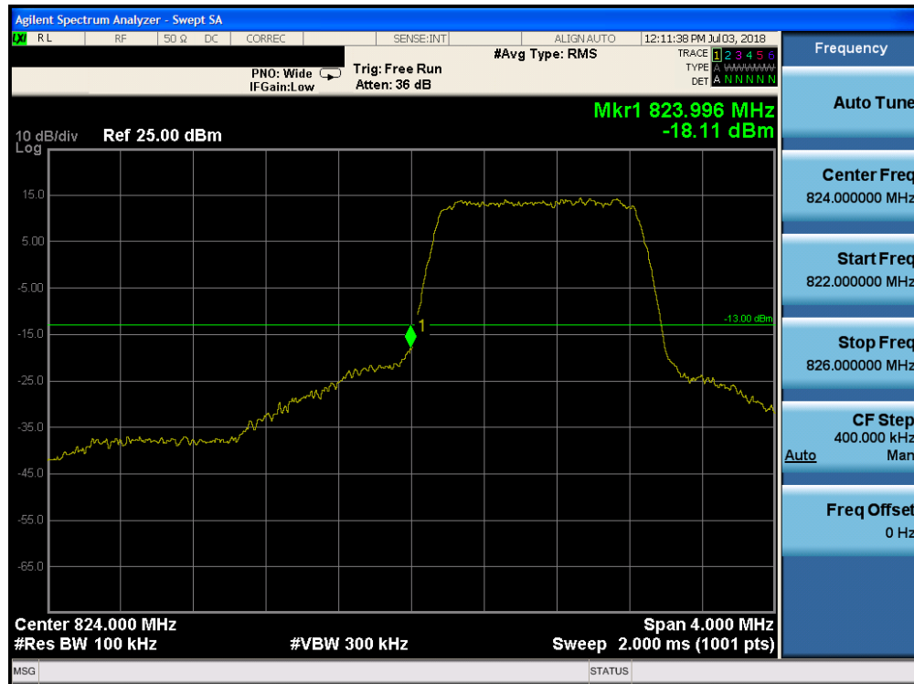
Plot 7-190. Lower Band Edge Plot (Band 5 - 1.4MHz QPSK - Full RB Configuration)
