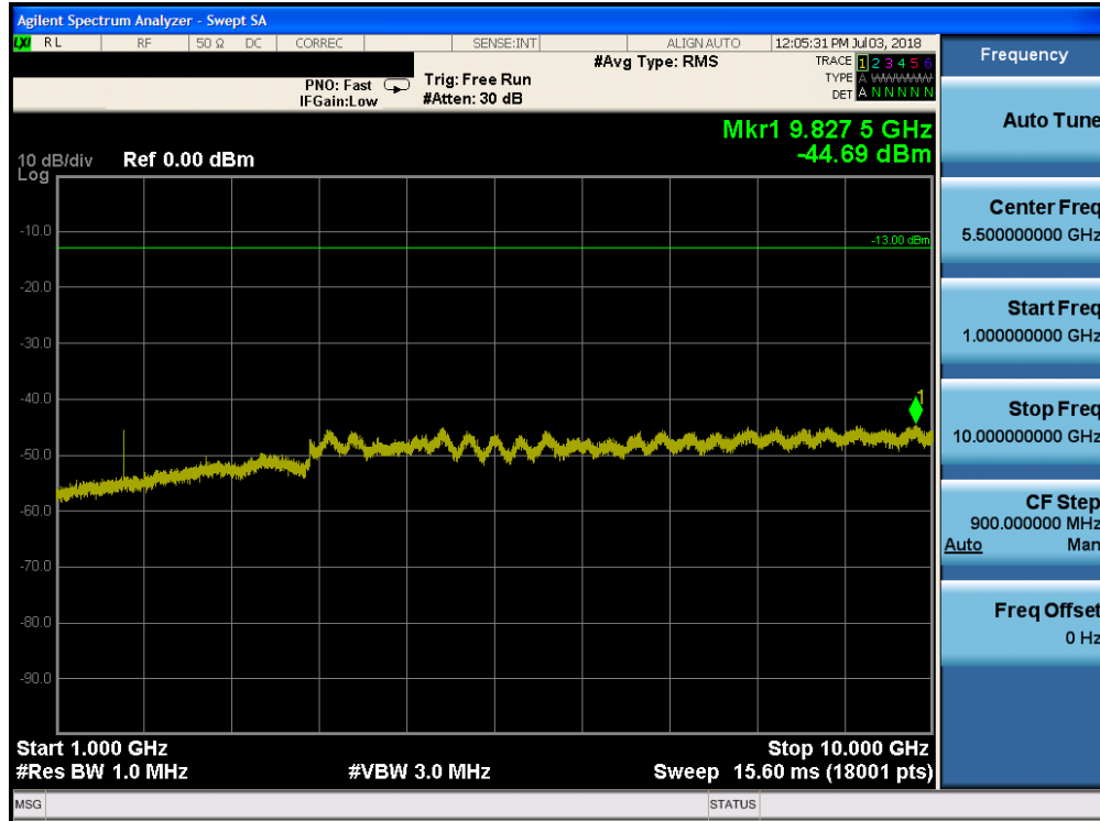
Plot 7-123. Conducted Spurious Plot (Band 5 - 3.0MHz QPSK - RB Size 1, RB Offset 0 - High Channel)
