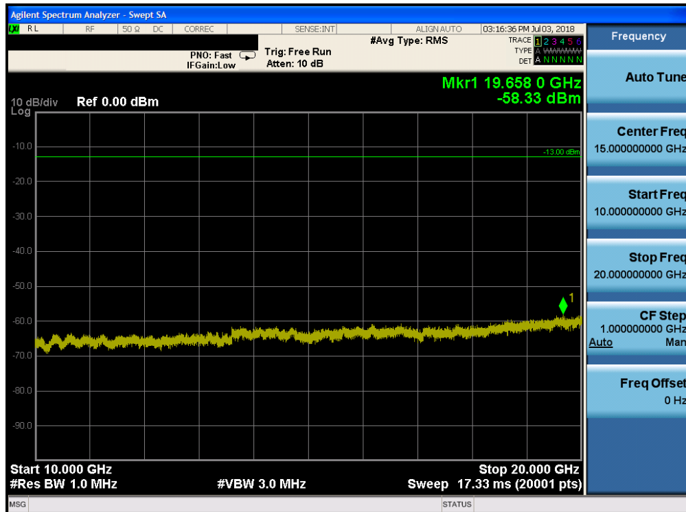
Plot 7-138. Conducted Spurious Plot (Band 25 - 15.0MHz QPSK - RB Size 1, RB Offset 0 - Mid Channel)
