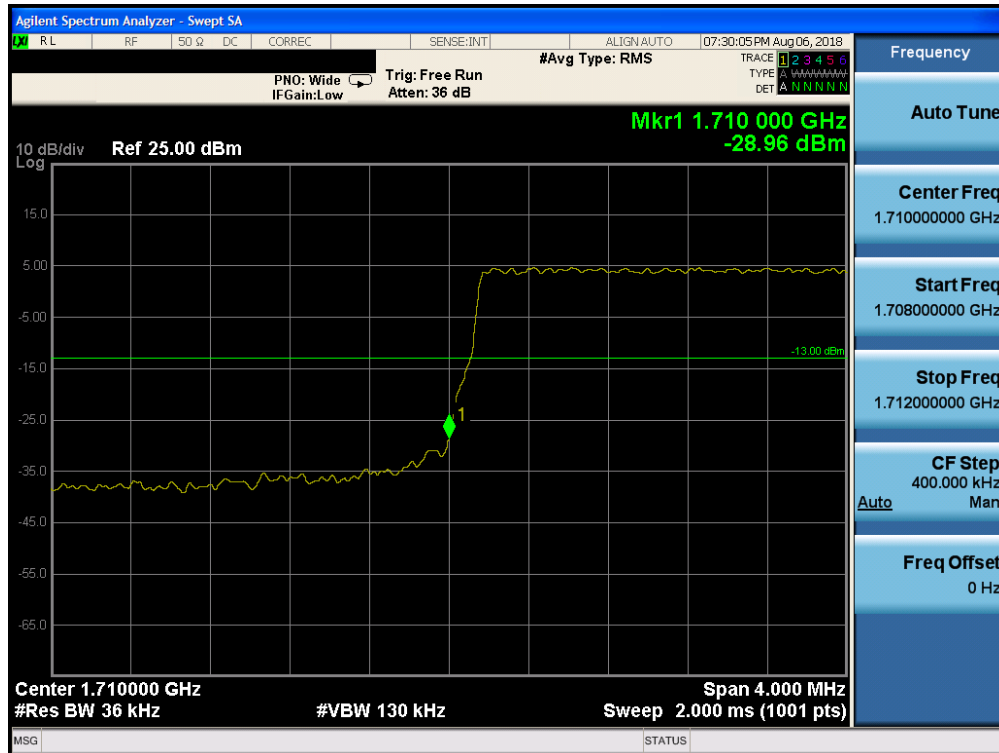
Plot 7-202. Lower Band Edge Plot (Band 4 - 3.0MHz QPSK - Full RB Configuration)
