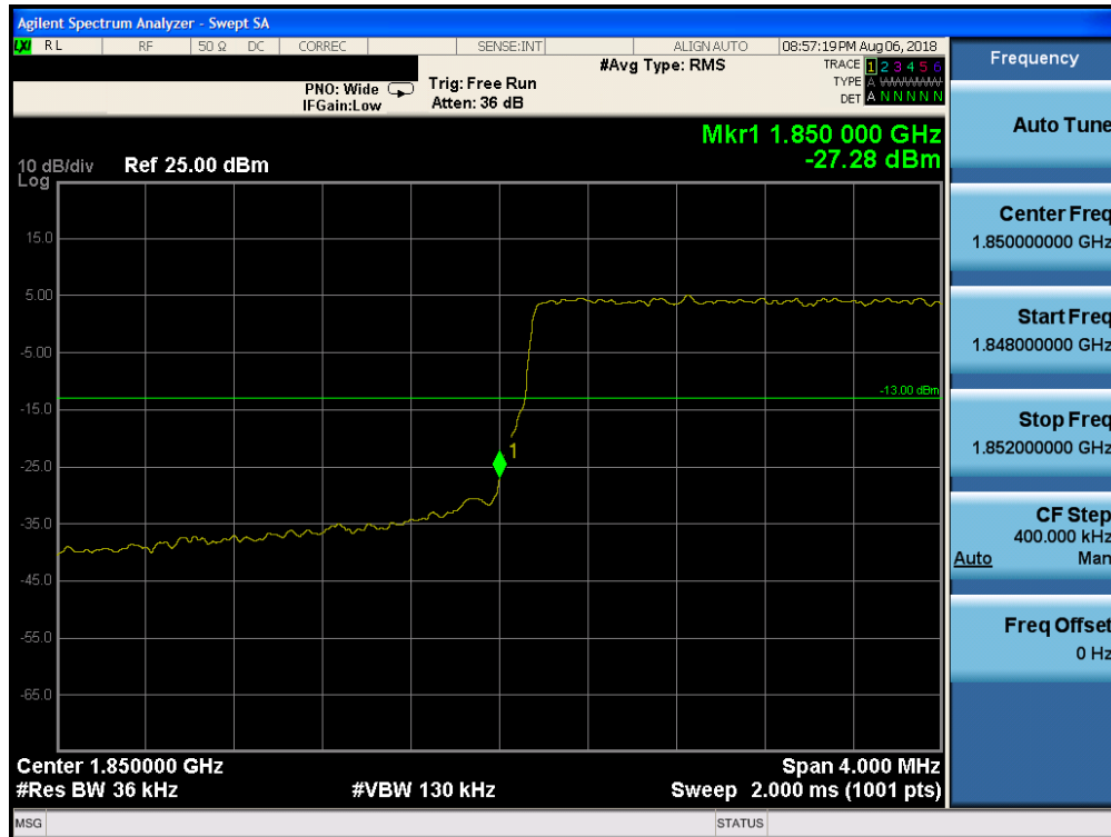
Plot 7-226. Lower Band Edge Plot (Band 25 - 3.0MHz QPSK - Full RB Configuration)
