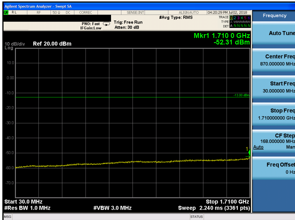
Plot 7-127. Conducted Spurious Plot (Band 4 - 10.0MHz QPSK - RB Size 1, RB Offset 0 - Mid Channel)
