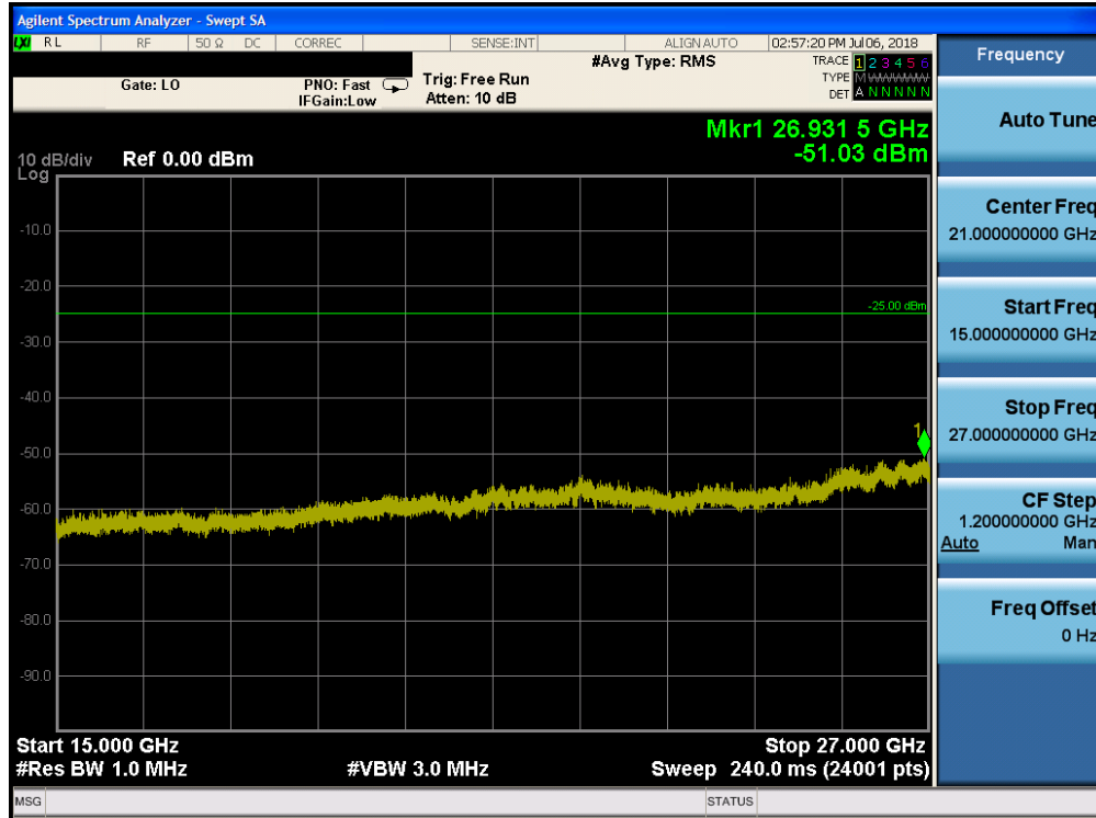
Plot 7-153. Conducted Spurious Plot (Band 41 - 20.0MHz QPSK - RB Size 1, RB Offset 0 - Low Channel)
