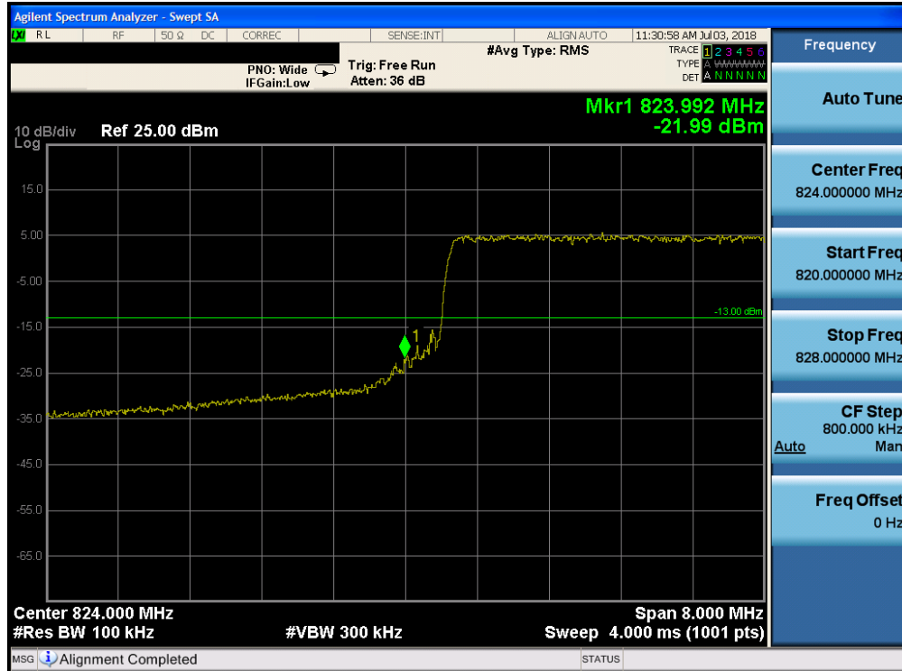
Plot 7-196. Lower Band Edge Plot (Band 5 - 10.0MHz QPSK - Full RB Configuration)
