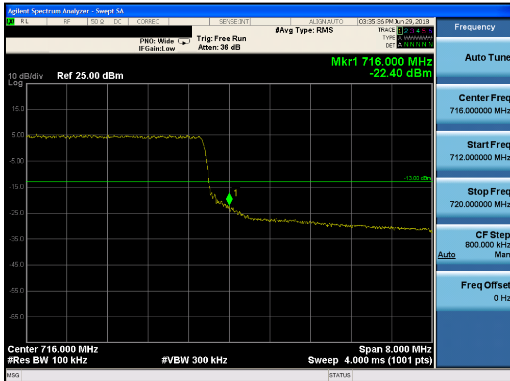
Plot 7-167. Upper Band Edge Plot (Band 12 - 10.0MHz QPSK - Full RB Configuration)
