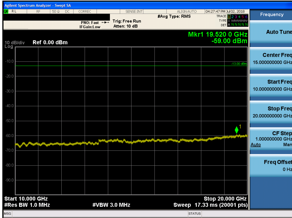
Plot 7-126. Conducted Spurious Plot (Band 4 - 10.0MHz QPSK - RB Size 1, RB Offset 0 - Low Channel)
