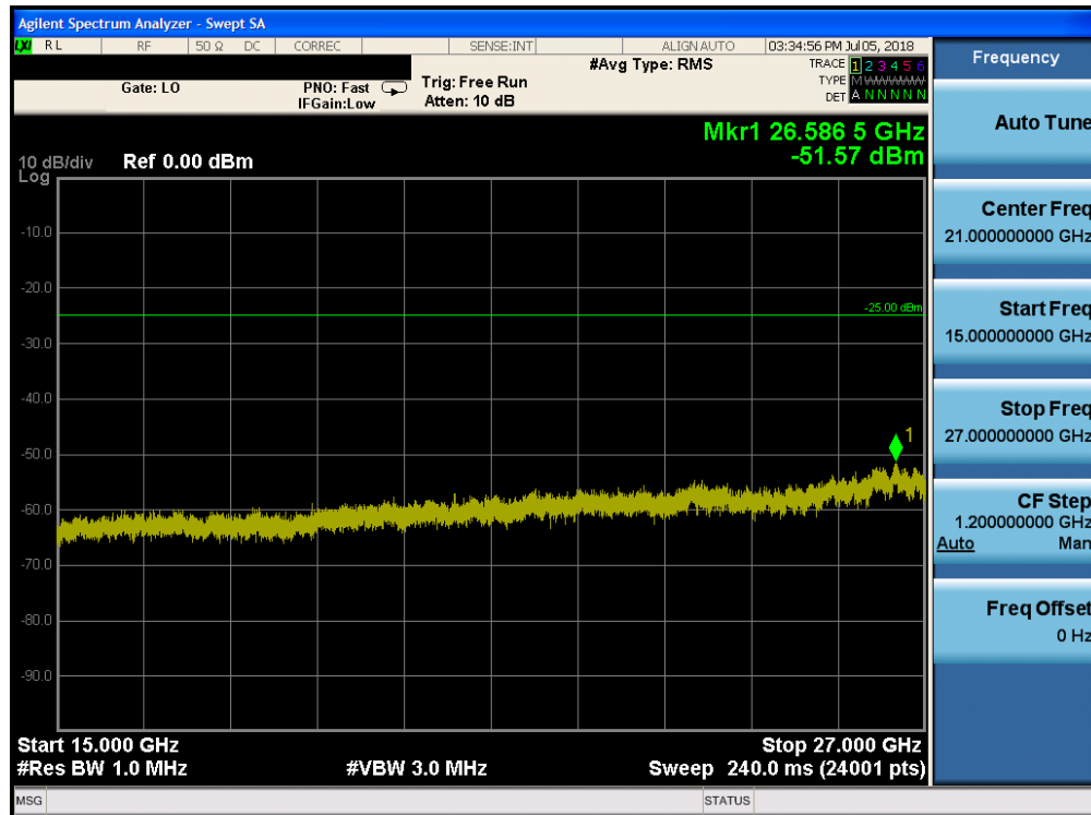
Plot 7-159. Conducted Spurious Plot (Band 41 - 20.0MHz QPSK - RB Size 1, RB Offset 0 - High Channel)
