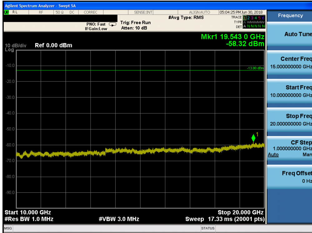
Plot 7-144. Conducted Spurious Plot (Band 2 - 20.0MHz QPSK - RB Size 1, RB Offset 0 - Low Channel)
