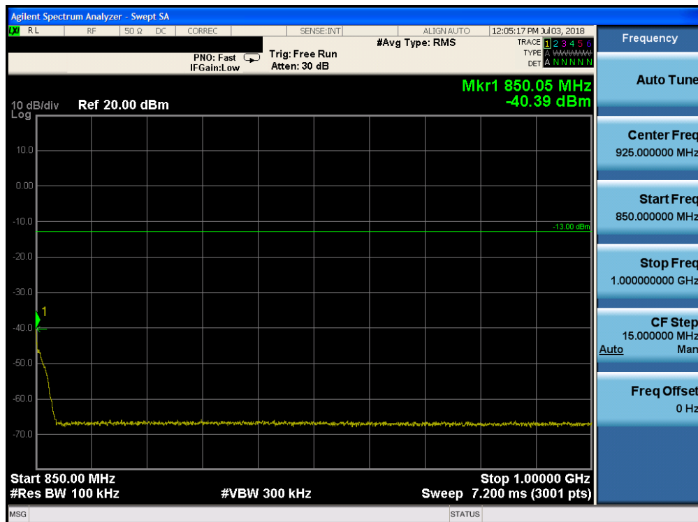
Plot 7-122. Conducted Spurious Plot (Band 5 - 3.0MHz QPSK - RB Size 1, RB Offset 0 - High Channel)
