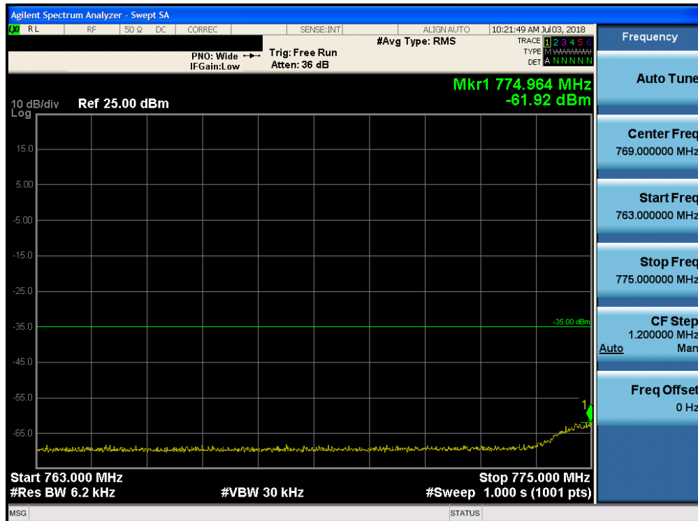
Plot 7-177. Lower Emission Mask Edge Plot (Band 13 - 10.0MHz QPSK - Full RB Configuration)
