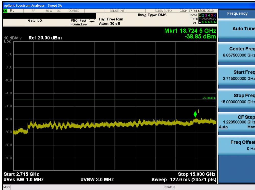
Plot 7-158. Conducted Spurious Plot (Band 41 - 20.0MHz QPSK - RB Size 1, RB Offset 0 - High Channel)
