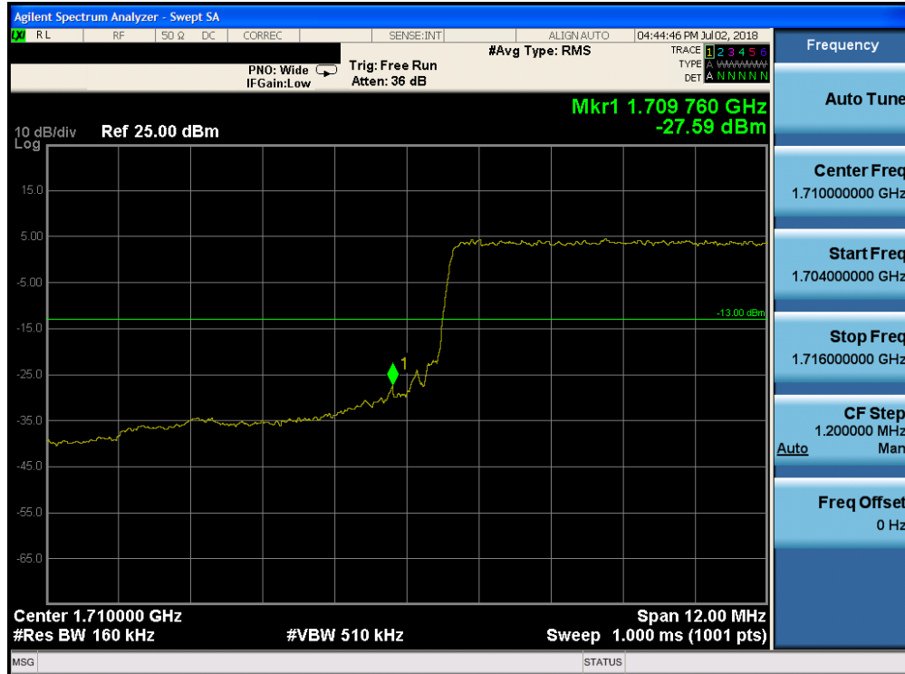
Plot 7-214. Lower Band Edge Plot (Band 4 - 15.0MHz QPSK - Full RB Configuration)
