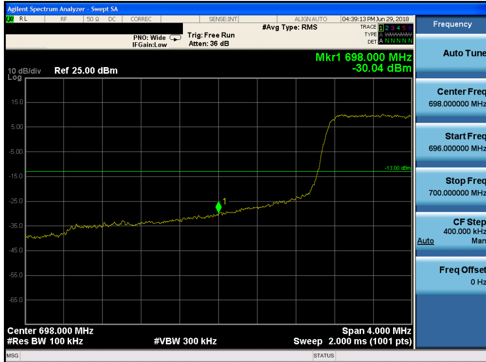
Plot 7-162. Lower Band Edge Plot (Band 12 - 3.0MHz QPSK - Full RB Configuration)
