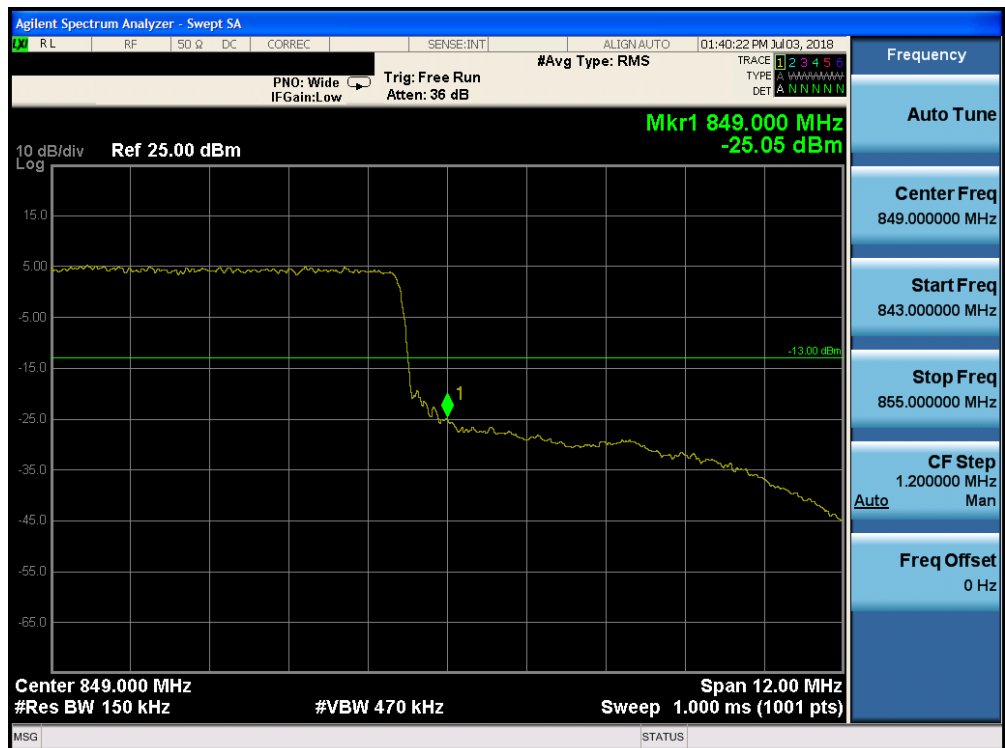
Plot 7-189. Upper Band Edge Plot (Band 26 - 15.0MHz QPSK - Full RB Configuration)
