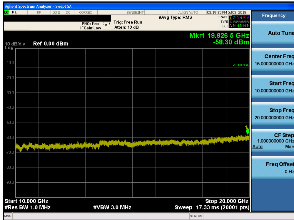
Plot 7-141. Conducted Spurious Plot (Band 25 - 15.0MHz QPSK - RB Size 1, RB Offset 0 - High Channel)
