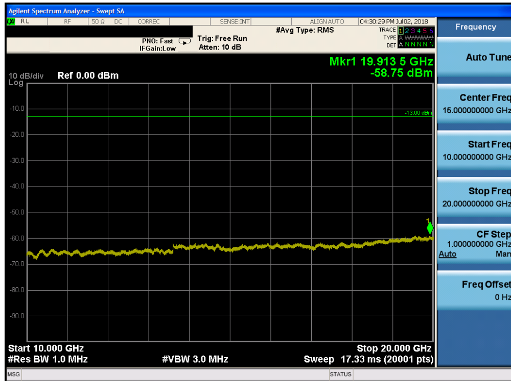
Plot 7-132. Conducted Spurious Plot (Band 4 - 10.0MHz QPSK - RB Size 1, RB Offset 0 - High Channel)
