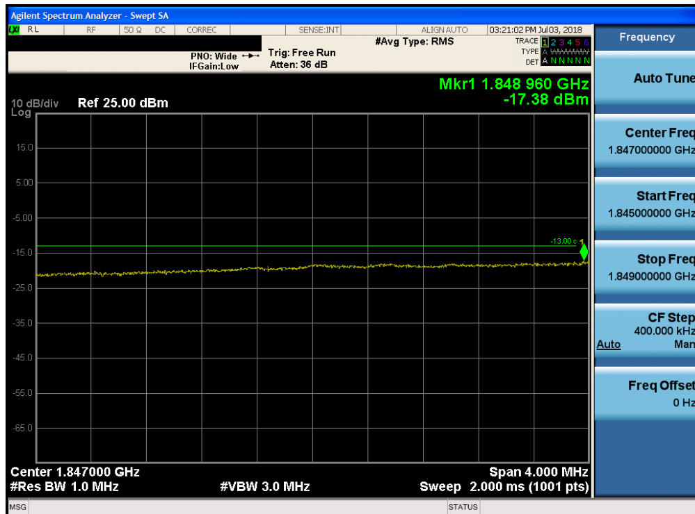
Plot 7-239. Lower Extended Band Edge Plot (Band 25 - 15.0MHz QPSK - Full RB Configuration)
