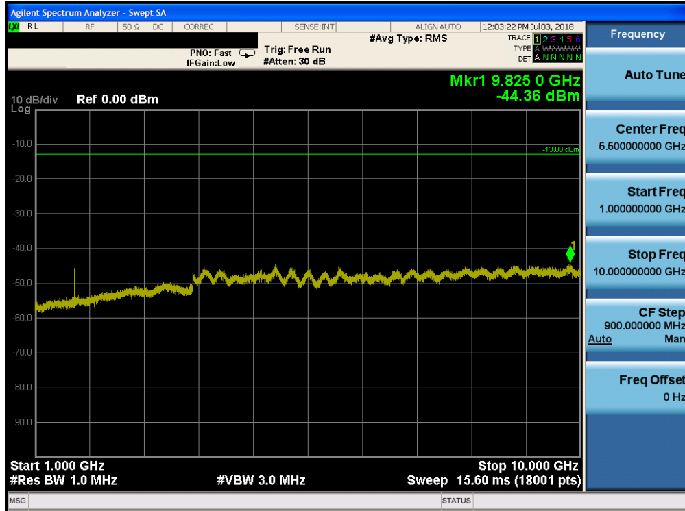
Plot 7-117. Conducted Spurious Plot (Band 5 - 3.0MHz QPSK - RB Size 1, RB Offset 0 - Low Channel)
