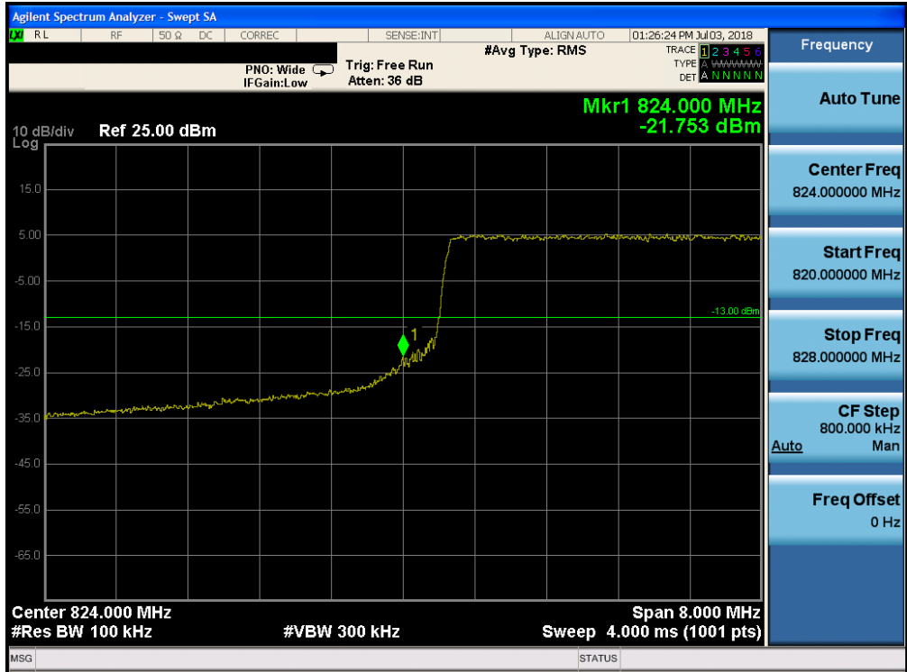
Plot 7-186. Lower Band Edge Plot (Band 26 - 10.0MHz QPSK - Full RB Configuration)
