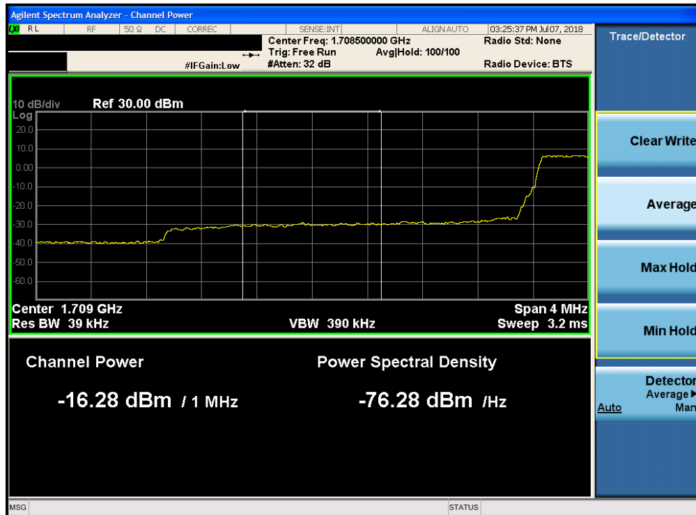
Plot 7-203. Lower Extended Band Edge Plot (Band 4 - 3.0MHz QPSK - Full RB Configuration)
