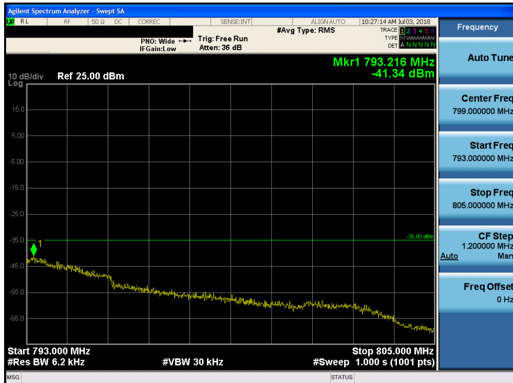
Plot 7-179. Upper Emission Mask Edge Plot (Band 13 - 10.0MHz QPSK - Full RB Configuration)
