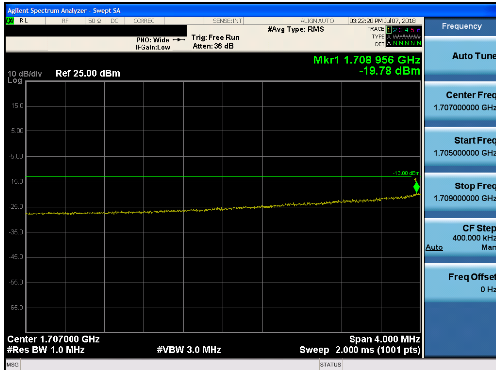
Plot 7-211. Lower Extended Band Edge Plot (Band 4 - 10.0MHz QPSK - Full RB Configuration)
