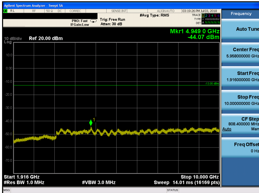
Plot 7-140. Conducted Spurious Plot (Band 25 - 15.0MHz QPSK - RB Size 1, RB Offset 0 - High Channel)
