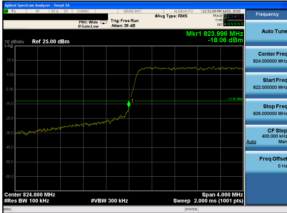
Plot 7-182. Lower Band Edge Plot (Band 26 - 3.0MHz QPSK - Full RB Configuration)
