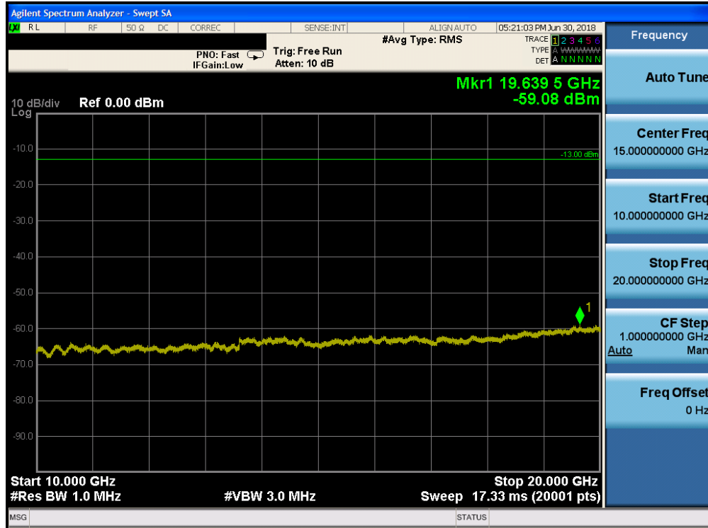
Plot 7-150. Conducted Spurious Plot (Band 2 - 20.0MHz QPSK - RB Size 1, RB Offset 0 - High Channel)
