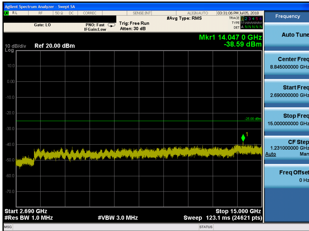
Plot 7-155. Conducted Spurious Plot (Band 41 - 20.0MHz QPSK - RB Size 1, RB Offset 0 - Mid Channel)
