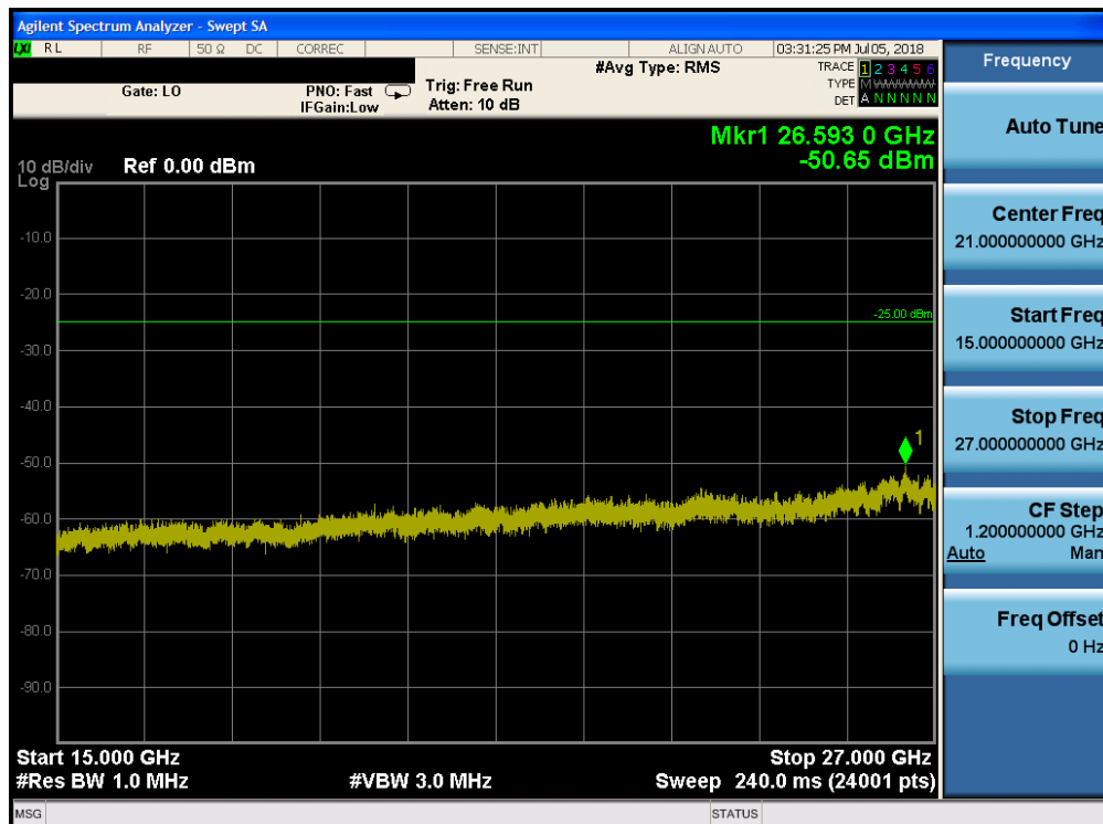
Plot 7-156. Conducted Spurious Plot (Band 41 - 20.0MHz QPSK - RB Size 1, RB Offset 0 - Mid Channel)
