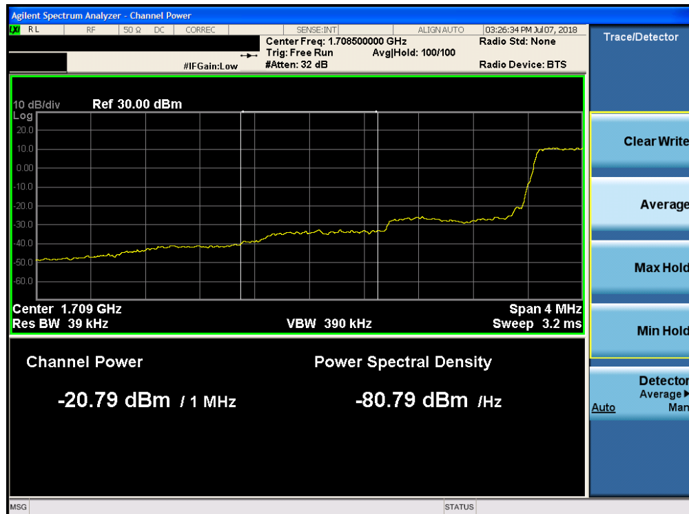
Plot 7-199. Lower Extended Band Edge Plot (Band 4 - 1.4MHz QPSK - Full RB Configuration)
