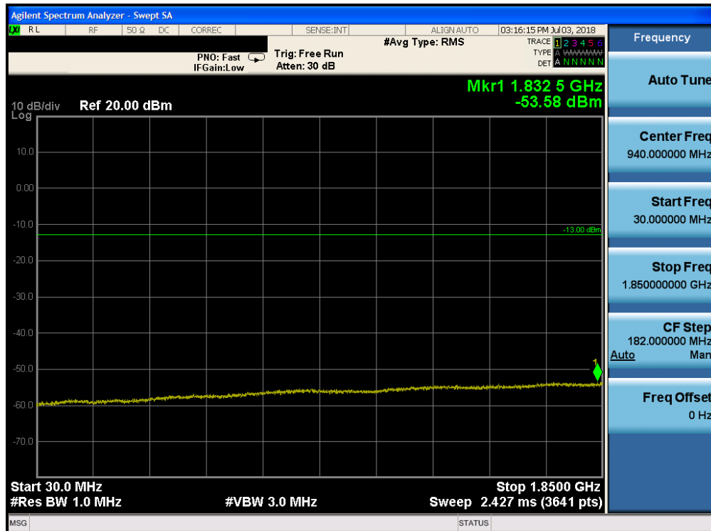
Plot 7-136. Conducted Spurious Plot (Band 25 - 15.0MHz QPSK - RB Size 1, RB Offset 0 - Mid Channel)
