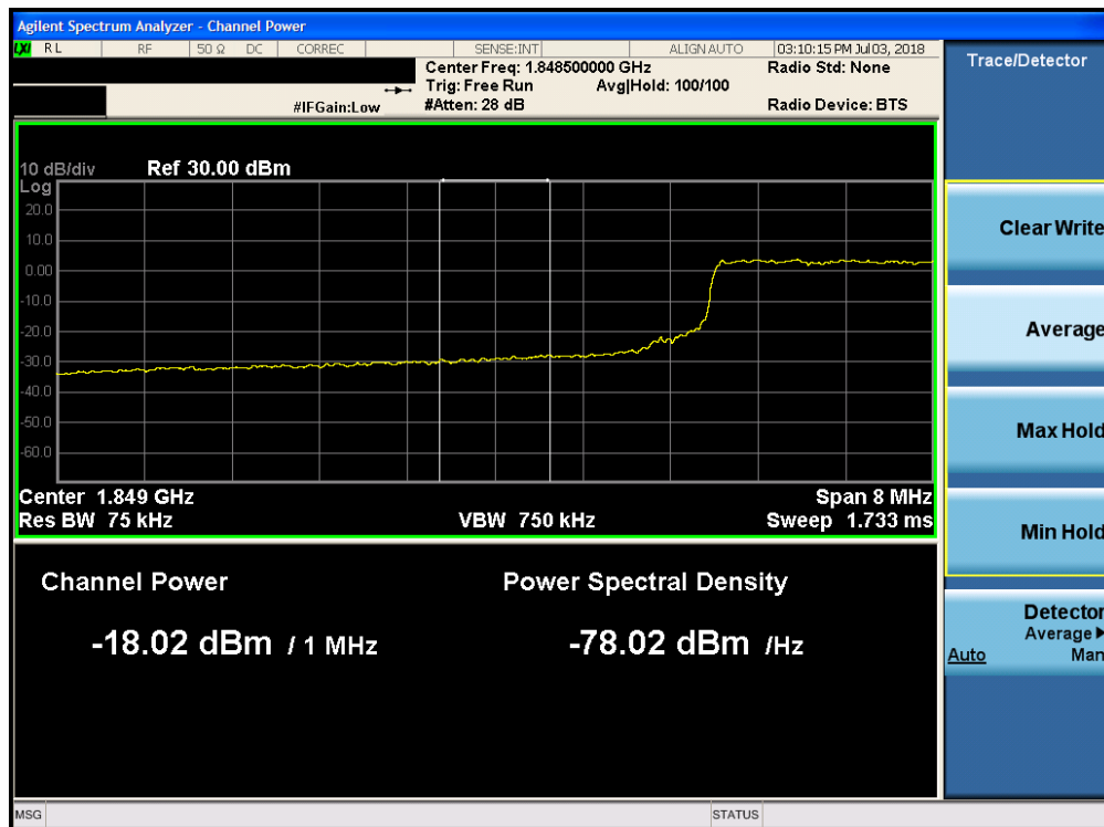
Plot 7-235. Lower Extended Band Edge Plot (Band 25 - 10.0MHz QPSK - Full RB Configuration)
