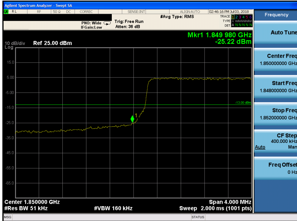
Plot 7-230. Lower Band Edge Plot (Band 25 - 5.0MHz QPSK - Full RB Configuration)
