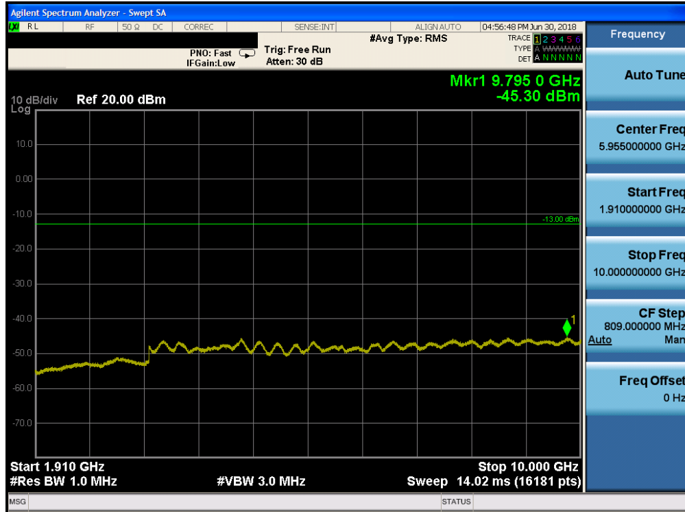
Plot 7-146. Conducted Spurious Plot (Band 2 - 20.0MHz QPSK - RB Size 1, RB Offset 0 - Mid Channel)
