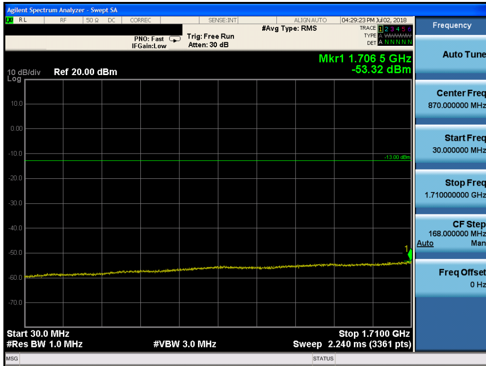
Plot 7-130. Conducted Spurious Plot (Band 4 - 10.0MHz QPSK - RB Size 1, RB Offset 0 - High Channel)
