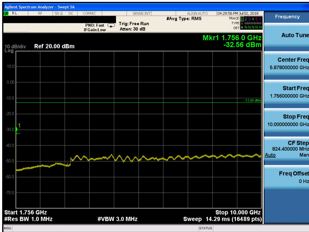
Plot 7-131. Conducted Spurious Plot (Band 4 - 10.0MHz QPSK - RB Size 1, RB Offset 0 - High Channel)
