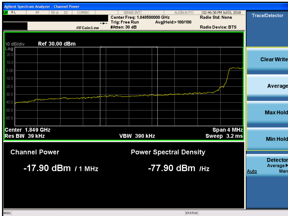
Plot 7-231. Lower Extended Band Edge Plot (Band 25 - 5.0MHz QPSK - Full RB Configuration)
