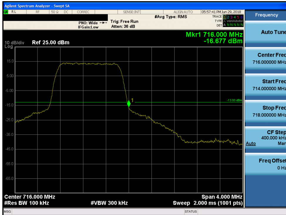
Plot 7-161. Upper Band Edge Plot (Band 12 - 1.4MHz QPSK - Full RB Configuration)
