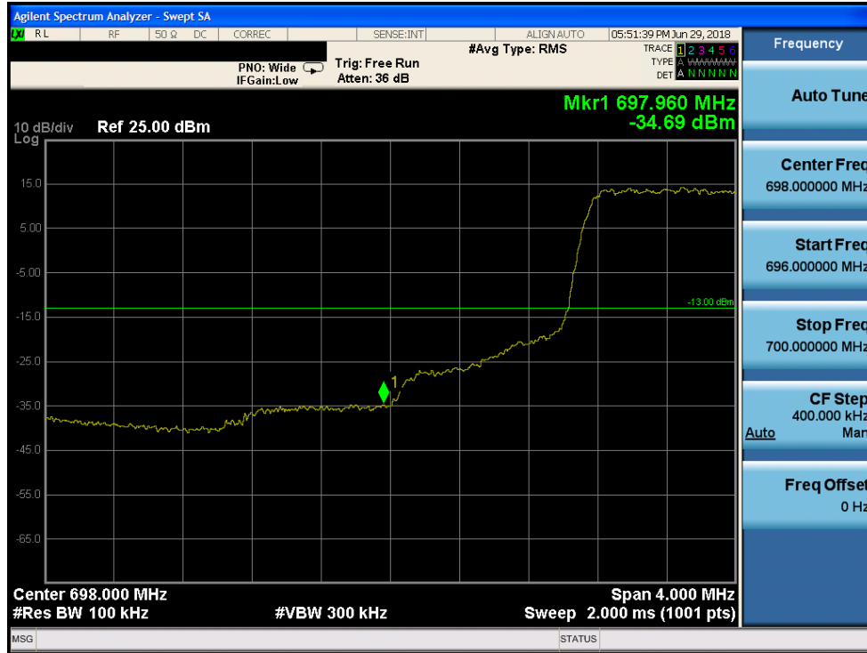
Plot 7-160. Lower Band Edge Plot (Band 12 - 1.4MHz QPSK - Full RB Configuration)
