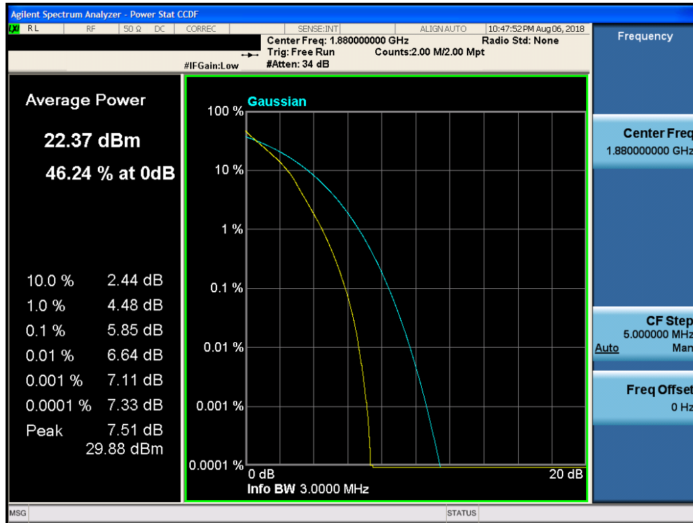
Plot 7-292. PAR Plot (Band 2 - 3.0MHz QPSK - Full RB Configuration)
