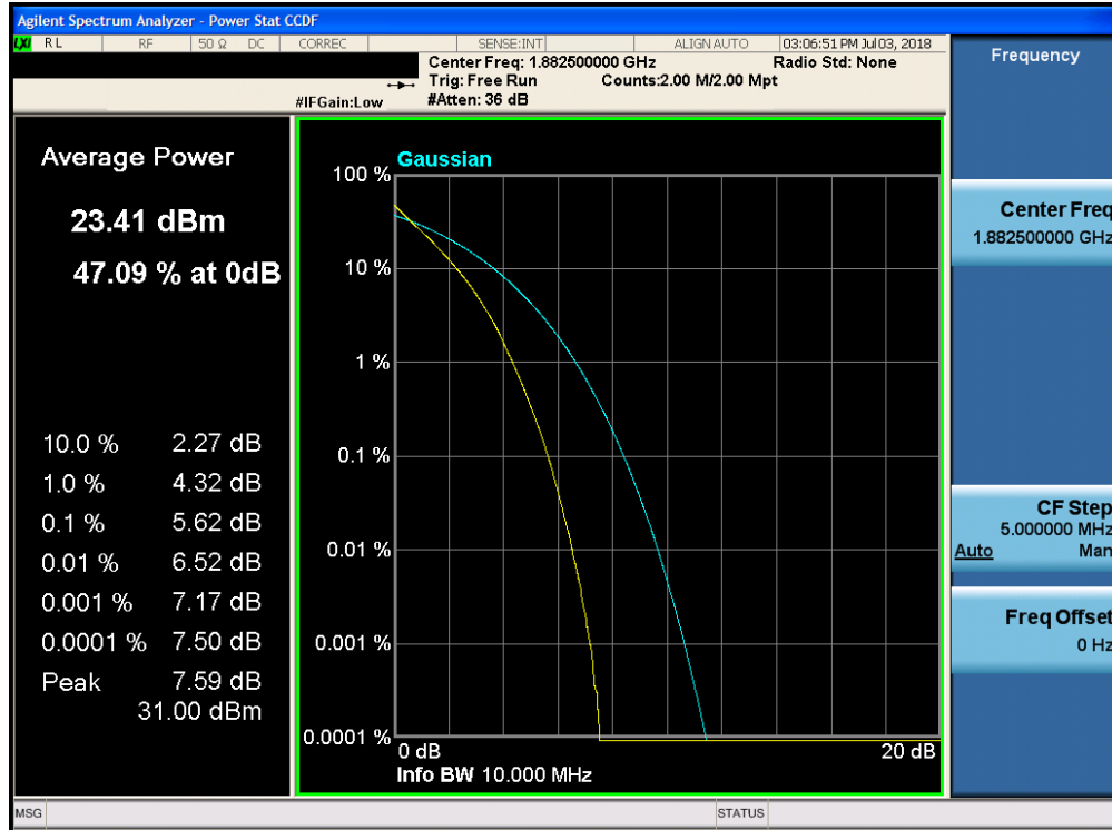
Plot 7-284. PAR Plot (Band 25 - 10.0MHz QPSK - Full RB Configuration)
