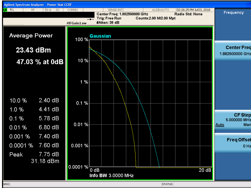
Plot 7-280. PAR Plot (Band 25 - 3.0MHz QPSK - Full RB Configuration)
