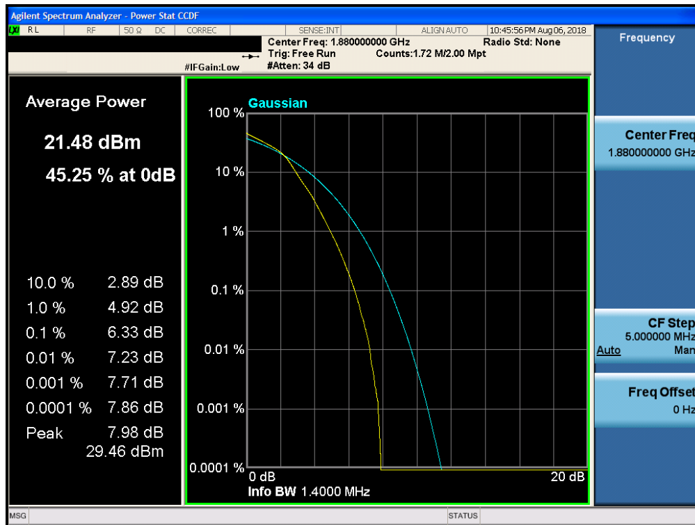
Plot 7-291. PAR Plot (Band 2 - 1.4MHz 16-QAM - Full RB Configuration)
