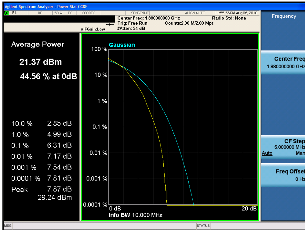
Plot 7-297. PAR Plot (Band 2 - 10.0MHz 16-QAM - Full RB Configuration)
