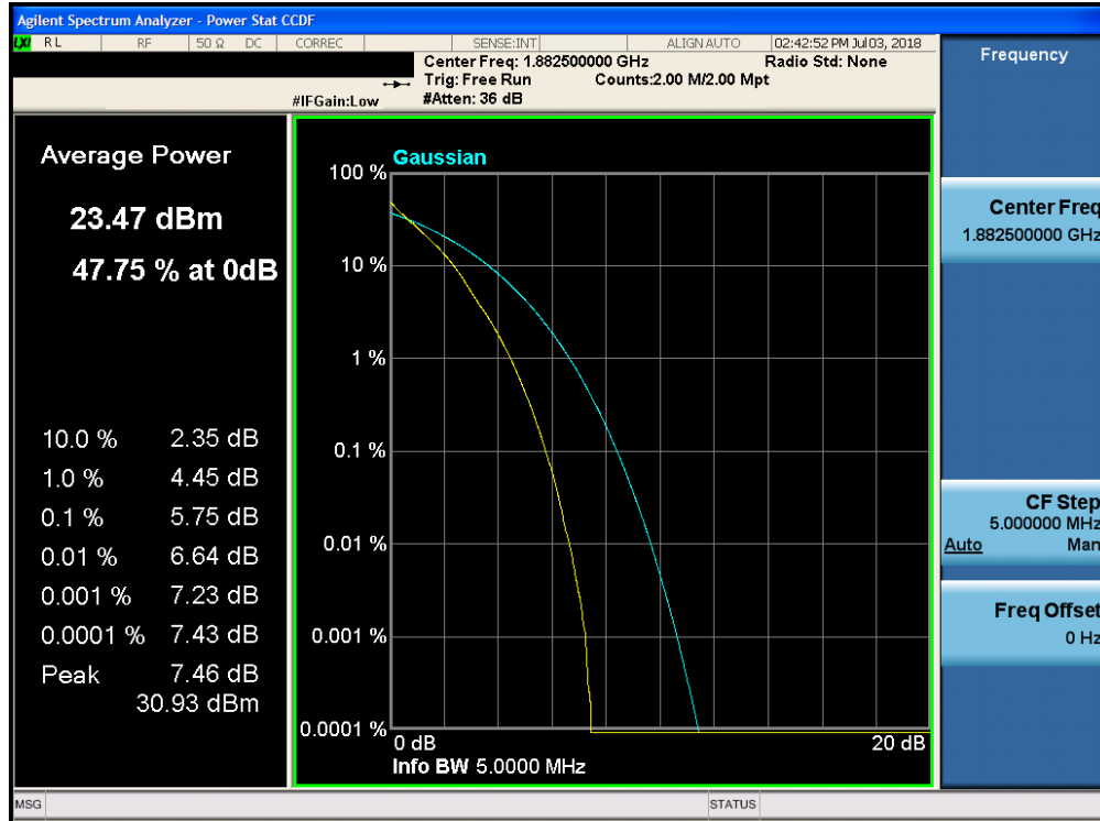
Plot 7-282. PAR Plot (Band 25 - 5.0MHz QPSK - Full RB Configuration)
