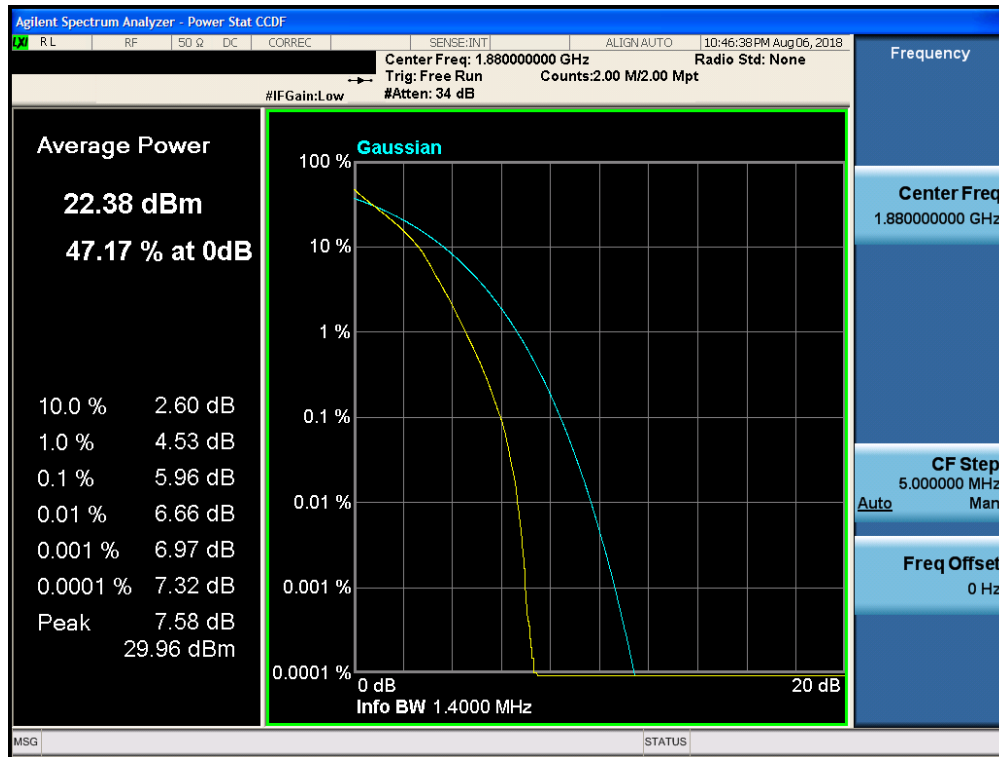
Plot 7-290. PAR Plot (Band 2 - 1.4MHz QPSK - Full RB Configuration)
