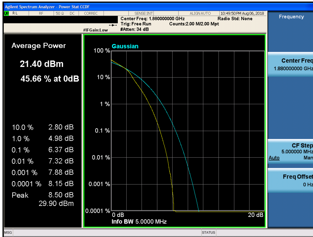
Plot 7-295. PAR Plot (Band 2 - 5.0MHz 16-QAM - Full RB Configuration)
