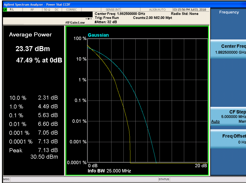
Plot 7-286. PAR Plot (Band 25 - 15.0MHz QPSK - Full RB Configuration)
