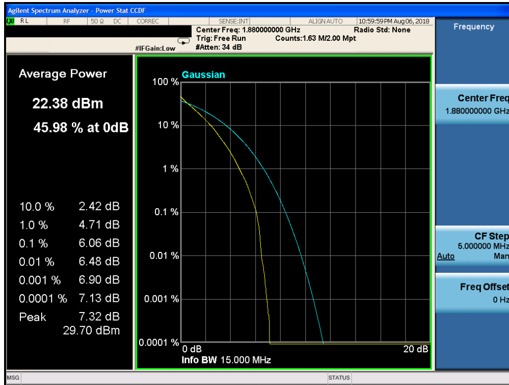
Plot 7-298. PAR Plot (Band 2 - 15.0MHz QPSK - Full RB Configuration)
