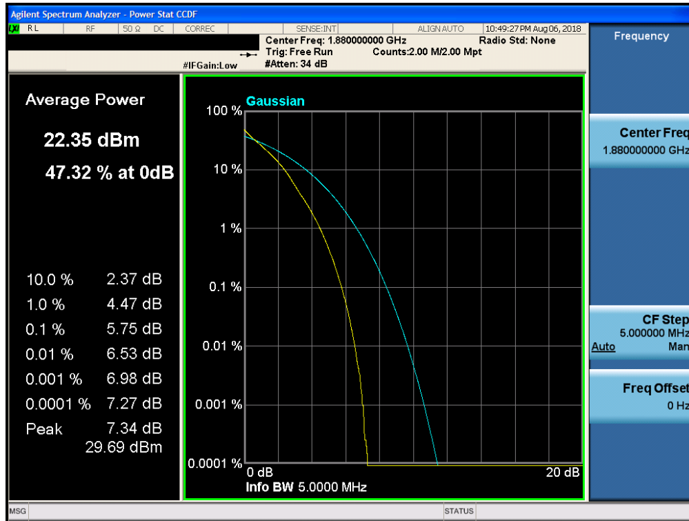
Plot 7-294. PAR Plot (Band 2 - 5.0MHz QPSK - Full RB Configuration)
