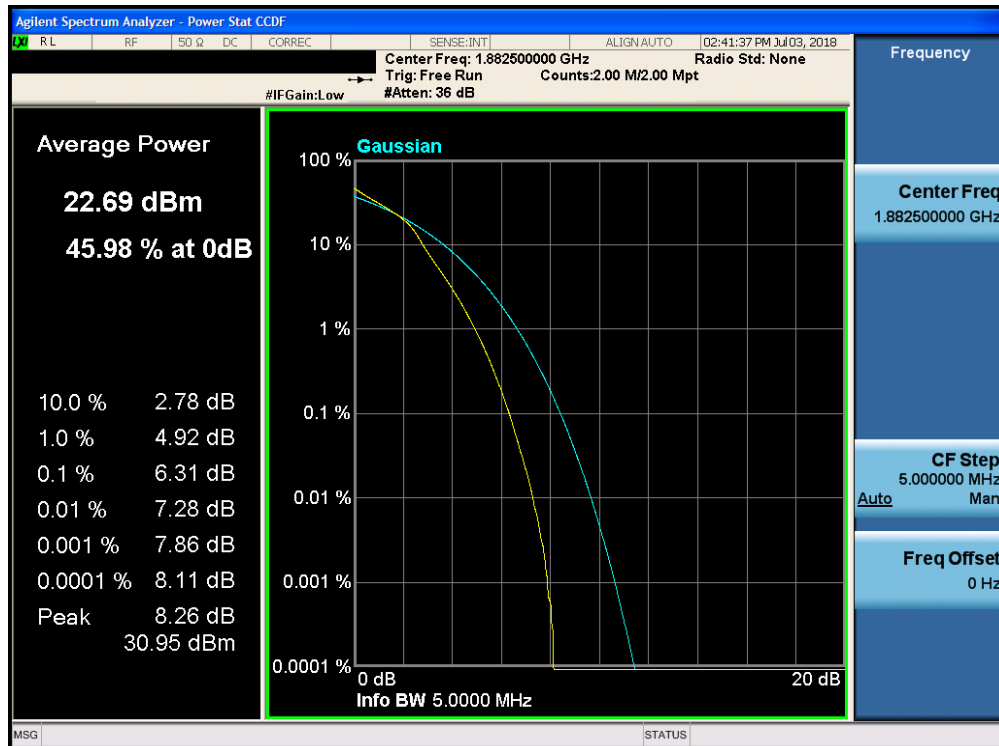
Plot 7-283. PAR Plot (Band 25 - 5.0MHz 16-QAM - Full RB Configuration)
