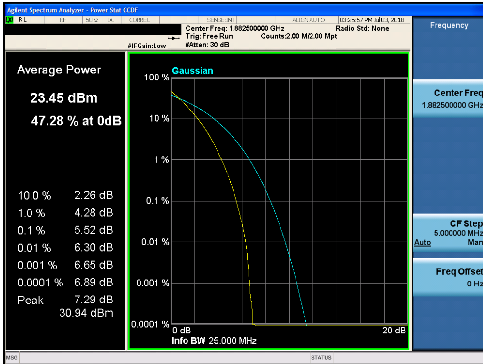
Plot 7-288. PAR Plot (Band 25 - 20.0MHz QPSK - Full RB Configuration)
