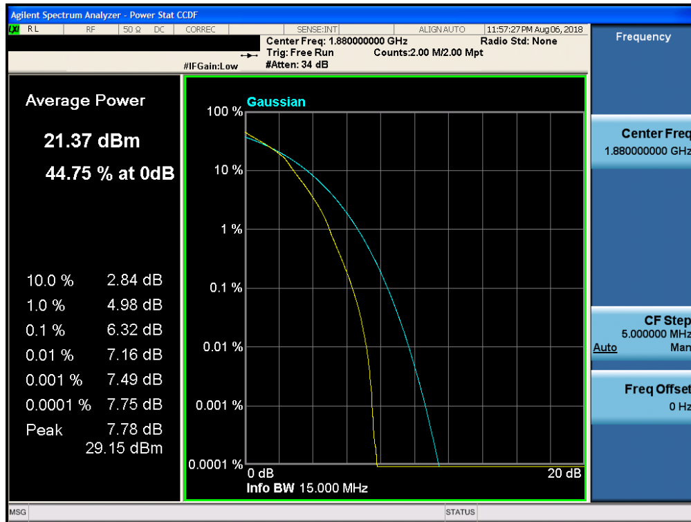
Plot 7-299. PAR Plot (Band 2 - 15.0MHz 16-QAM - Full RB Configuration)
