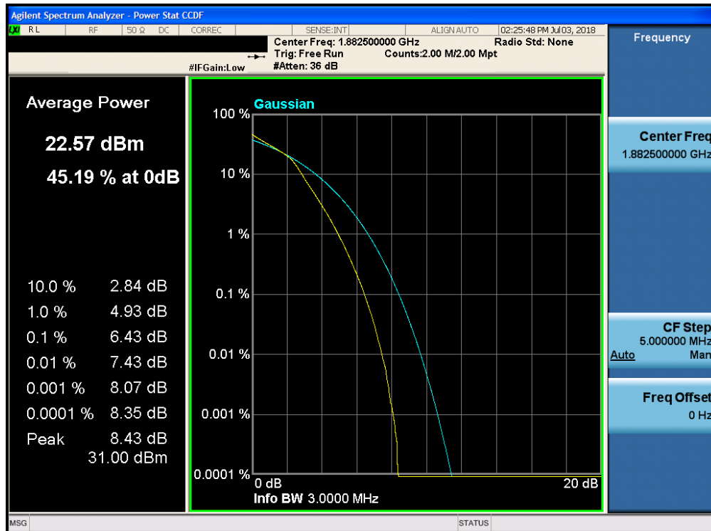
Plot 7-281. PAR Plot (Band 25 - 3.0MHz 16-QAM - Full RB Configuration)
