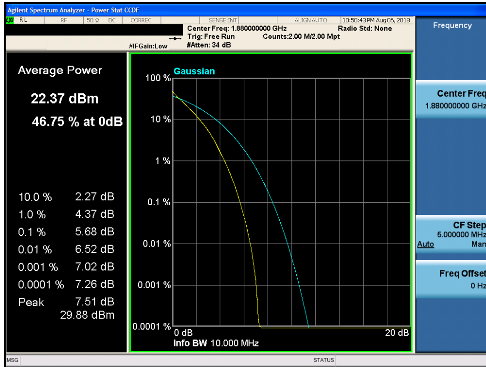
Plot 7-296. PAR Plot (Band 2 - 10.0MHz QPSK - Full RB Configuration)
