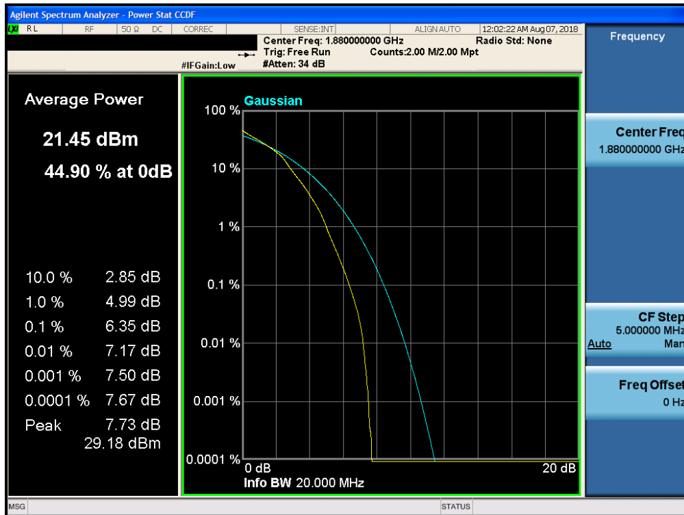
Plot 7-301. PAR Plot (Band 2 - 20.0MHz 16-QAM - Full RB Configuration)
