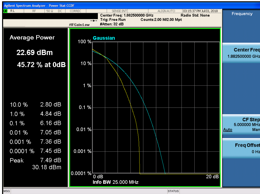
Plot 7-287. PAR Plot (Band 25 - 15.0MHz 16-QAM - Full RB Configuration)
