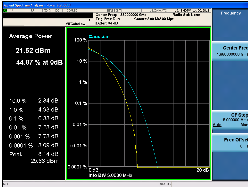
Plot 7-293. PAR Plot (Band 2 - 3.0MHz 16-QAM - Full RB Configuration)
