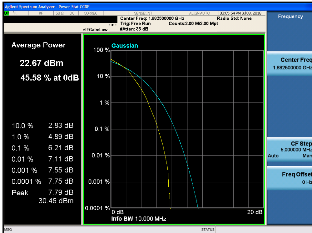
Plot 7-285. PAR Plot (Band 25 - 10.0MHz 16-QAM - Full RB Configuration)
