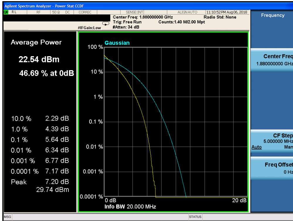
Plot 7-300. PAR Plot (Band 2 - 20.0MHz QPSK - Full RB Configuration)
