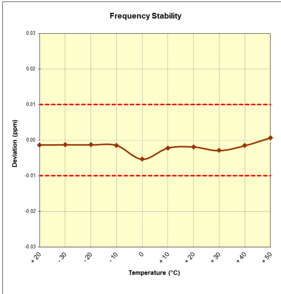
Figure 7-8. Frequency Stability Plot (Reader 100% Ask 1 out of 4)
