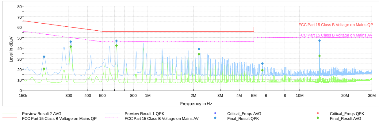
Plot 7-7. Line-Conducted Test Plot (L1, with WCP + AC/DC Adapter)
