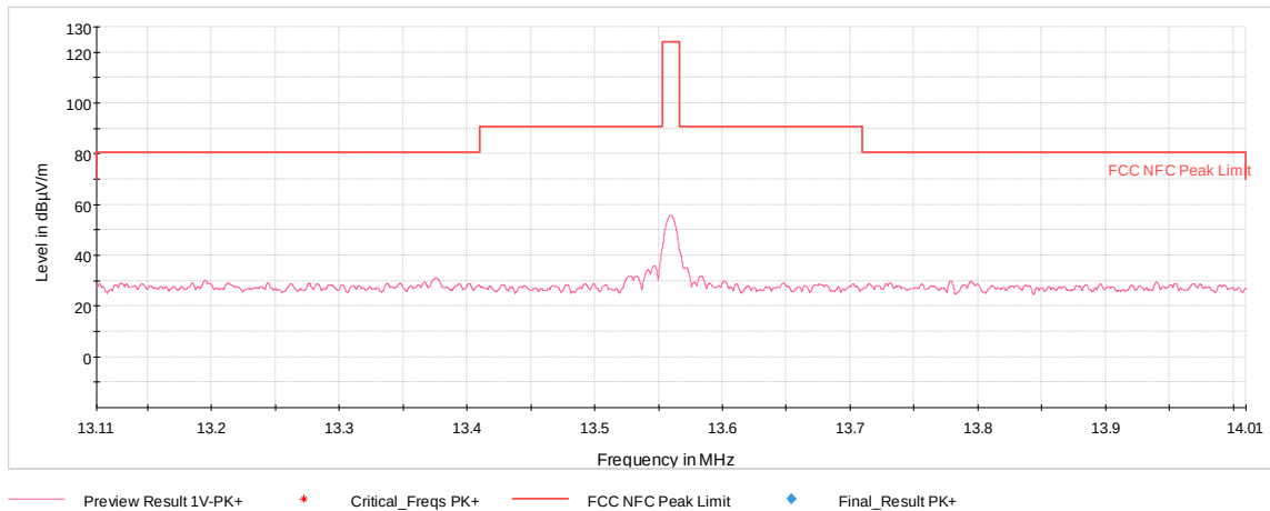
Plot 7-1. In Band Radiated Spurious Plot (CE A 848kbps, Pol. X)
