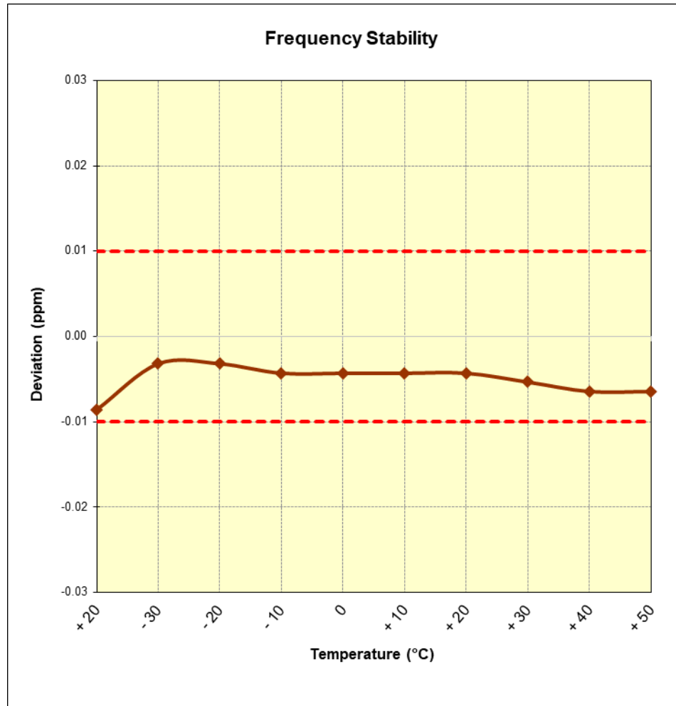
Figure 7-7. Frequency Stability Plot (CE A 848kbps)
