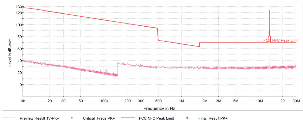
Plot 7-4. Radiated Spurious Plot 9kHz – 30MHz (Reader 100 Ask 1 out of 4, Pol. X)
