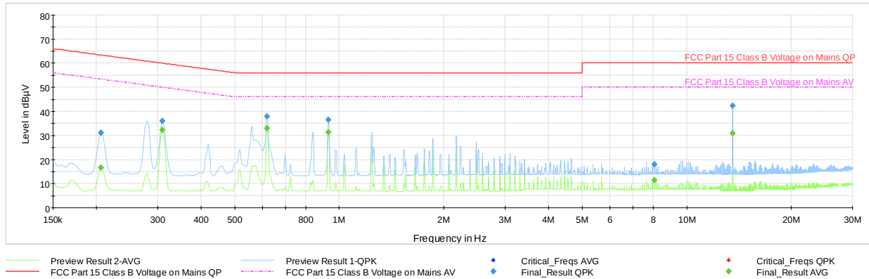
Plot 7-8. Line-Conducted Test Plot (N, with WCP + AC/DC Adapter)
