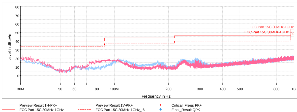
Plot 7-6. Radiated Spurious Plot 30MHz – 1GHz (Reader 100 Ask 1 out of 4, Pol. H & V, with WCP + AC/DC Adapter)
