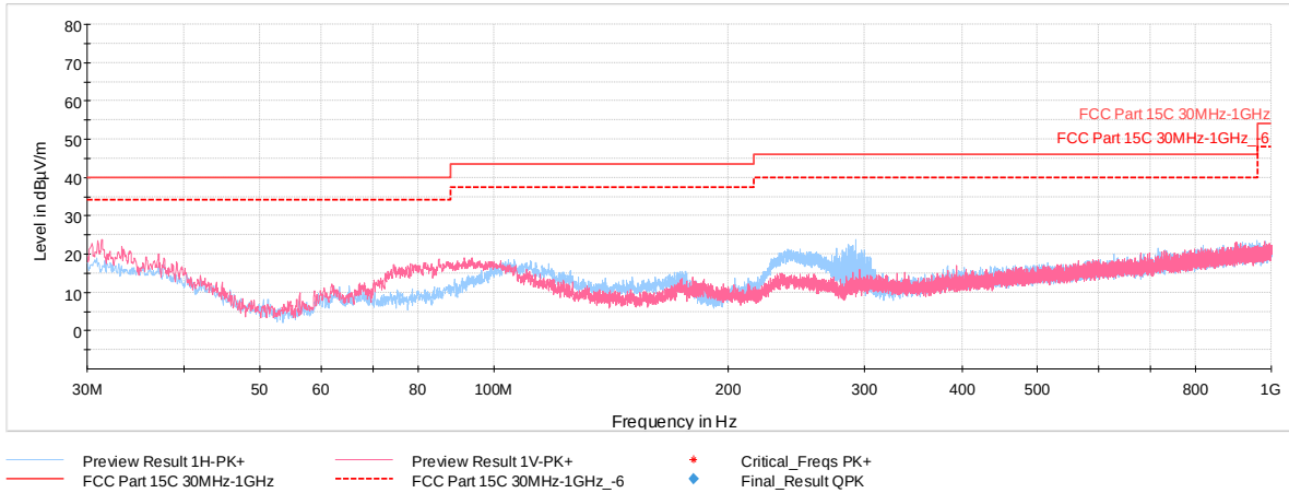
Plot 7-5. Radiated Spurious Plot 30MHz – 1GHz (CE A 848kbps, Pol. H & V, with WCP + AC/DC Adapter)
