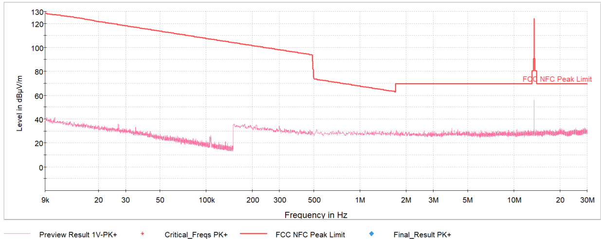
Plot 7-3. Radiated Spurious Plot 9kHz – 30MHz (CE A 848kbps, Pol. X)
