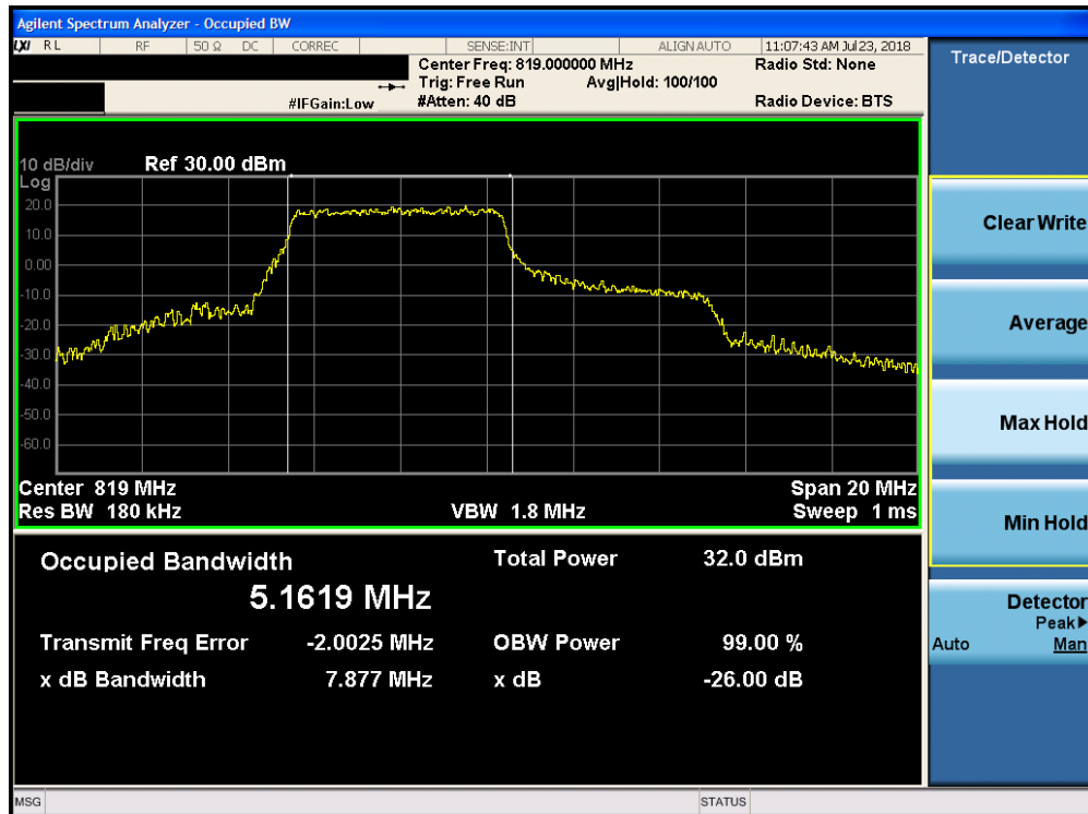
Plot 7-8. Occupied Bandwidth Plot (10MHz 16-QAM – RB Size 27, RB Offset 0 Configuration)
