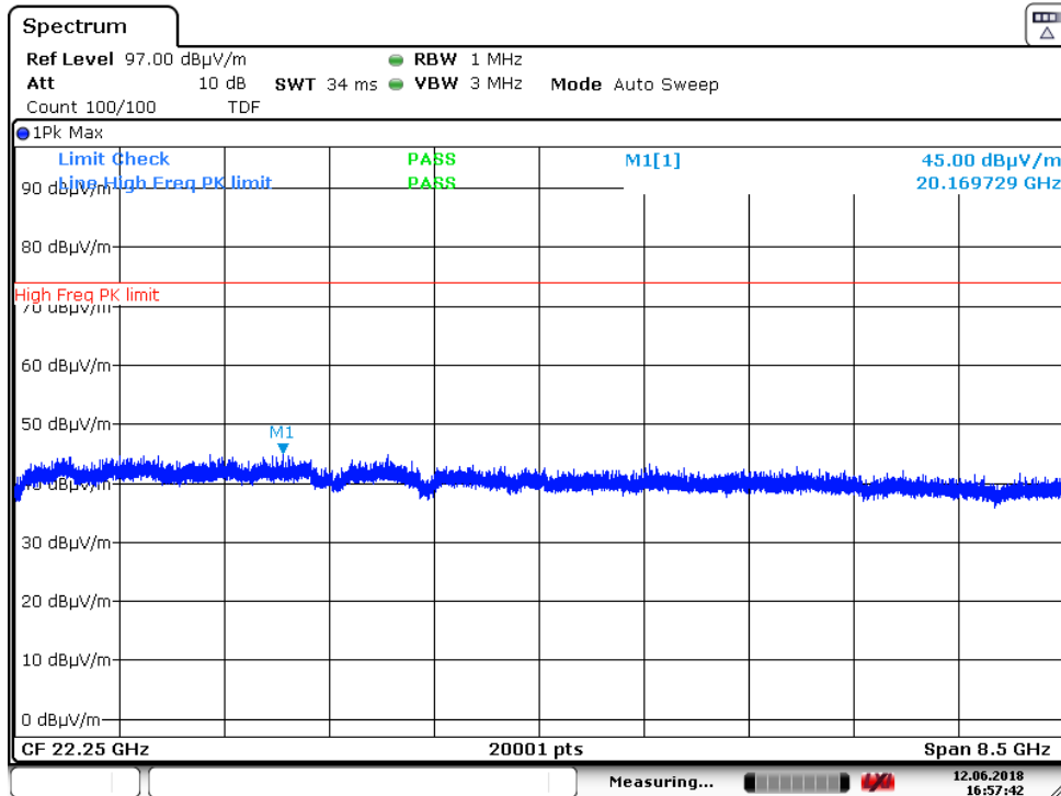
Plot 7-35. Radiated Spurious Plot above 18GHz (802.11b – Ch. 13, Ant. Pol. V)
