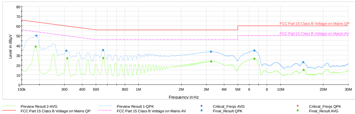
Plot 7-46. Line Conducted Plot with 802.11b (L1, with WCP + Laptop)
