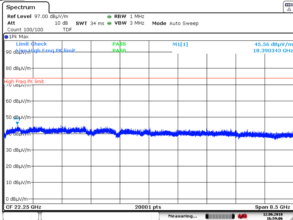
Plot 7-34. Radiated Spurious Plot above 18GHz (802.11b – Ch. 13, Ant. Pol. H)
