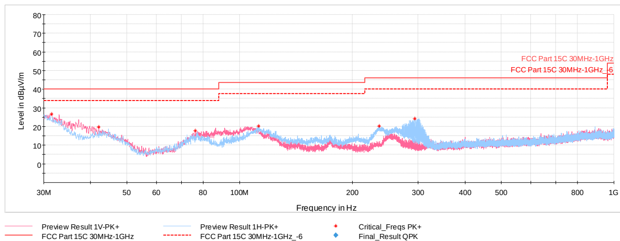
Plot 7-45. Radiated Spurious Plot below 1GHz (802.11b, with WCP + AC/DC Adapter)
