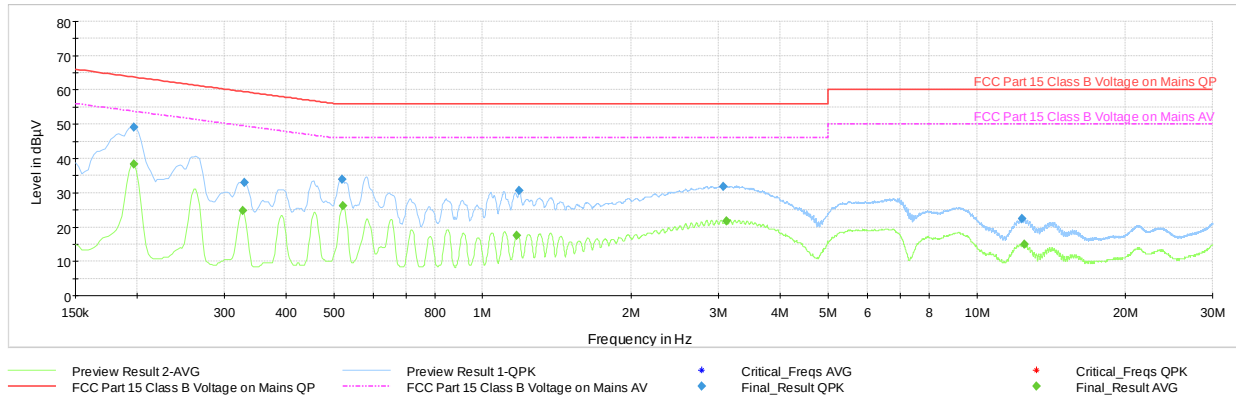
Plot 7-47. Line Conducted Plot with 802.11b (N, with WCP + Laptop)
