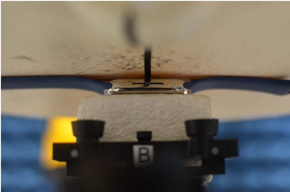
SAR Test Setup Photo 10: Stainless Steel with Sport wristband, Back side at 0.0 cm
