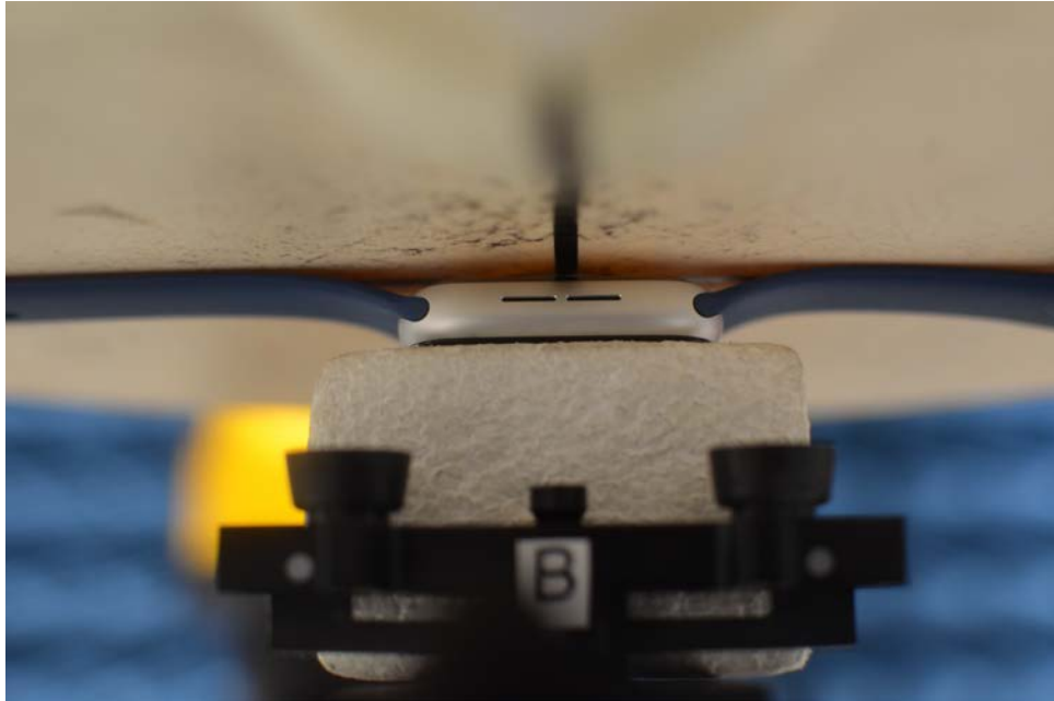
SAR Test Setup Photo 7: Aluminum with Sport wristband, Back side at 0.0 cm
