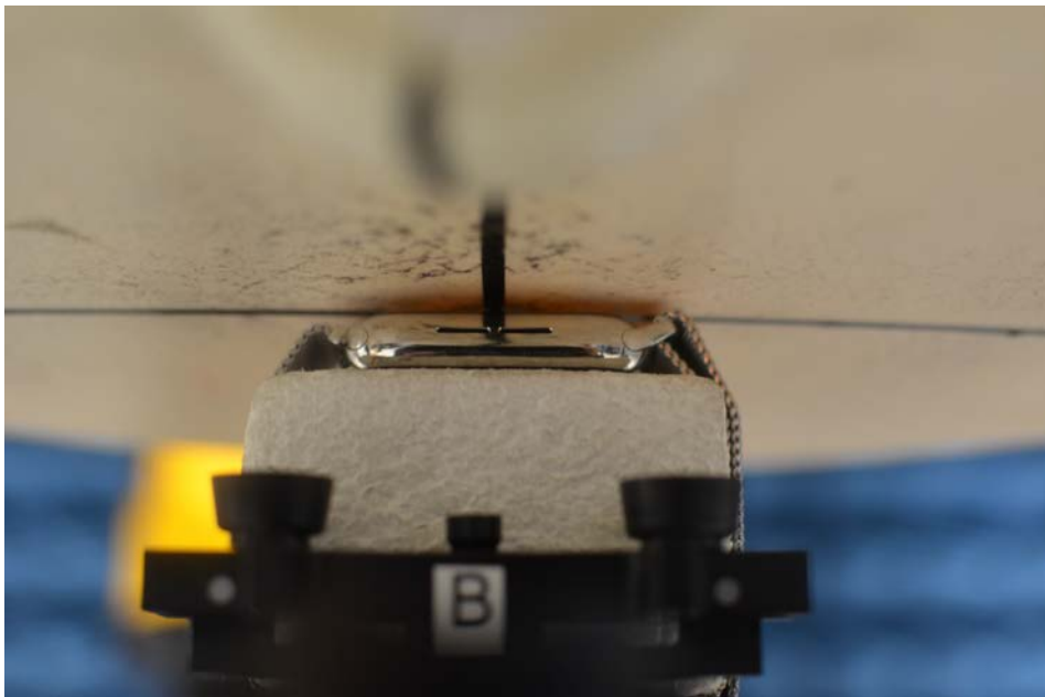
SAR Test Setup Photo 12: Stainless Steel with Metal Loop wristband, Back side at 0.0 cm
