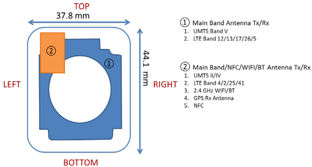
Figure F-1 DUT Antenna Locations
