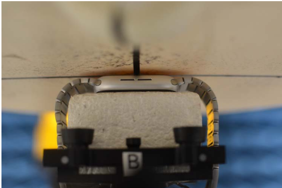
SAR Test Setup Photo 8: Aluminum with Metal Links wristband, Back side at 0.0 cm
