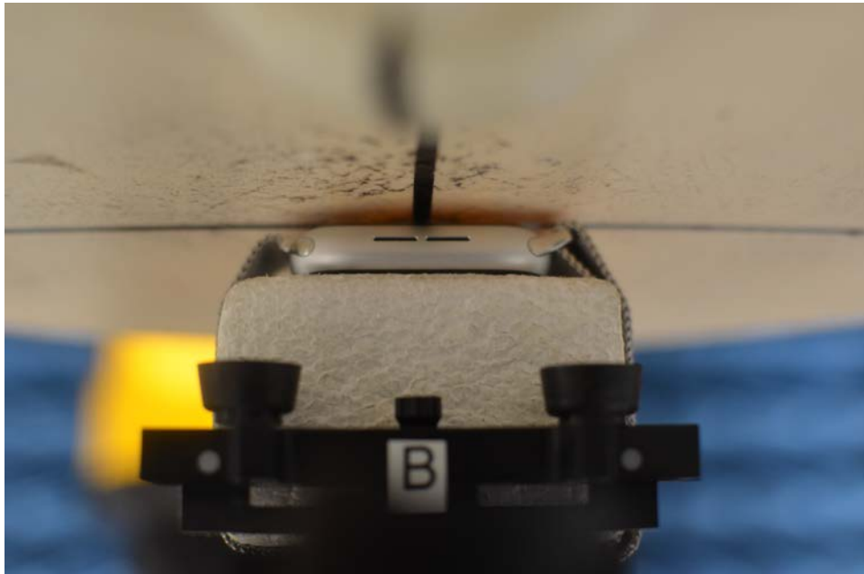
SAR Test Setup Photo 9: Aluminum with Metal Loop wristband, Back side at 0.0 cm
