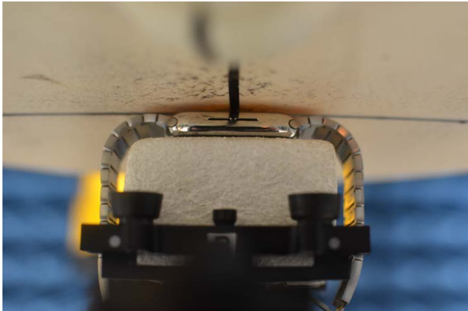
SAR Test Setup Photo 11: Stainless Steel with Metal Links wristband, Back side at 0.0 cm
