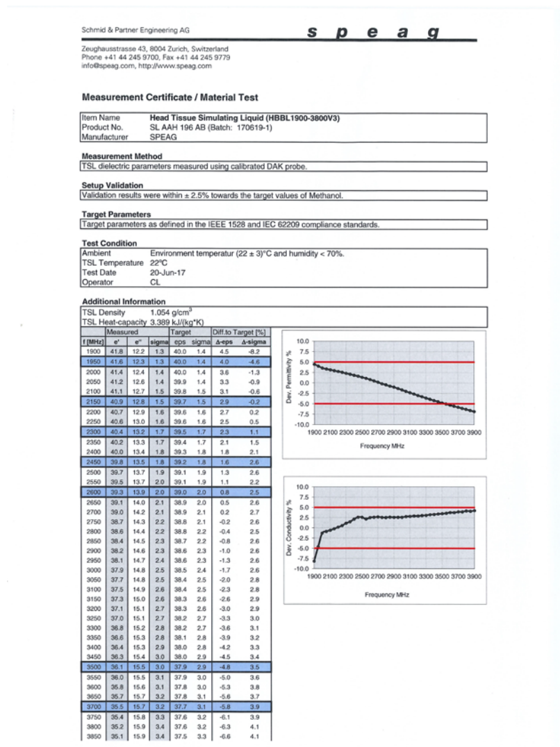
Figure D-2 2.45 GHz Head Tissue Equivalent Matter
