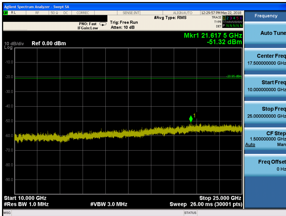
Plot 7-30. Conducted Spurious Plot (Bluetooth (HDR), 4Mbps, ePA – Ch. 38)
