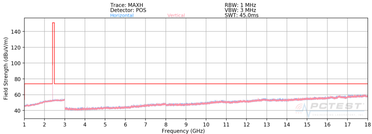
Plot 7-39. Radiated Spurious Plot above 1GHz (4Mbps, ePA – Ch.1, Ant. Pol. H & V)
