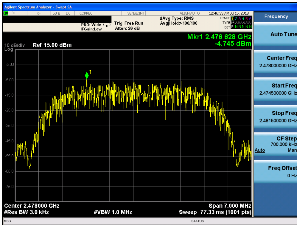
Plot 7-18. Power Spectral Density Plot (Bluetooth (HDR), 8Mbps, iPA – Ch. 75)
