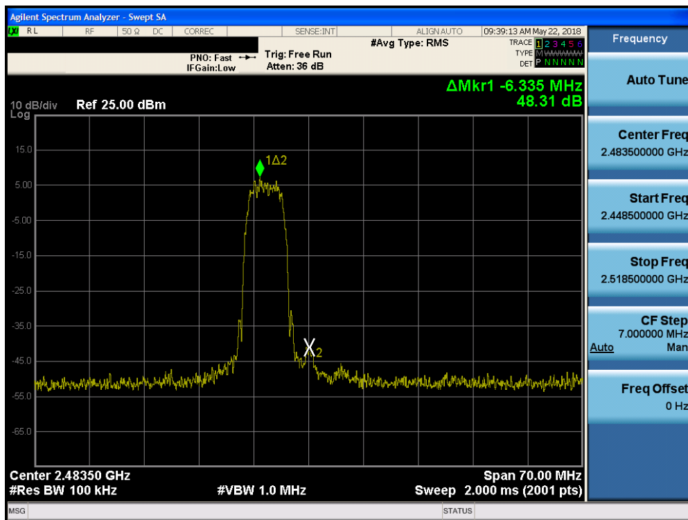
Plot 7-24. Band Edge Plot (Bluetooth (HDR), 8Mbps, ePA – Ch. 75)
