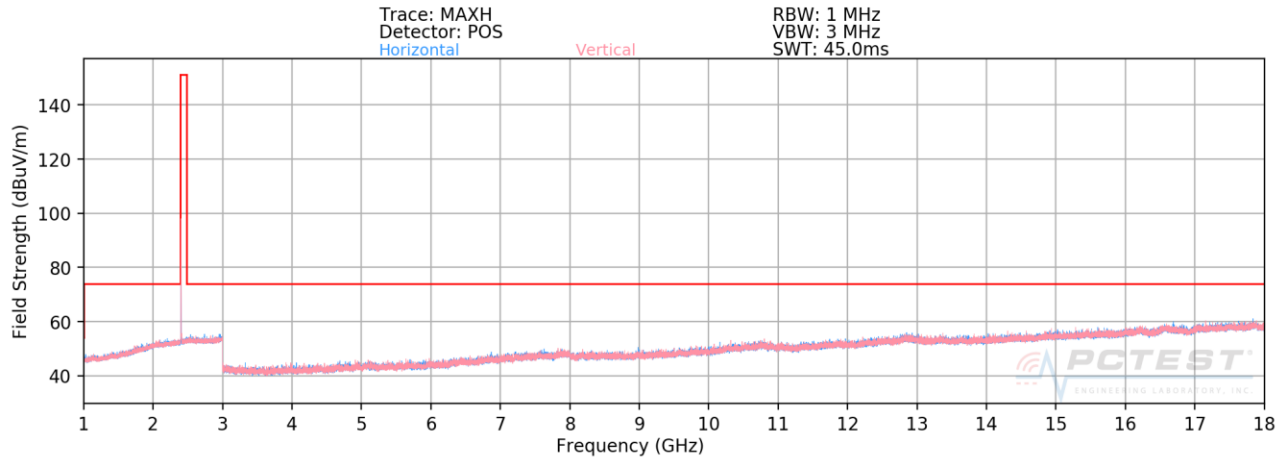
Plot 7-42. Radiated Spurious Plot above 1GHz (8Mbps, ePA – Ch.1, Ant. Pol. H & V)
