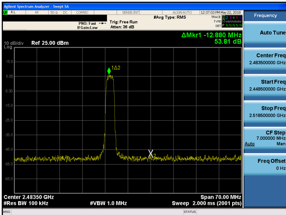
Plot 7-22. Band Edge Plot (Bluetooth (HDR), 4Mbps, iPA – Ch. 75)
