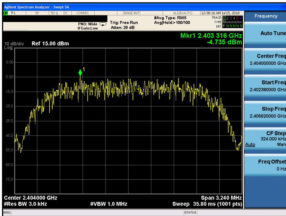
Plot 7-7. Power Spectral Density Plot (Bluetooth (HDR), 4Mbps, ePA – Ch. 1)
