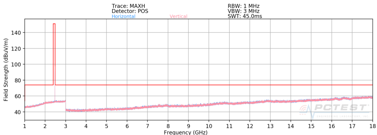
Plot 7-41. Radiated Spurious Plot above 1GHz (4Mbps, ePA – Ch.75, Ant. Pol. H & V)
