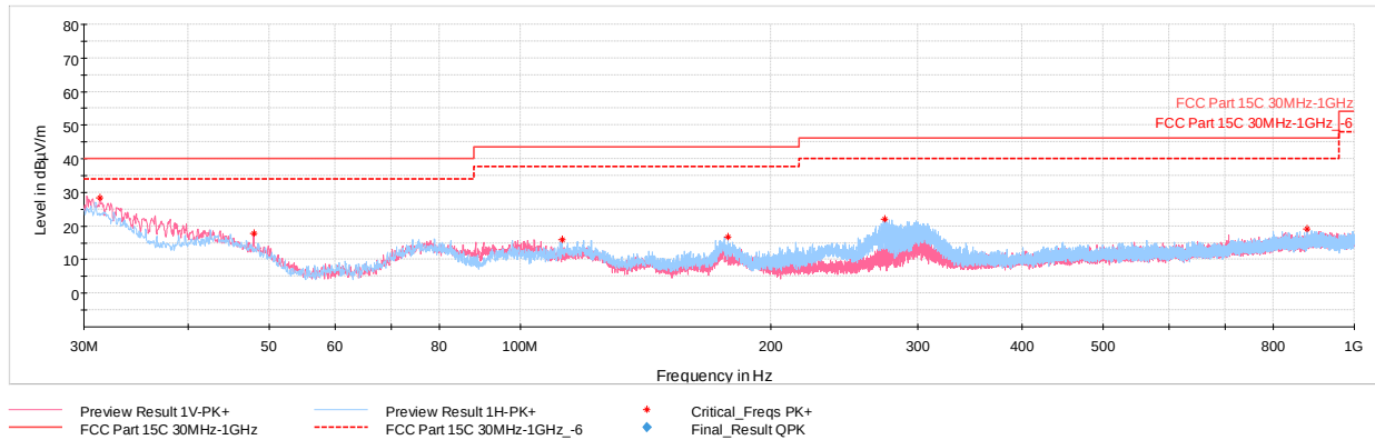
Plot 7-51. Radiated Spurious Plot below 1GHz (4Mbps, ePA, Pol. H & V, with WCP + AC/DC Adapter attached)
