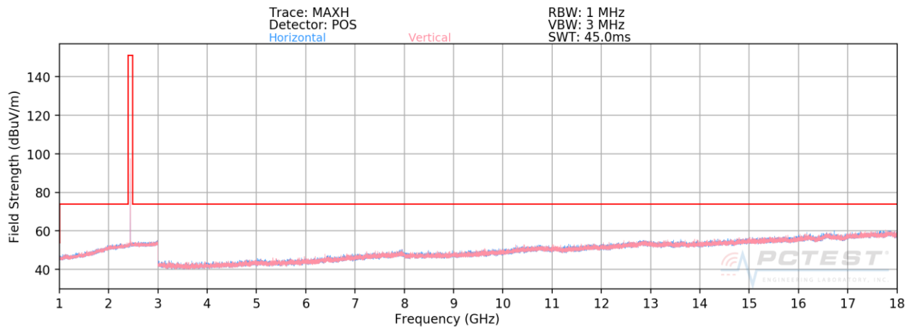
Plot 7-43. Radiated Spurious Plot above 1GHz (8Mbps, ePA – Ch.38, Ant. Pol. H & V)
