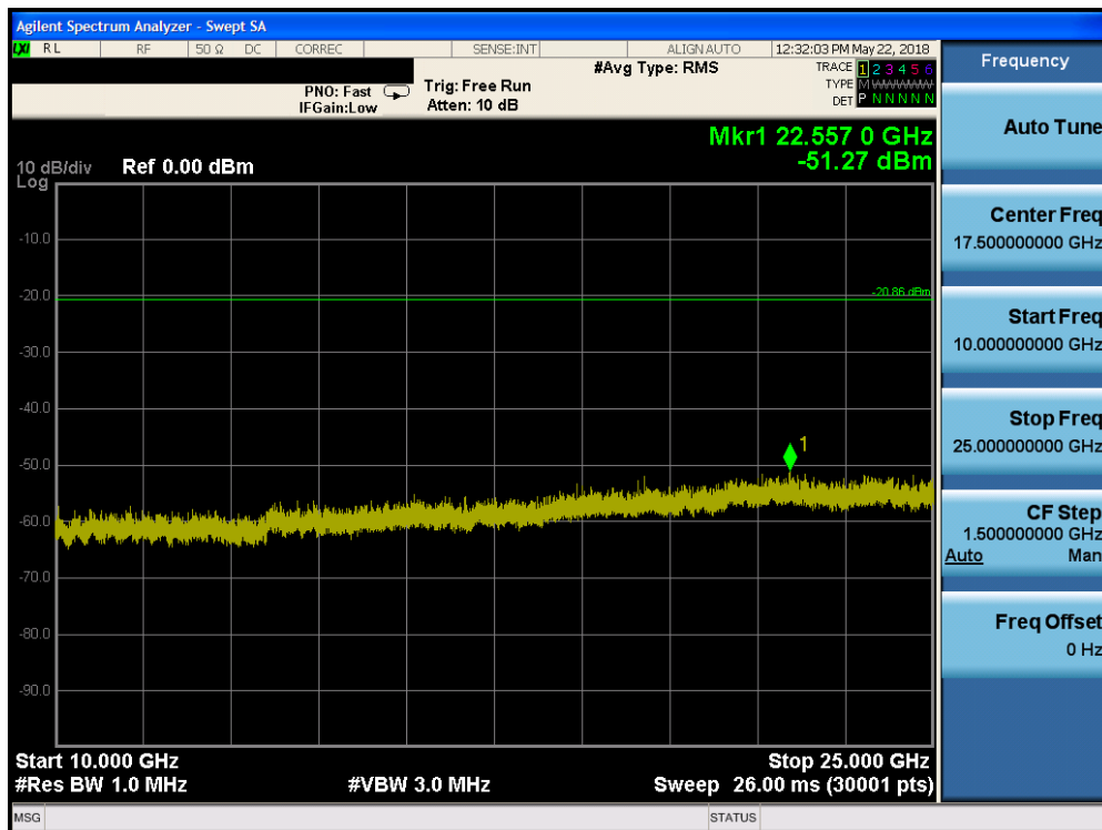
Plot 7-32. Conducted Spurious Plot (Bluetooth (HDR), 4Mbps, ePA – Ch. 75)
