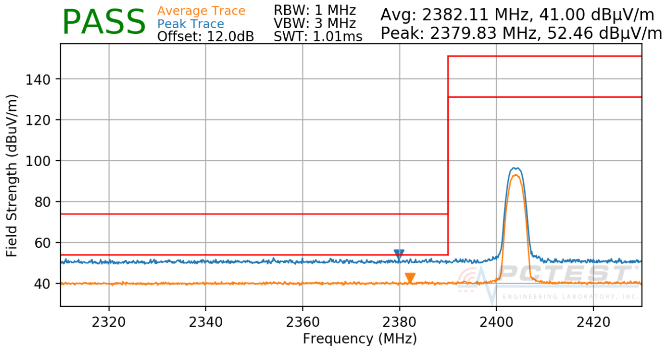
Plot 7-47. Radiated Restricted Lower Band Edge Measurement (Average & Peak)
