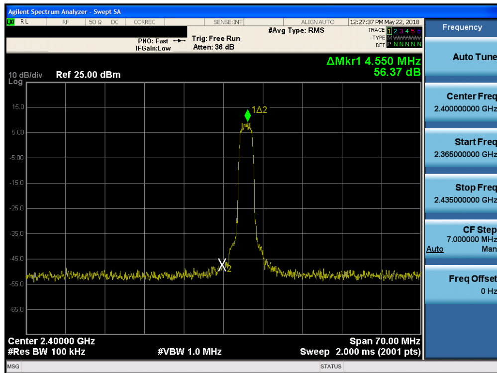
Plot 7-19. Band Edge Plot (Bluetooth (HDR), 4Mbps, ePA – Ch. 1)
