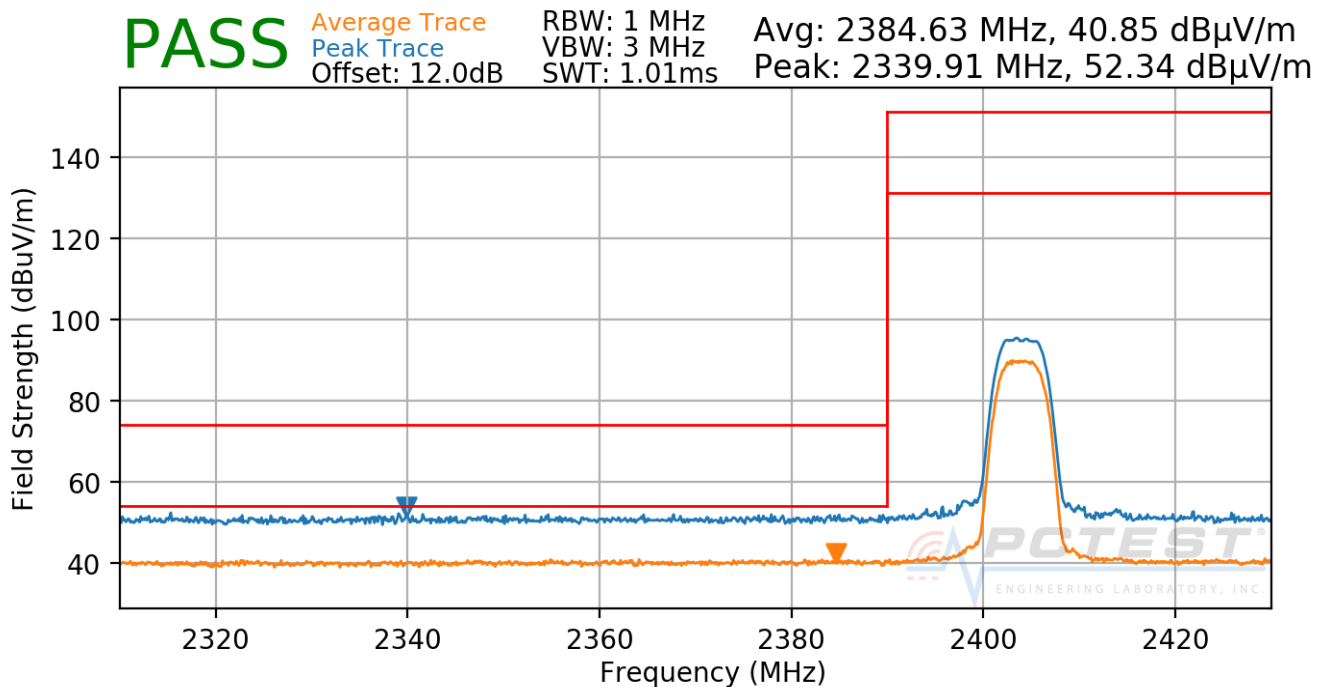
Plot 7-48. Radiated Restricted Lower Band Edge Measurement (Average & Peak)
