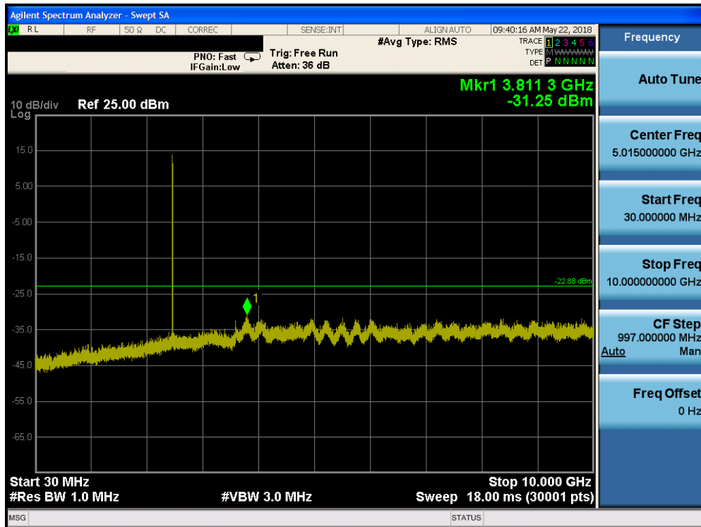
Plot 7-37. Conducted Spurious Plot (Bluetooth (HDR), 8Mbps, ePA – Ch. 75)
