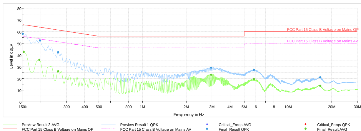
Plot 7-53. Line Conducted Plot with Bluetooth HDR (L1, with WCP + Laptop attached)
