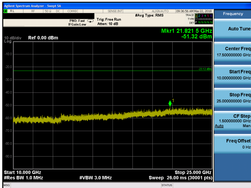
Plot 7-36. Conducted Spurious Plot (Bluetooth (HDR), 8Mbps, ePA – Ch. 38)
