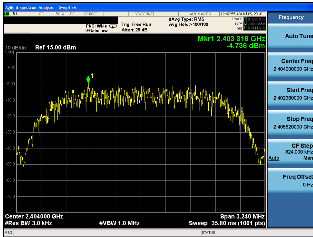
Plot 7-10. Power Spectral Density Plot (Bluetooth (HDR), 4Mbps, iPA – Ch. 1)
