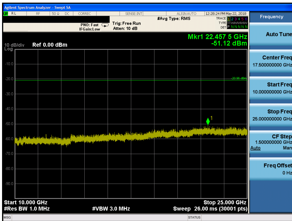
Plot 7-28. Conducted Spurious Plot (Bluetooth (HDR), 4Mbps, ePA – Ch. 1)
