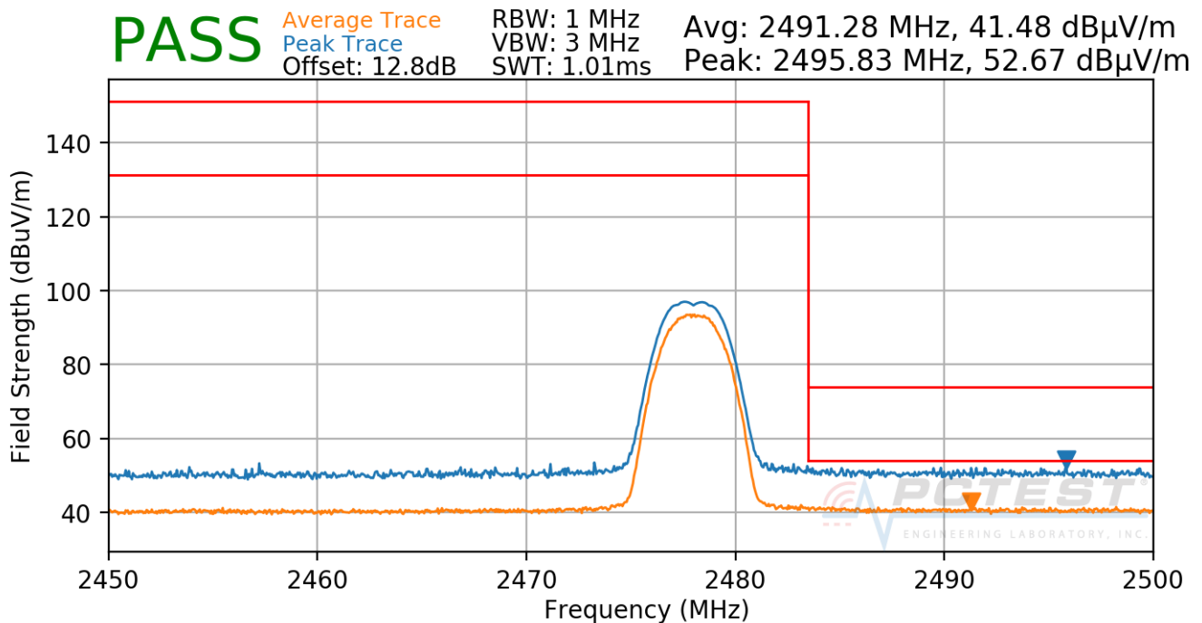
Plot 7-49. Radiated Restricted Upper Band Edge Measurement (Average & Peak)
