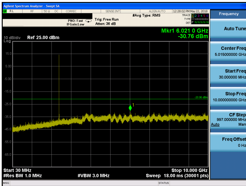
Plot 7-27. Conducted Spurious Plot (Bluetooth (HDR), 4Mbps, ePA – Ch. 1)
