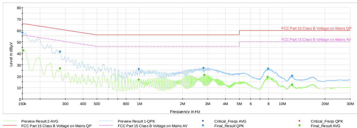
Plot 7-54. Line Conducted Plot with Bluetooth HDR (N, with WCP + Laptop attached)
