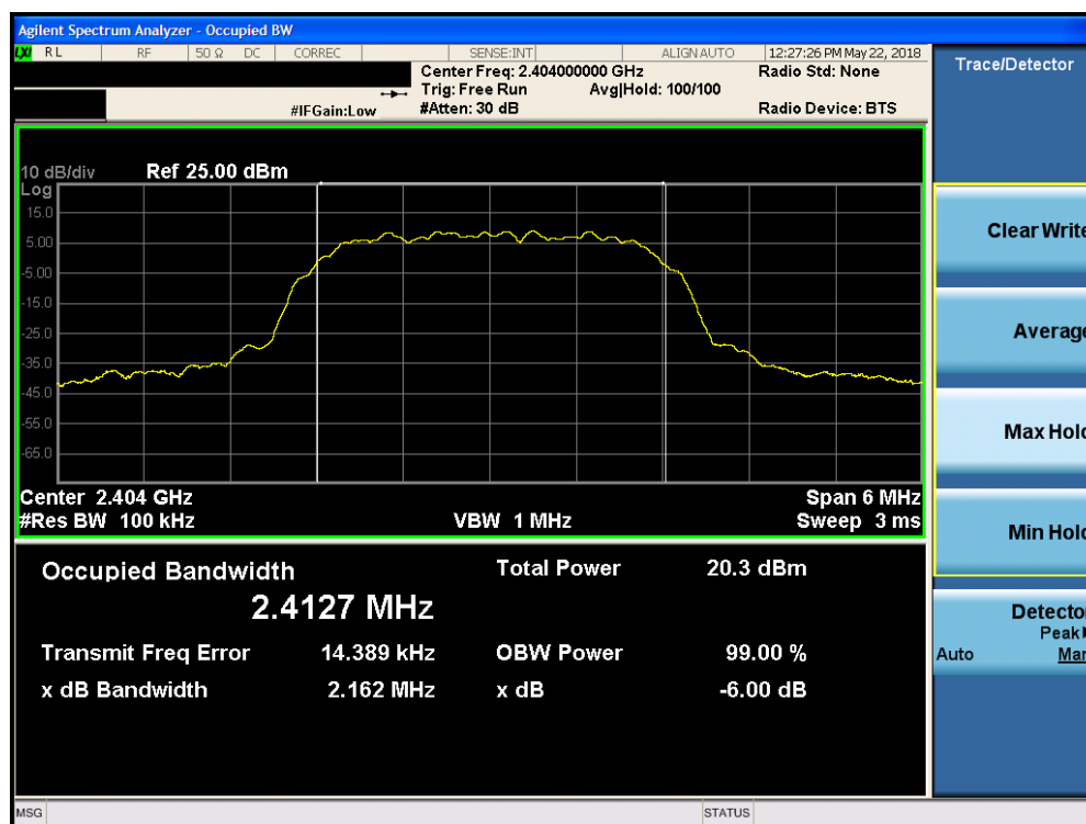
Plot 7-1. 6dB Bandwidth Plot (Bluetooth (HDR), 4Mbps, ePA – Ch. 1)
