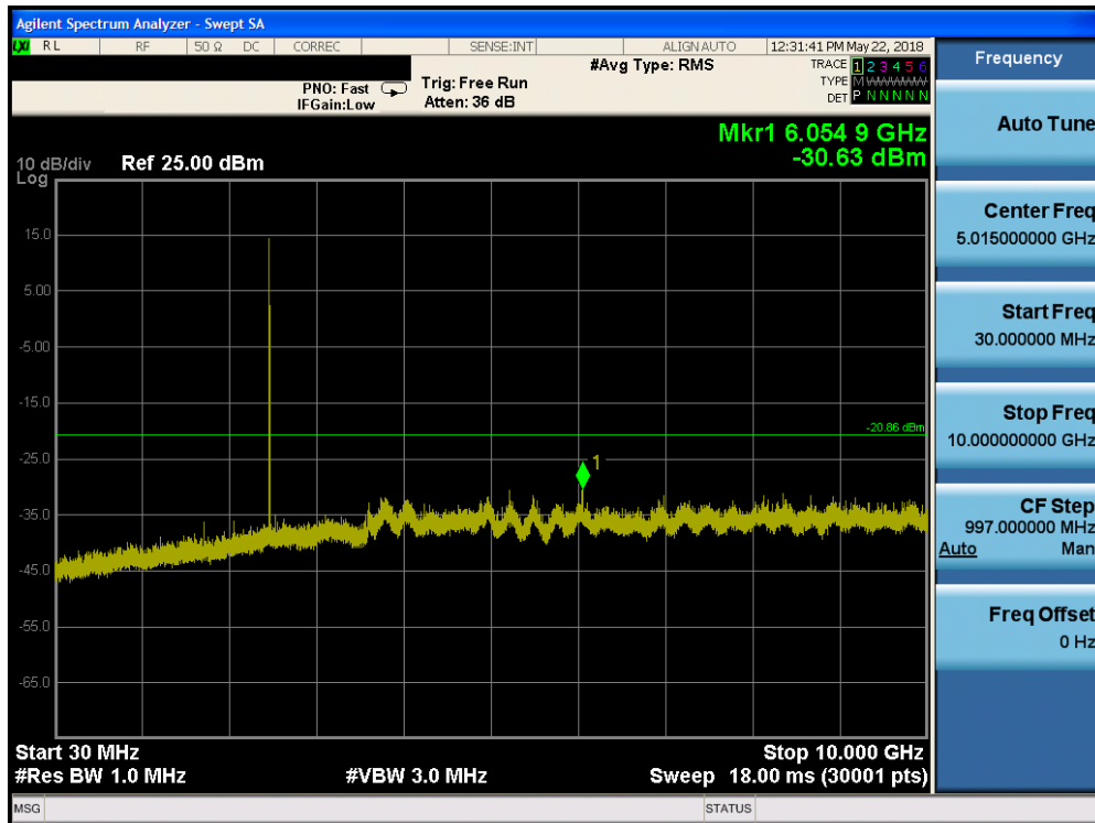
Plot 7-31. Conducted Spurious Plot (Bluetooth (HDR), 4Mbps, ePA – Ch. 75)
