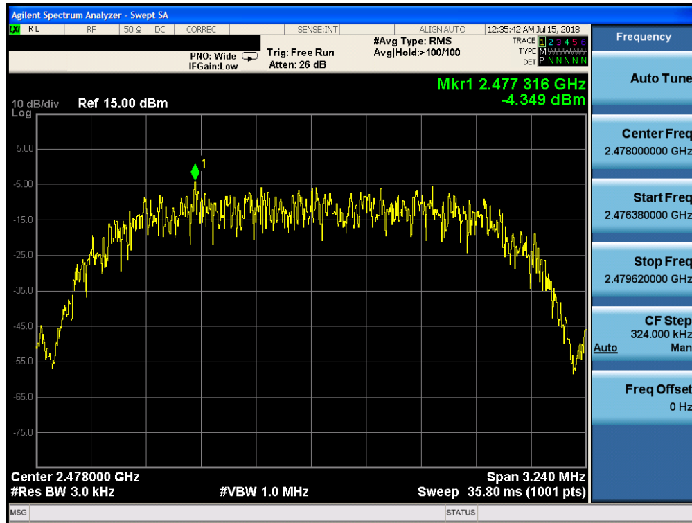
Plot 7-9. Power Spectral Density Plot (Bluetooth (HDR), 4Mbps, ePA – Ch. 75)
