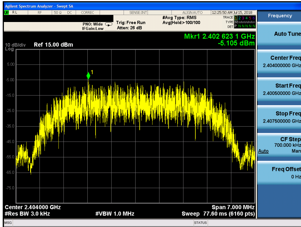
Plot 7-13. Power Spectral Density Plot (Bluetooth (HDR), 8Mbps, ePA – Ch. 1)
