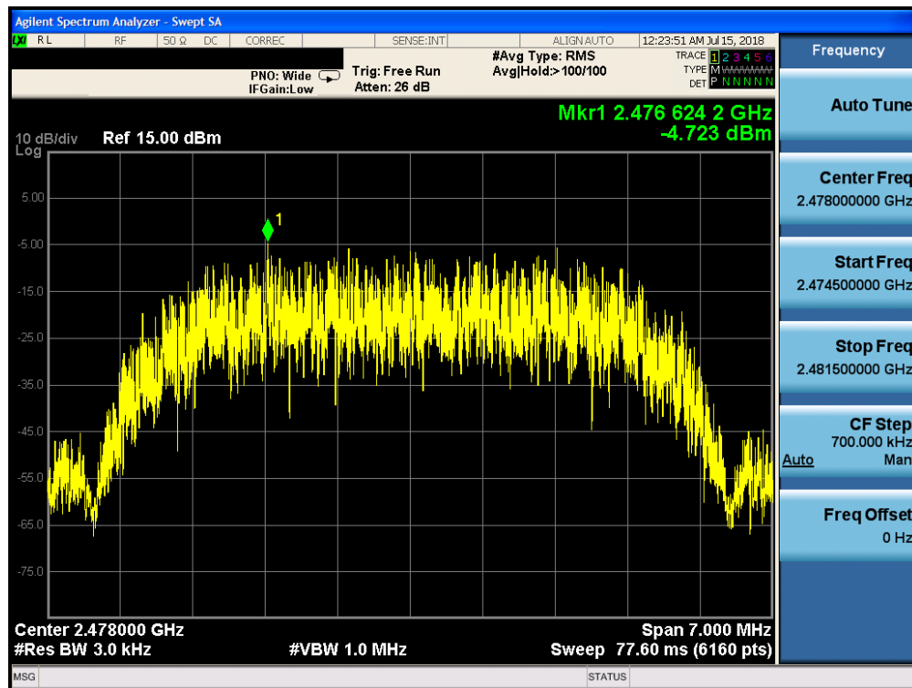
Plot 7-15. Power Spectral Density Plot (Bluetooth (HDR), 8Mbps, ePA – Ch. 75)
