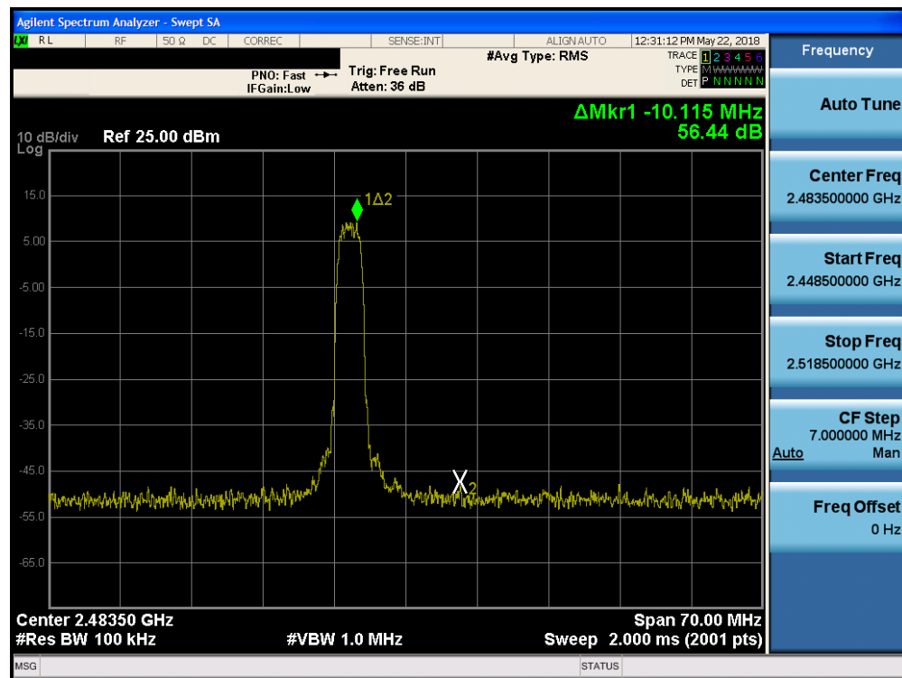
Plot 7-20. Band Edge Plot (Bluetooth (HDR), 4Mbps, ePA – Ch. 75)
