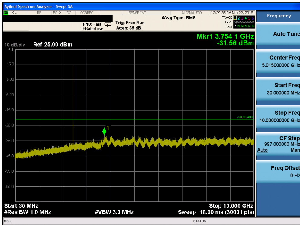
Plot 7-29. Conducted Spurious Plot (Bluetooth (HDR), 4Mbps, ePA – Ch. 38)
