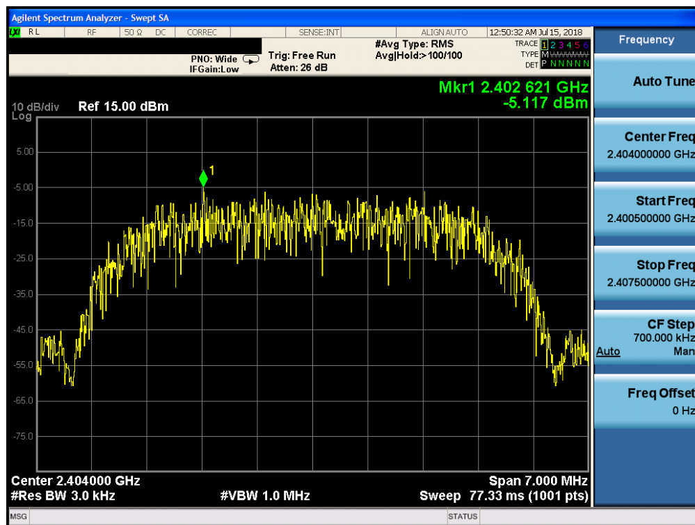
Plot 7-16. Power Spectral Density Plot (Bluetooth (HDR), 8Mbps, iPA – Ch. 1)
