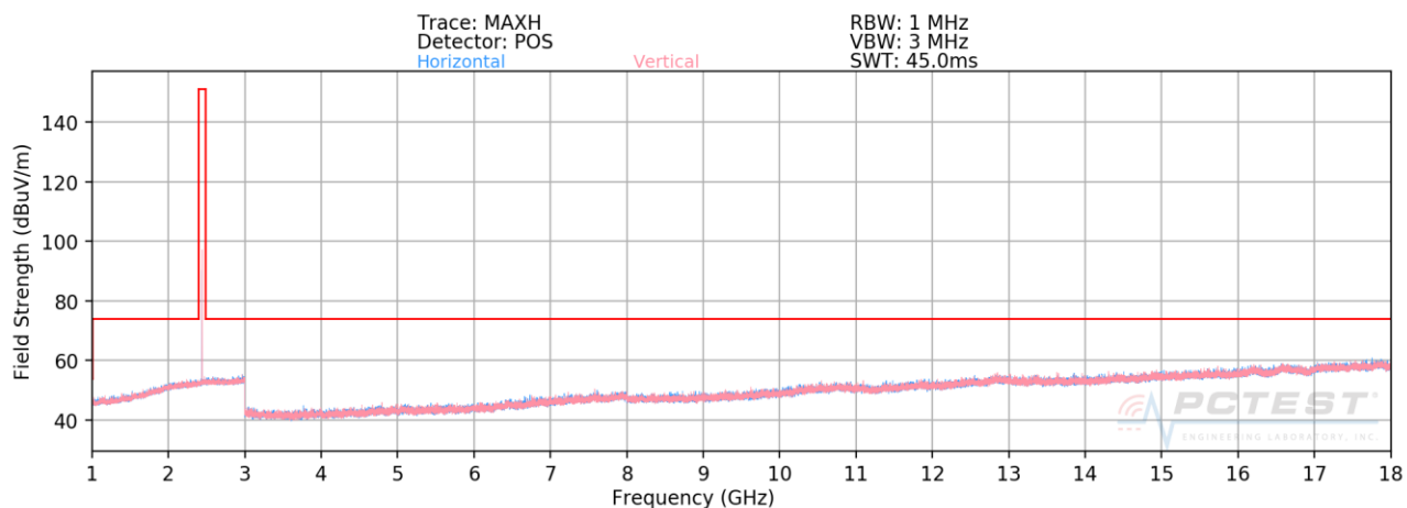
Plot 7-40. Radiated Spurious Plot above 1GHz (4Mbps, ePA – Ch.38, Ant. Pol. H & V)
