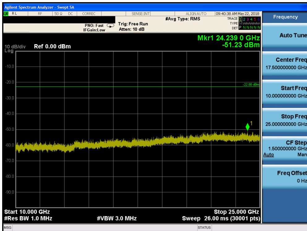
Plot 7-38. Conducted Spurious Plot (Bluetooth (HDR), 8Mbps, ePA – Ch. 75)
