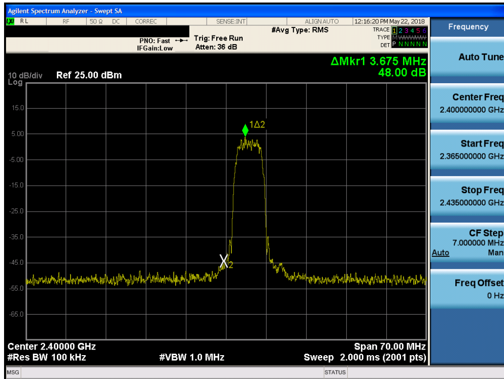
Plot 7-25. Band Edge Plot (Bluetooth (HDR), 8Mbps, iPA – Ch. 1)
