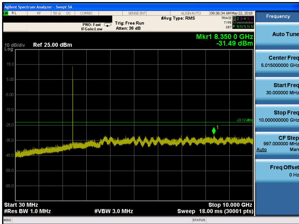
Plot 7-35. Conducted Spurious Plot (Bluetooth (HDR), 8Mbps, ePA – Ch. 38)
