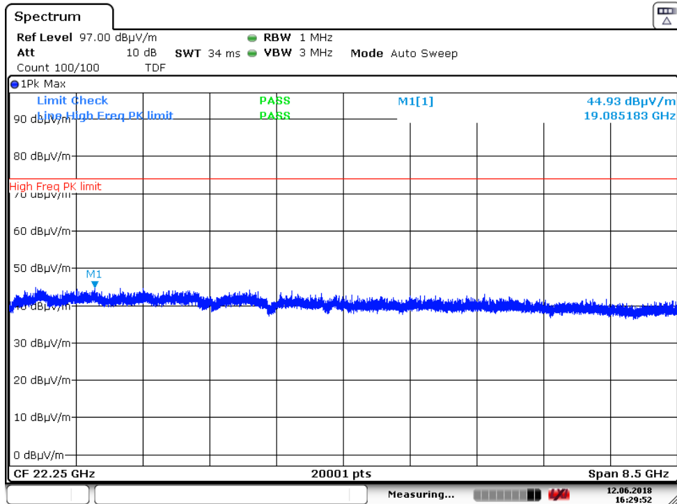
Plot 7-45. Radiated Spurious Plot above 1GHz (8Mbps, ePA, Ant. Pol. H)
