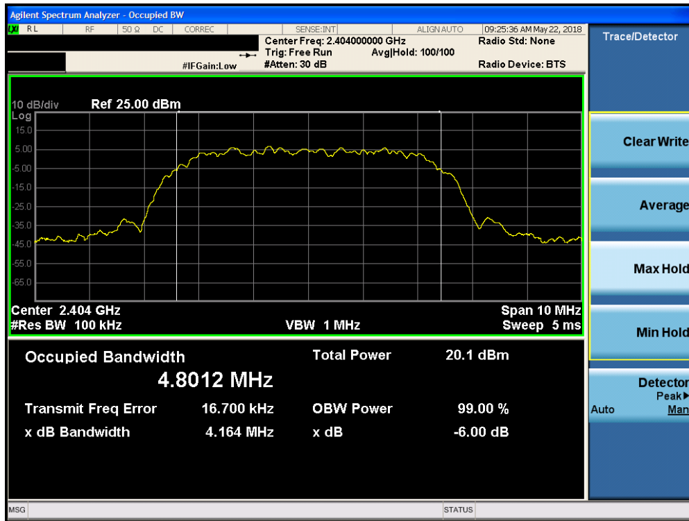
Plot 7-4. 6dB Bandwidth Plot (Bluetooth (HDR), 8Mbps, ePA – Ch. 1)
