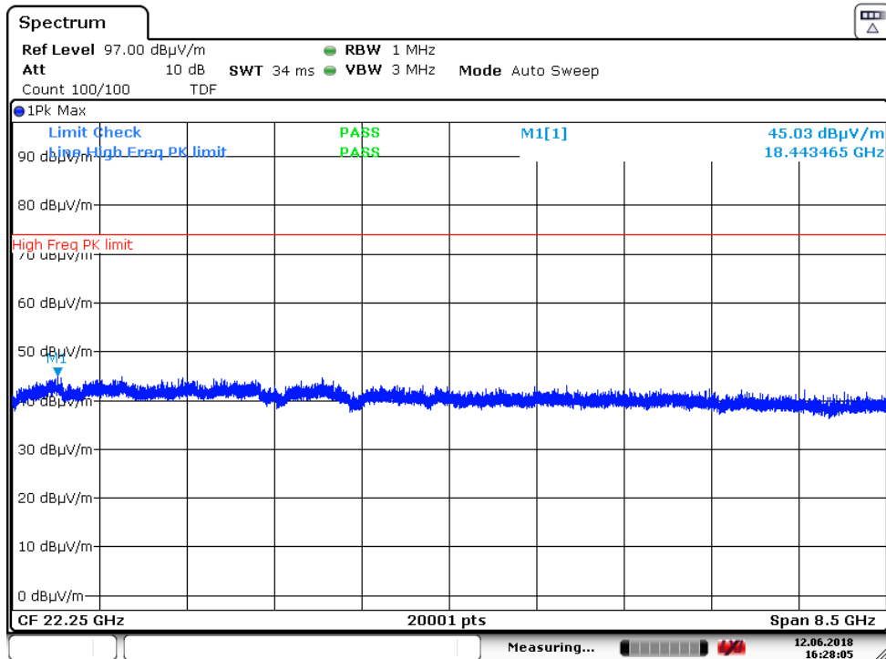
Plot 7-46. Radiated Spurious Plot above 1GHz (8Mbps, ePA, Ant. Pol. V)
