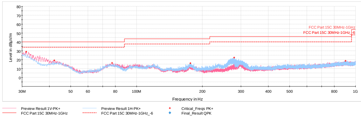
Plot 7-52. Radiated Spurious Plot below 1GHz (8Mbps, ePA, Pol. H & V, with WCP + AC/DC Adapter attached)
