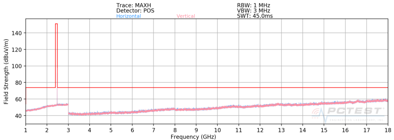
Plot 7-44. Radiated Spurious Plot above 1GHz (8Mbps, ePA – Ch.75, Ant. Pol. H & V)
