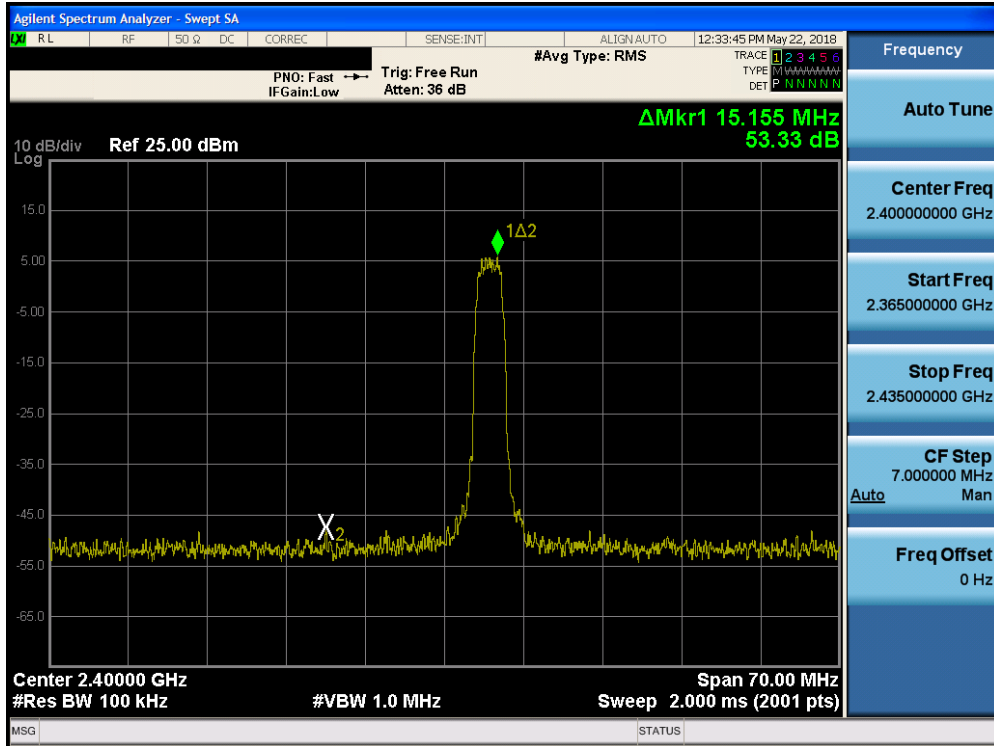
Plot 7-21. Band Edge Plot (Bluetooth (HDR), 4Mbps, iPA – Ch. 1)
