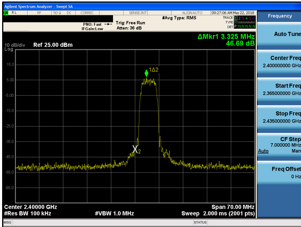
Plot 7-23. Band Edge Plot (Bluetooth (HDR), 8Mbps, ePA – Ch. 1)
