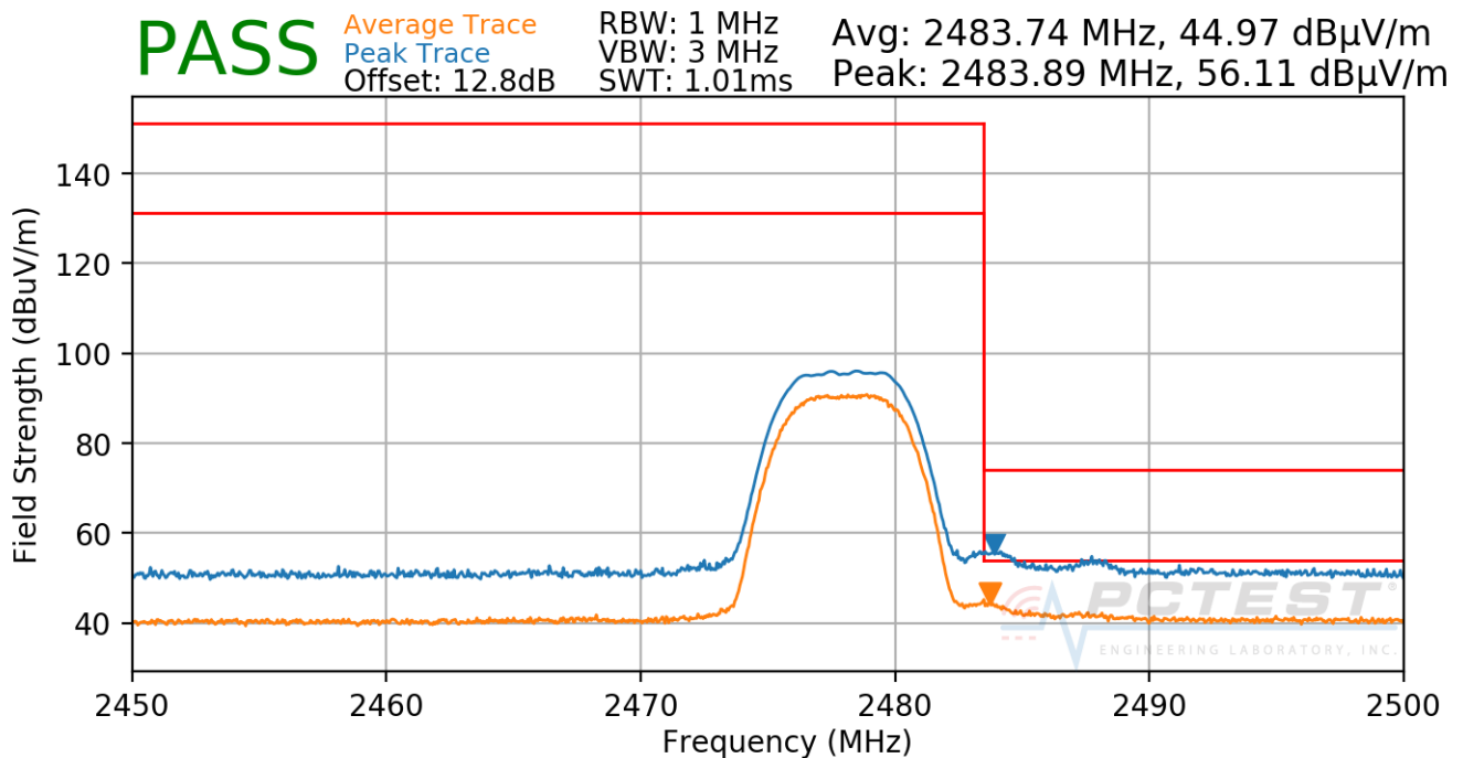
Plot 7-50. Radiated Restricted Upper Band Edge Measurement (Average & Peak)
