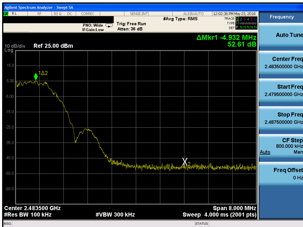
Plot 7-32. Band Edge Plot (Bluetooth (LE), 2Mbps, iPA - Ch. 39)
