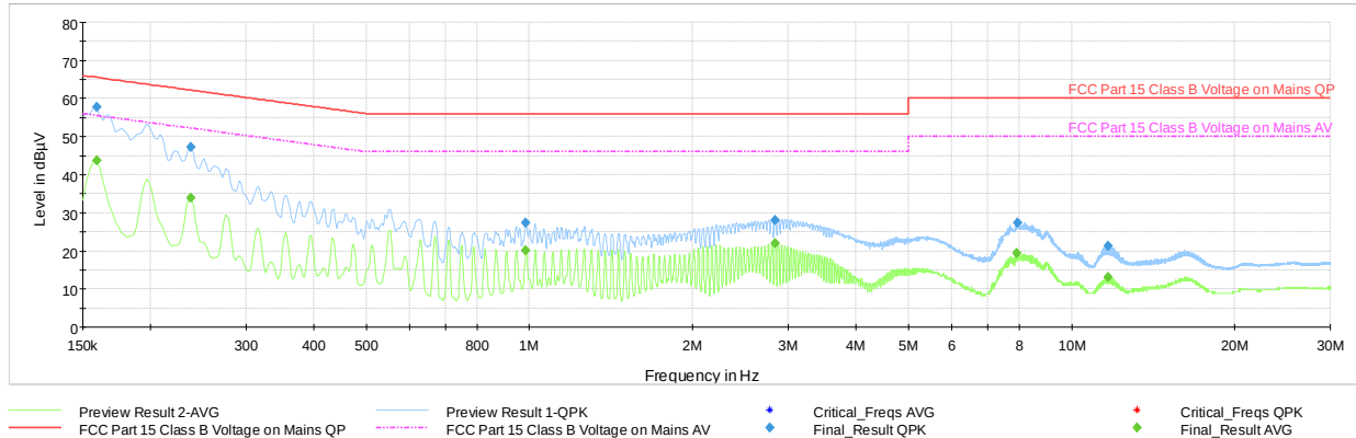
Plot 7-56. Line Conducted Plot with Bluetooth LE (N)
