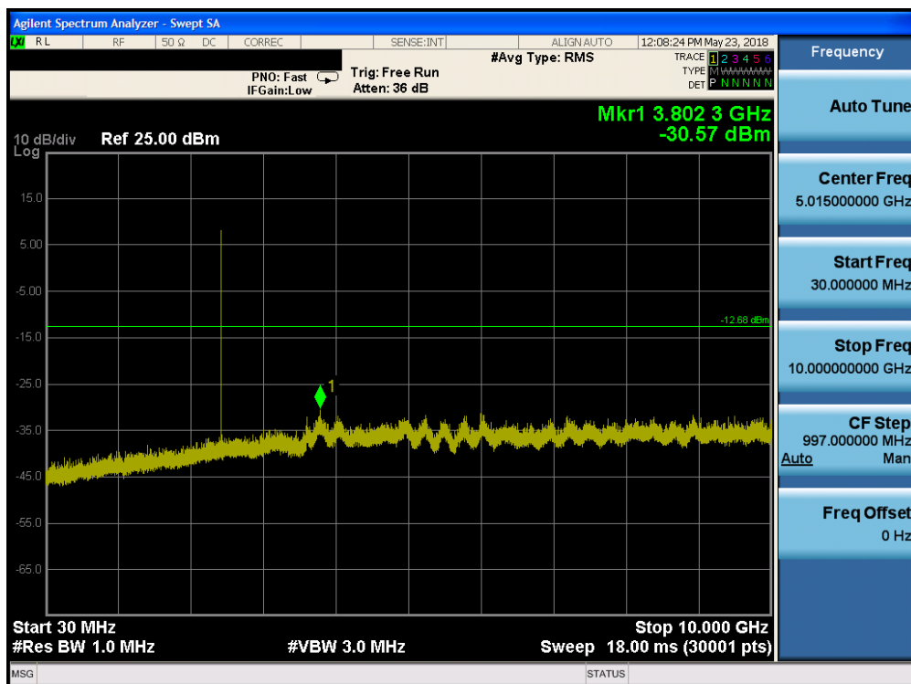
Plot 7-35. Conducted Spurious Plot (Bluetooth (LE), 1Mbps, ePA – Ch. 19)
