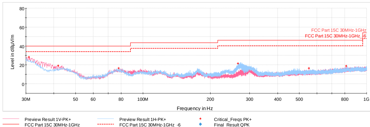
Plot 7-54. Radiated Spurious Plot below 1GHz (1Mbps, ePA, Pol. H & V, with WCP + AC/DC Adapter attached)
