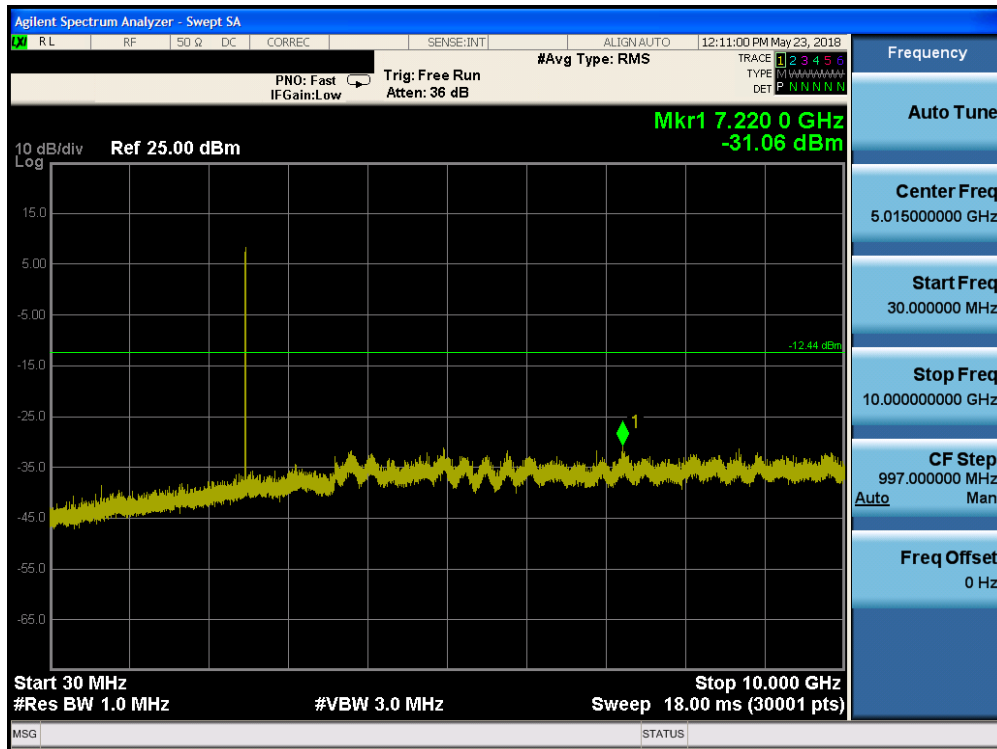
Plot 7-37. Conducted Spurious Plot (Bluetooth (LE), 1Mbps, ePA – Ch. 39)
