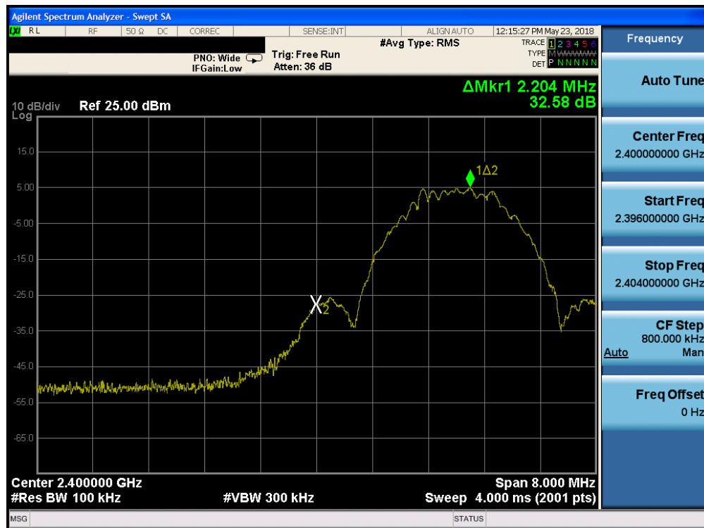
Plot 7-29. Band Edge Plot (Bluetooth (LE), 2Mbps, ePA – Ch. 0)
