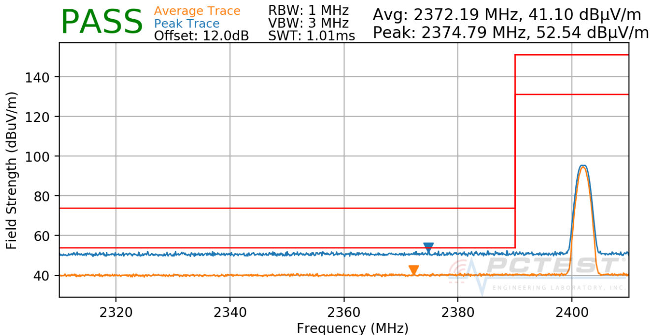
Plot 7-51. Radiated Restricted Lower Band Edge Measurement (Average & Peak)
