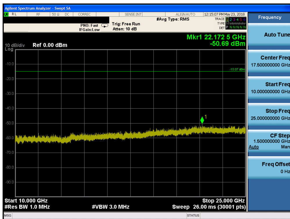
Plot 7-40. Conducted Spurious Plot (Bluetooth (LE), 2Mbps, ePA – Ch. 0)
