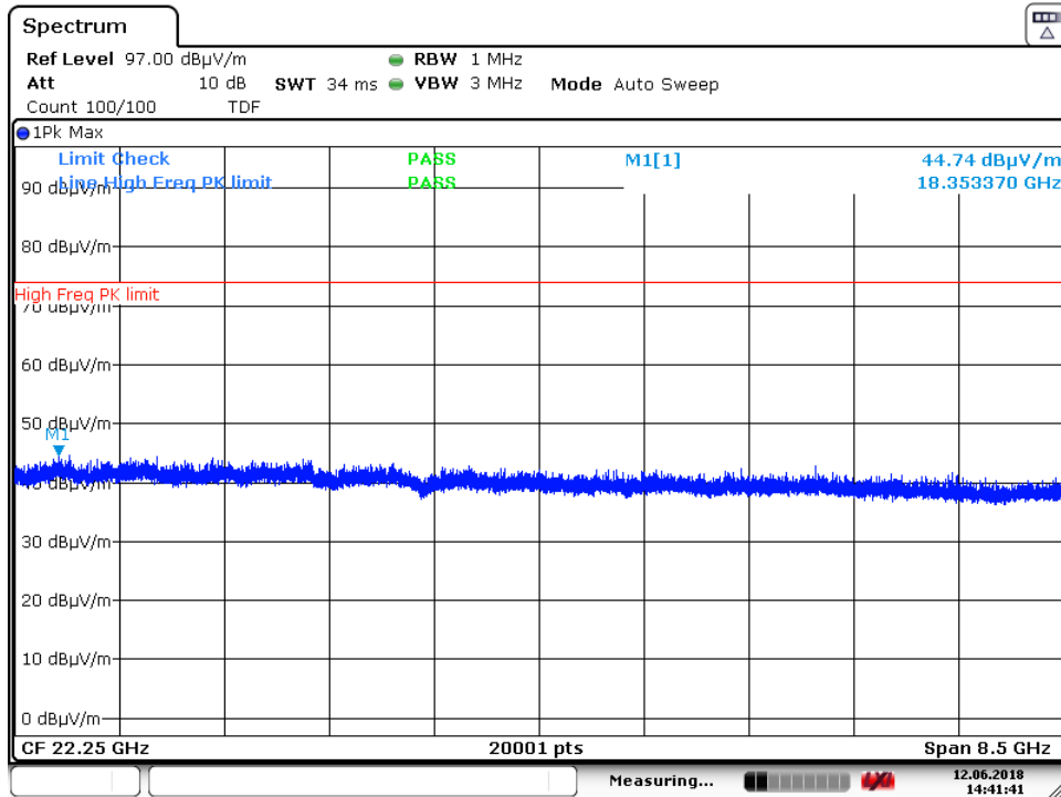
Plot 7-48. Radiated Spurious Plot Above 18GHz (1Mbps, ePA, Ant. Pol. H)
