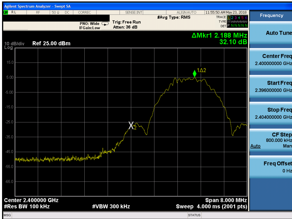
Plot 7-31. Band Edge Plot (Bluetooth (LE), 2Mbps, iPA - Ch. 0)
