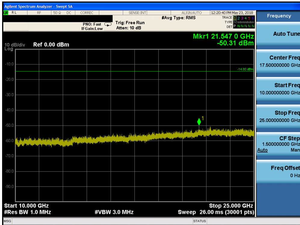
Plot 7-44. Conducted Spurious Plot (Bluetooth (LE), 2Mbps, ePA – Ch. 39)
