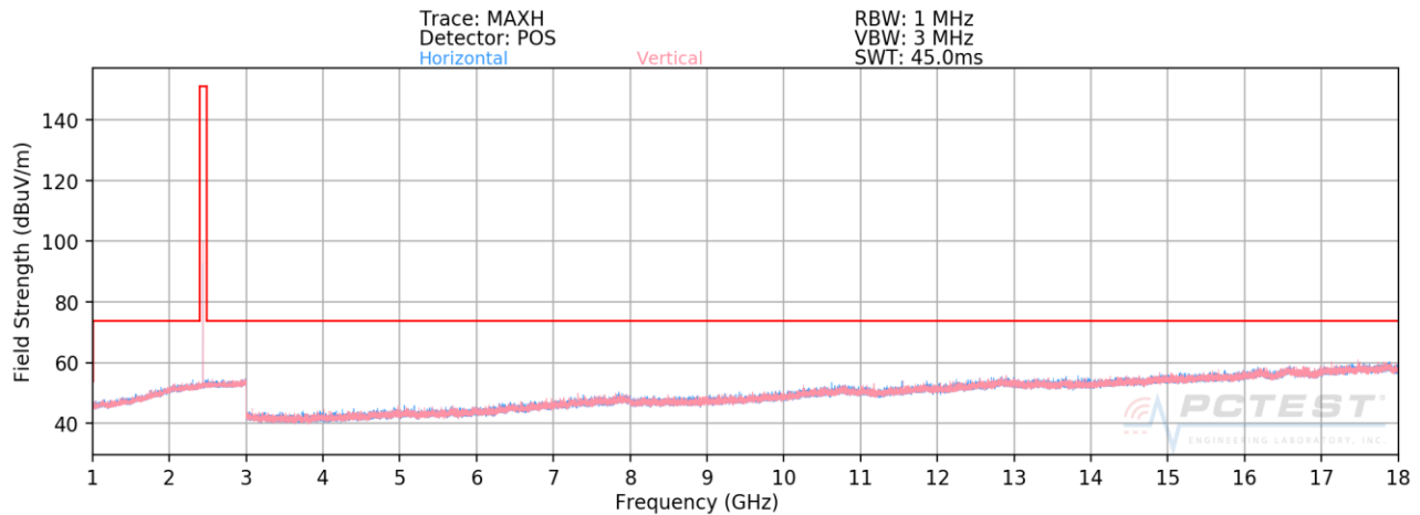
Plot 7-46. Radiated Spurious Plot Above 1GHz (1Mbps, ePA – Ch. 19, Ant. Pol. H & V)
