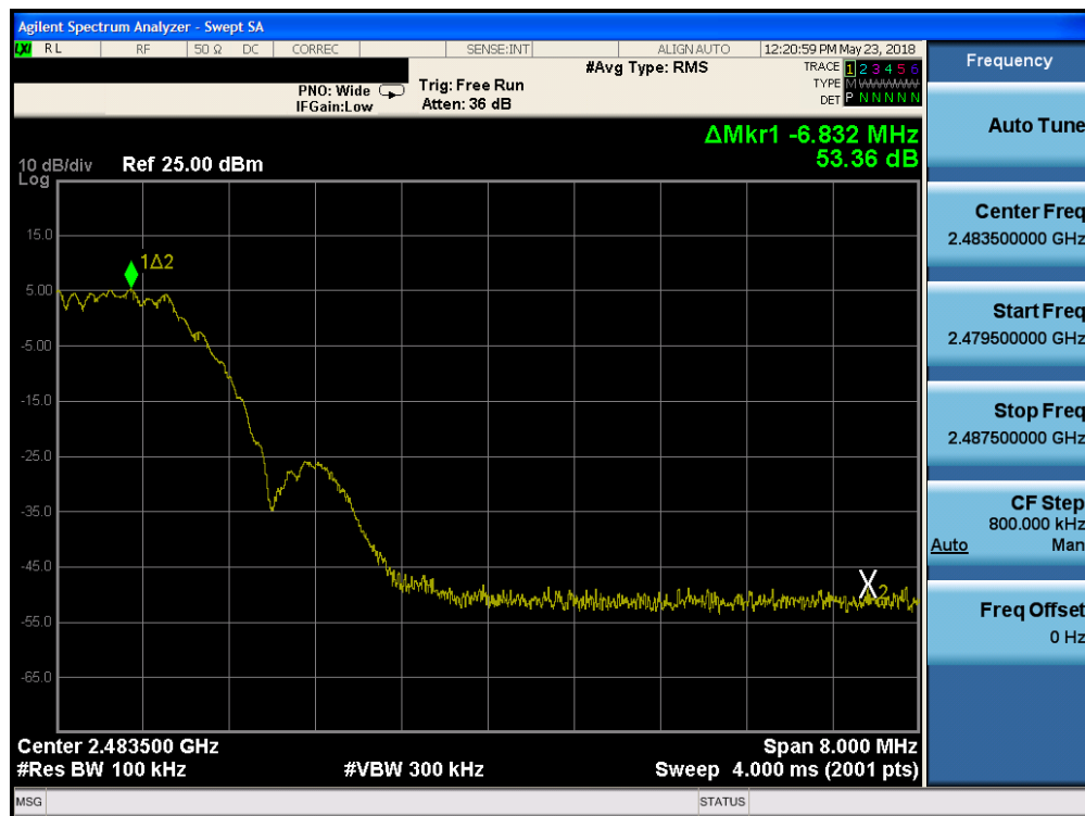
Plot 7-30. Band Edge Plot (Bluetooth (LE), 2Mbps, ePA – Ch. 39)
