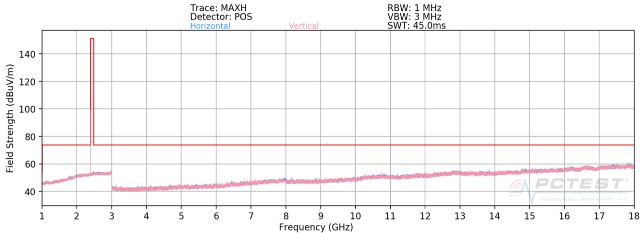
Plot 7-45. Radiated Spurious Plot Above 1GHz (1Mbps, ePA – Ch. 0, Ant. Pol. H & V)
