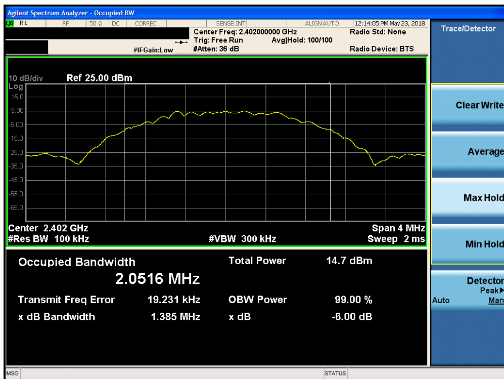
Plot 7-7. 6dB Bandwidth Plot (Bluetooth (LE), 2Mbps, ePA – Ch. 0)
