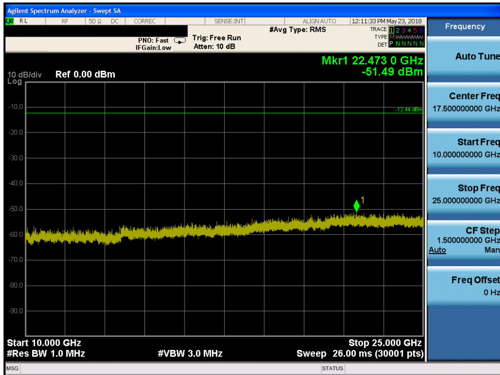
Plot 7-38. Conducted Spurious Plot (Bluetooth (LE), 1Mbps, ePA – Ch. 39)
