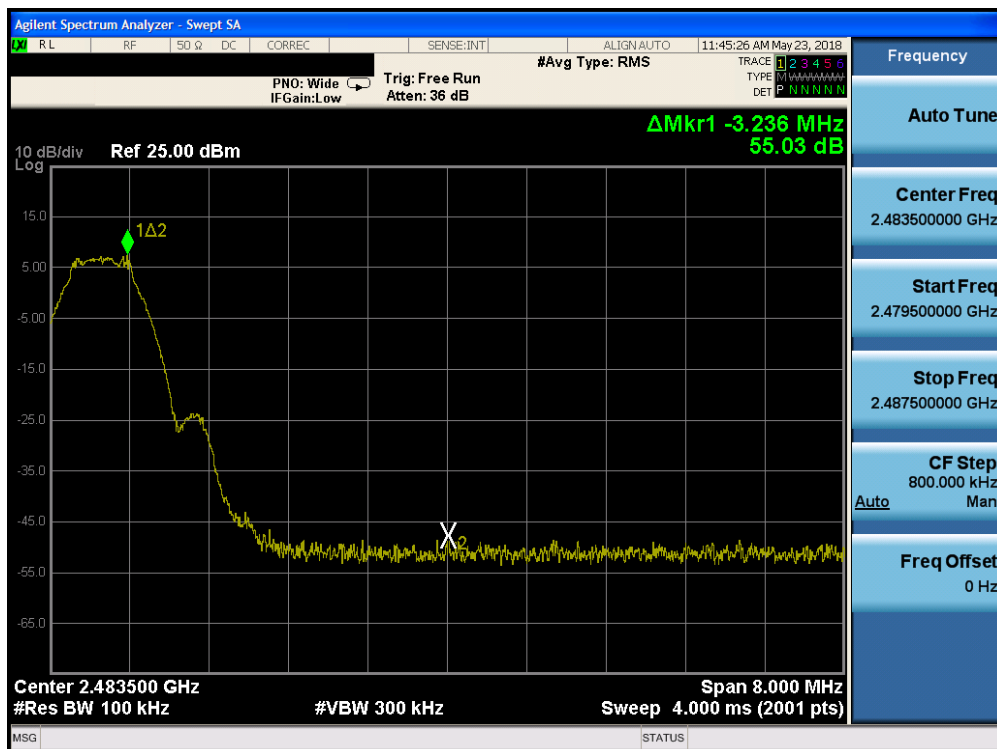
Plot 7-28. Band Edge Plot (Bluetooth (LE), 1Mbps, iPA - Ch. 39)
