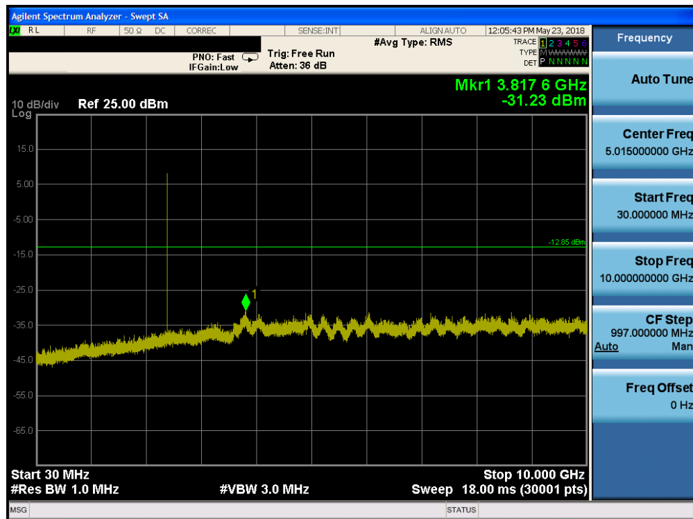
Plot 7-33. Conducted Spurious Plot (Bluetooth (LE), 1Mbps, ePA – Ch. 0)
