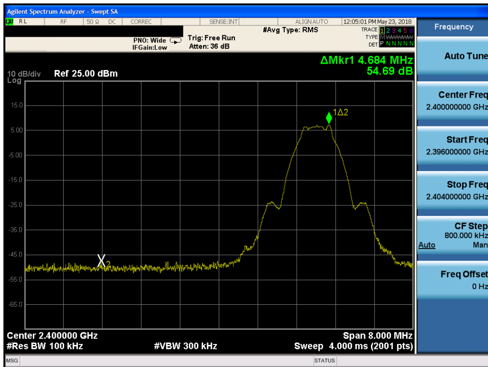
Plot 7-25. Band Edge Plot (Bluetooth (LE), 1Mbps, ePA – Ch. 0)
