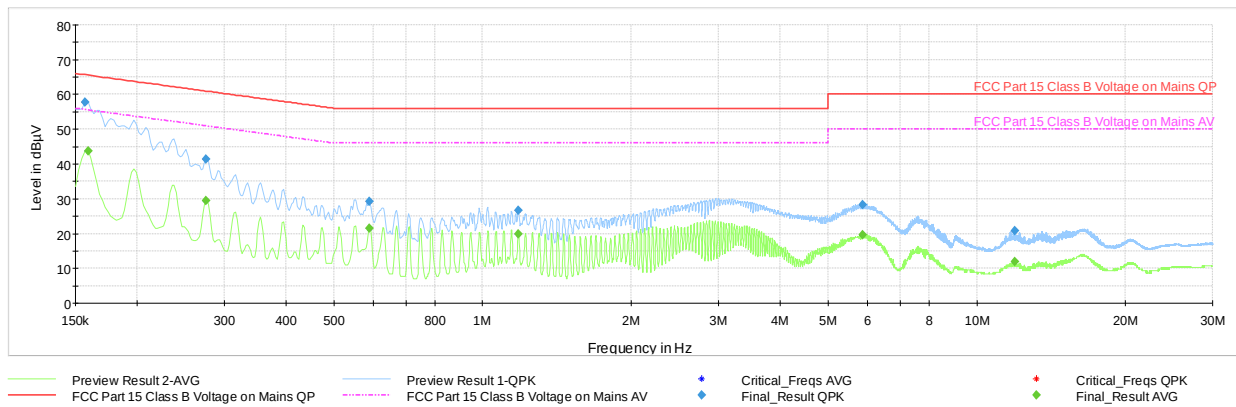
Plot 7-55. Line Conducted Plot with Bluetooth LE (L1)
