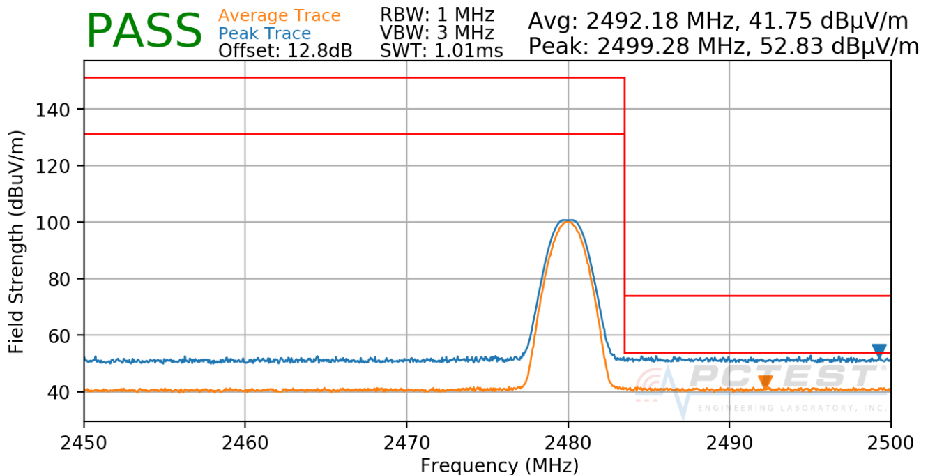
Plot 7-52. Radiated Restricted Upper Band Edge Measurement (Average & Peak)
