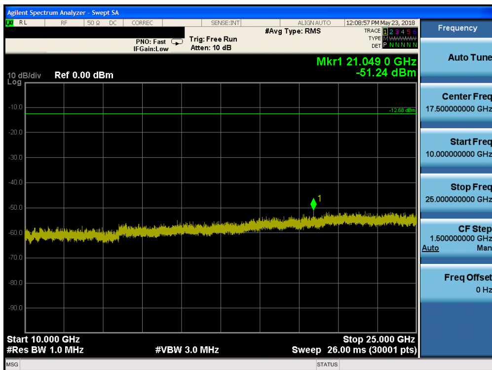
Plot 7-36. Conducted Spurious Plot (Bluetooth (LE), 1Mbps, ePA – Ch. 19)
