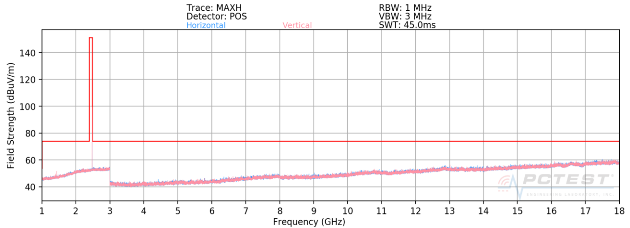
Plot 7-47. Radiated Spurious Plot Above 1GHz (1Mbps, ePA – Ch. 39, Ant. Pol. H & V)
