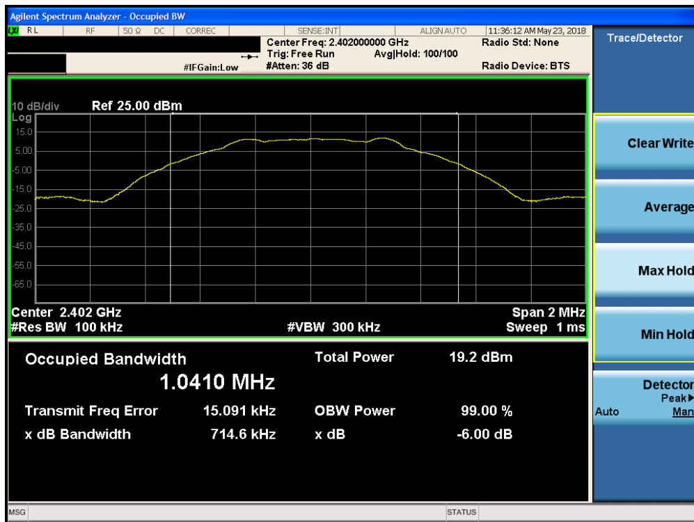
Plot 7-4. 6dB Bandwidth Plot (Bluetooth (LE), 1Mbps, iPA – Ch. 0)
