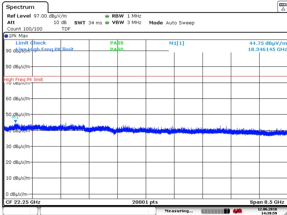
Plot 7-49. Radiated Spurious Plot Above 18GHz (1Mbps, ePA, Ant. Pol. V)
