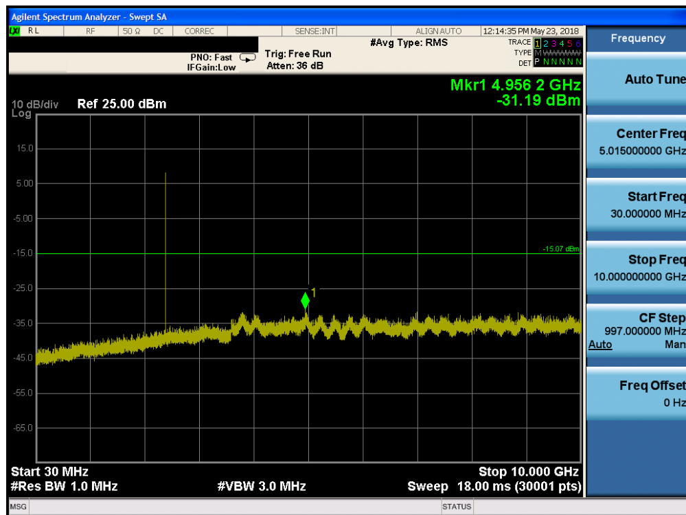
Plot 7-39. Conducted Spurious Plot (Bluetooth (LE), 2Mbps, ePA – Ch. 0)
