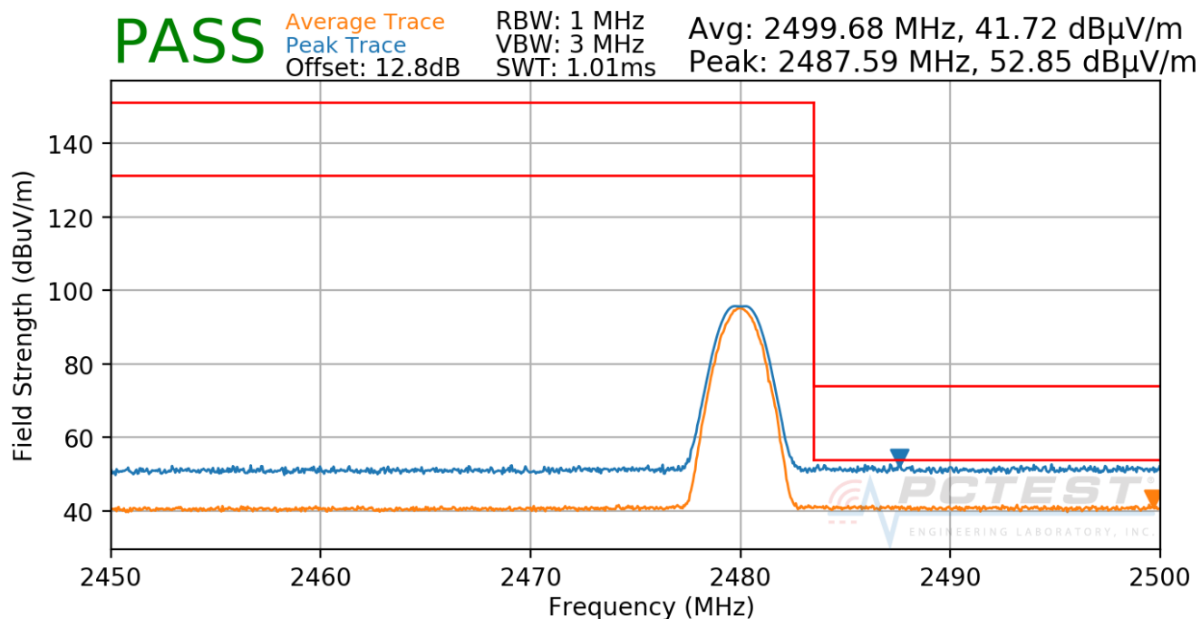
Plot 7-53. Radiated Restricted Upper Band Edge Measurement (Average & Peak)
