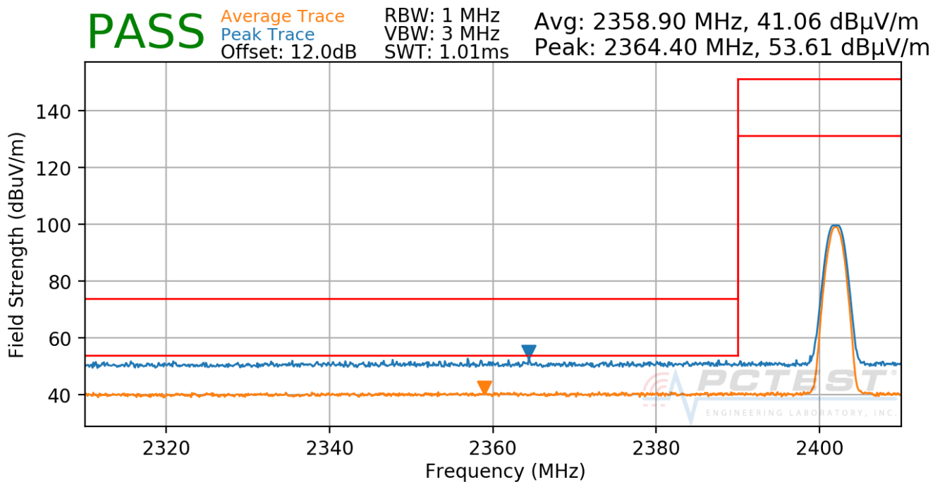
Plot 7-50. Radiated Restricted Lower Band Edge Measurement (Average & Peak)
