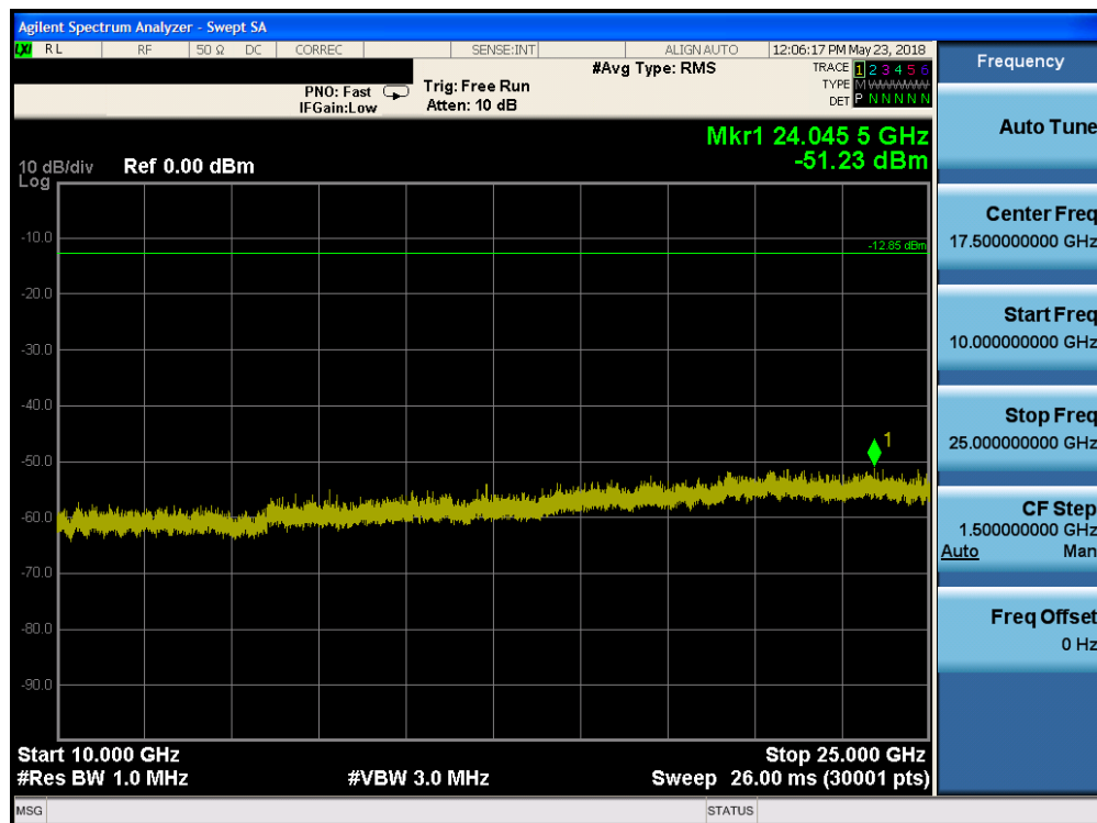
Plot 7-34. Conducted Spurious Plot (Bluetooth (LE), 1Mbps, ePA – Ch. 0)
