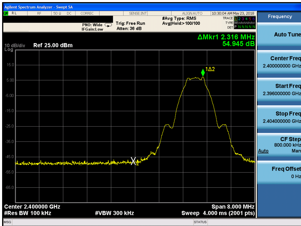
Plot 7-27. Band Edge Plot (Bluetooth (LE), 1Mbps, iPA - Ch. 0)
