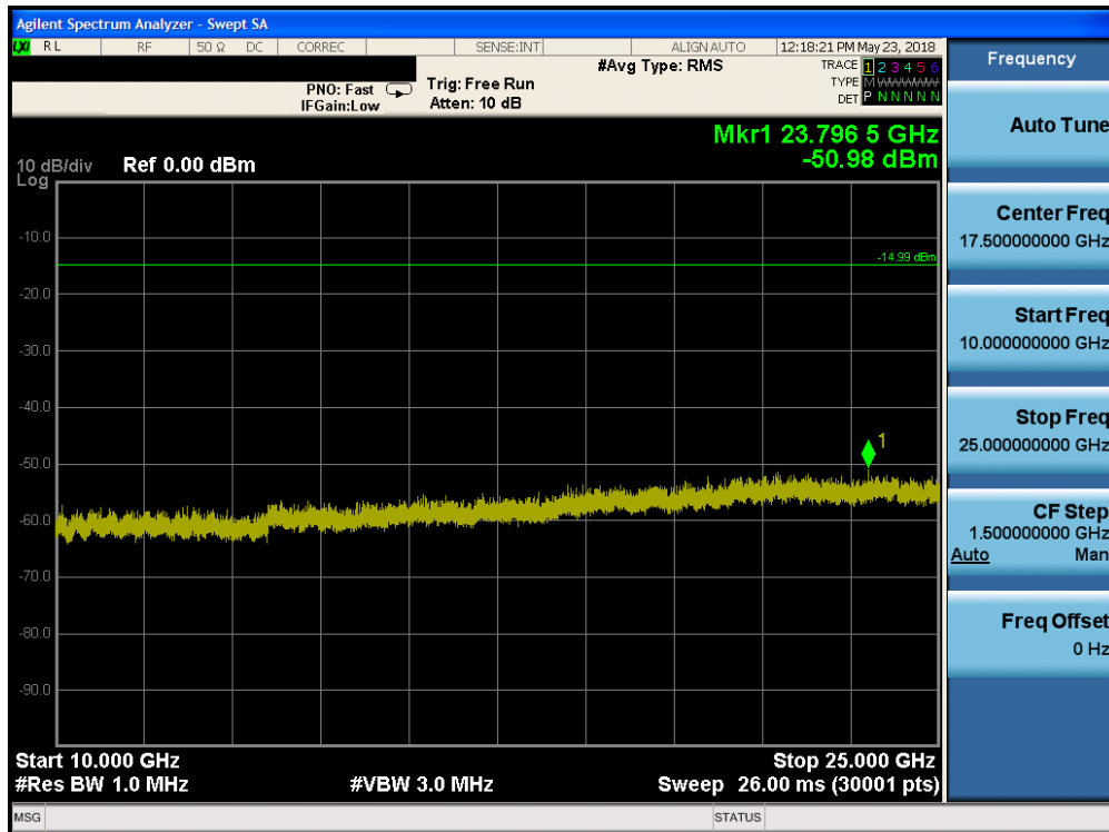
Plot 7-42. Conducted Spurious Plot (Bluetooth (LE), 2Mbps, ePA – Ch. 19)
