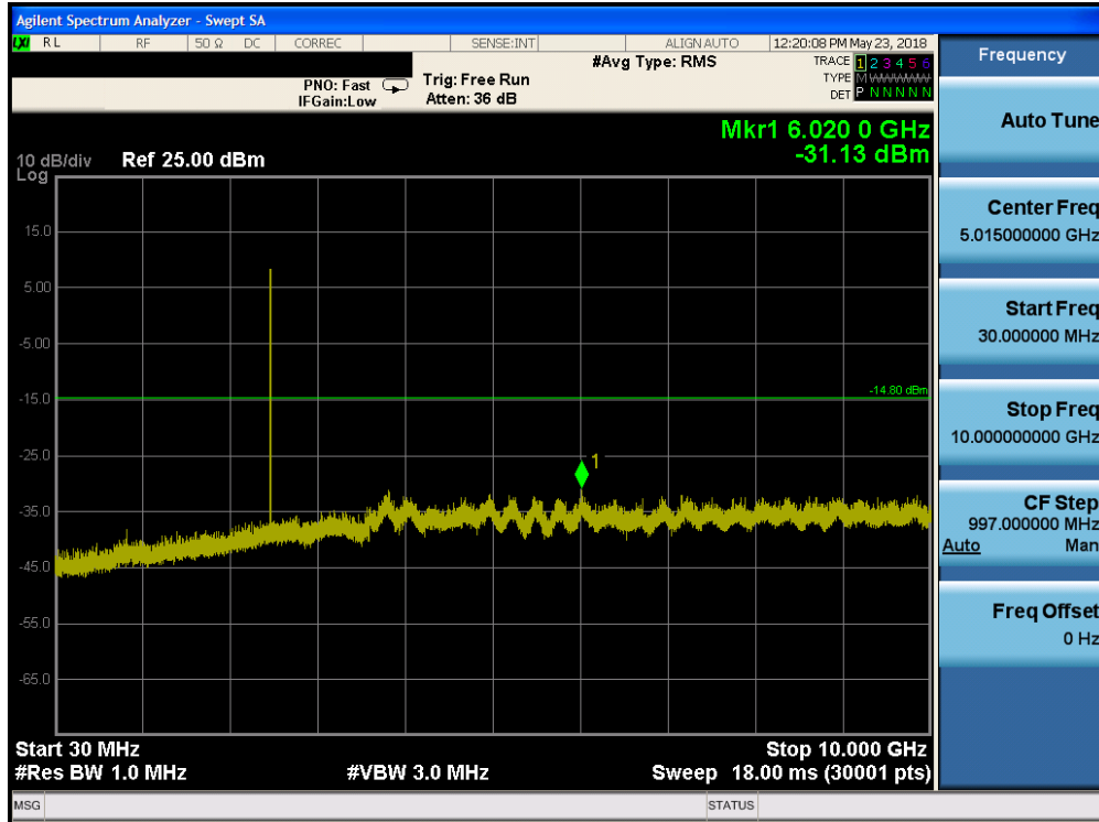
Plot 7-43. Conducted Spurious Plot (Bluetooth (LE), 2Mbps, ePA – Ch. 39)
