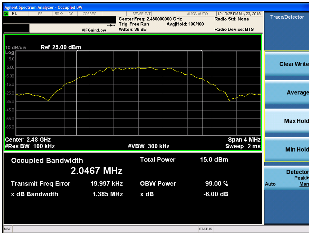
Plot 7-9. 6dB Bandwidth Plot (Bluetooth (LE), 2Mbps, ePA – Ch. 39)
