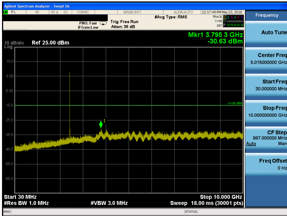
Plot 7-41. Conducted Spurious Plot (Bluetooth (LE), 2Mbps, ePA – Ch. 19)
