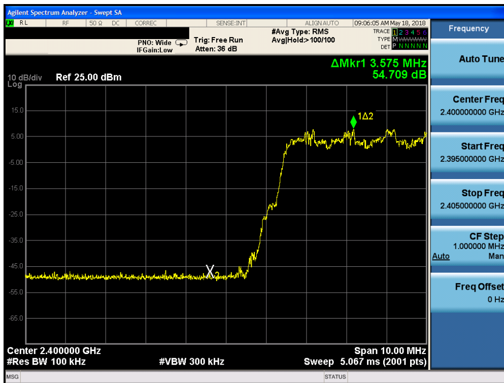
Plot 7-39. Band Edge Plot (Bluetooth with Hopping Enabled, 8DPSK, iPA)
