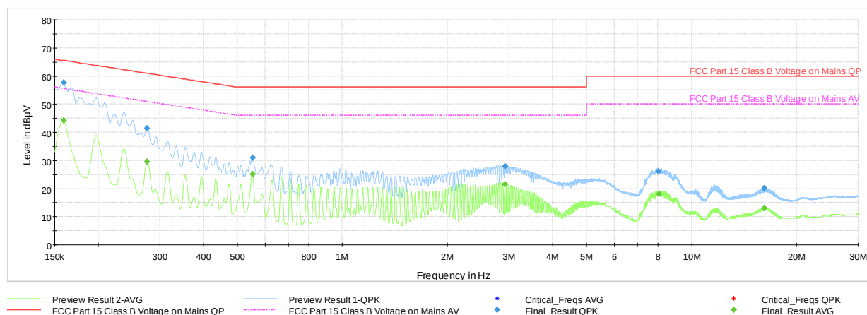
Plot 7-76. Line-Conducted Test Plot (N)
