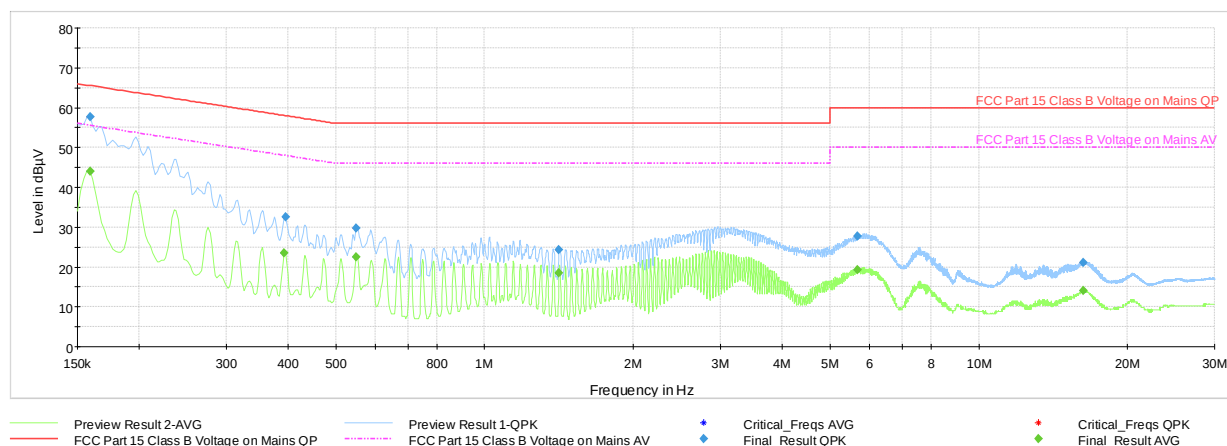
Plot 7-75. Line-Conducted Test Plot (L1)
