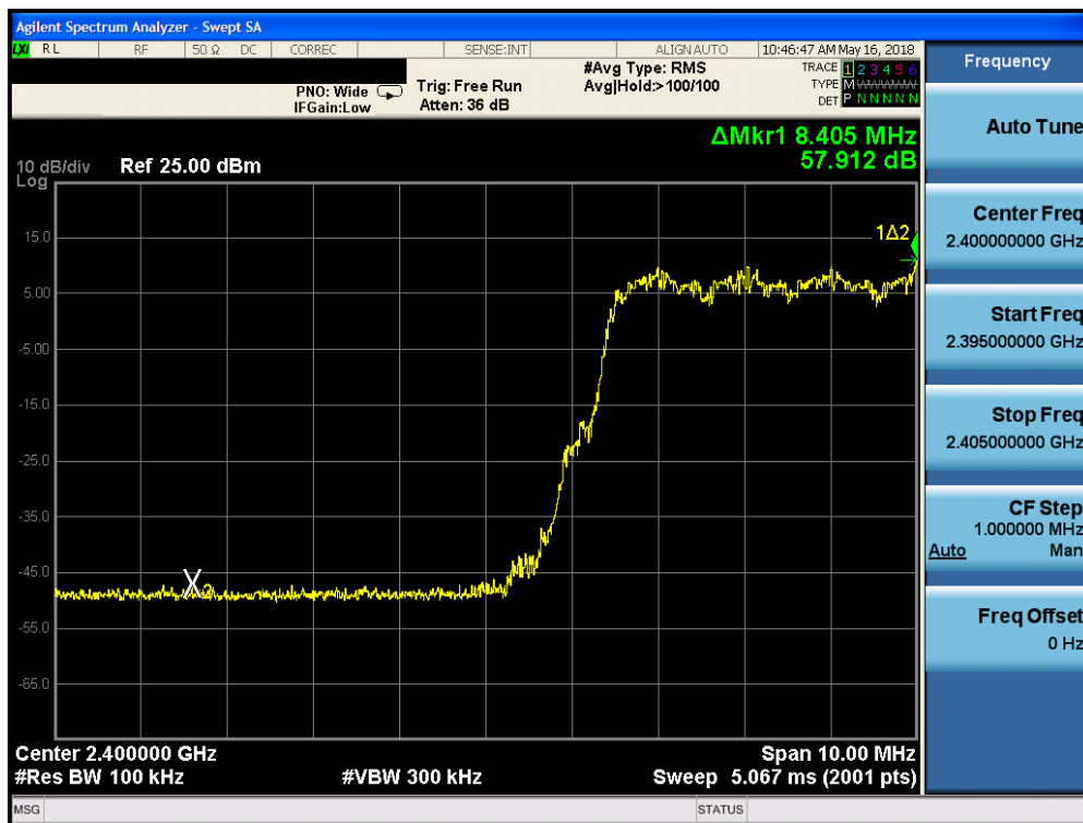
Plot 7-35. Band Edge Plot (Bluetooth with Hopping Enabled, 8DPSK, ePA)
