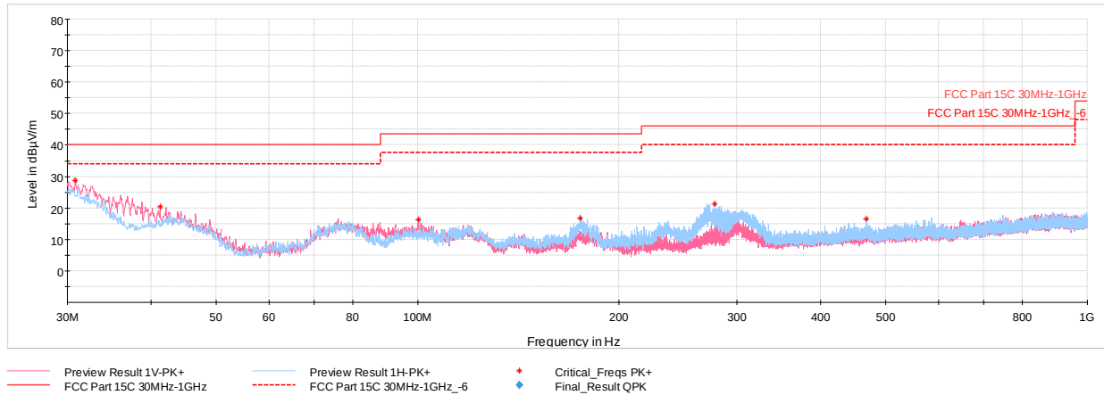
Plot 7-74. Radiated Spurious Plot below 1GHz (GFSK, ePA, with WCP + AC/DC Adapter attached)
