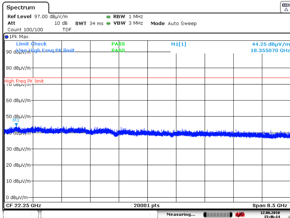
Plot 7-65. Radiated Spurious Plot above 18GHz GFSK ePA (Vertical)
