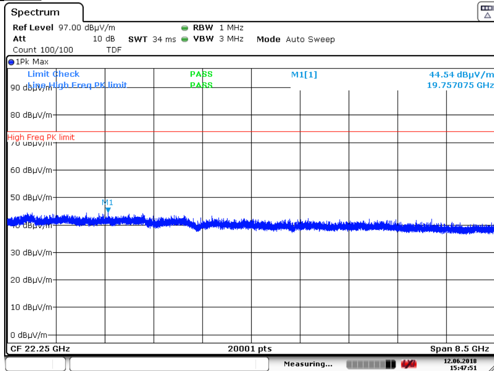
Plot 7-64. Radiated Spurious Plot above 18GHz GFSK ePA (Horizontal)
