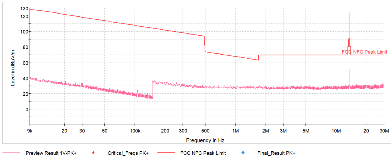
Plot 7-4. Radiated Spurious Plot 9kHz – 30MHz (Reader 100% Ask 1 out of 4 - Pol. Z)
