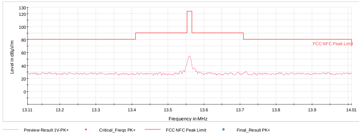
Plot 7-1. In Band Radiated Spurious Plot (CE A 848kdps, Pol. X)
