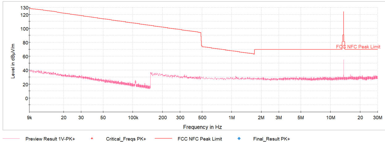
Plot 7-3. Radiated Spurious Plot 9kHz – 30MHz (CE A 848kbps - Pol. Z)
