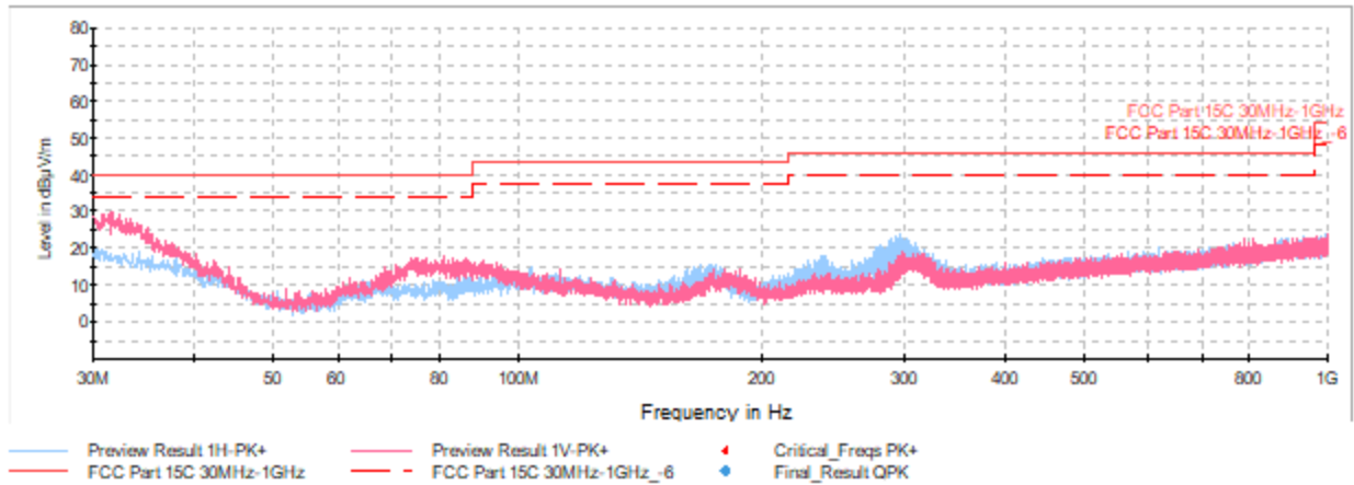
Plot 7-5. Radiated Spurious Plot 30MHz – 1GHz (CE A 848kdps, Pol. H & V, with WCP + AC/DC Adapter attached)
