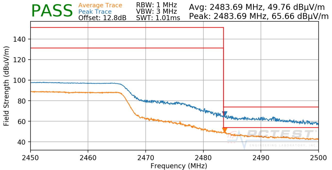
Plot 7-42. Radiated Restricted Upper Band Edge Measurement Ch. 10
