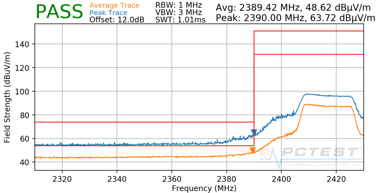
Plot 7-40. Radiated Restricted Lower Band Edge Measurement Ch. 2
