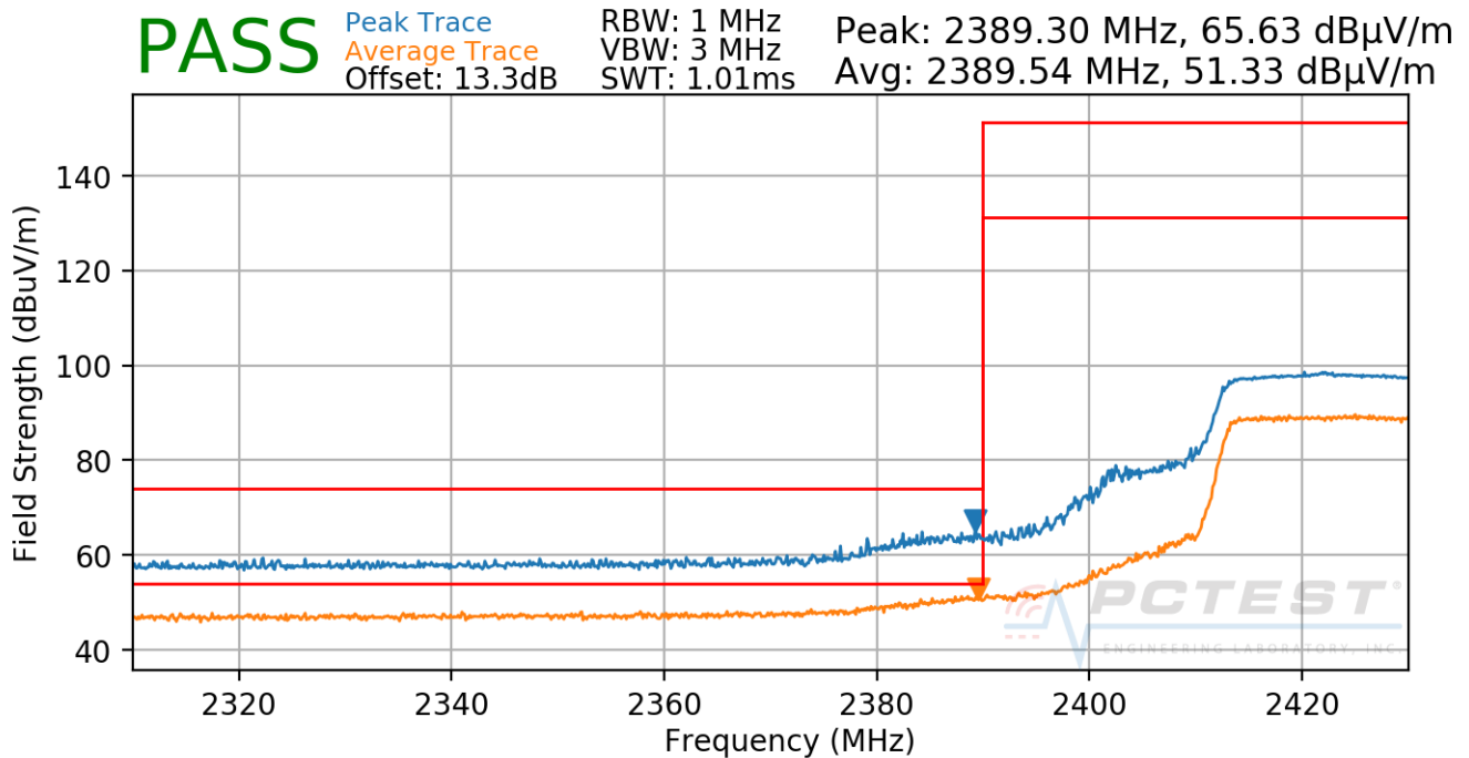
Plot 7-41. Radiated Restricted Lower Band Edge Measurement Ch. 3
