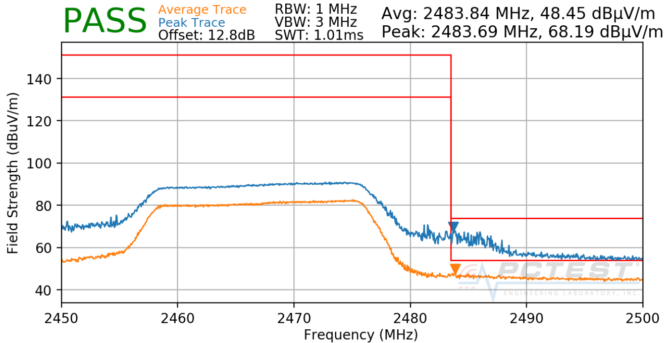
Plot 7-44. Radiated Restricted Upper Band Edge Measurement Ch. 12
