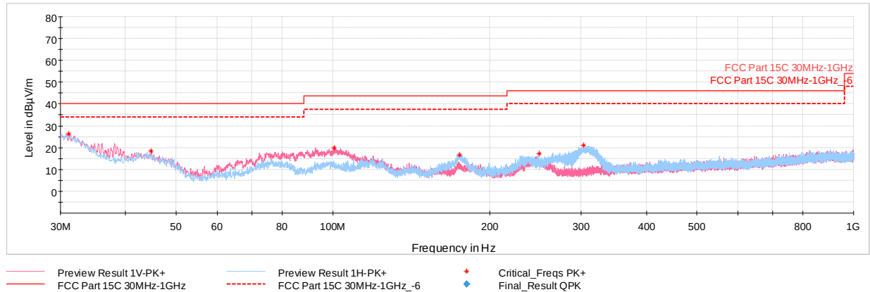
Plot 7-46. Radiated Spurious Plot below 1GHz (with WCP + AC/DC Adapter attached)
