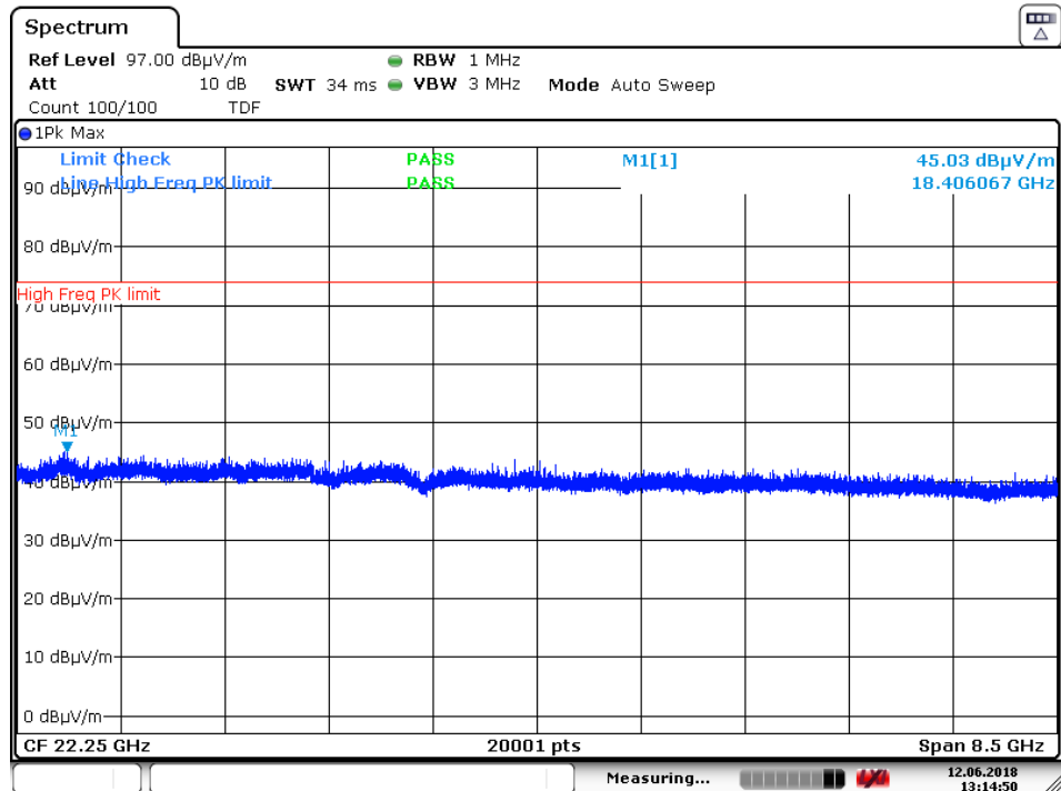
Plot 7-35. Radiated Spurious Plot above 18GHz (802.11b – Ch. 7) Vertical
