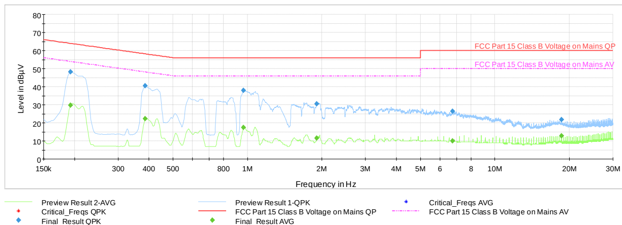
Plot 7-47. Line Conducted Plot with 802.11b (L1 with WCP + AC/DC Adapter attached)
