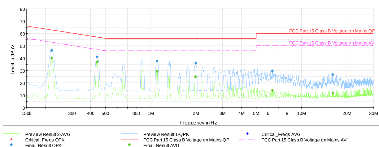
Plot 7-48. Line Conducted Plot with 802.11b (N with WCP + AC/DC Adapter attached)
