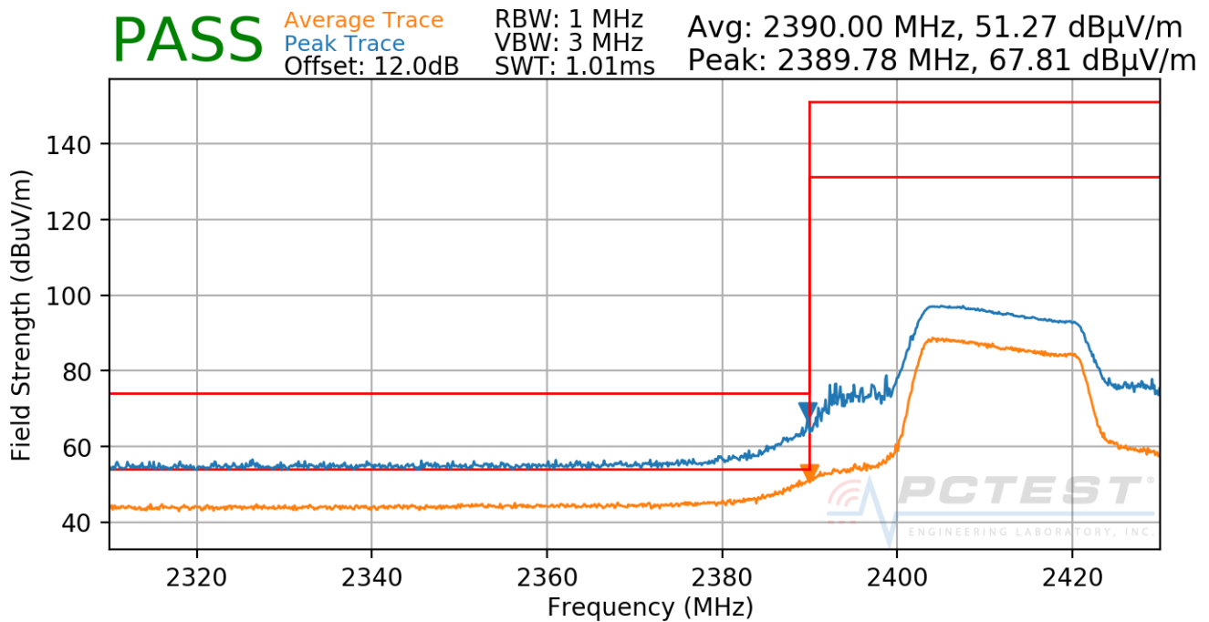
Plot 7-39. Radiated Restricted Lower Band Edge Measurement Ch. 1
