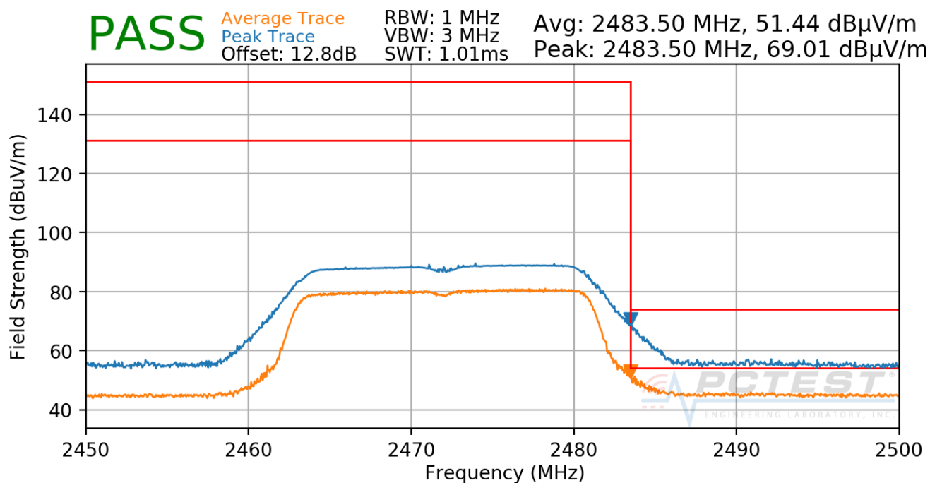
Plot 7-45. Radiated Restricted Upper Band Edge Measurement Ch. 13
