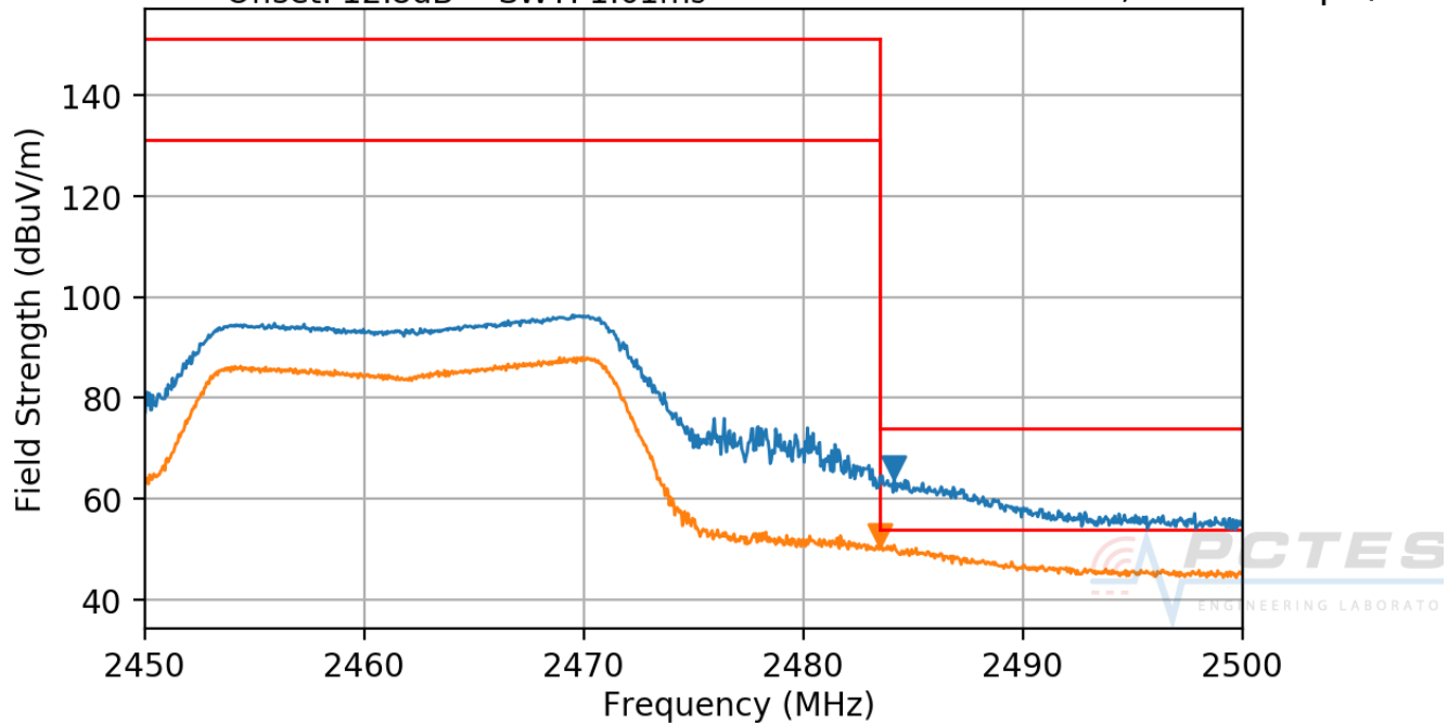
Plot 7-43. Radiated Restricted Upper Band Edge Measurement Ch. 11
