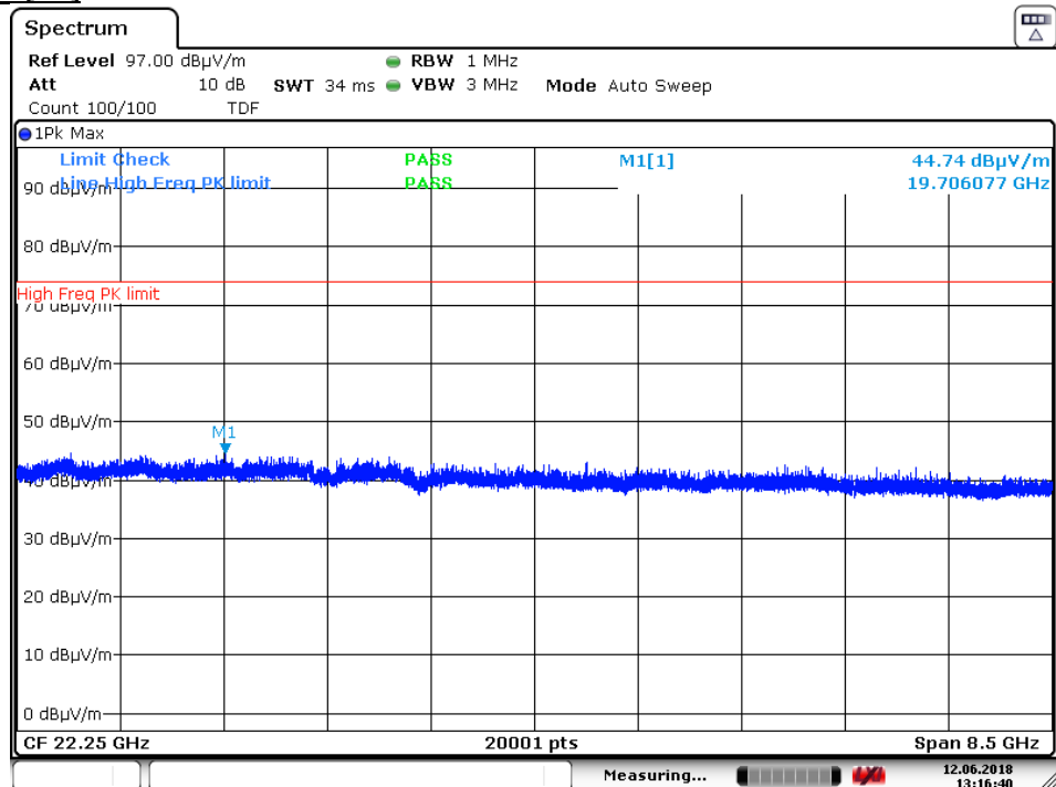
Plot 7-34. Radiated Spurious Plot above 18GHz (802.11b – Ch. 7) Horizontal
