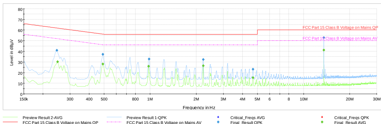
Plot 7-8. Line-Conducted Test Plot (N, with WCP + AC/DC Adapter attached)
