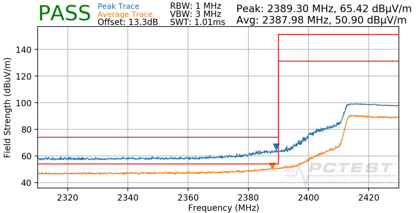
Plot 7-41. Radiated Restricted Lower Band Edge Measurement (Average & Peak)
