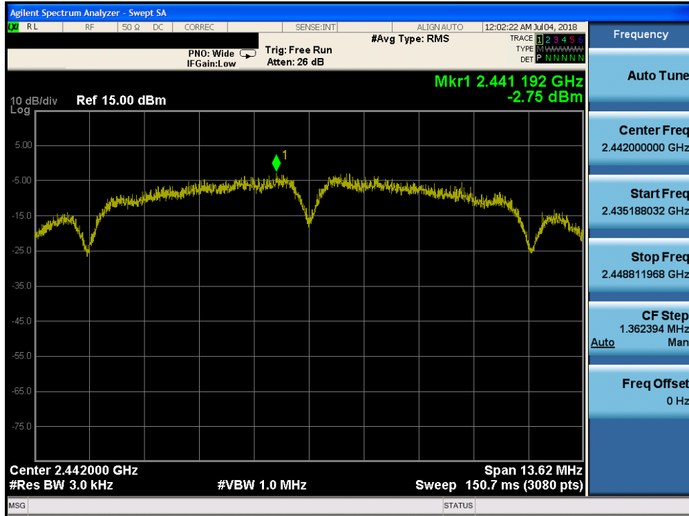
Plot 7-11. Power Spectral Density Plot (802.11b – Ch. 7)
