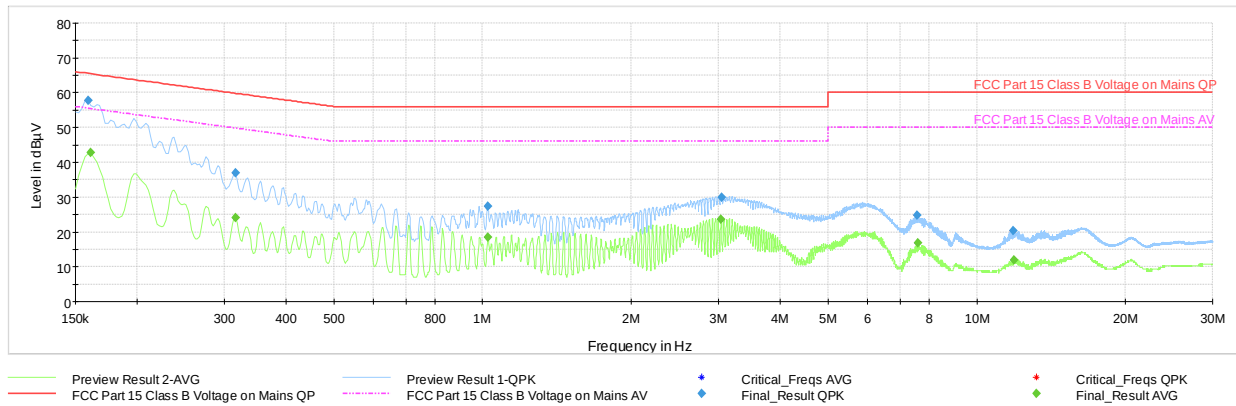
Plot 7-47. Line Conducted Plot with 802.11b (L1, with WCP + Laptop attached)
