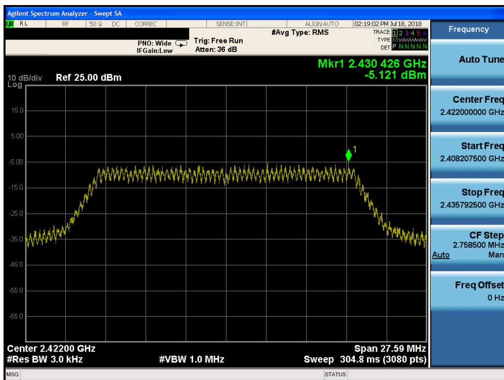
Plot 7-16. Power Spectral Density Plot (802.11n (2.4GHz) – Ch. 3)
