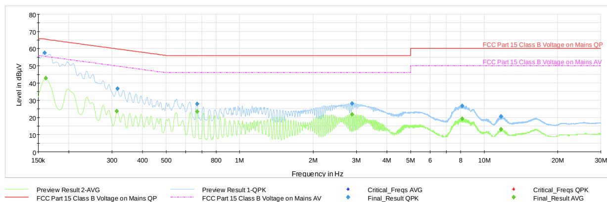
Plot 7-48. Line Conducted Plot with 802.11b (N, with WCP + Laptop attached)
