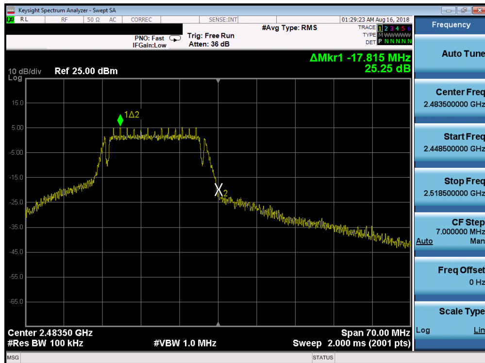
Plot 7-22. Band Edge Plot (802.11g - Ch. 13)
