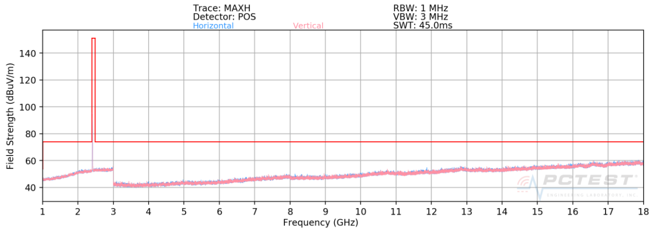
Plot 7-31. Radiated Spurious Plot above 1GHz (802.11b – Ch. 1, Ant. Pol. H & V)
