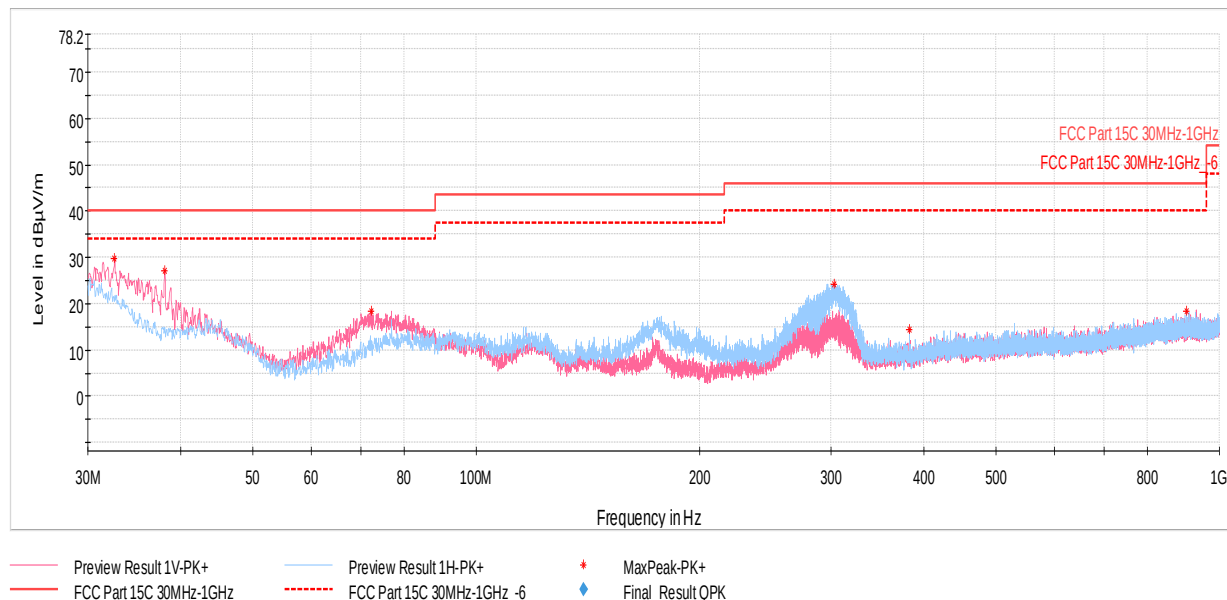
Plot 7-46. Radiated Spurious Plot below 1GHz (802.11b – Ch. 7, Pol. H & V, with WCP + AC/DC Adapter attached)
