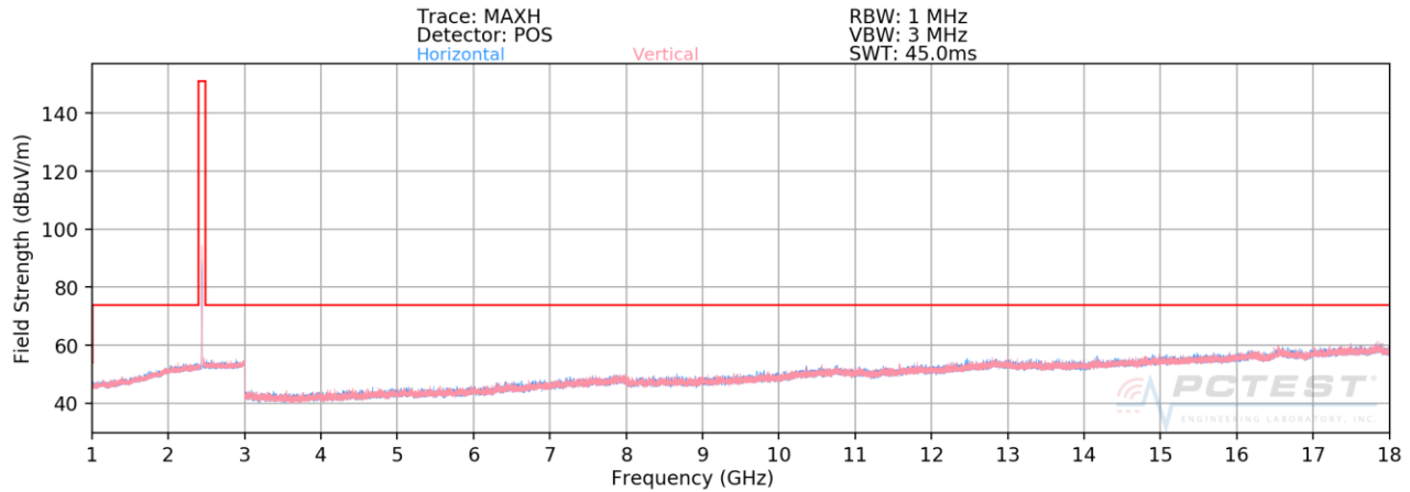
Plot 7-32. Radiated Spurious Plot above 1GHz (802.11b – Ch. 7, Ant. Pol. H & V)
