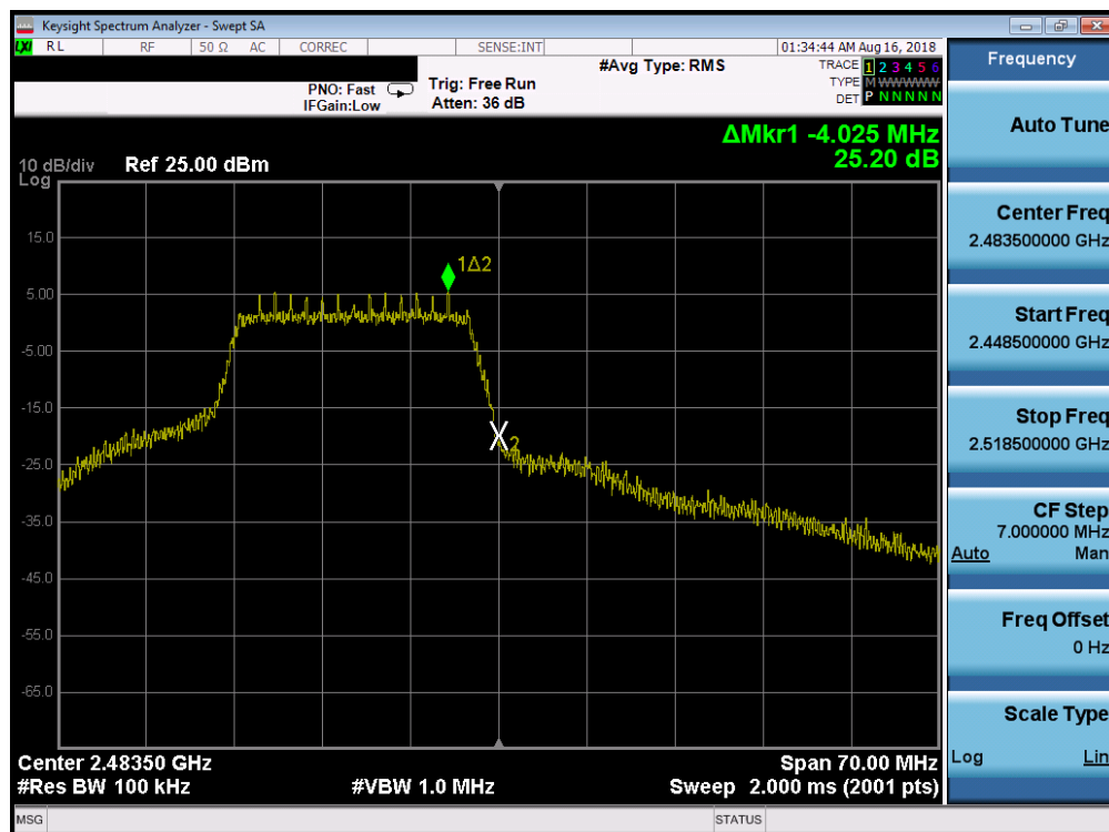
Plot 7-24. Band Edge Plot (802.11n (2.4GHz) – Ch. 13)
