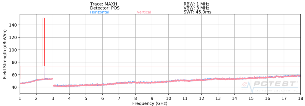
Plot 7-33. Radiated Spurious Plot above 1GHz (802.11b – Ch. 13, Ant. Pol. H & V)
