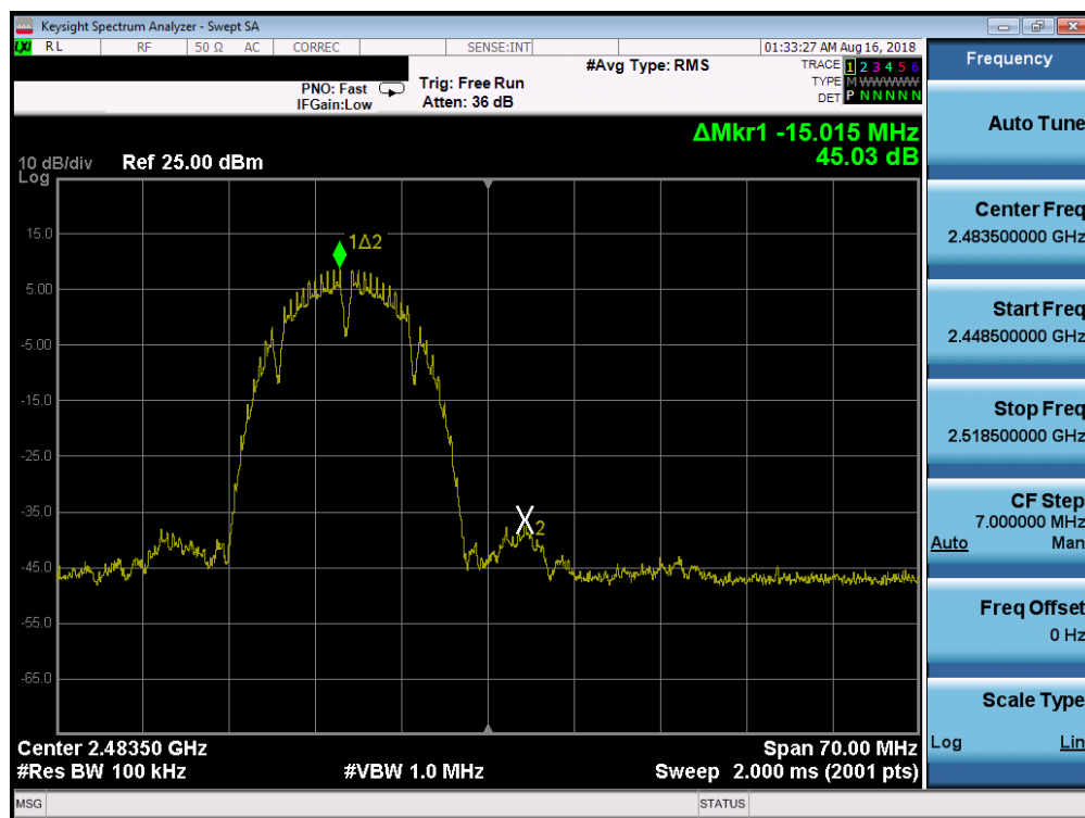
Plot 7-20. Band Edge Plot (802.11b – Ch. 13)
