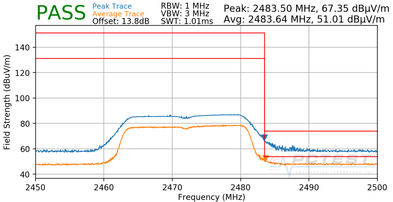
Plot 7-45. Radiated Restricted Upper Band Edge Measurement (Average & Peak)
