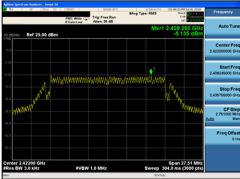
Plot 7-13. Power Spectral Density Plot (802.11g – Ch. 3)
