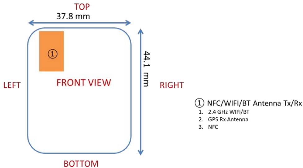
Figure F-1 DUT Antenna Locations
