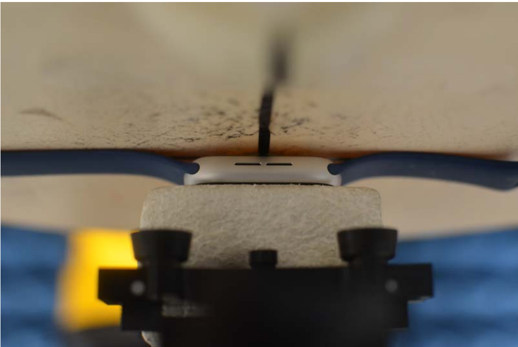
SAR Test Setup Photo 4: Aluminum back side at 0.0 cm with Sport wrist band
