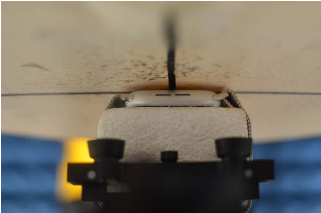
SAR Test Setup Photo 6: Aluminum back side at 0.0 cm with Metal Loop band
