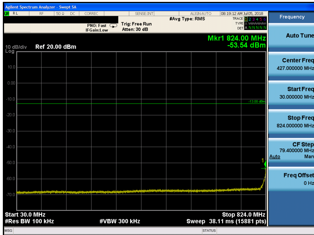
Plot 7-5. Conducted Spurious Plot (Cellular WCDMA Mode - Mid Channel)
