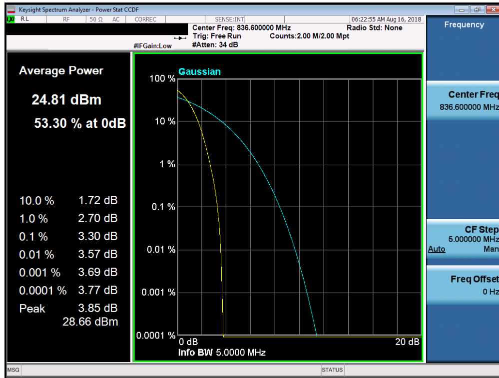
Plot 7-13. Peak-Average Ratio Plot (Cellular WCDMA Mode)
