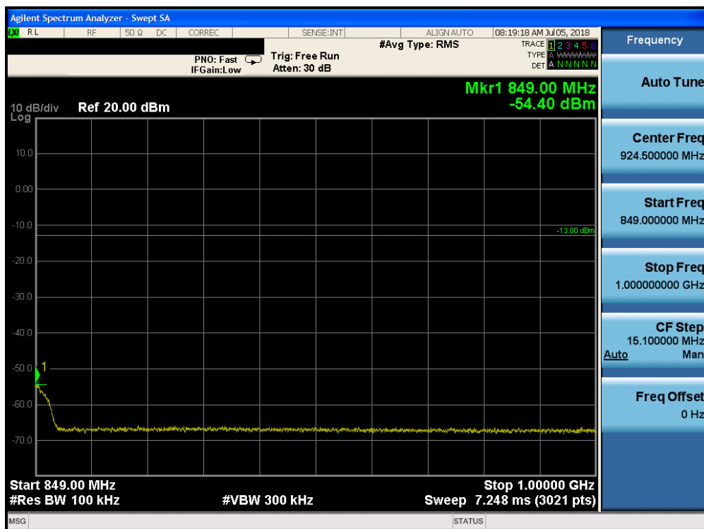
Plot 7-6. Conducted Spurious Plot (Cellular WCDMA Mode - Mid Channel)
