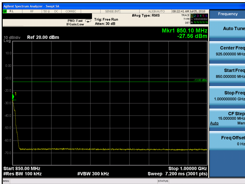
Plot 7-9. Conducted Spurious Plot (Cellular WCDMA Mode - High Channel)
