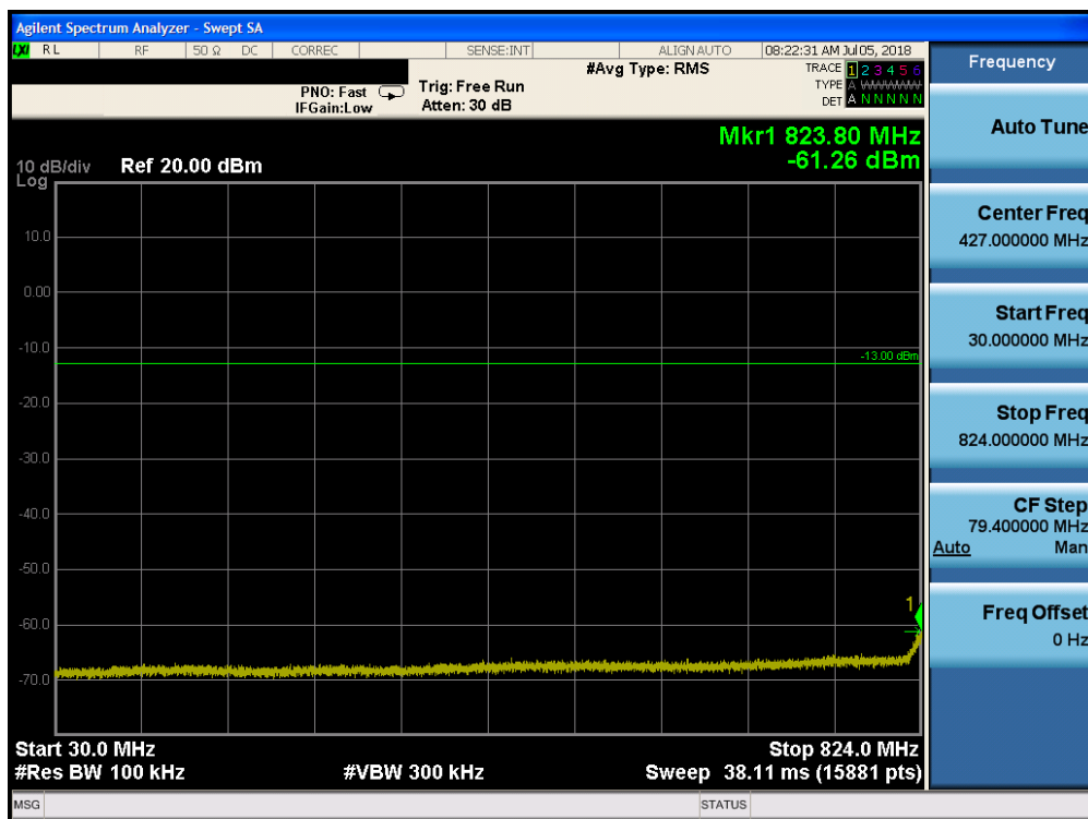
Plot 7-8. Conducted Spurious Plot (Cellular WCDMA Mode - High Channel)
