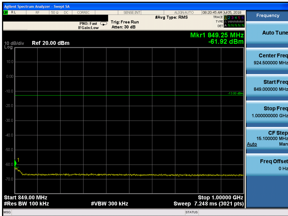
Plot 7-3. Conducted Spurious Plot (Cellular WCDMA Mode - Low Channel)
