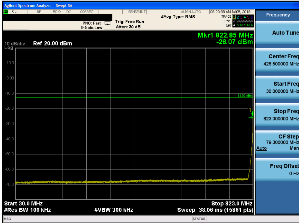
Plot 7-2. Conducted Spurious Plot (Cellular WCDMA Mode - Low Channel)
