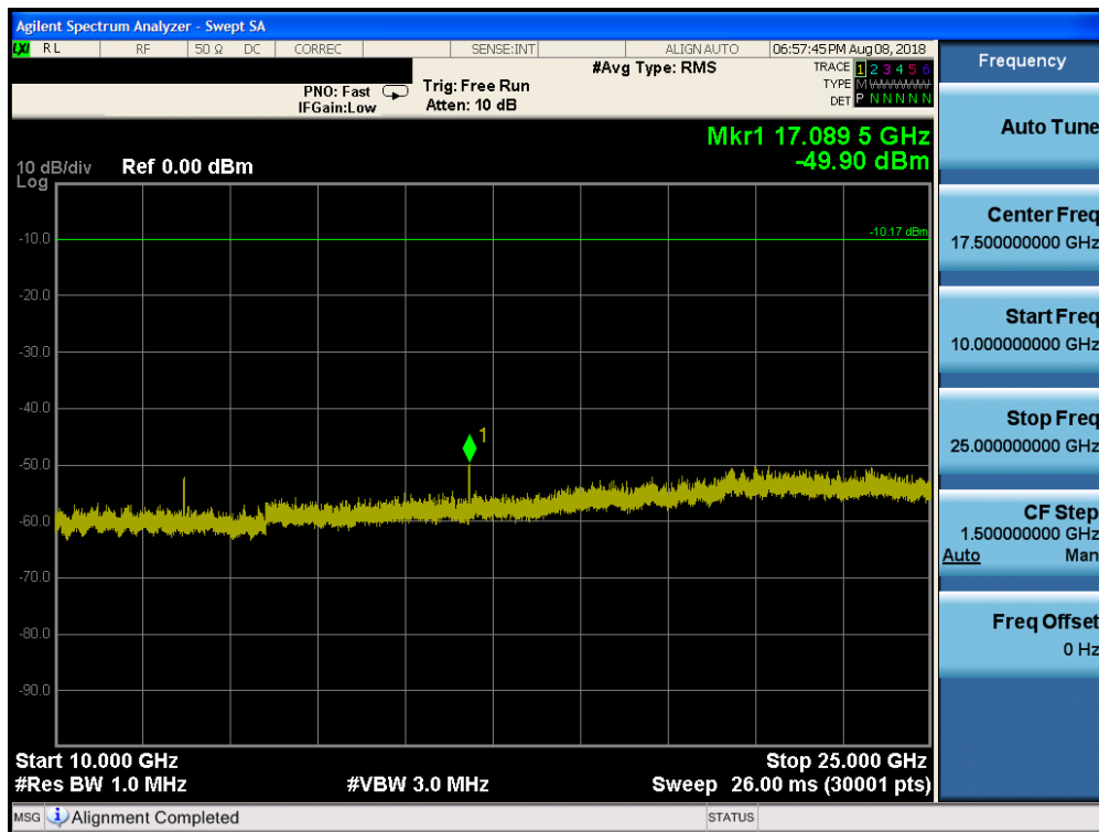
Plot 7-36. Conducted Spurious Plot (Bluetooth (HDR, ePA), 4Mbps – Ch. 38)
