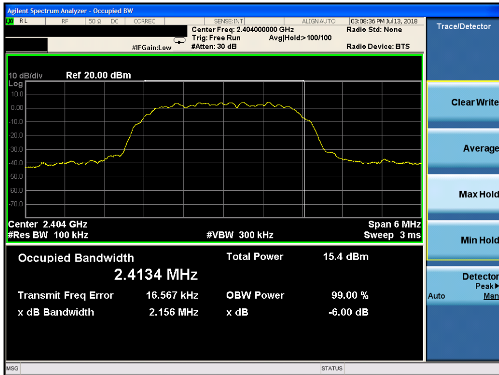
Plot 7-1. 6dB Bandwidth Plot (Bluetooth (HDR, ePA), 4Mbps – Ch. 1)
