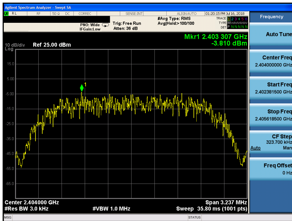
Plot 7-16. Power Spectral Density Plot (Bluetooth (HDR4, iPA), 4Mbps - Ch. 1)
