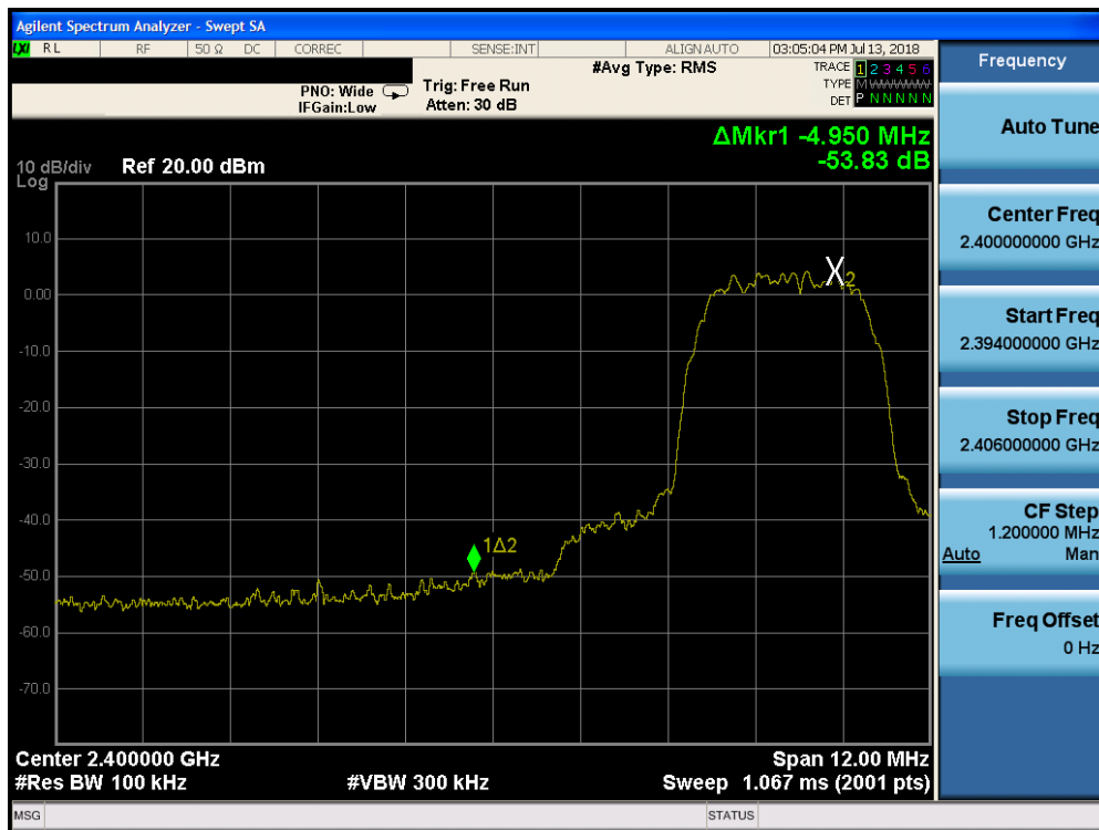
Plot 7-25. Band Edge Plot (Bluetooth (HDR, ePA), 4Mbps – Ch. 1)
