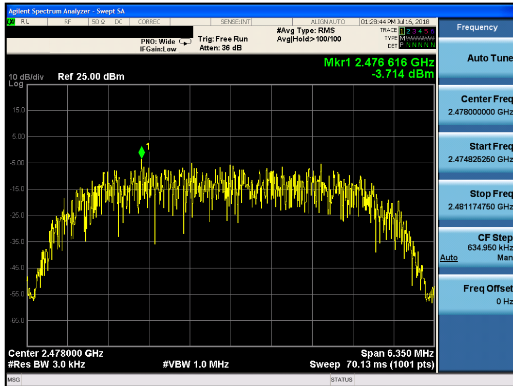
Plot 7-21. Power Spectral Density Plot (Bluetooth (HDR8, ePA), 8Mbps - Ch. 75)
