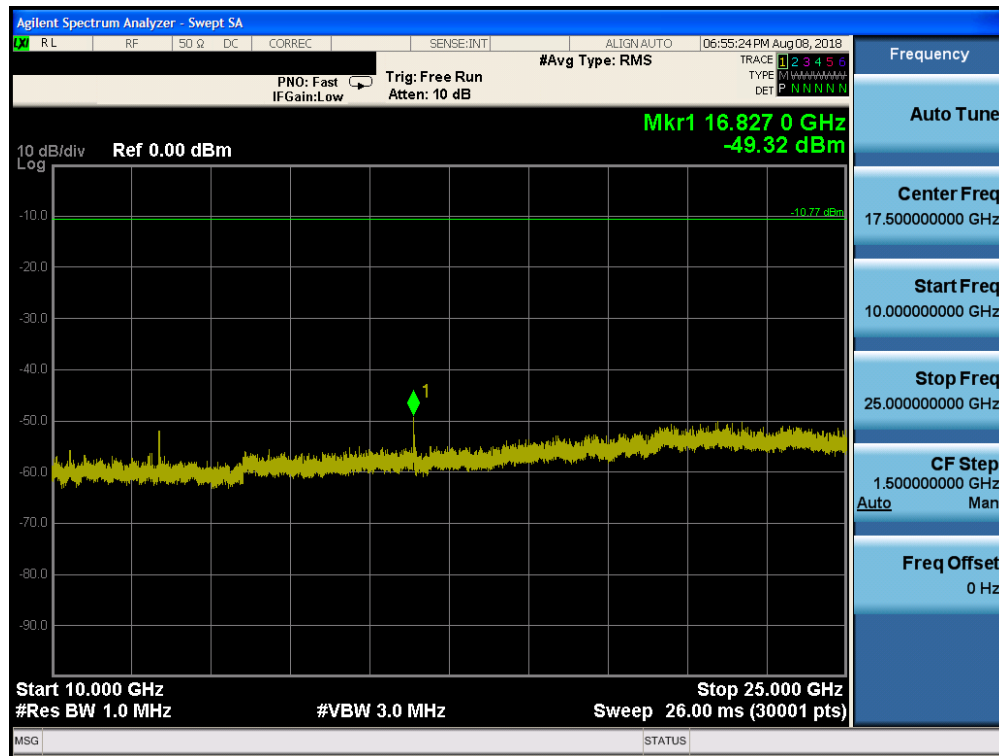
Plot 7-34. Conducted Spurious Plot (Bluetooth (HDR, ePA), 4Mbps - Ch. 1)
