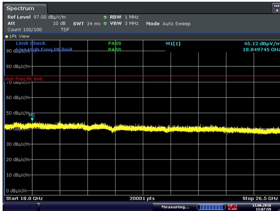
Plot 7-51. Radiated Spurious Plot above 18GHz ((HDR, ePA), 8Mbps, Pol. H)
