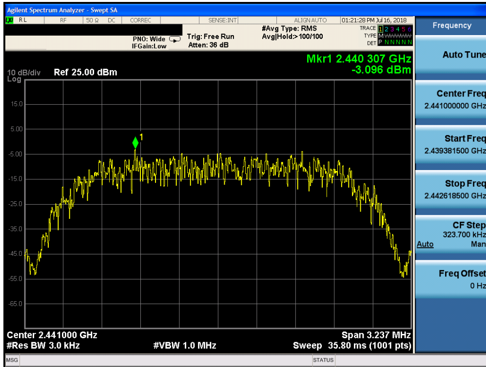
Plot 7-17. Power Spectral Density Plot (Bluetooth (HDR4, iPA), 4Mbps – Ch. 38)
