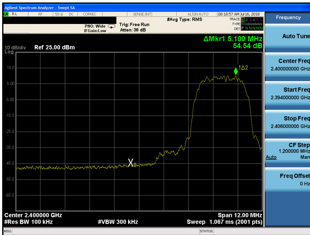
Plot 7-27. Band Edge Plot (Bluetooth (HDR, iPA), 4Mbps – Ch. 1)
