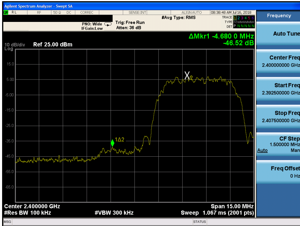
Plot 7-31. Band Edge Plot (Bluetooth (HDR, iPA), 8Mbps - Ch. 1)
