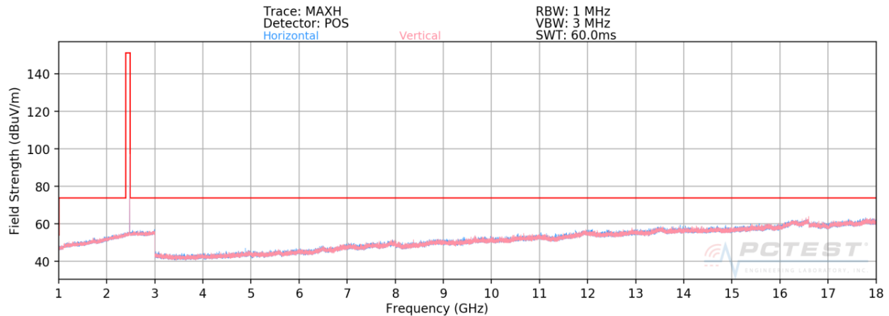
Plot 7-47. Radiated Spurious Plot ((HDR, ePA), 4Mbps – Ch. 75, Ant. Pol. H & V)
