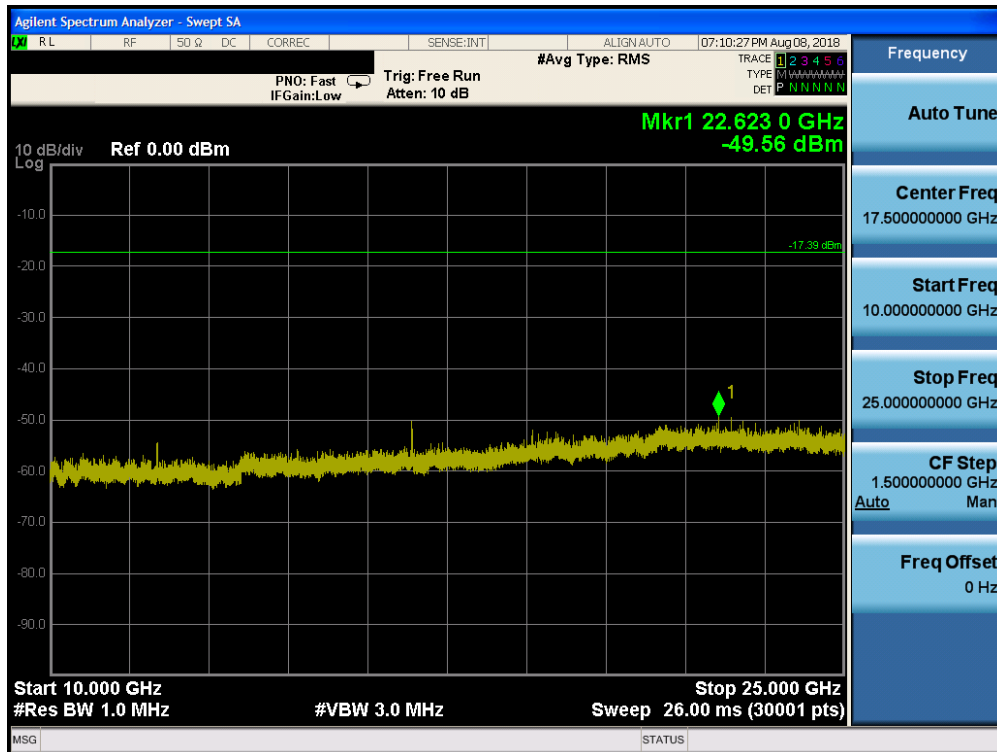
Plot 7-40. Conducted Spurious Plot (Bluetooth (HDR, ePA), 8Mbps – Ch. 1)
