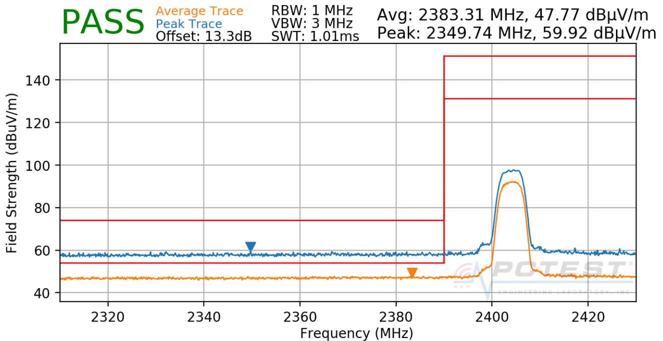
Plot 7-54. Radiated Restricted Lower Band Edge Measurement (Average & Peak)
