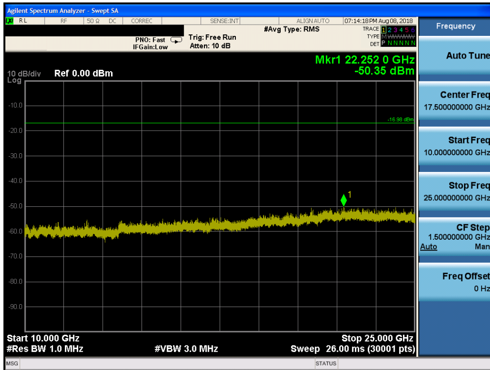
Plot 7-44. Conducted Spurious Plot (Bluetooth (HDR, ePA), 8Mbps – Ch. 75)
