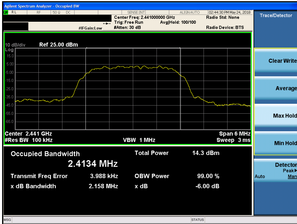
Plot 7-5. 6dB Bandwidth Plot (Bluetooth (HDR, iPA), 4Mbps – Ch. 38)
