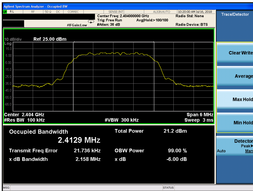
Plot 7-4. 6dB Bandwidth Plot (Bluetooth (HDR, iPA), 4Mbps – Ch. 1)
