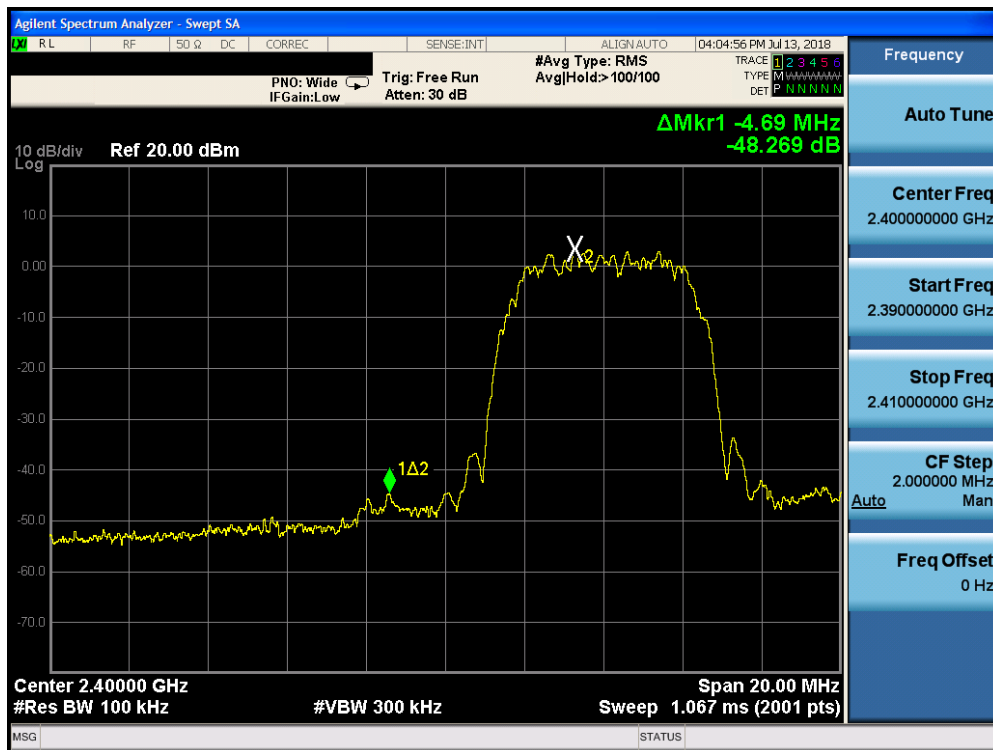
Plot 7-29. Band Edge Plot (Bluetooth (HDR, ePA), 8Mbps – Ch. 1)
