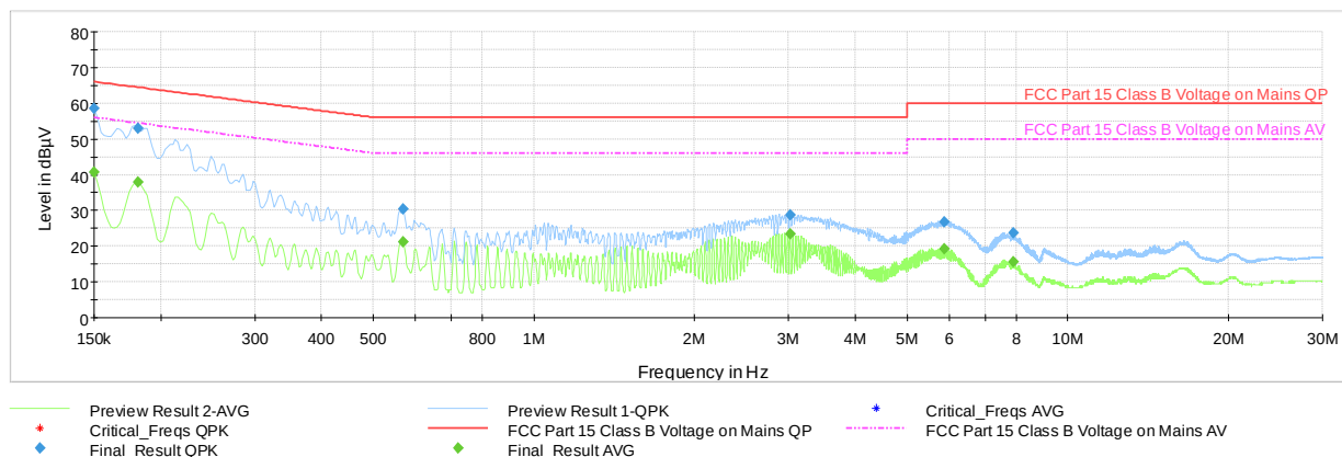
Plot 7-59. Line Conducted Plot with Bluetooth HDR (L1, with WCP + Laptop))
