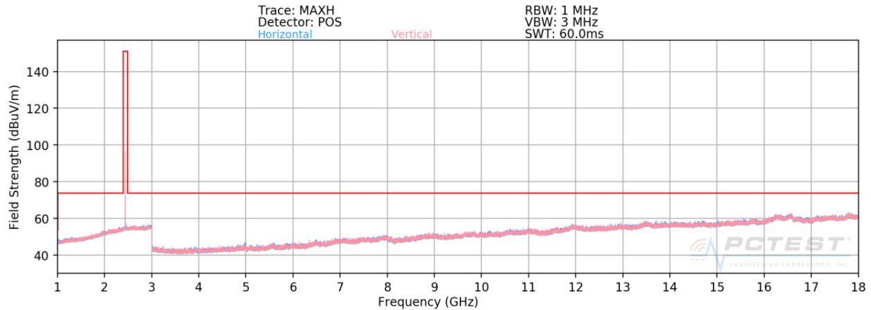
Plot 7-46. Radiated Spurious Plot ((HDR, ePA), 4Mbps – Ch. 38, Ant. Pol. H & V)
