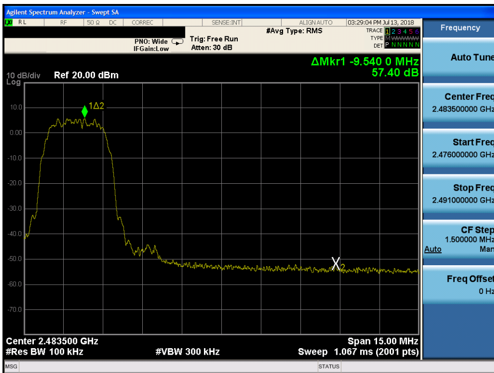
Plot 7-26. Band Edge Plot (Bluetooth (HDR, ePA), 4Mbps – Ch. 75)
