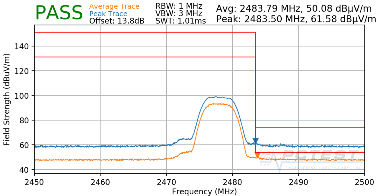
Plot 7-56. Radiated Restricted Upper Band Edge Measurement (Average & Peak)
