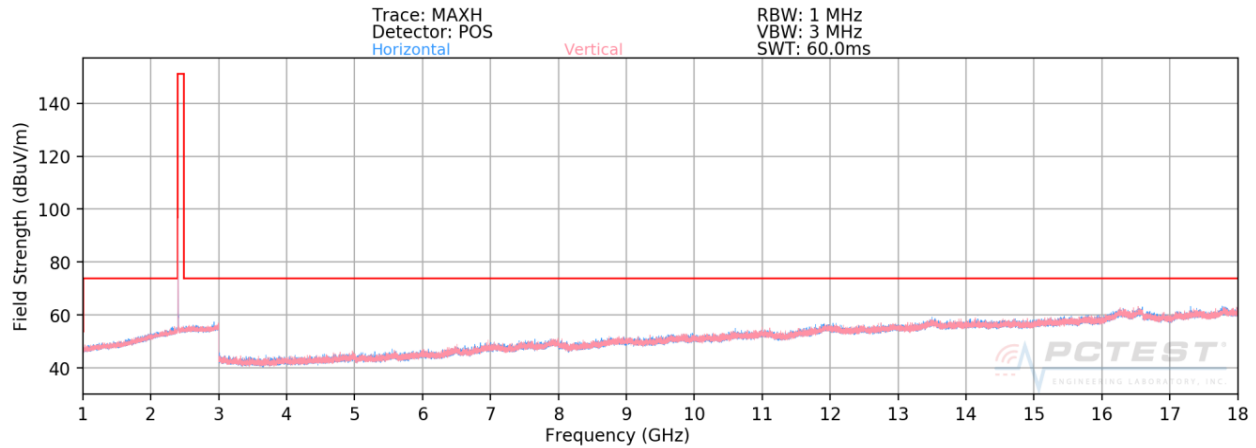
Plot 7-45. Radiated Spurious Plot ((HDR, ePA), 4Mbps – Ch. 1, Ant. Pol. H & V)
