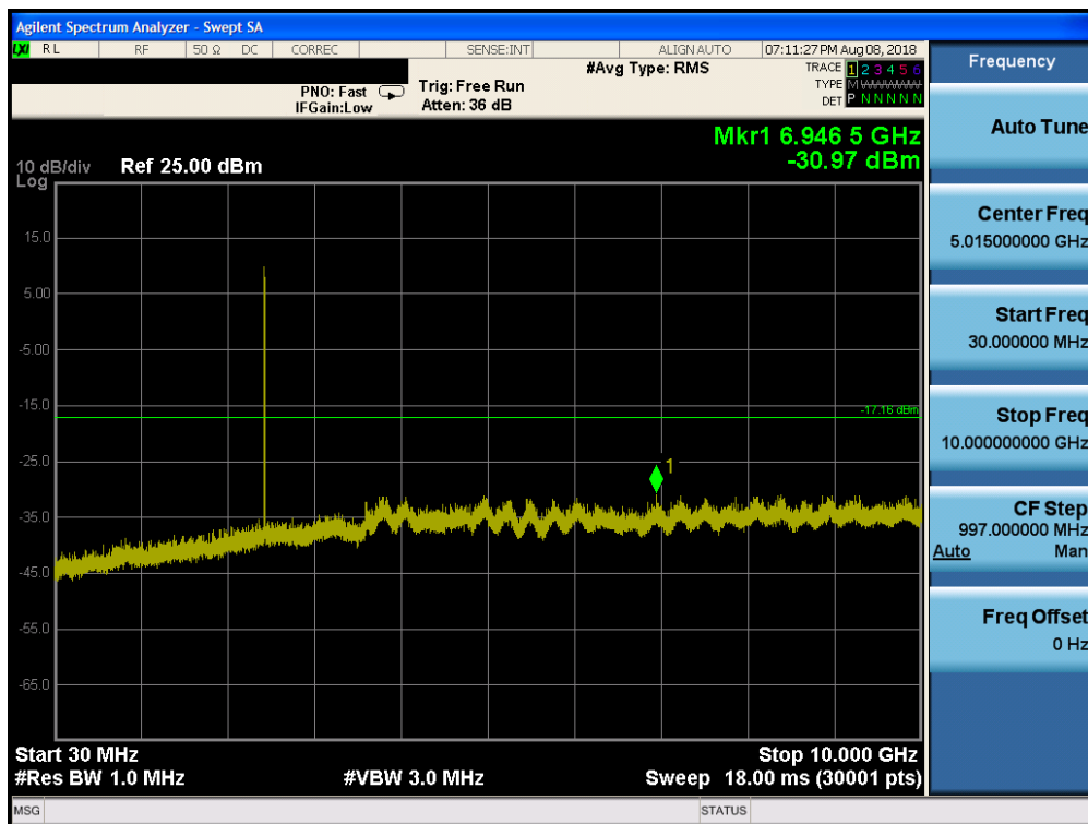
Plot 7-41. Conducted Spurious Plot (Bluetooth (HDR, ePA), 8Mbps – Ch. 38)
