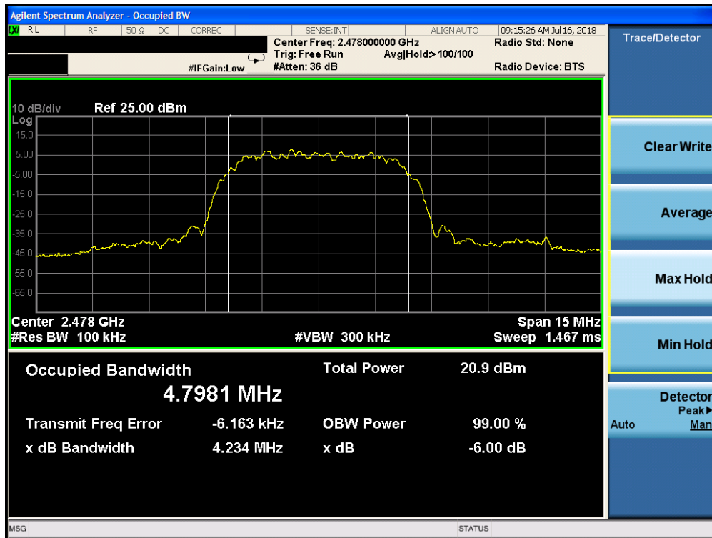
Plot 7-12. 6dB Bandwidth Plot (Bluetooth (HDR, ePA), 8Mbps – Ch. 75)
