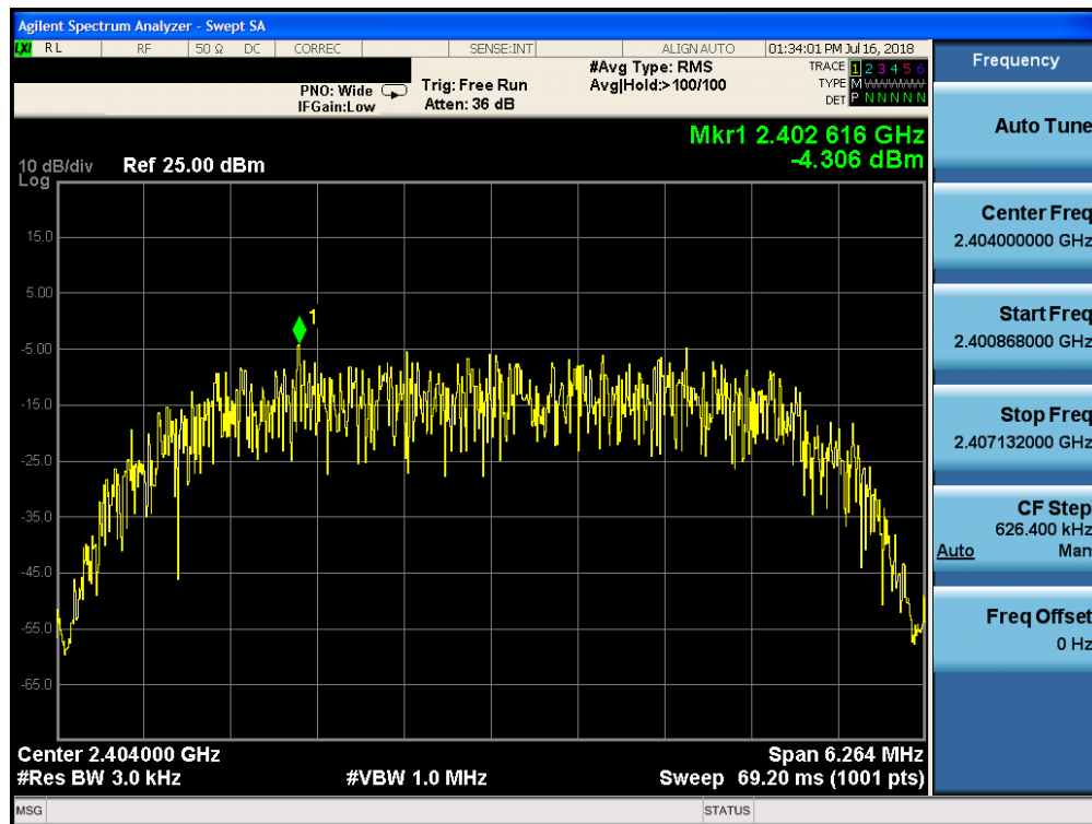
Plot 7-22. Power Spectral Density Plot (Bluetooth (HDR8, iPA), 8Mbps - Ch. 1)
