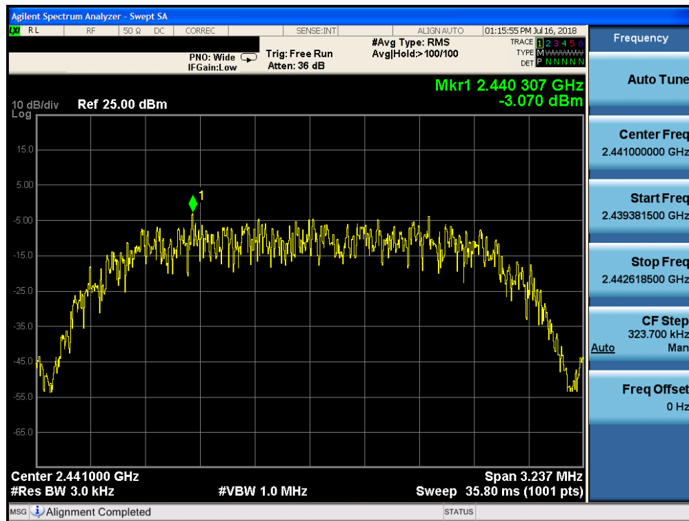
Plot 7-14. Power Spectral Density Plot (Bluetooth (HDR4, ePA), 4Mbps – Ch. 38)
