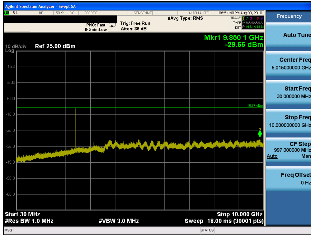
Plot 7-33. Conducted Spurious Plot (Bluetooth (HDR, ePA), 4Mbps - Ch. 1)
