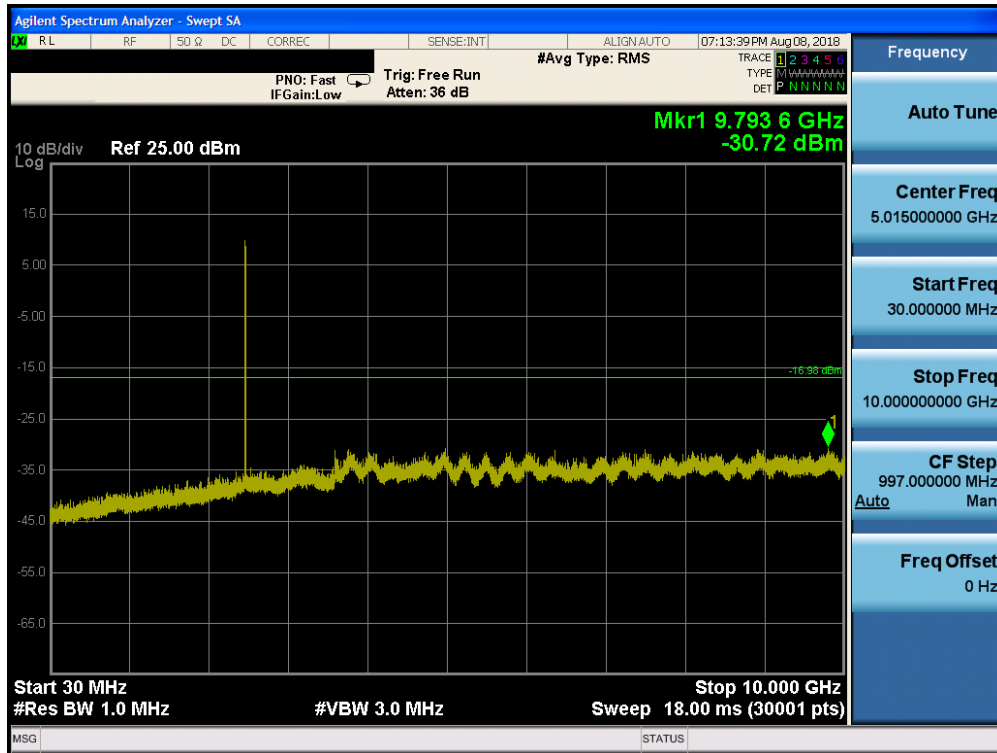
Plot 7-43. Conducted Spurious Plot (Bluetooth (HDR, ePA), 8Mbps – Ch. 75)
