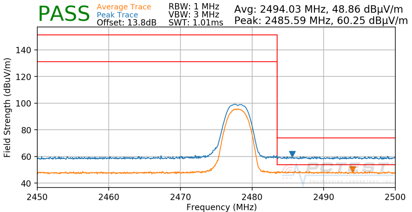
Plot 7-55. Radiated Restricted Upper Band Edge Measurement (Average & Peak)
