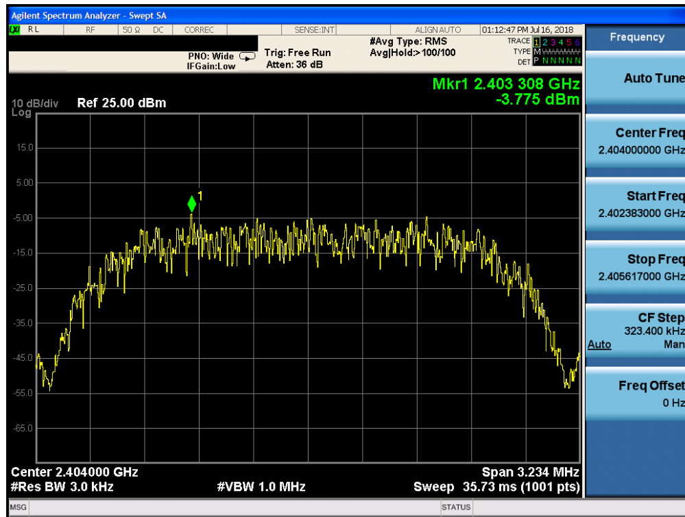
Plot 7-13. Power Spectral Density Plot (Bluetooth (HDR4, ePA), 4Mbps – Ch. 1)
