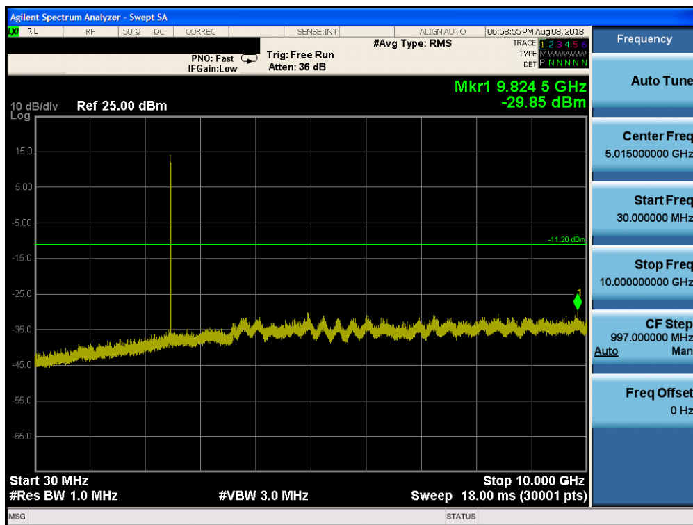
Plot 7-37. Conducted Spurious Plot (Bluetooth (HDR, ePA), 4Mbps – Ch. 75)
