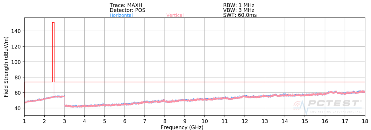
Plot 7-50. Radiated Spurious Plot ((HDR, ePA), 8Mbps – Ch. 75, Ant. Pol. H & V)
