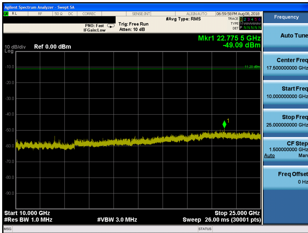
Plot 7-38. Conducted Spurious Plot (Bluetooth (HDR, ePA), 4Mbps – Ch. 75)
