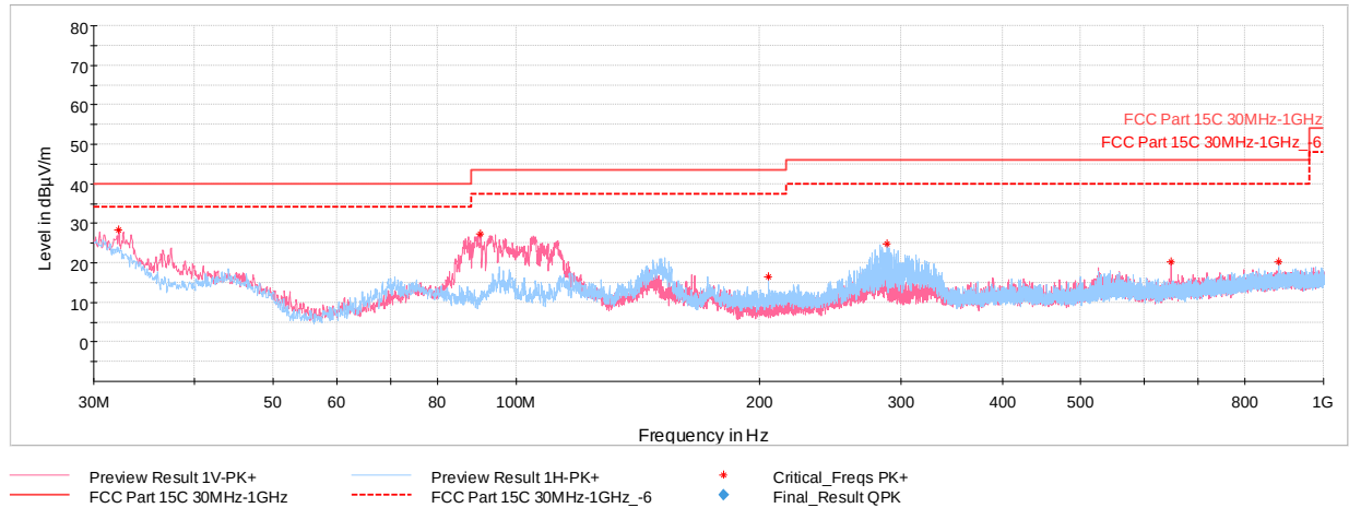
Plot 7-57. Radiated Spurious Plot below 1GHz (4Mbps, ePA, Pol. H & V, with WCP + Laptop)
