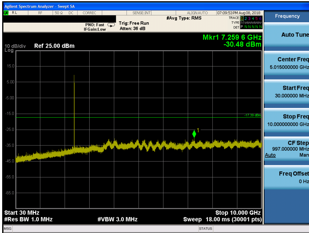
Plot 7-39. Conducted Spurious Plot (Bluetooth (HDR, ePA), 8Mbps – Ch. 1)
