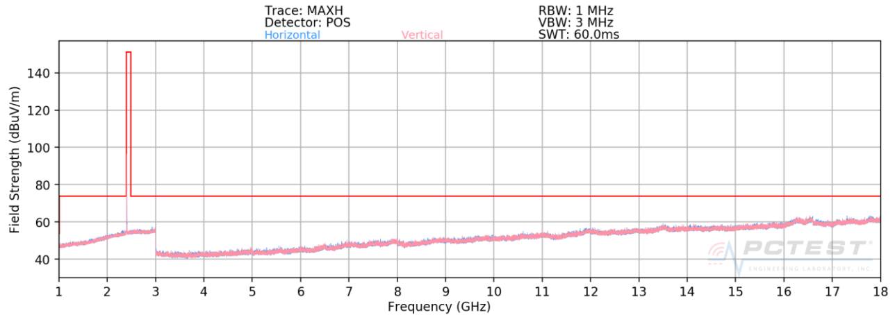
Plot 7-48. Radiated Spurious Plot ((HDR, ePA), 8Mbps – Ch. 1, Ant. Pol. H & V)
