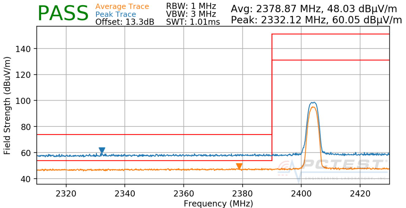
Plot 7-53. Radiated Restricted Lower Band Edge Measurement (Average & Peak)
