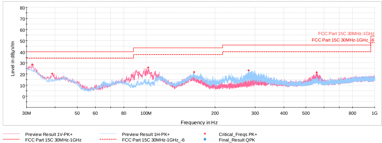
Plot 7-58. Radiated Spurious Plot below 1GHz (8Mbps, ePA, Pol. H & V, with WCP + Laptop)
