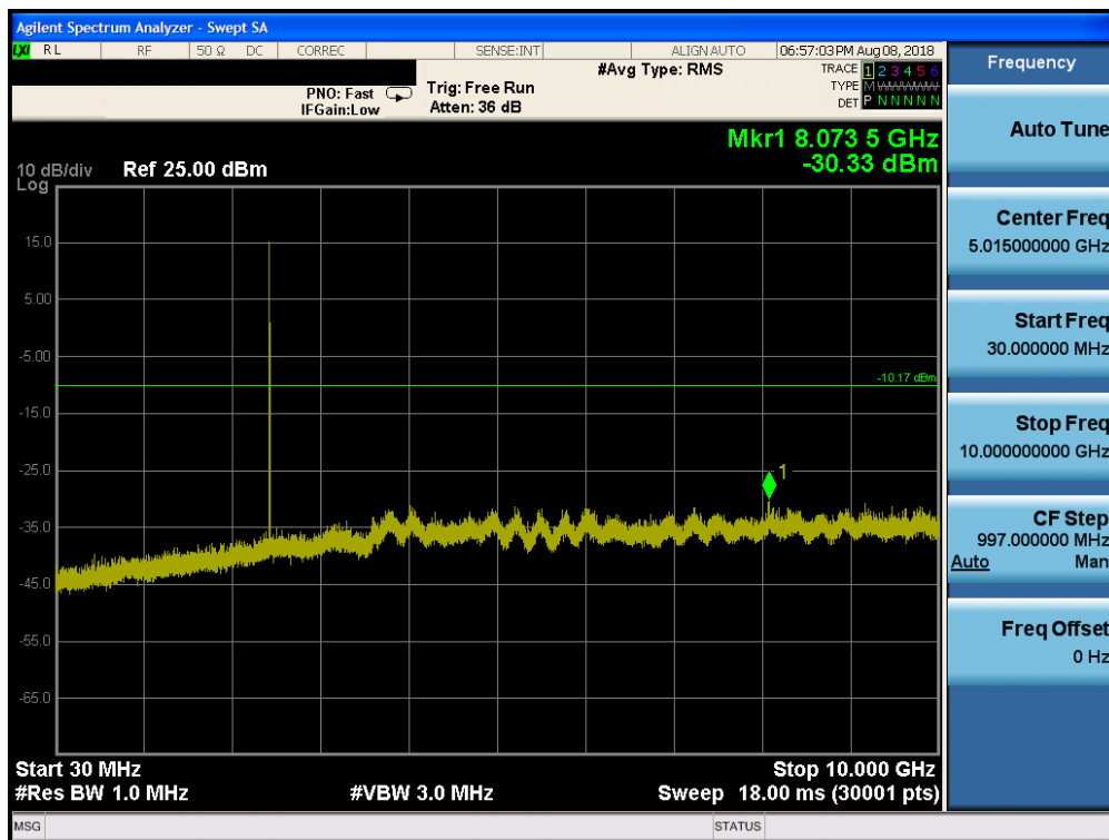
Plot 7-35. Conducted Spurious Plot (Bluetooth (HDR, ePA), 4Mbps – Ch. 38)
