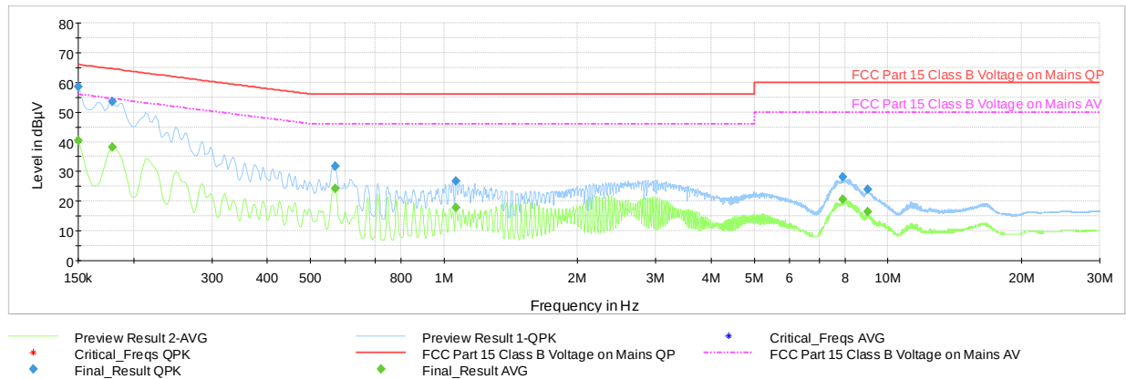
Plot 7-60. Line Conducted Plot with Bluetooth HDR (N, with WCP + Laptop))
