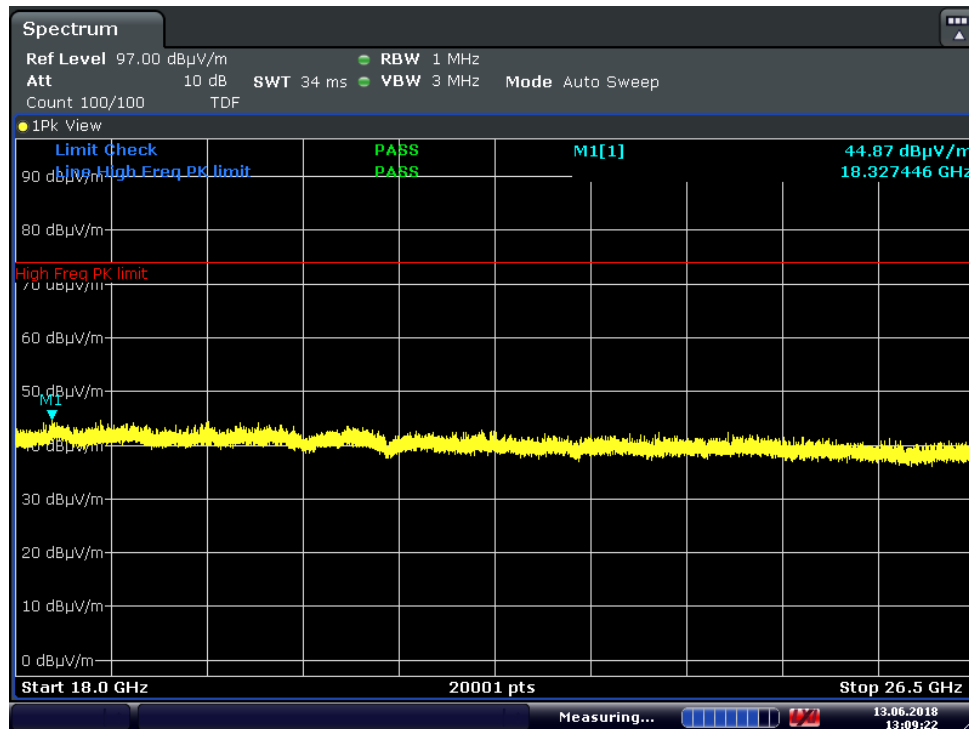
Plot 7-52. Radiated Spurious Plot above 18GHz ((HDR, ePA), 8Mbps Pol. V)
