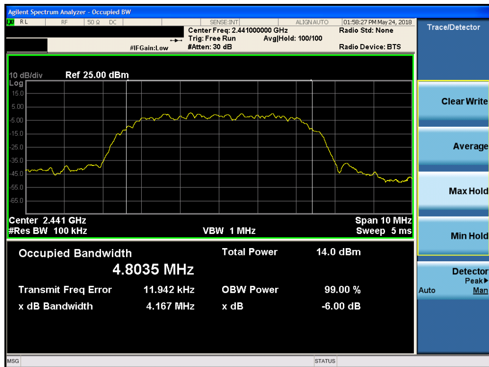
Plot 7-8. 6dB Bandwidth Plot (Bluetooth (HDR, ePA), 8Mbps – Ch. 38)
