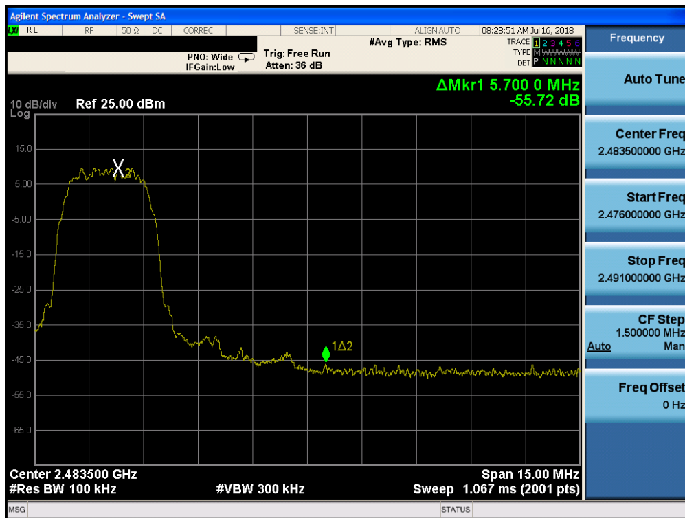
Plot 7-28. Band Edge Plot (Bluetooth (HDR, iPA), 4Mbps – Ch. 75)
