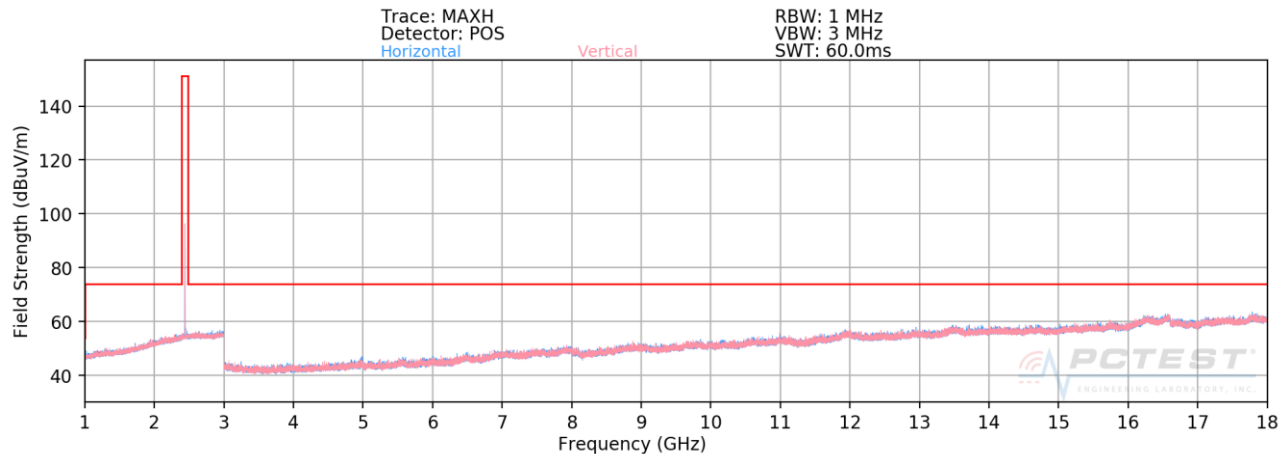
Plot 7-49. Radiated Spurious Plot ((HDR, ePA), 8Mbps – Ch. 38, Ant. Pol. H & V)
