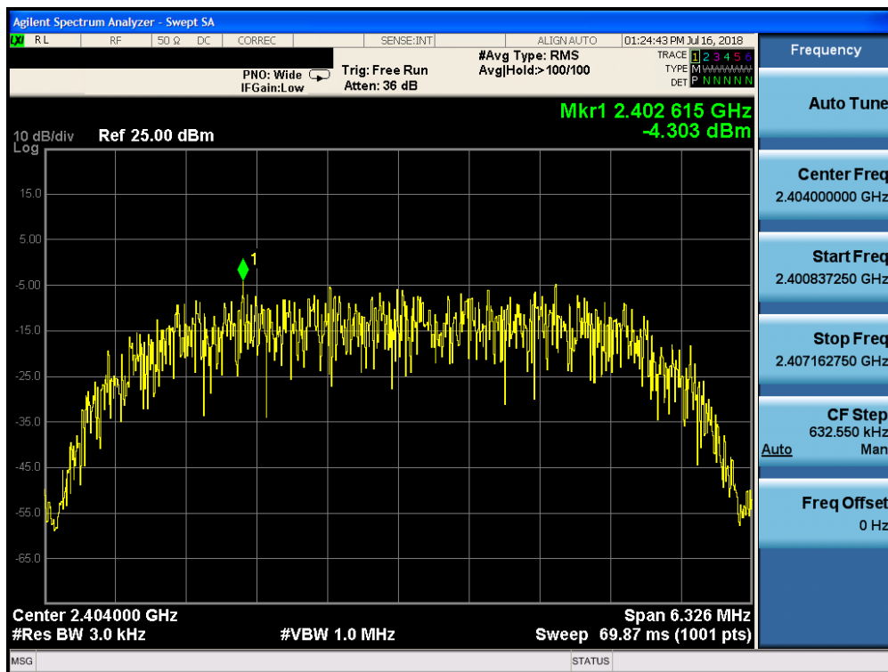
Plot 7-19. Power Spectral Density Plot (Bluetooth (HDR8, ePA), 8Mbps – Ch. 1)
