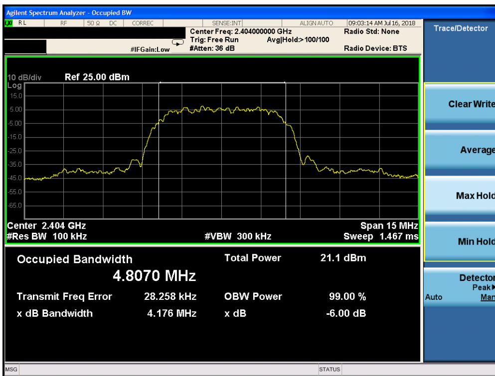
Plot 7-10. 6dB Bandwidth Plot (Bluetooth (HDR, ePA), 8Mbps – Ch. 1)
