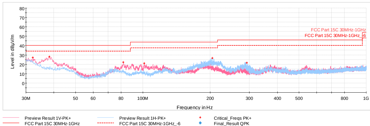
Plot 7-54. Radiated Spurious Plot below 1GHz (1Mbps, ePA, Pol. H & V, with WCP + Laptop)
