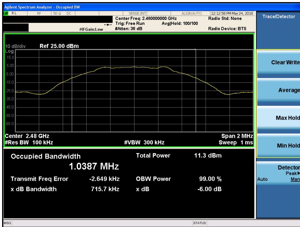
Plot 7-6. 6dB Bandwidth Plot (Bluetooth (LE), iPA, 1Mbps – Ch. 39)
