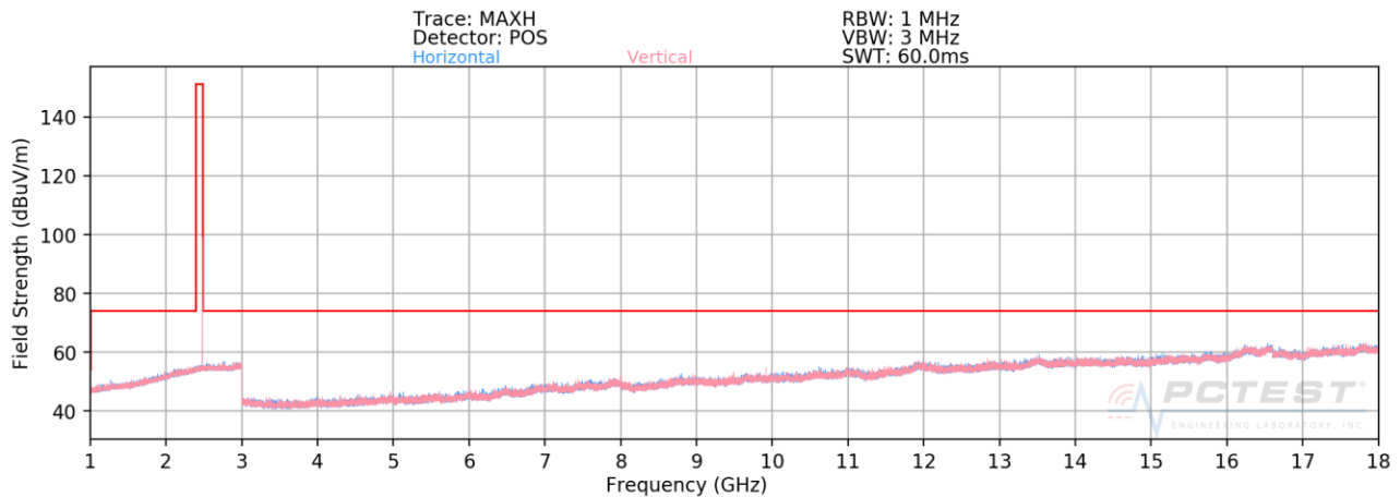
Plot 7-47. Radiated Spurious Plot Above 1GHz (1Mbps, ePA – Ch. 39, Ant. Pol. H & V)
