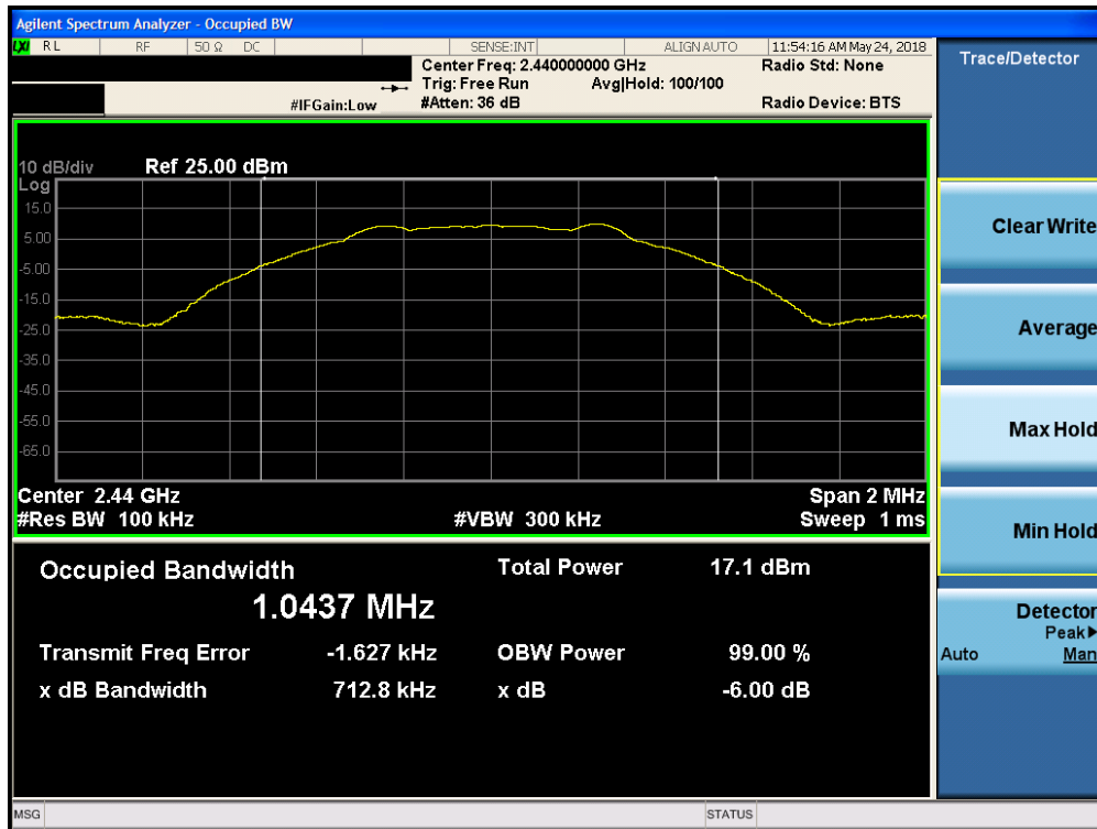
Plot 7-2. 6dB Bandwidth Plot (Bluetooth (LE), ePA, 1Mbps – Ch. 19)
