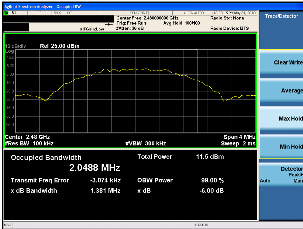
Plot 7-12. 6dB Bandwidth Plot (Bluetooth (LE), iPA, 2Mbps – Ch. 39)
