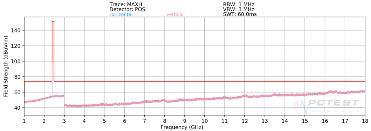
Plot 7-45. Radiated Spurious Plot Above 1GHz (1Mbps, ePA – Ch. 0, Ant. Pol. H & V)
