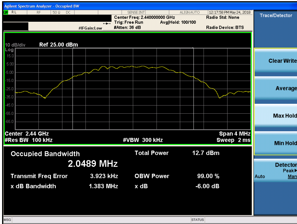
Plot 7-11. 6dB Bandwidth Plot (Bluetooth (LE), iPA, 2Mbps – Ch. 19)
