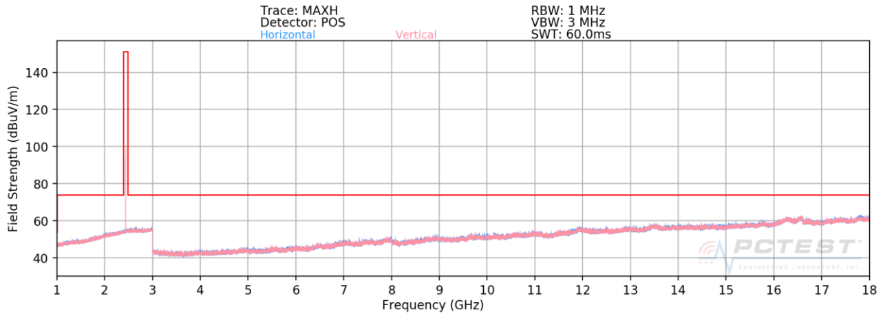
Plot 7-46. Radiated Spurious Plot Above 1GHz (1Mbps, ePA – Ch. 19, Ant. Pol. H & V)
