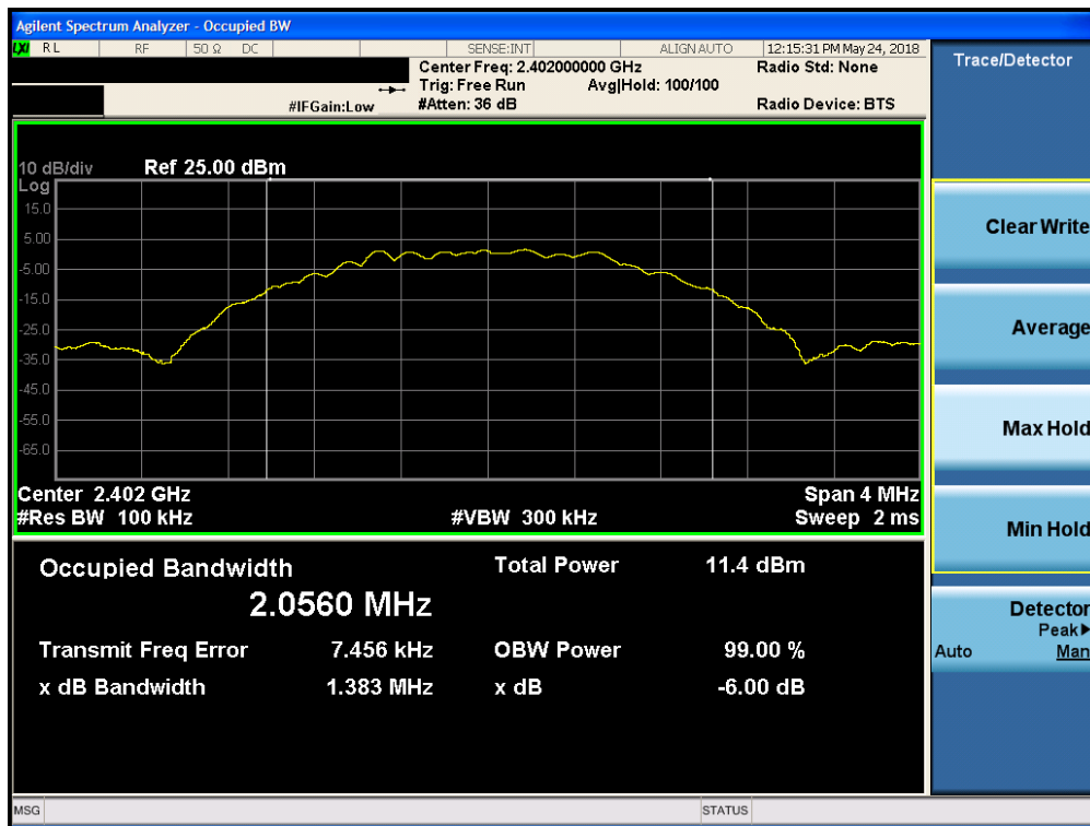
Plot 7-10. 6dB Bandwidth Plot (Bluetooth (LE), iPA, 2Mbps – Ch. 0)
