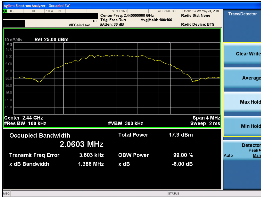
Plot 7-8. 6dB Bandwidth Plot (Bluetooth (LE), ePA, 2Mbps – Ch. 19)
