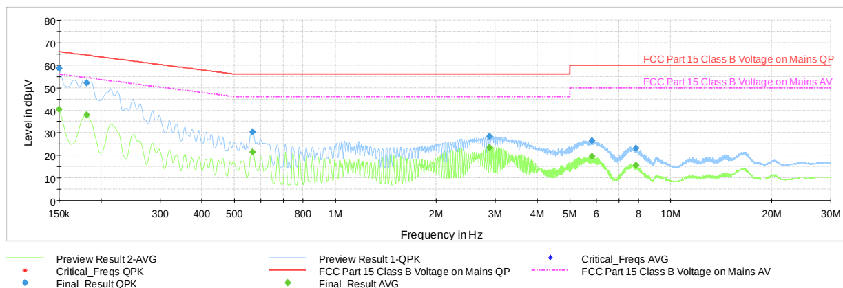
Plot 7-55. Line Conducted Plot with Bluetooth LE (L1, with WCP + Laptop)
