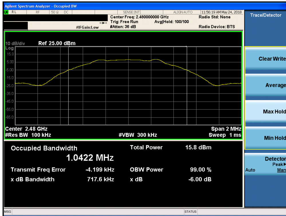
Plot 7-3. 6dB Bandwidth Plot (Bluetooth (LE), ePA, 1Mbps – Ch. 39)
