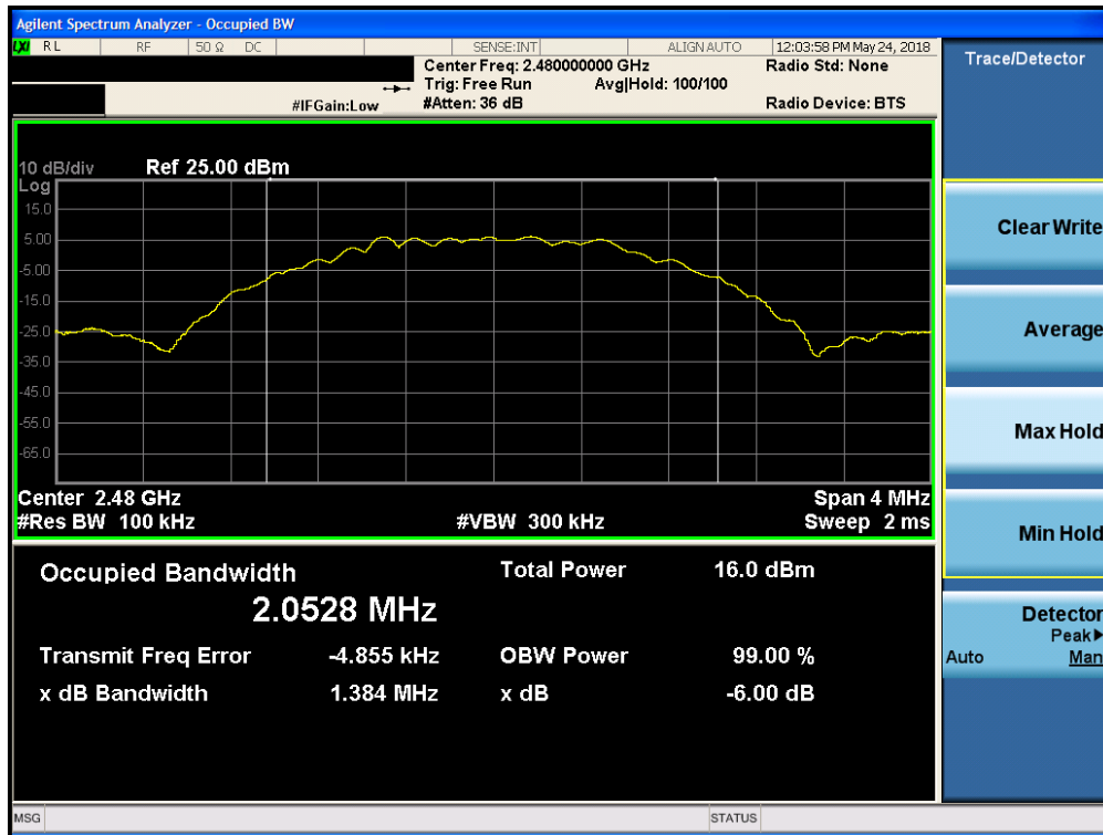
Plot 7-9. 6dB Bandwidth Plot (Bluetooth (LE), ePA, 2Mbps – Ch. 39)
