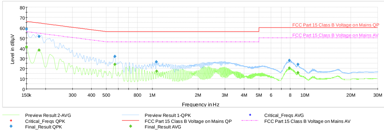
Plot 7-56. Line Conducted Plot with Bluetooth LE (N, with WCP + Laptop)
