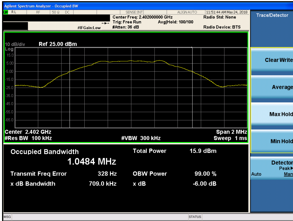
Plot 7-1. 6dB Bandwidth Plot (Bluetooth (LE), ePA, 1Mbps – Ch. 0)
