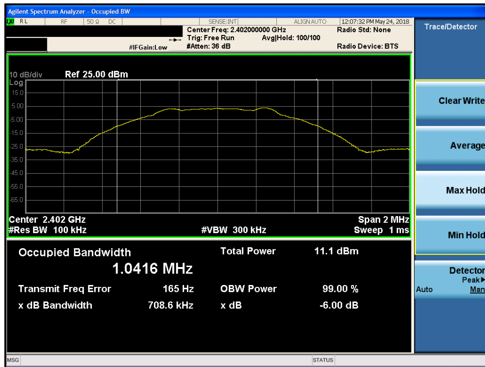
Plot 7-4. 6dB Bandwidth Plot (Bluetooth (LE), iPA, 1Mbps – Ch. 0)
