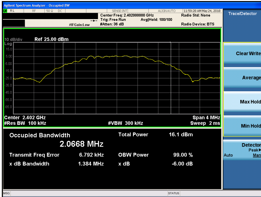
Plot 7-7. 6dB Bandwidth Plot (Bluetooth (LE), ePA, 2Mbps – Ch. 0)
