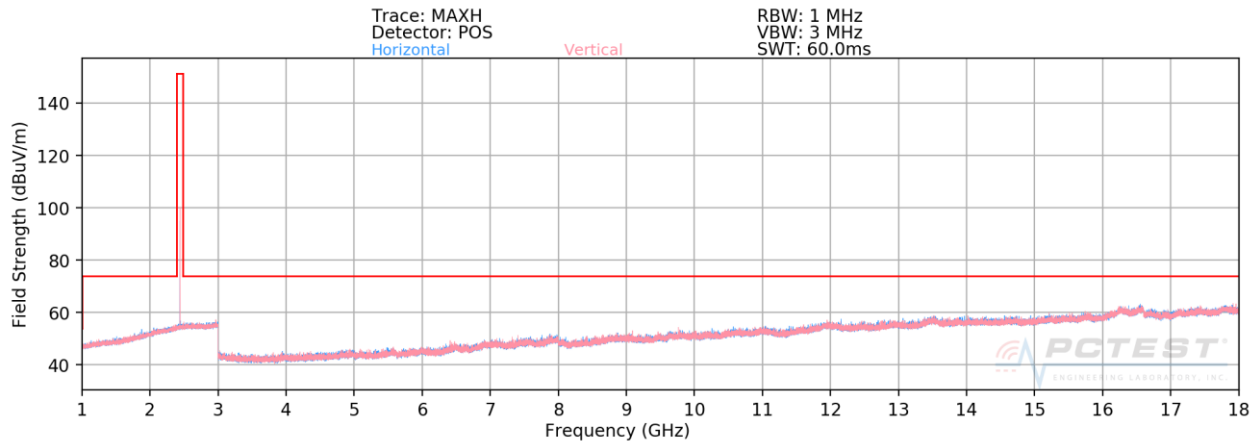
Plot 7-62. Radiated Spurious Plot above 1GHz (BT GFSK ePA – Ch. 39)
