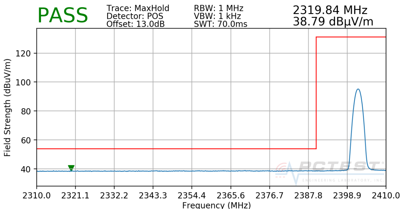
Plot 7-68. Radiated Restricted Lower Band Edge Measurement (Average)
