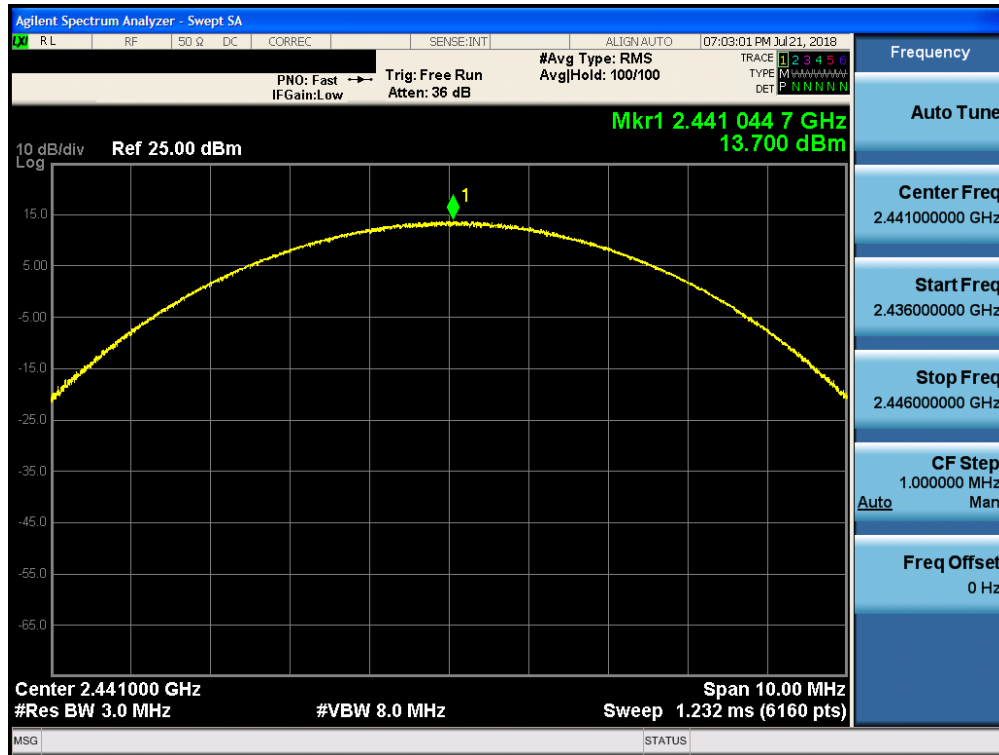
Plot 7-23. Peak Conducted Plot (Bluetooth, 8DPSK, iPA – Ch. 39)
