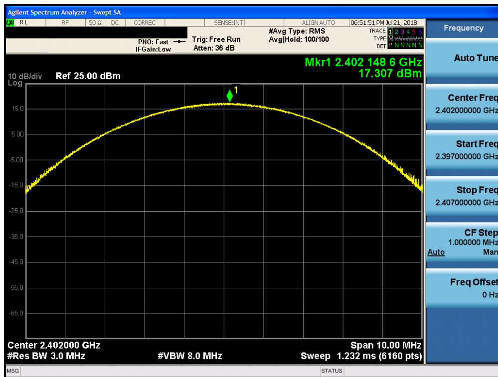
Plot 7-19. Peak Conducted Plot (Bluetooth, 8DPSK, ePA – Ch. 0)
