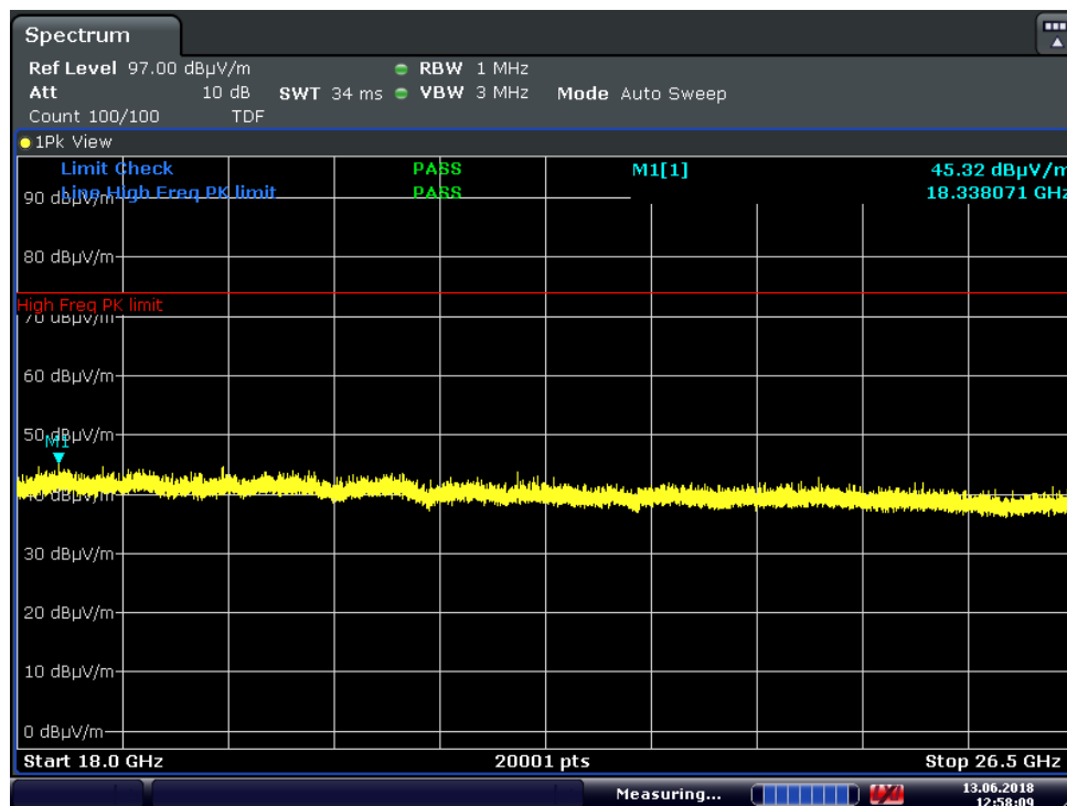
Plot 7-65. Radiated Spurious Plot above 18GHz (GFSK ePA, Ant. Pol. V)
