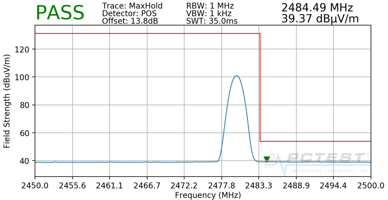
Plot 7-70. Radiated Restricted Upper Band Edge Measurement (Average)
