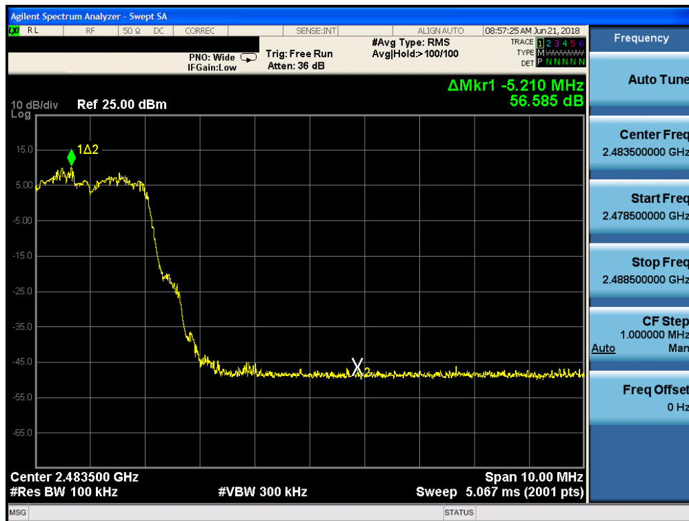
Plot 7-40. Band Edge Plot (Bluetooth with Hopping Enabled, 8DPSK, iPA)
