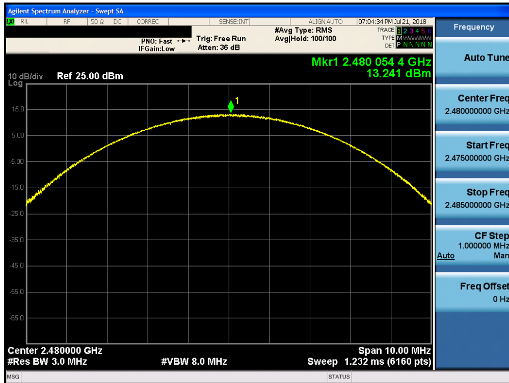
Plot 7-24. Peak Conducted Plot (Bluetooth, 8DPSK, iPA – Ch. 78)
