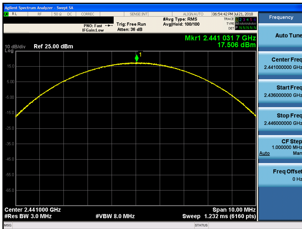
Plot 7-20. Peak Conducted Plot (Bluetooth, 8DPSK, ePA – Ch. 39)
