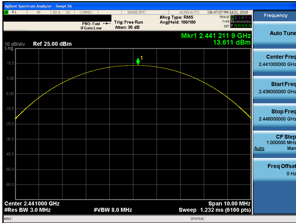
Plot 7-17. Peak Conducted Plot (Bluetooth, GFSK, iPA – Ch. 39)
