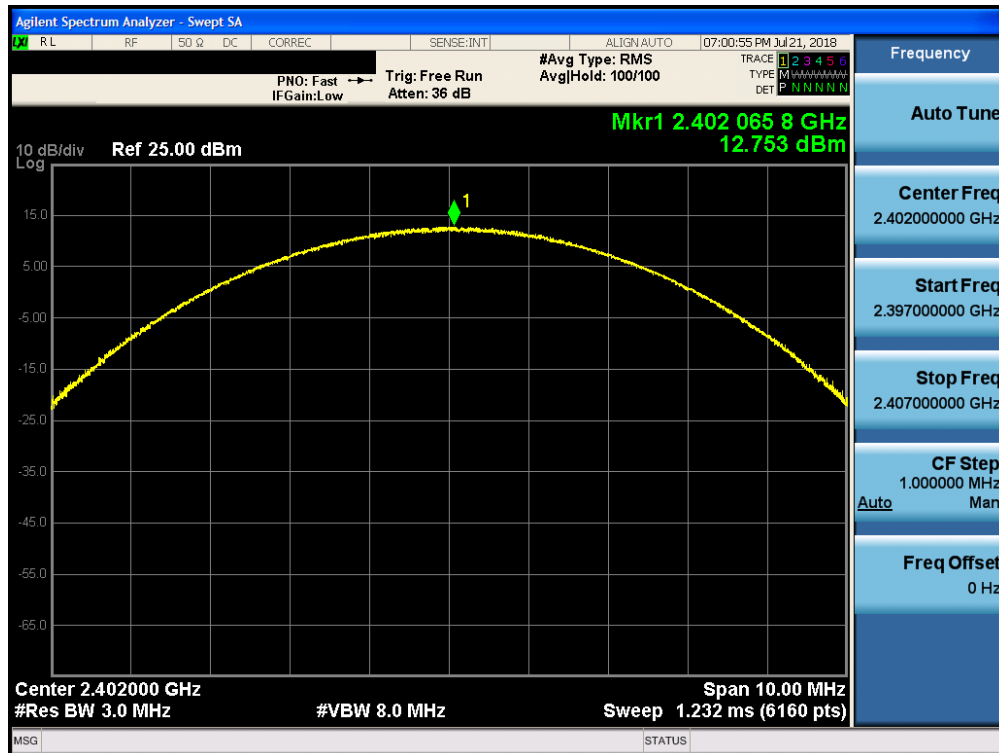
Plot 7-22. Peak Conducted Plot (Bluetooth, 8DPSK, iPA – Ch. 0)
