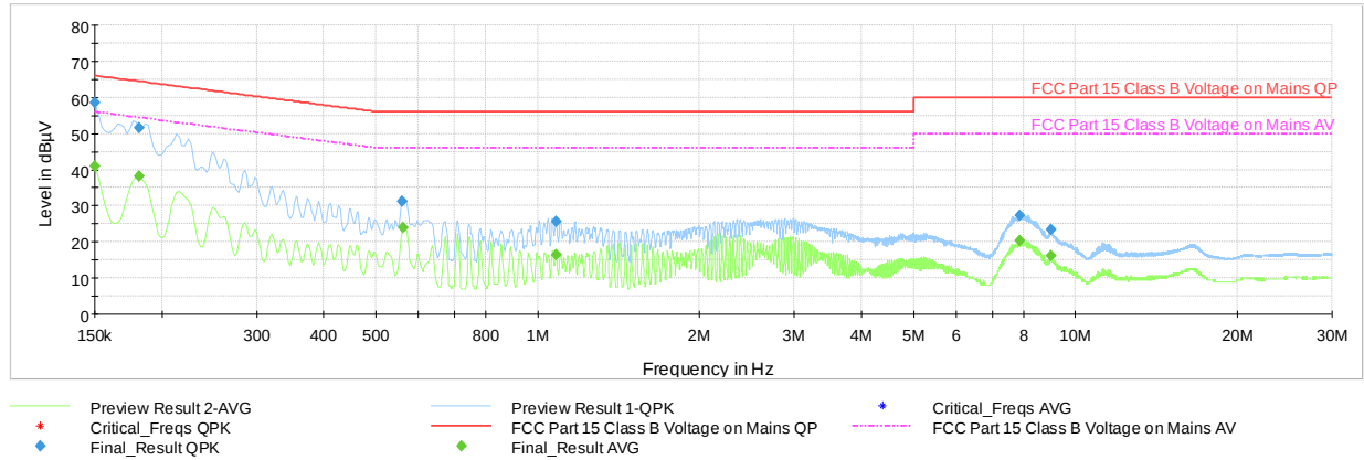
Plot 7-76. Line-Conducted Test Plot (N)
