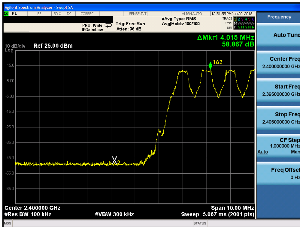
Plot 7-31. Band Edge Plot (Bluetooth with Hopping Enabled, GFSK, iPA)
