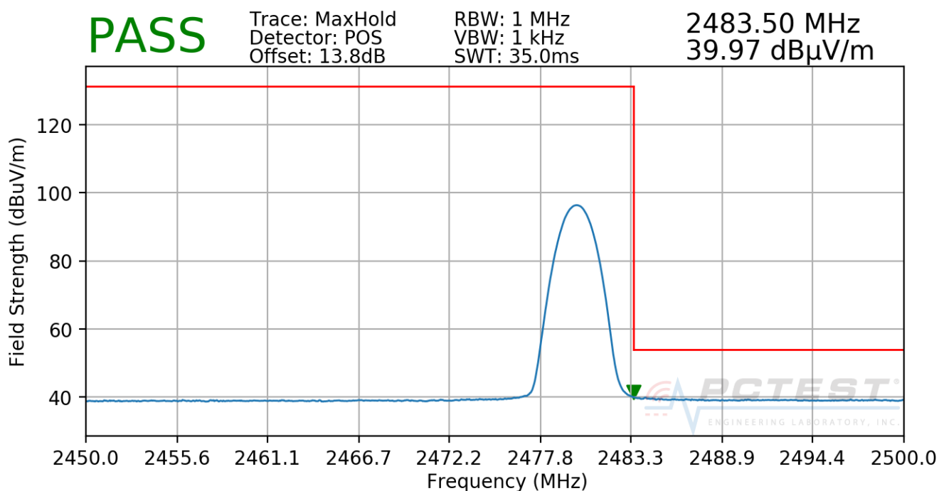
Plot 7-72. Radiated Restricted Upper Band Edge Measurement (Average)
