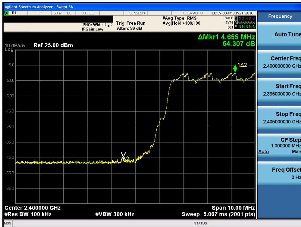
Plot 7-39. Band Edge Plot (Bluetooth with Hopping Enabled, 8DPSK, iPA)
