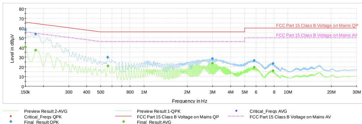
Plot 7-75. Line-Conducted Test Plot (L1)
