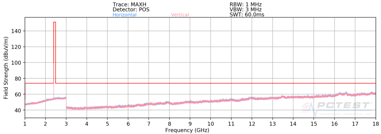
Plot 7-61. Radiated Spurious Plot above 1GHz (BT GFSK ePA – Ch. 0)
