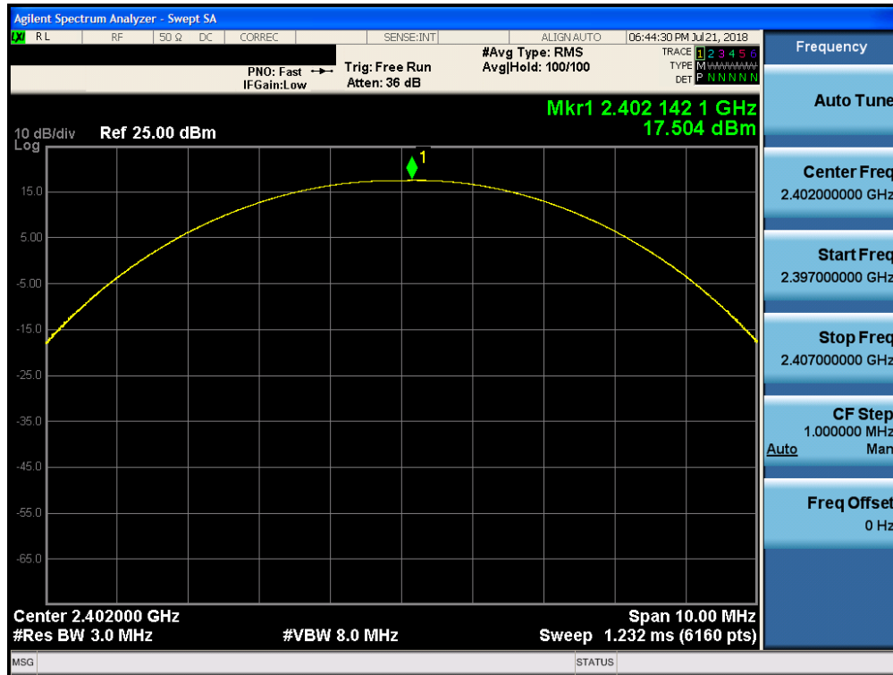
Plot 7-13. Peak Conducted Plot (Bluetooth, GFSK, ePA – Ch. 0)
