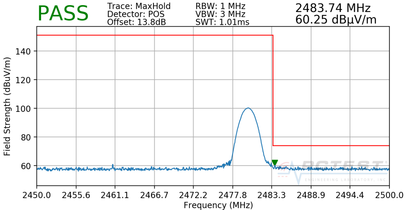
Plot 7-73. Radiated Restricted Upper Band Edge Measurement (Peak)
