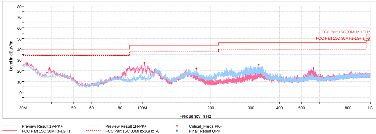
Plot 7-74. Radiated Spurious Plot below 1GHz (GFSK ePA, Pol. H & V, with WCP + Laptop)
