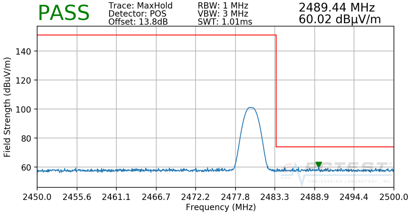
Plot 7-71. Radiated Restricted Upper Band Edge Measurement (Peak)
