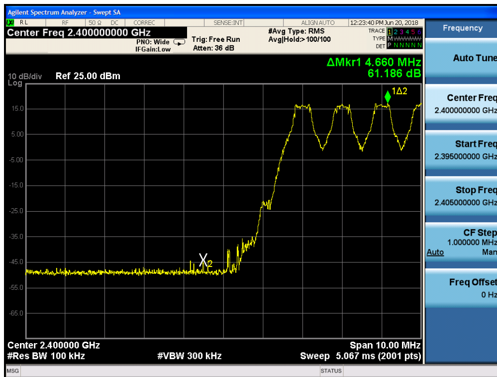
Plot 7-27. Band Edge Plot (Bluetooth with Hopping Enabled, GFSK, ePA)
