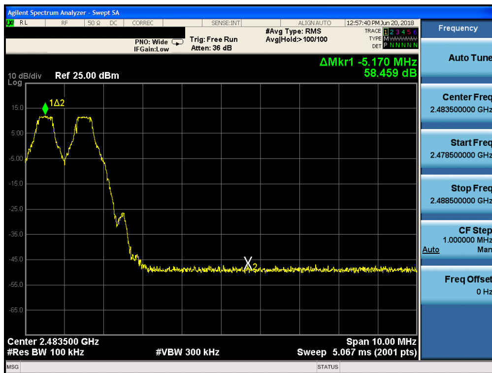
Plot 7-32. Band Edge Plot (Bluetooth with Hopping Enabled, GFSK, iPA)
