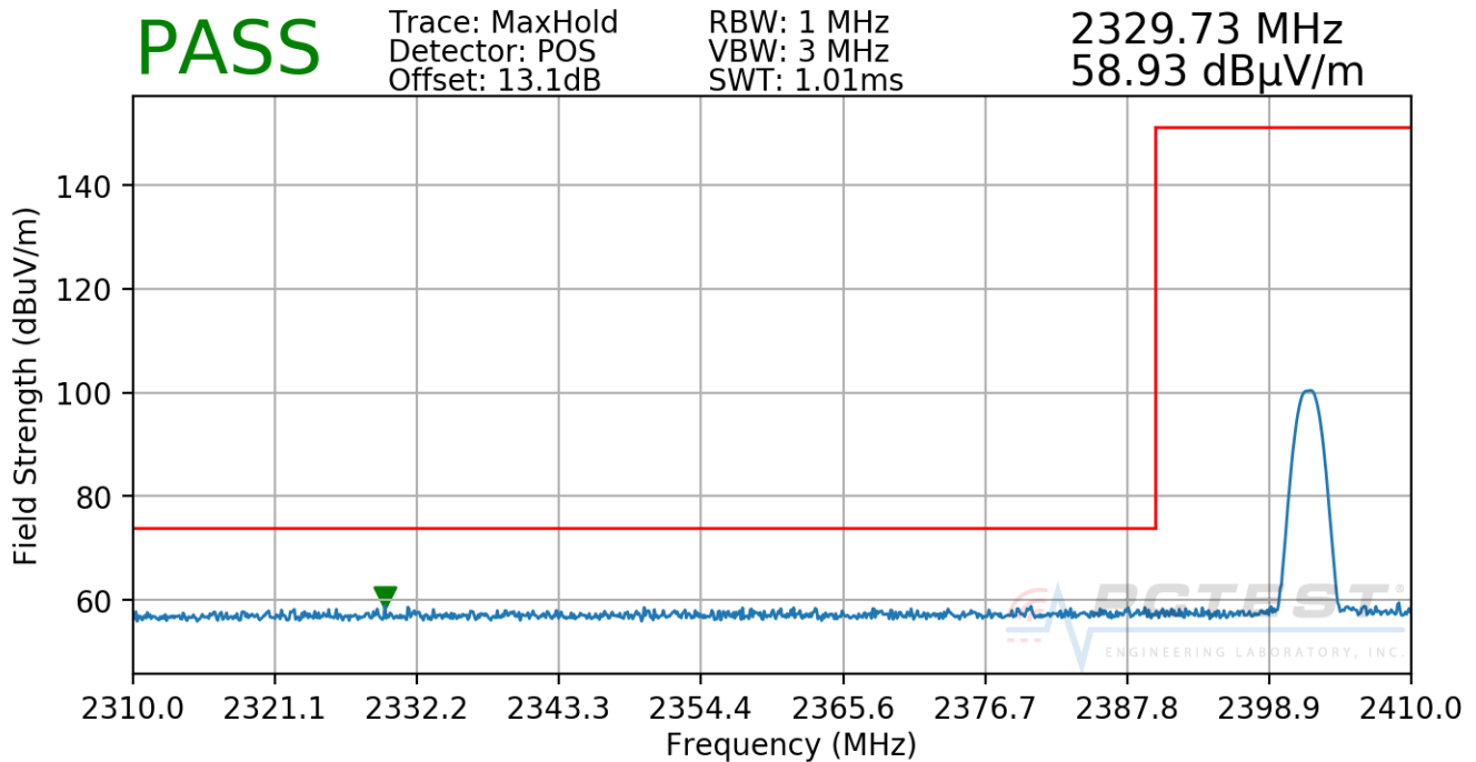
Plot 7-67. Radiated Restricted Lower Band Edge Measurement (Peak)
