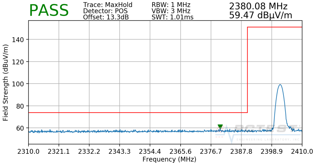
Plot 7-69. Radiated Restricted Lower Band Edge Measurement (Peak)
