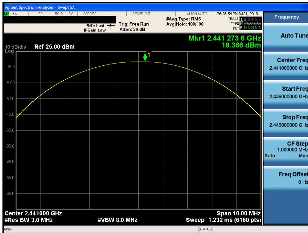
Plot 7-14. Peak Conducted Plot (Bluetooth, GFSK, ePA – Ch. 39)
