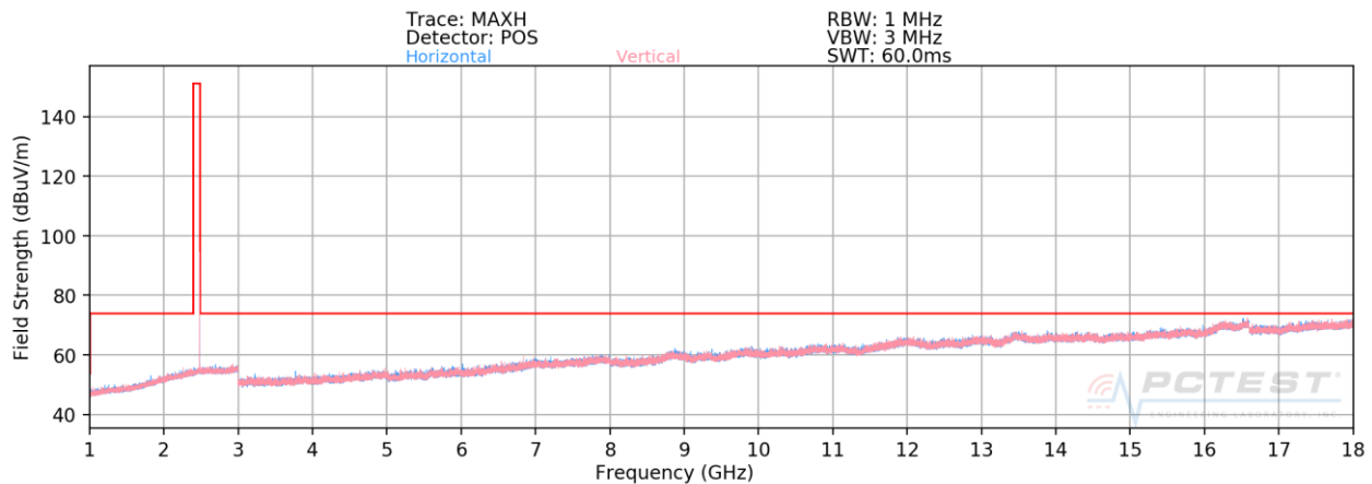
Plot 7-63. Radiated Spurious Plot above 1GHz (BT GFSK ePA – Ch. 78)
