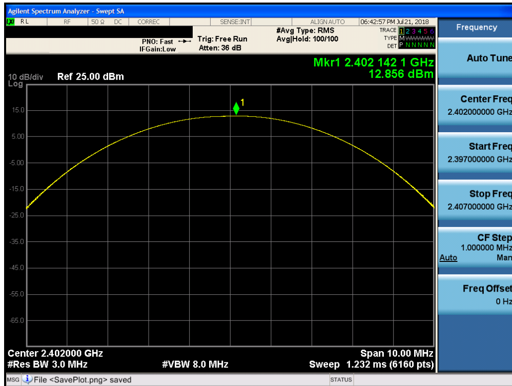
Plot 7-16. Peak Conducted Plot (Bluetooth, GFSK, iPA – Ch. 0)
