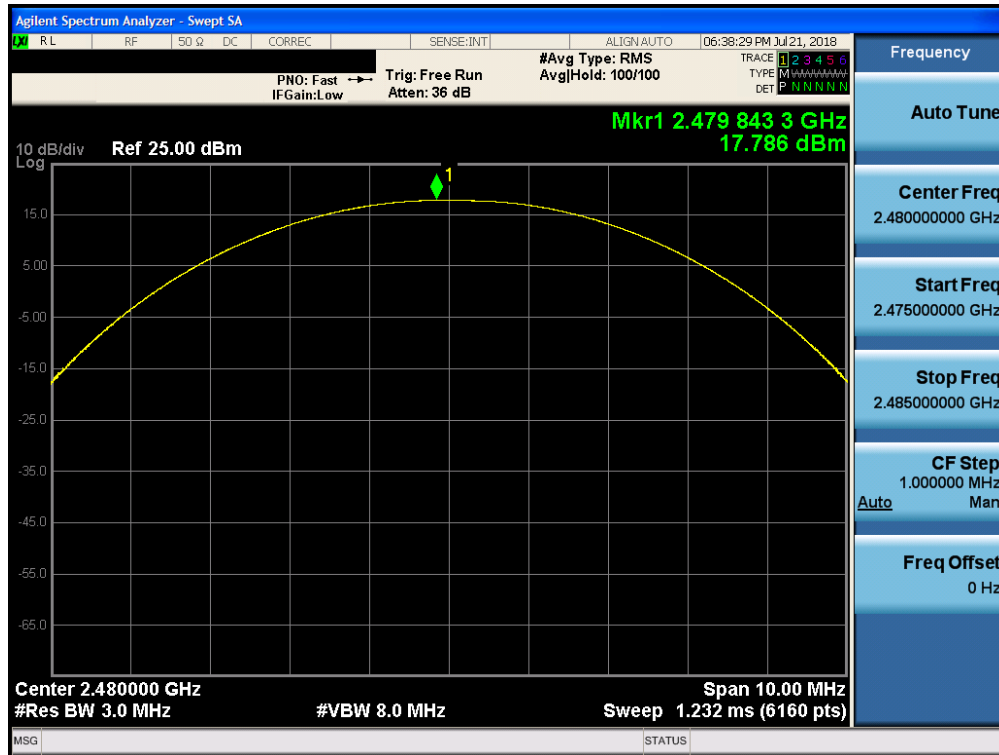
Plot 7-15. Peak Conducted Plot (Bluetooth, GFSK, ePA – Ch. 78)
