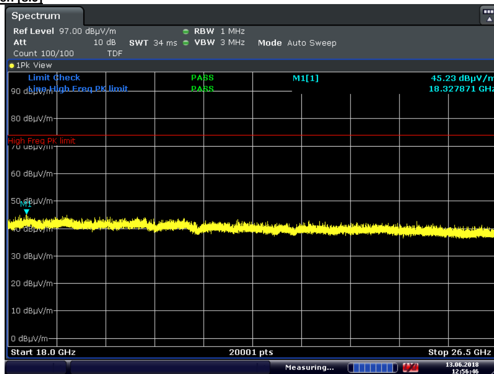
Plot 7-64. Radiated Spurious Plot above 18GHz (GFSK ePA, Ant. Pol. H)
