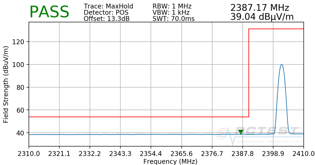
Plot 7-66. Radiated Restricted Lower Band Edge Measurement (Average)
