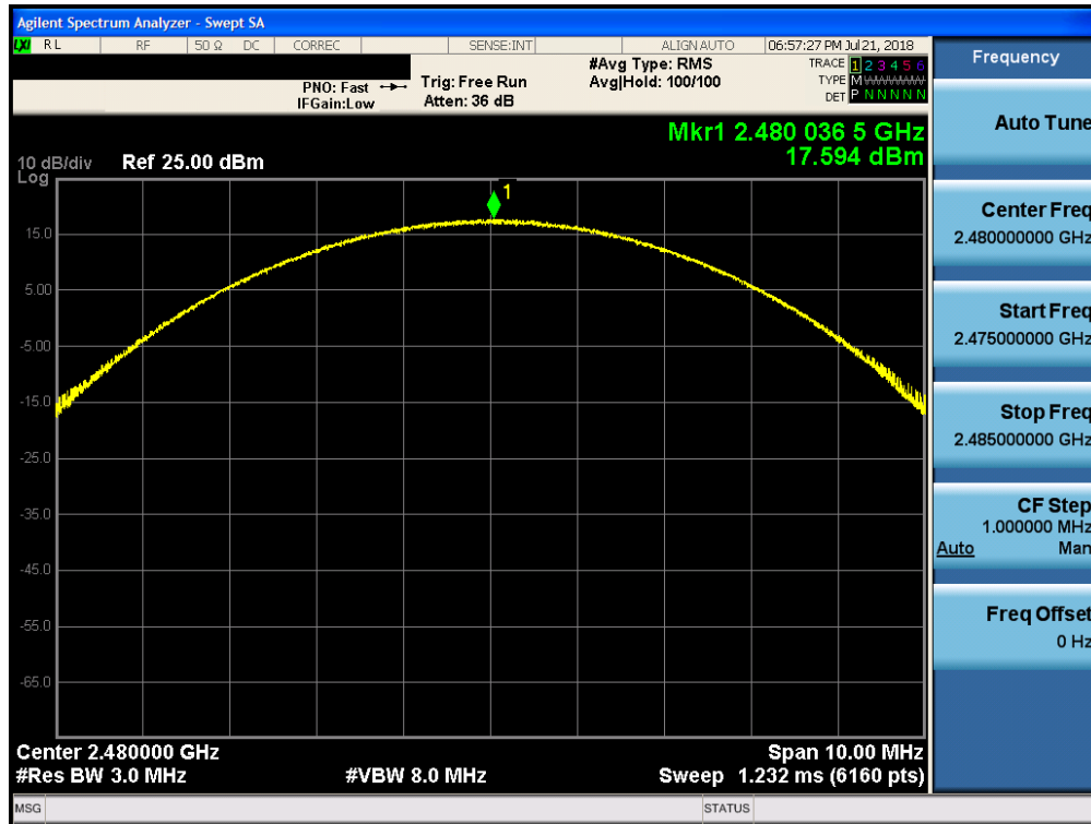
Plot 7-21. Peak Conducted Plot (Bluetooth, 8DPSK, ePA – Ch. 78)
