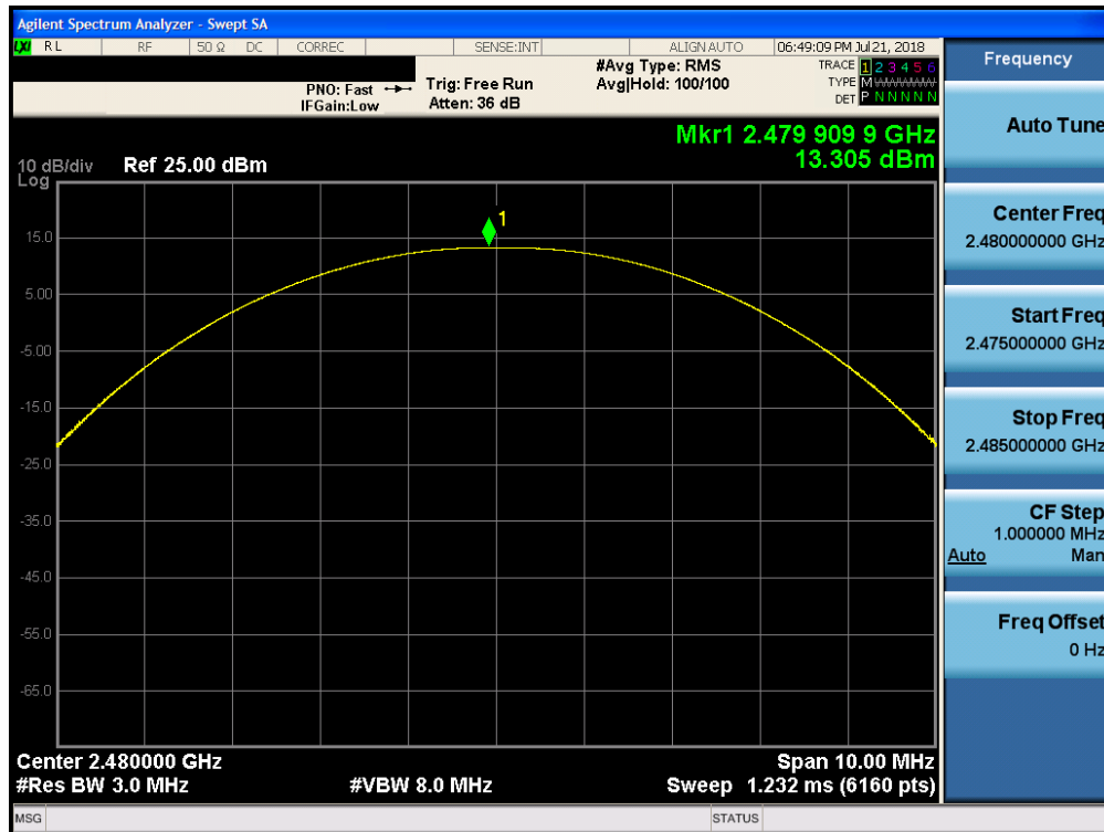
Plot 7-18. Peak Conducted Plot (Bluetooth, GFSK, iPA – Ch. 78)
