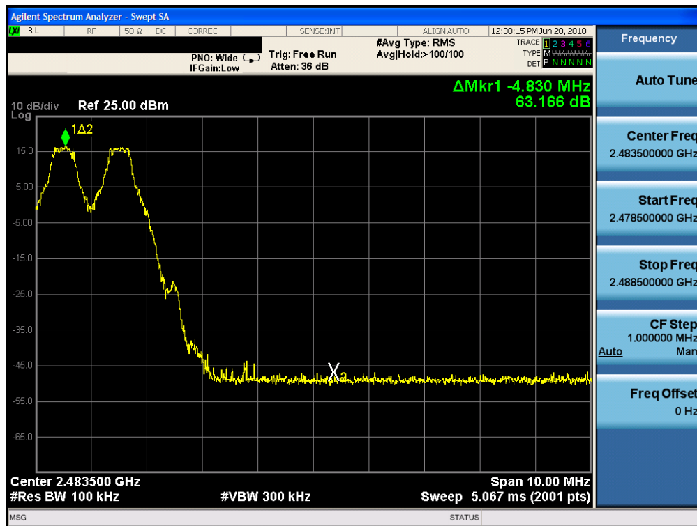
Plot 7-28. Band Edge Plot (Bluetooth with Hopping Enabled, GFSK, ePA)
