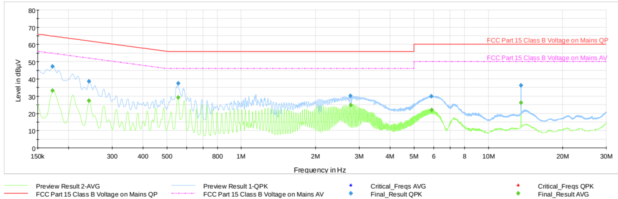
Plot 7-7. Line-Conducted Test Plot (L1, with WCP + Laptop)
