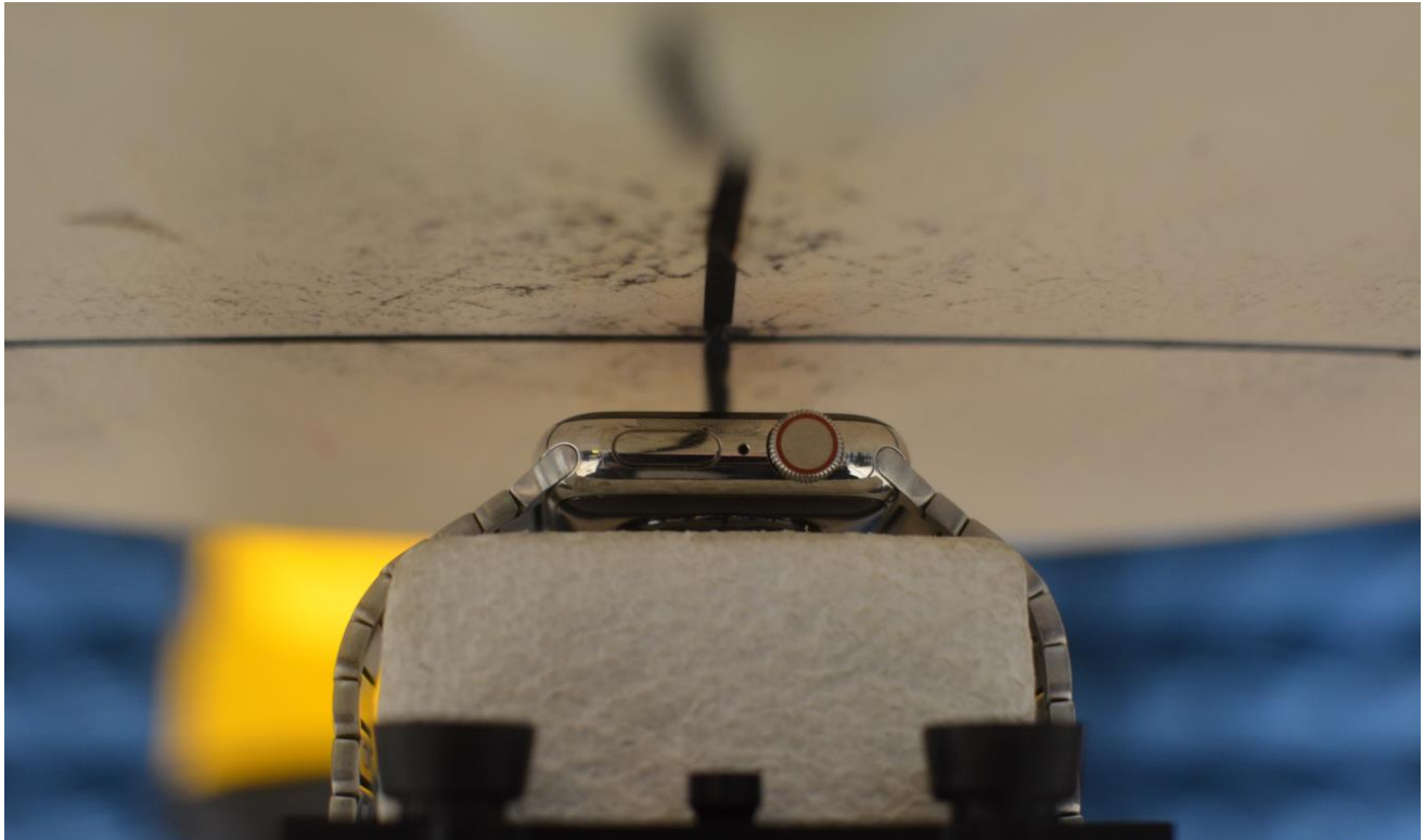
SAR Test Setup Photo 5: Stainless Steel with Metal Links wristband, Front side at 1.0 cm
