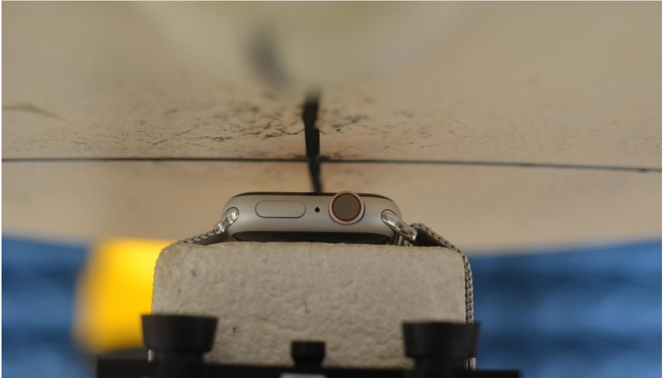
SAR Test Setup Photo 3: Aluminum with Metal Loop wristband, Front side at 1.0 cm
