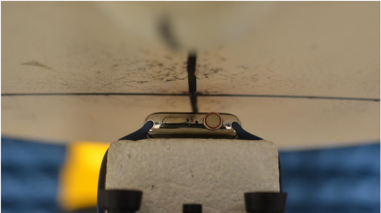
SAR Test Setup Photo 4: Stainless Steel with Sport wristband, Front side at 1.0 cm
