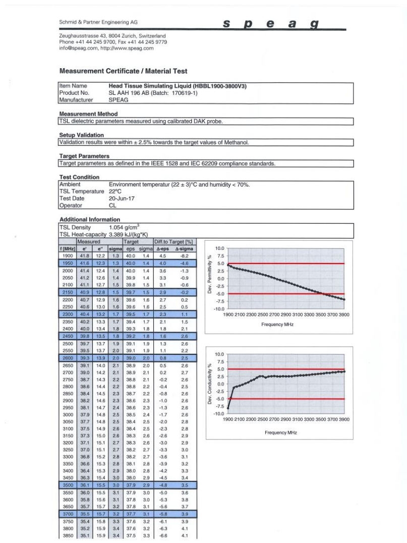
Figure D-2 2.4-2.6 GHz Head Tissue Equivalent Matter
